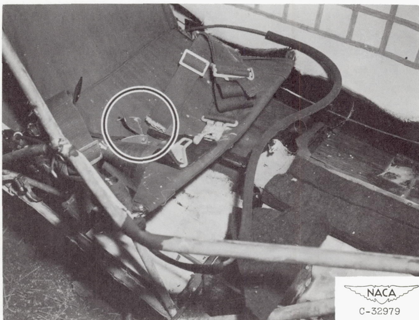
(b) Failure of 2-inch seat belt during crash.
