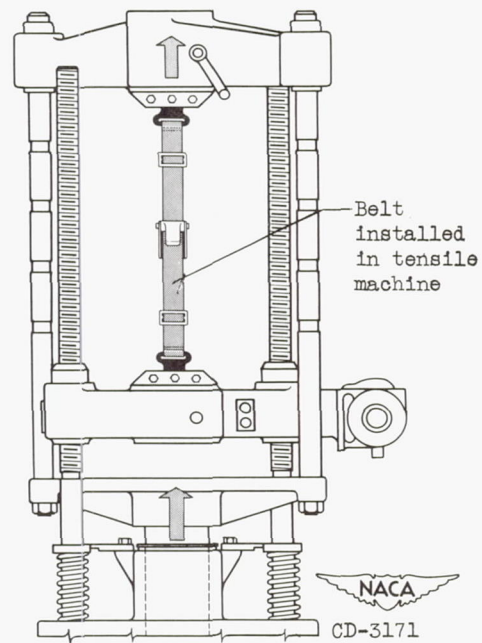
(a) Light-airplane seat belt (new). Width, 2 inches; Air Associates model number, M-5100; rated strength of assembly, 1500 pounds.
