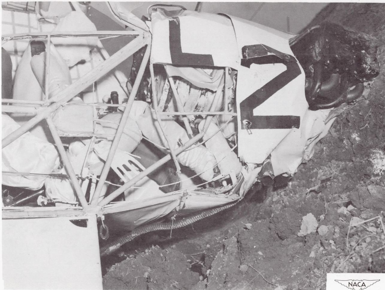
Figure 16. - Concluded. Position of parachute dummy in front seat of airplane after crash.
