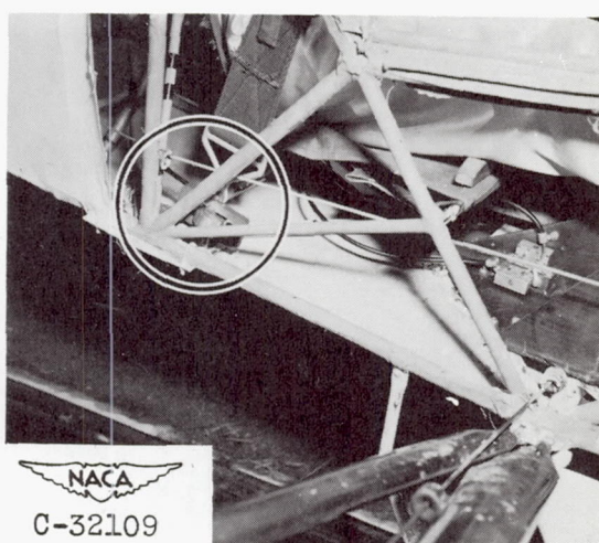
(i) Seat-belt tensiometers at rear seat.
