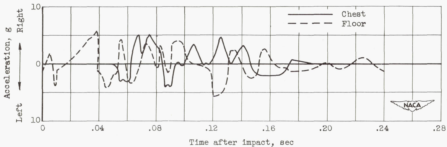
Figure 10. - Time history of lateral acceleration as measured on chest of rear dummy and fuselage floor at rear seat in 42-mph crash.
