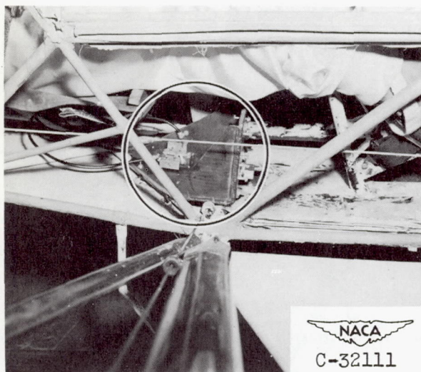
(g) Accelerometers installed on fuselage floor at rear seat in 60-mph crash.
