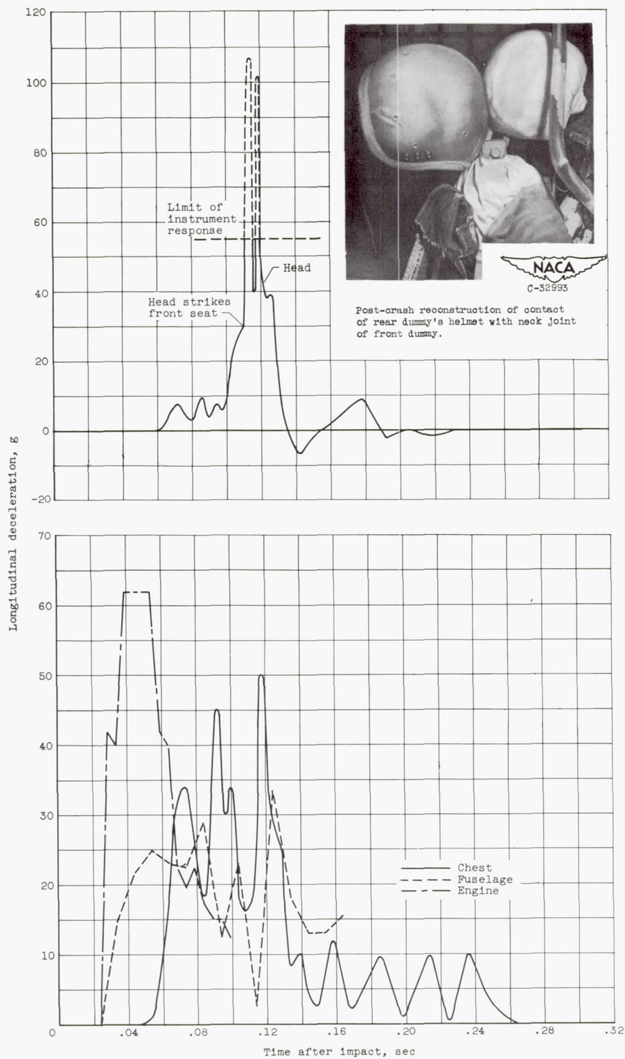
Figure 6. - Longitudinal deceleration of engine, fuselage floor at rear seat, and chest and head of rear dummy.
