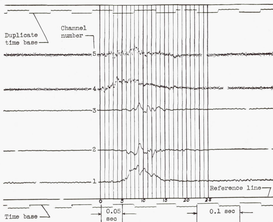
(j) Oscillograph records from 47-mph crash.
