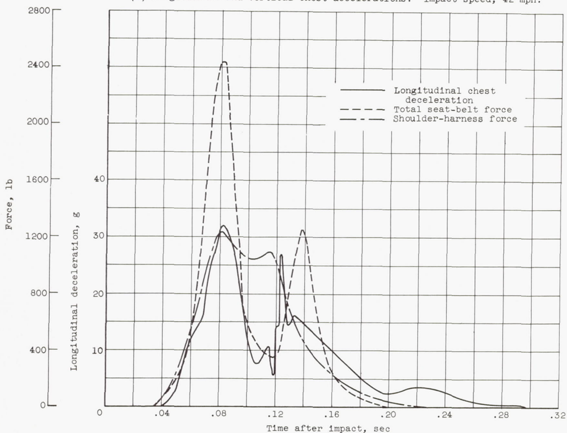
(b) Longitudinal chest deceleration and restraining forces. Impact speed, 42 mph.
