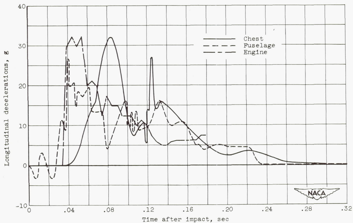
Figure 6. - Concluded. Longitudinal deceleration of engine, fuselage floor at rear seat, and chest and head of rear dummy.
