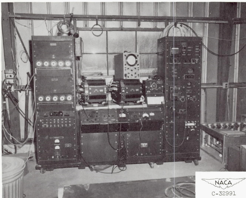
(c) Ten-channel telemetry receiving and recording station.
