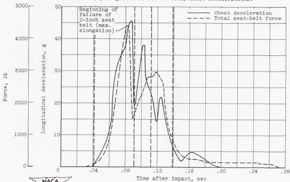
(d) Longitudinal chest deceleration and total seat-belt force.
