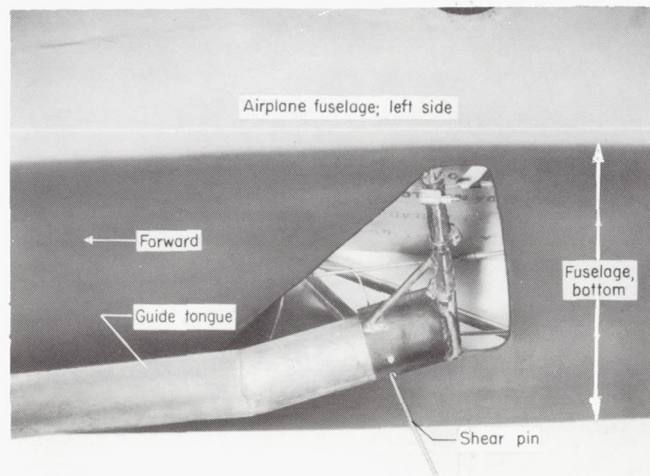
(d) Attachment of tongue to fuselage, showing shear-pin location.
