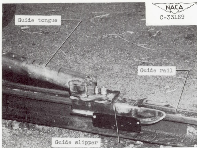
(b) Guide slipper and guide tongue assembly installed on guide rail.
