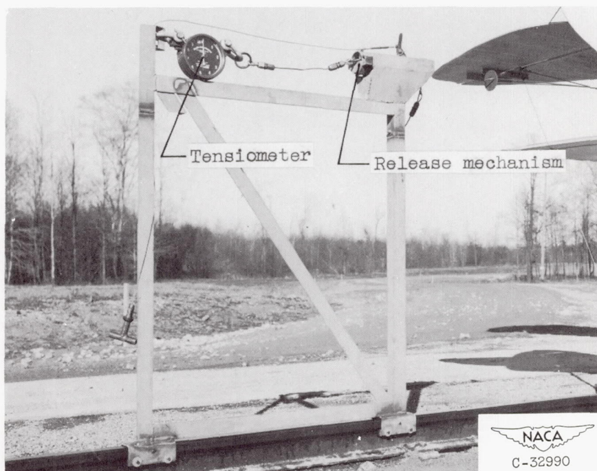
(f) Anchor pier installed on guide rail to retain airplane before release.
