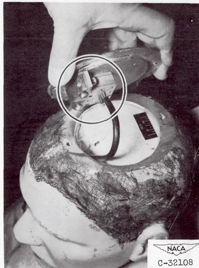
(f) Accelerometer installed in head of rear dummy.
