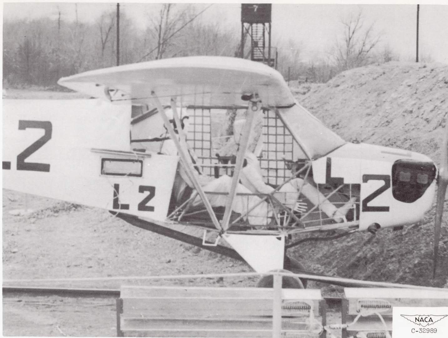
Figure 3. - Typical installation of anthropomorphic and parachute dummies in airplane.
