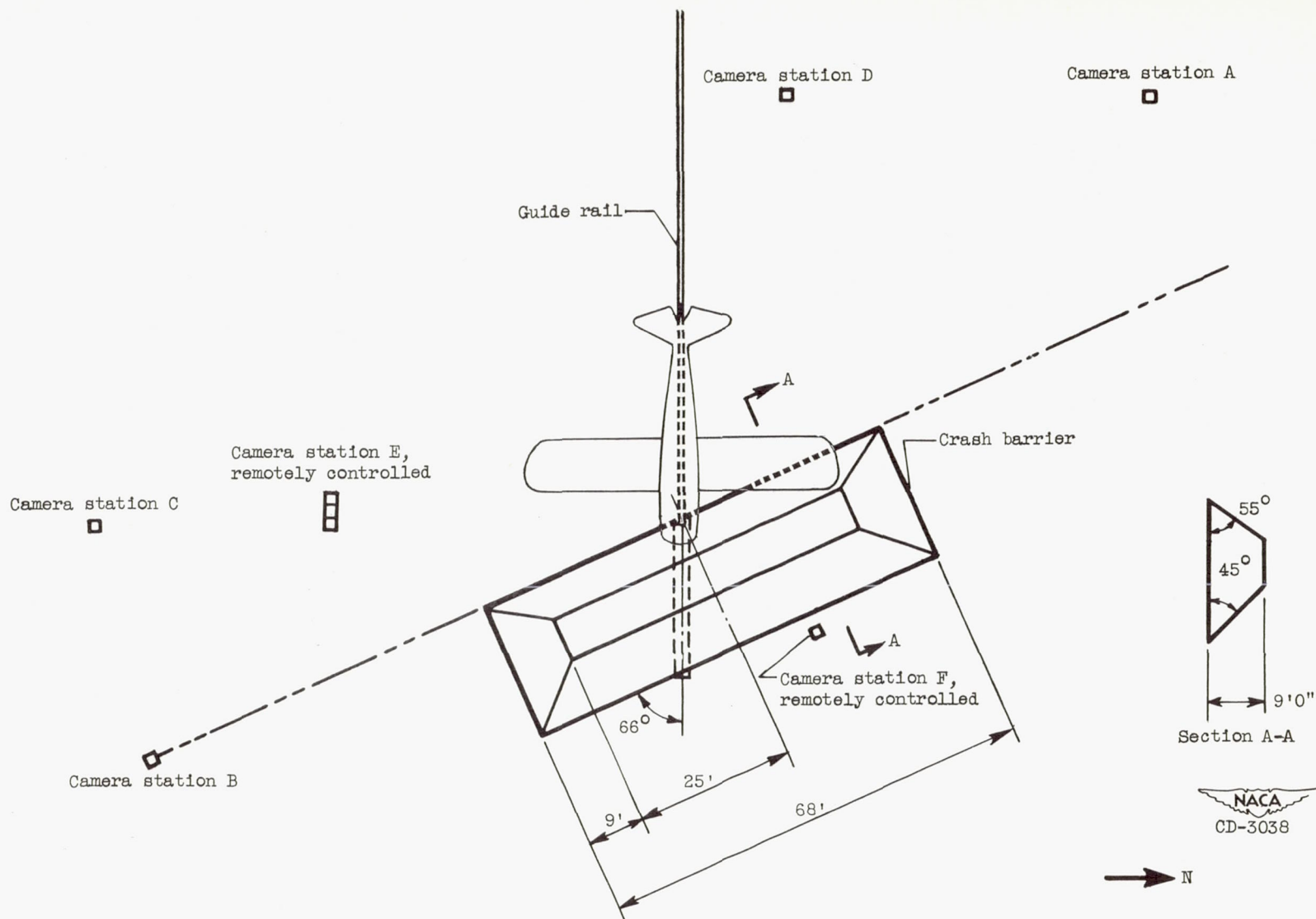
Figure 2. - Plan view of crash area for conducting light-airplane crash investigation.
