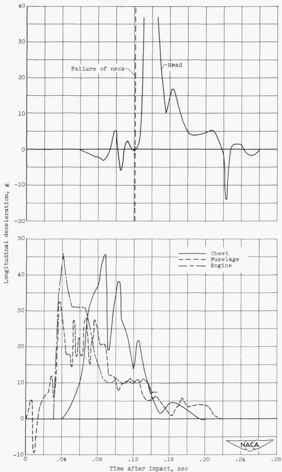
Figure 6. - Continued. Longitudinal deceleration of engine, fuselage floor at rear seat, and chest and head of rear dummy.
