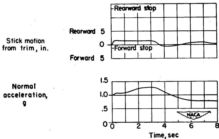
(b) Single-rotor helicopter, level flight, tail on at 0^\circ .
