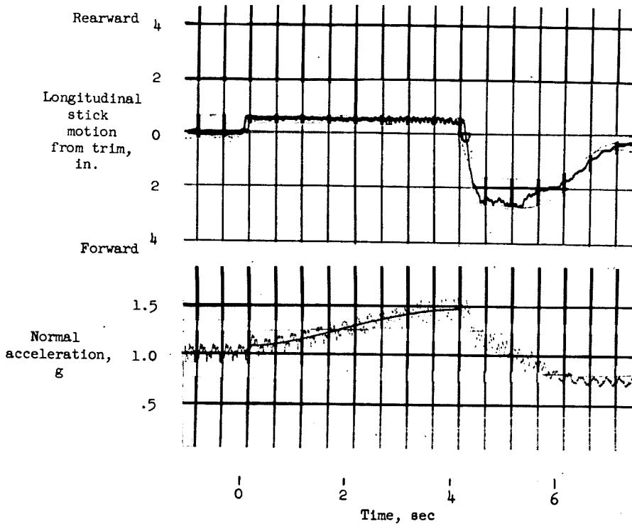
(c) Tandem-rotor helicopter, forward center of gravity, level flight.
