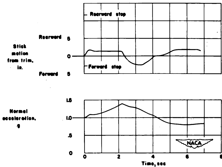
(a) Single-rotor helicopter, level flight, tail off.
