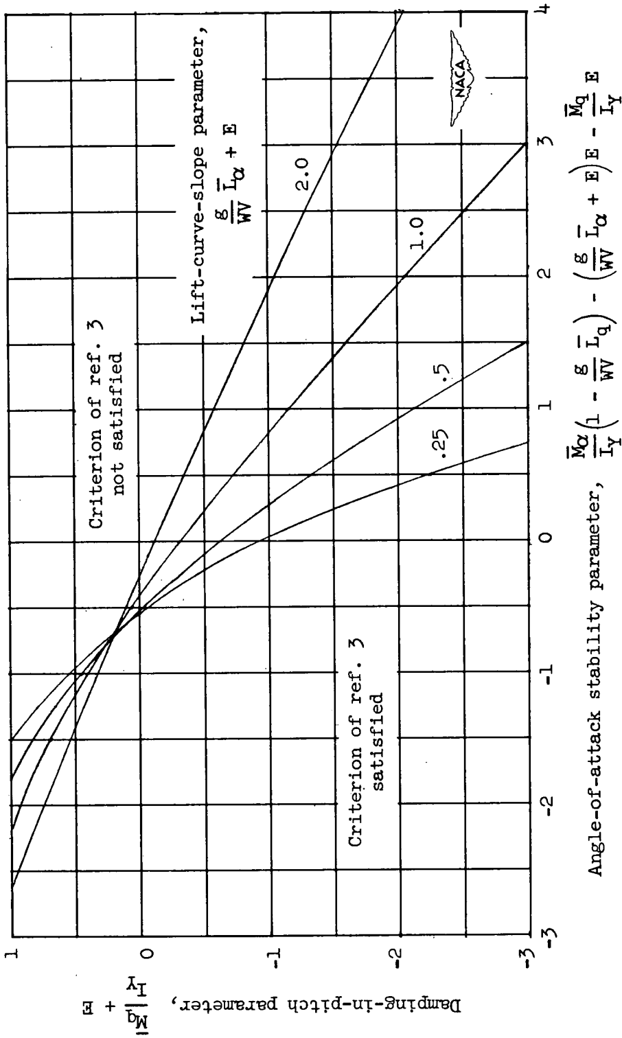
Figure 2.- Damping-in-pitch parameter plotted against angle-of-attack stability parameter for various values of lift-curve-slope parameter
