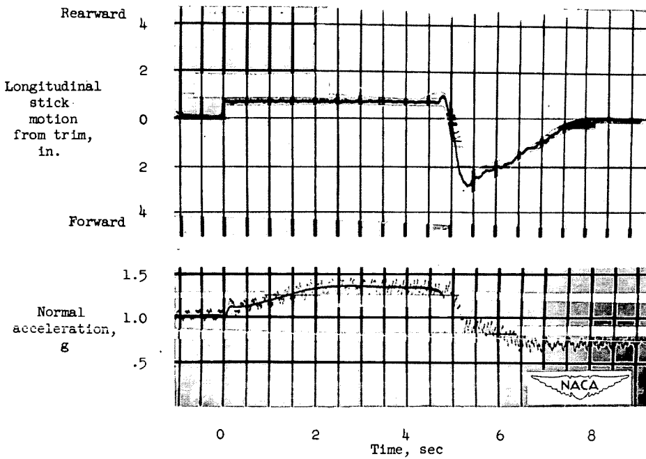
(d) Tandem-rotor helicopter, forward center of gravity, partial-power descent.
