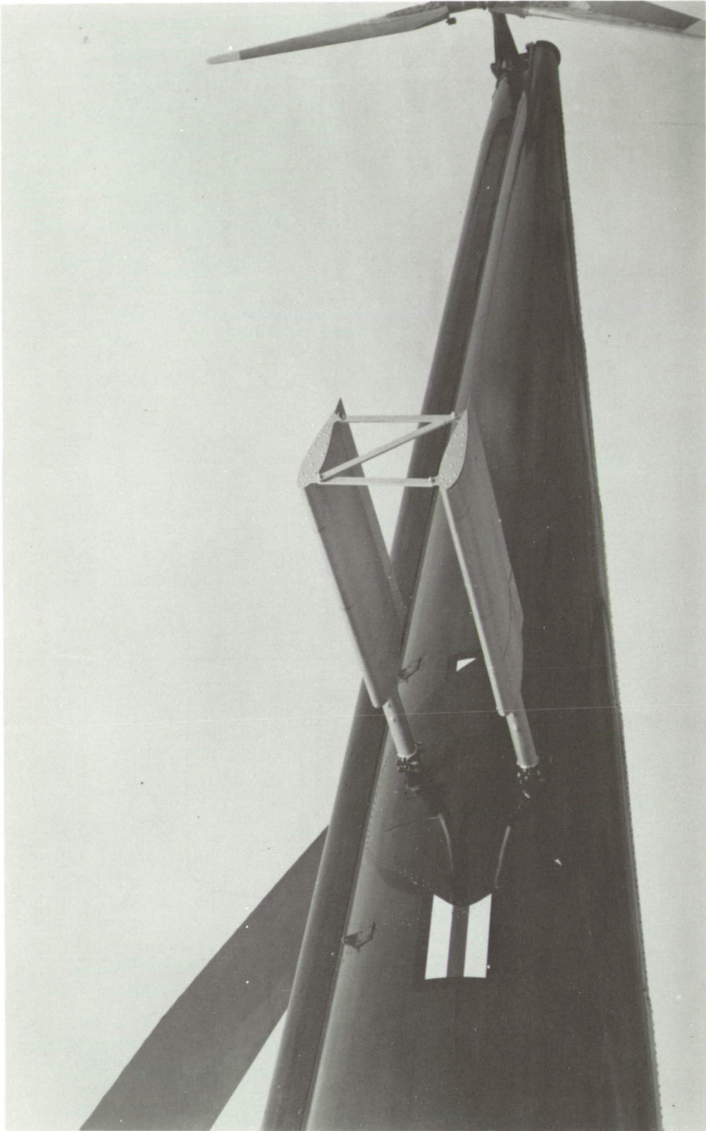
Figure 6.- Biplane tail surface used to vary angle-of-attack stability of single-rotor helicopter.
