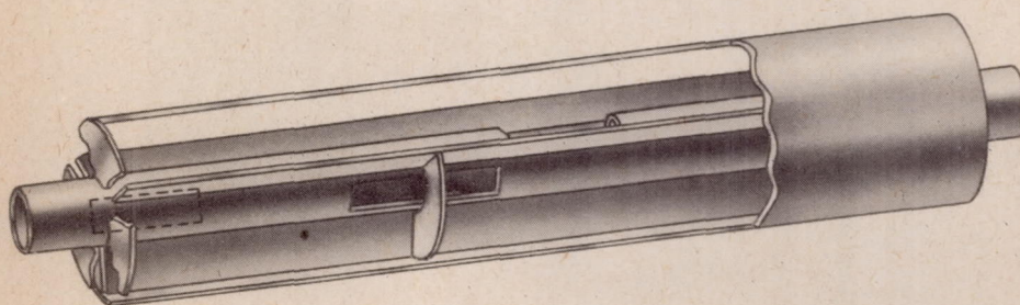
(f) Combination of several quarter-wave resonators (muffler 74).
