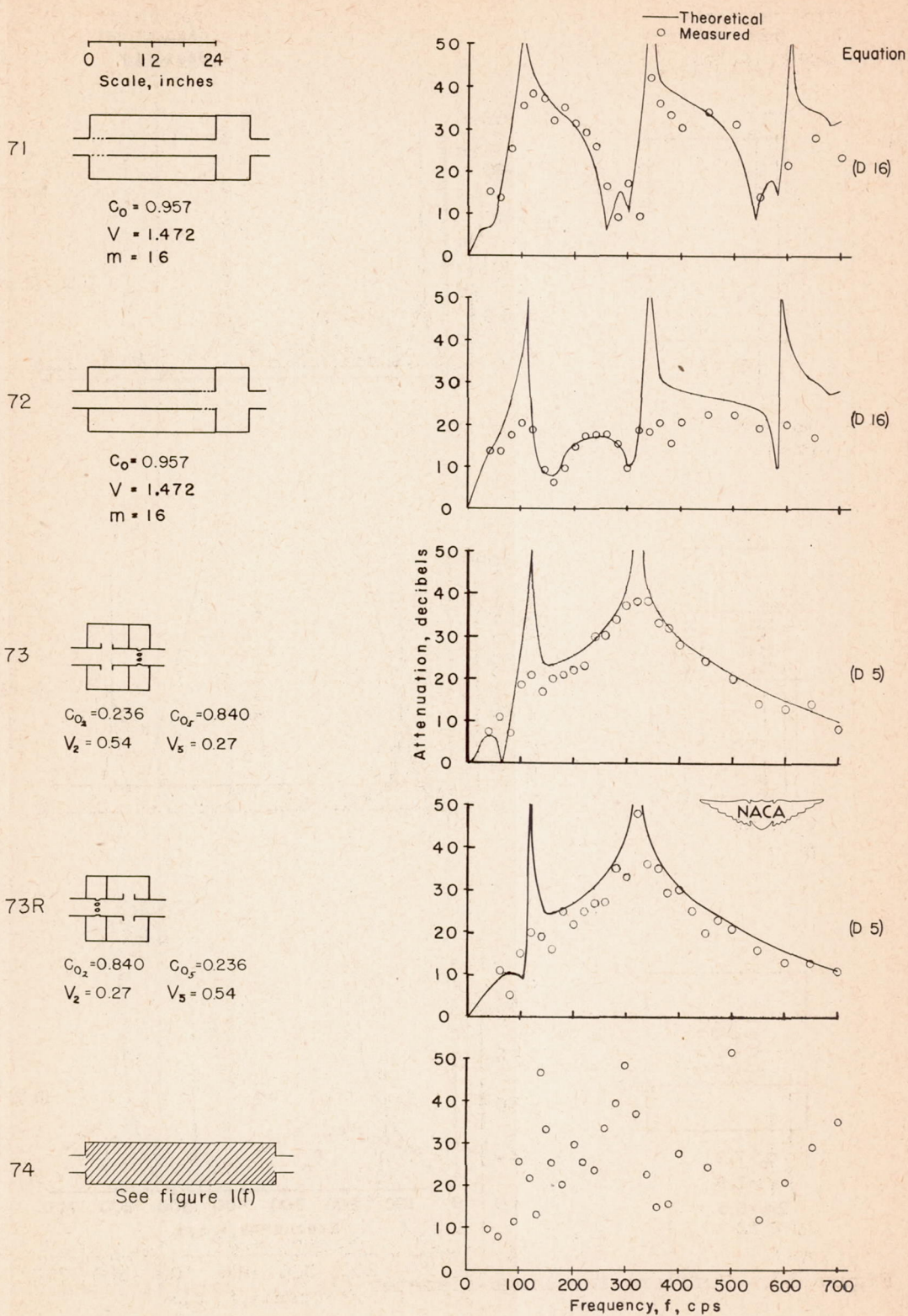
Figure 16.- Combination mufflers.
