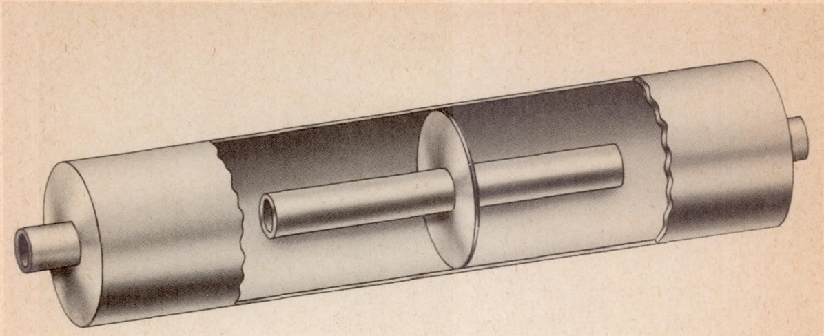
(a) Double expansion chamber with internal connecting tube (muffler 19).
