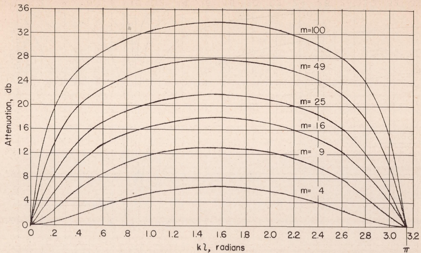
Figure 19.- Expansion-chamber design curves.
