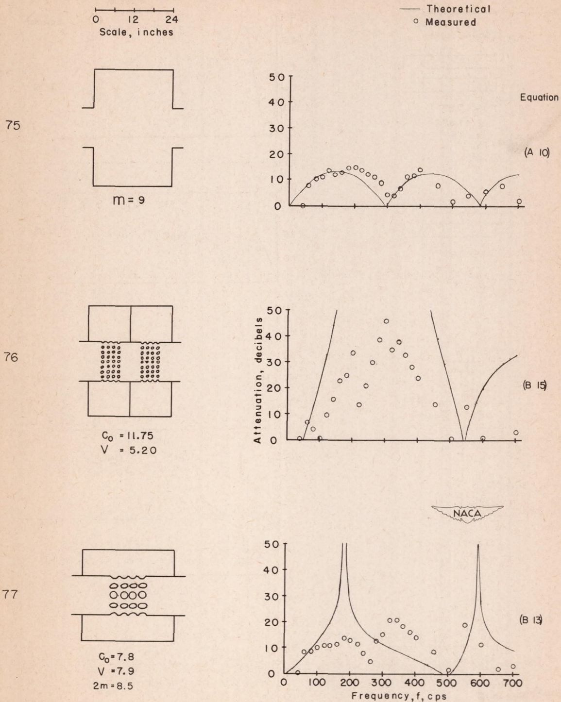
Figure 17.- Mufflers for large-diameter (12 in.) exhaust pipes.
