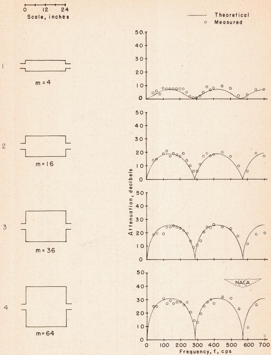
(a) Effect of expansion ratio m .
