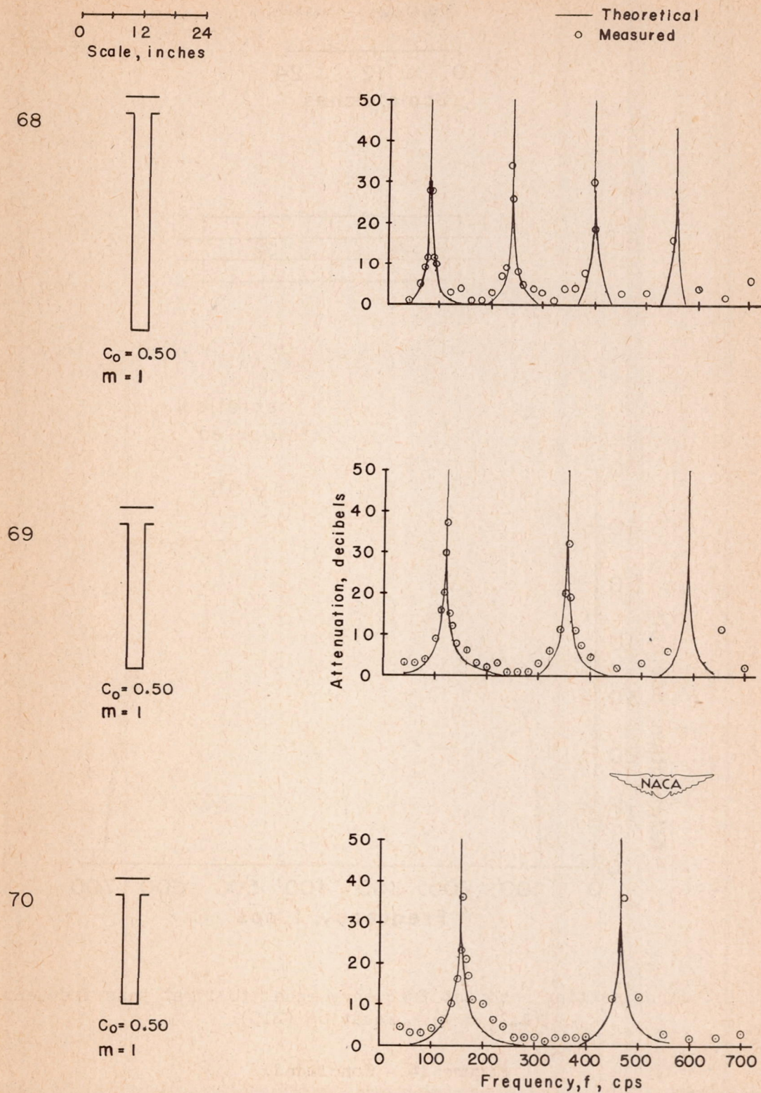
Figure 15.- Side-branch tubes with same diameter as exhaust pipe. Equation (B13).
