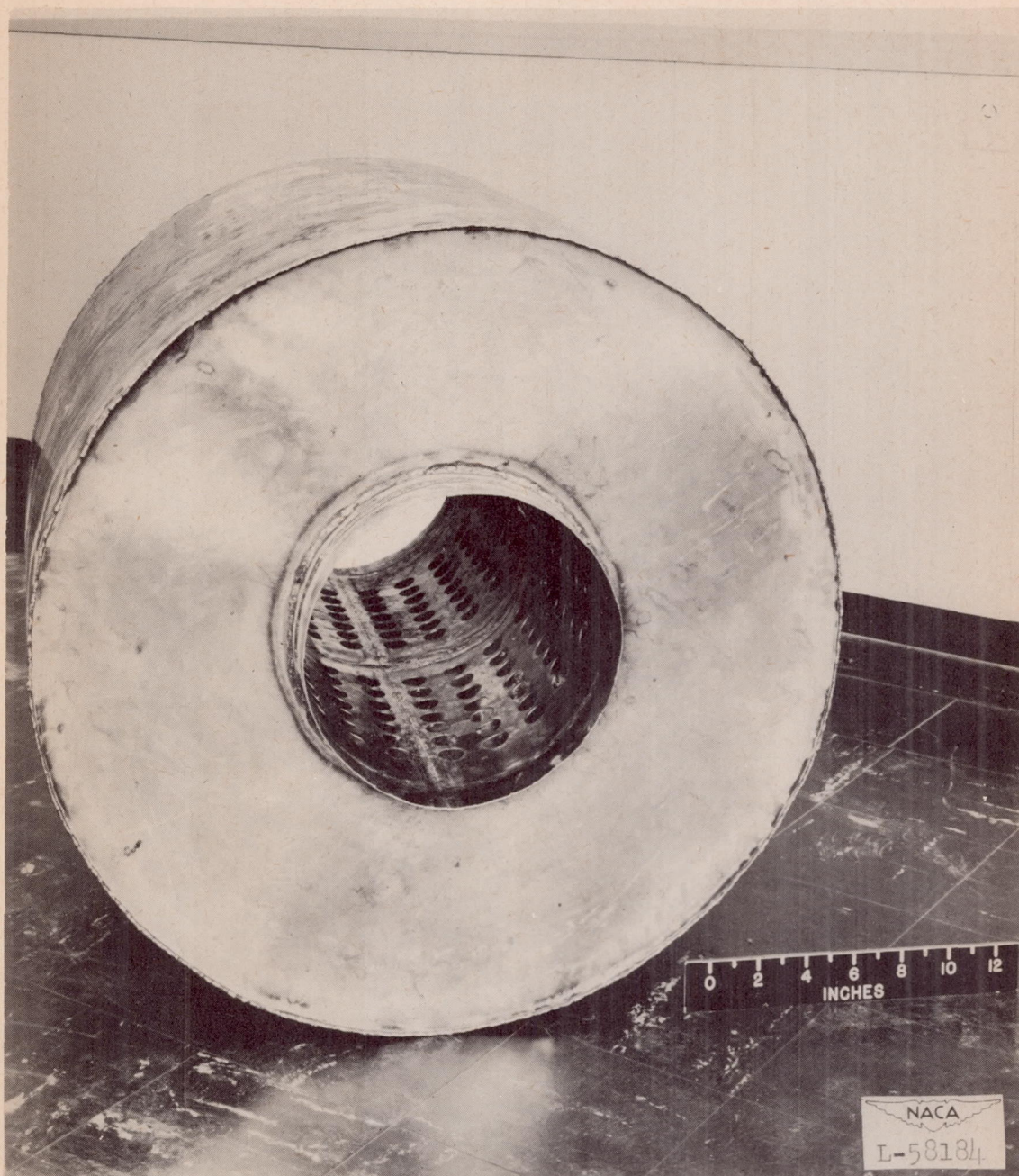
(b) Central-tube diameter, 12 inches; muffler 74.
