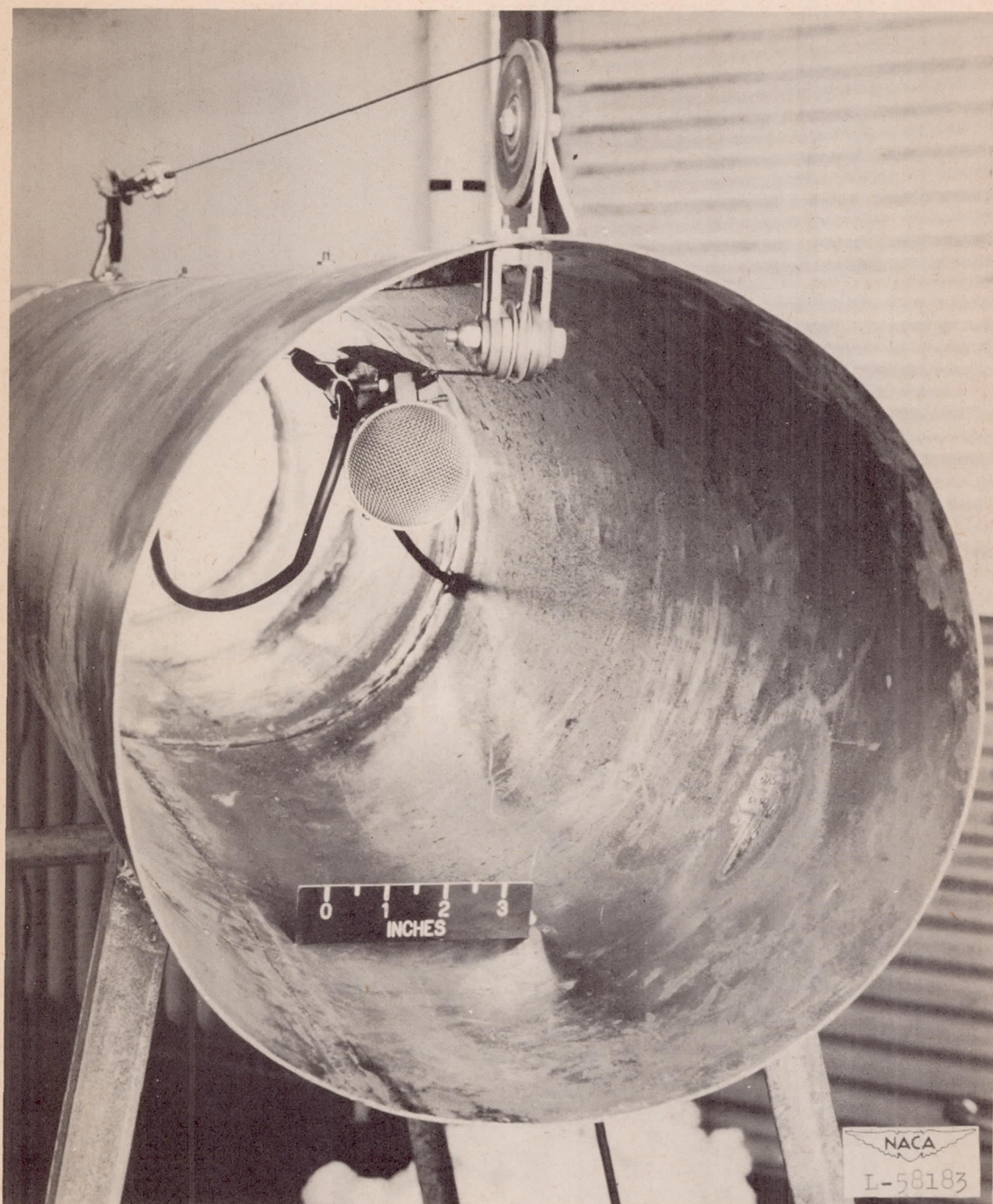
Figure 6.- Movable-microphone arrangement in the 12-inch tail pipe.
