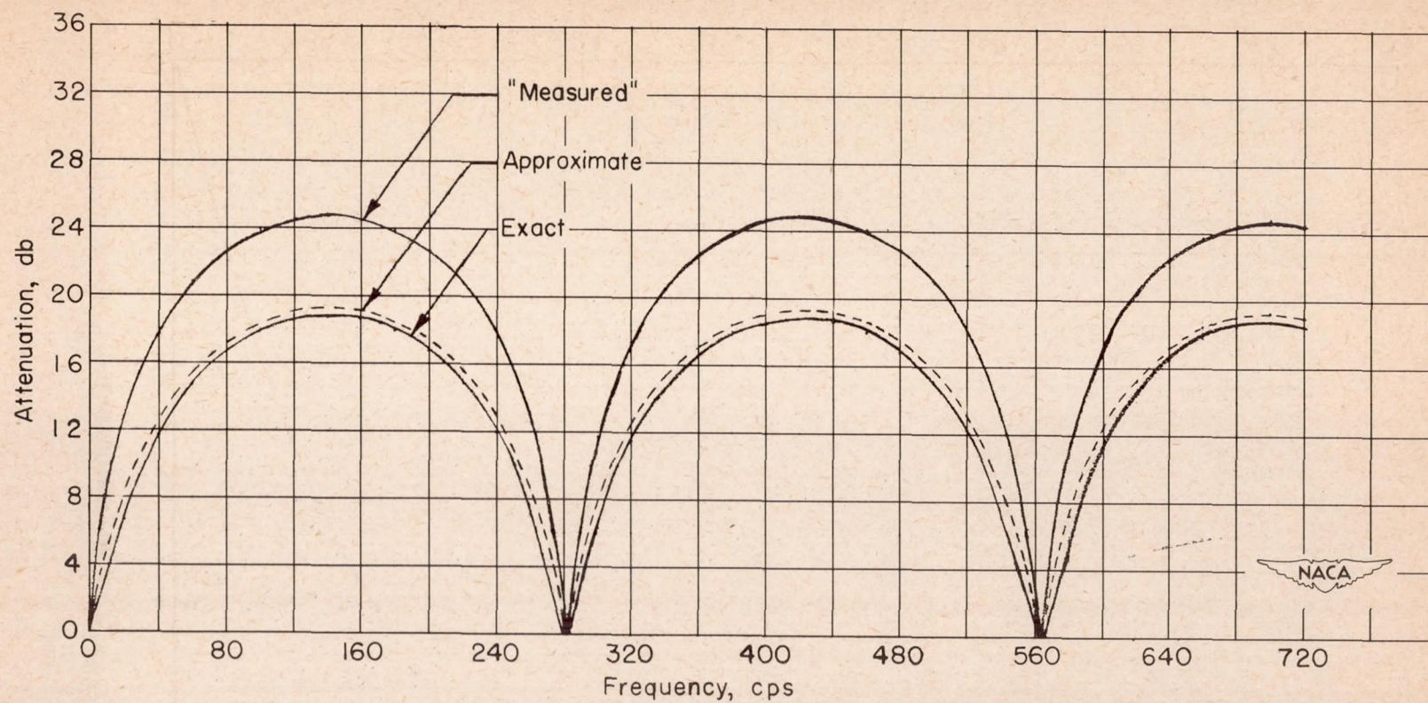
Figure 8.- Computed comparison of exact and approximately corrected attenuation curves for a single expansion chamber.
