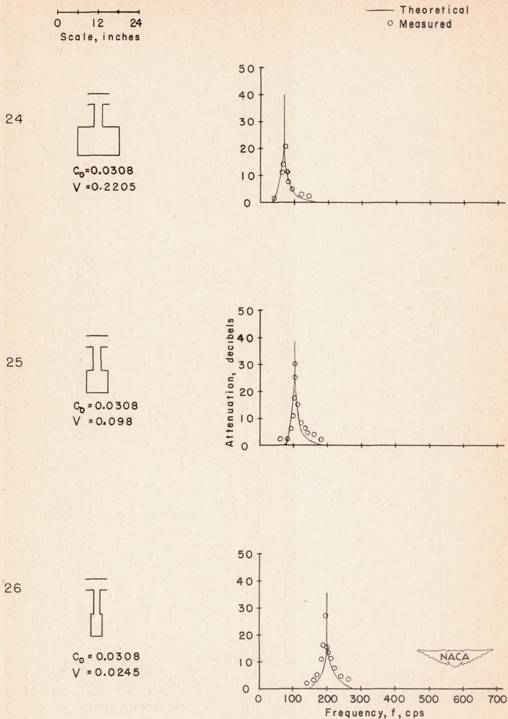
(a) Effect of volume V . Equation (B4).
