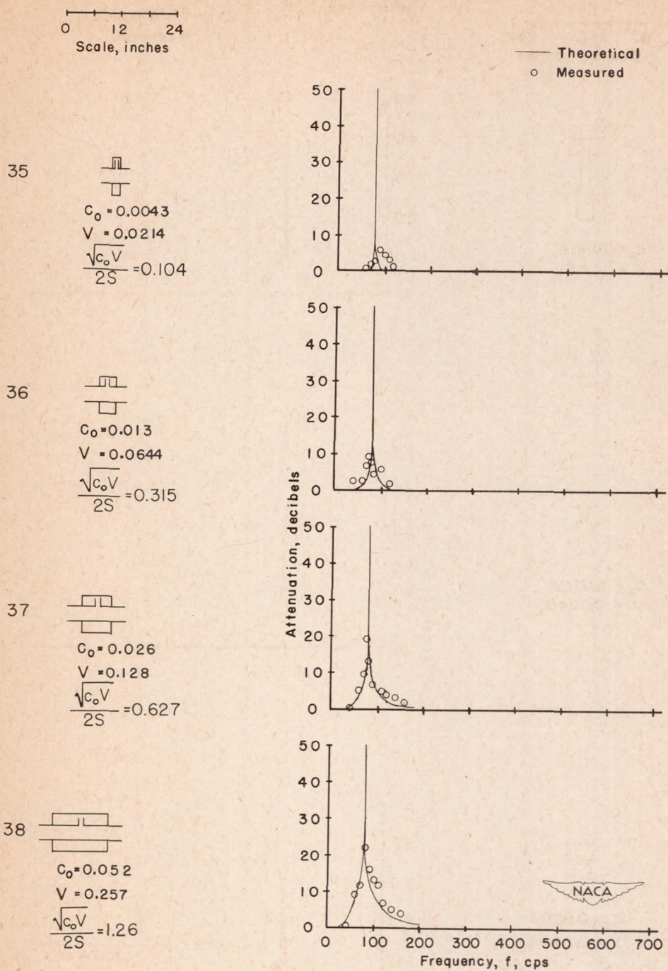
(a) Effect of varying \frac{\sqrt{C_0 V}}{2S} with the resonance parameter \sqrt{\frac{C_0}{V}} constant. Equation (B10).
