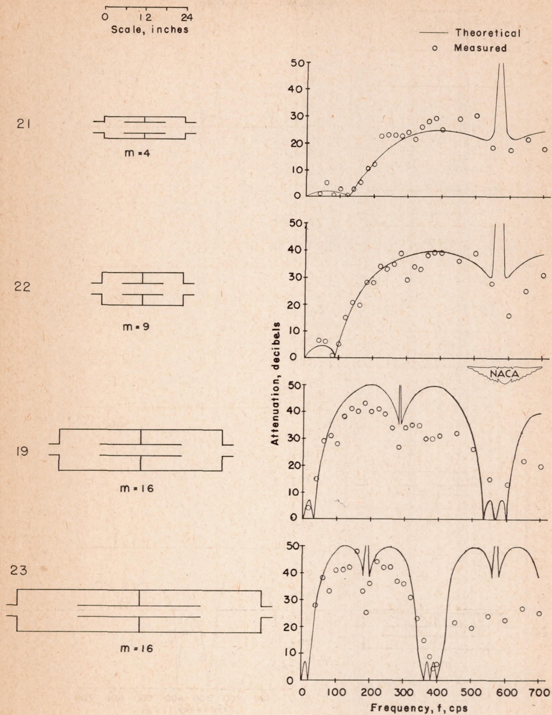
(d) Mufflers with internal connecting tubes equal in length to the individual chamber lengths. Equation (A17).
