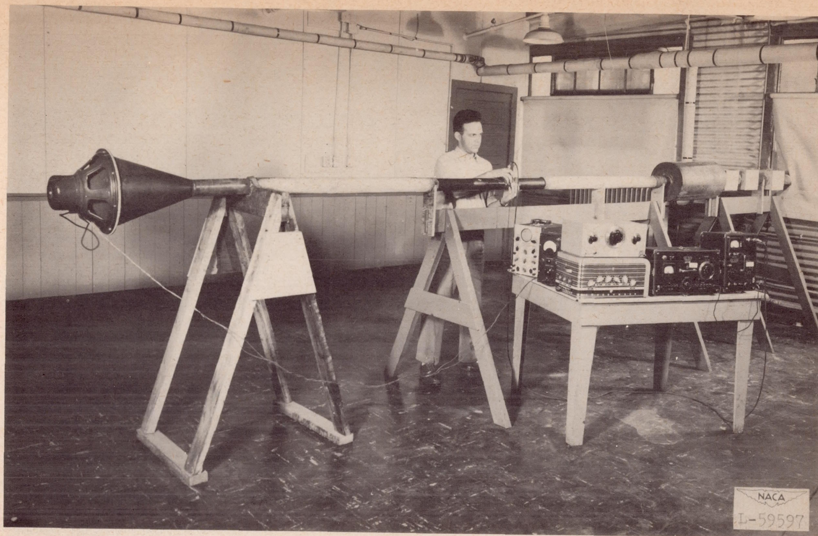
Figure 4.- Apparatus used for testing mufflers designed for a 3-inch exhaust pipe.
