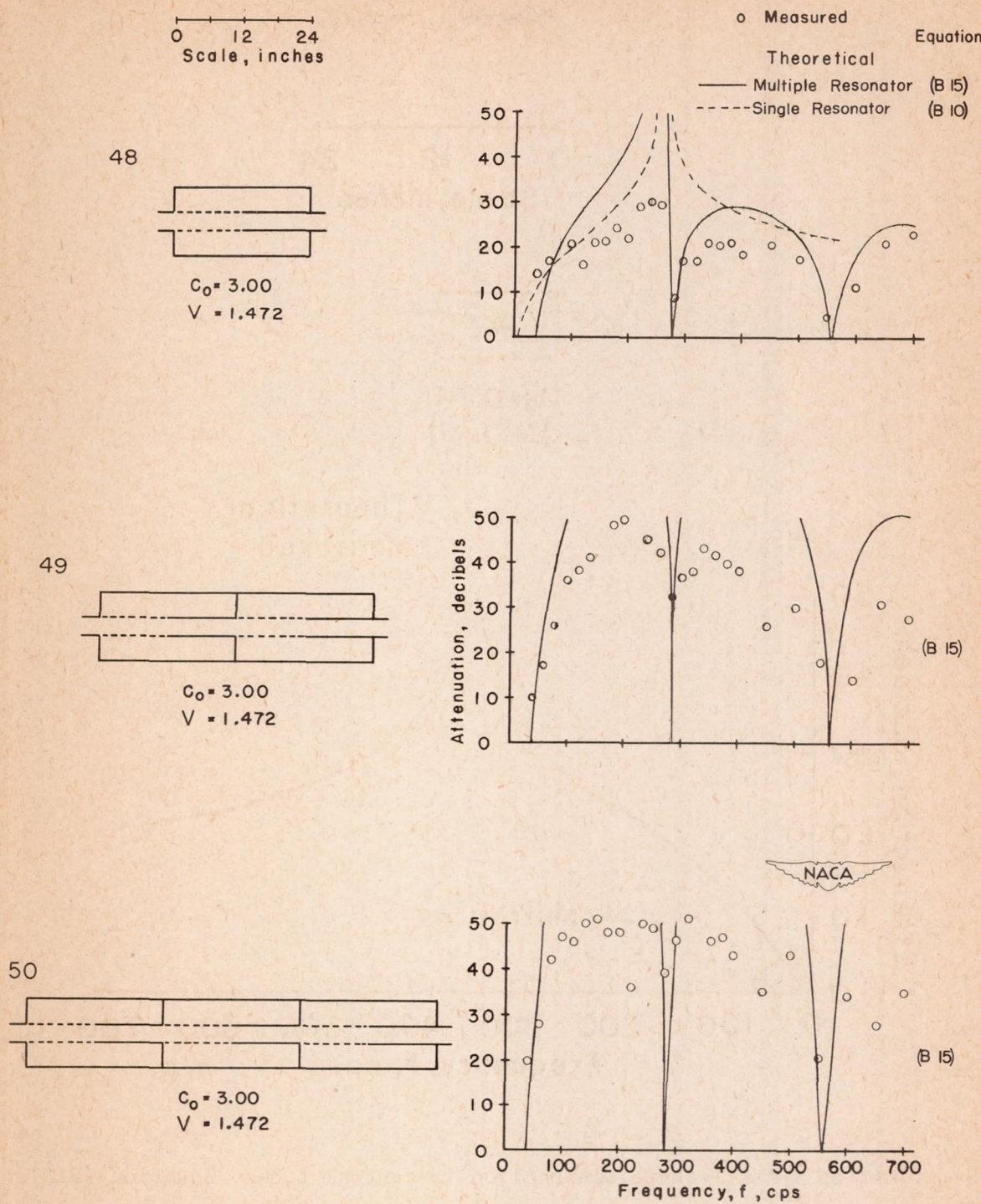
(a) Effect of number of chambers.
