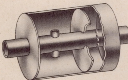
(e) Two resonators tuned to different frequencies (muffler 73).
