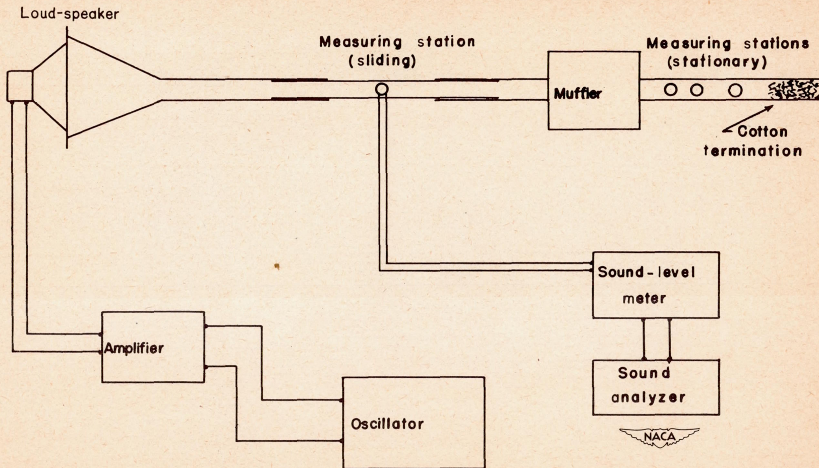
Figure 3.- Schematic diagram of experimental apparatus.
