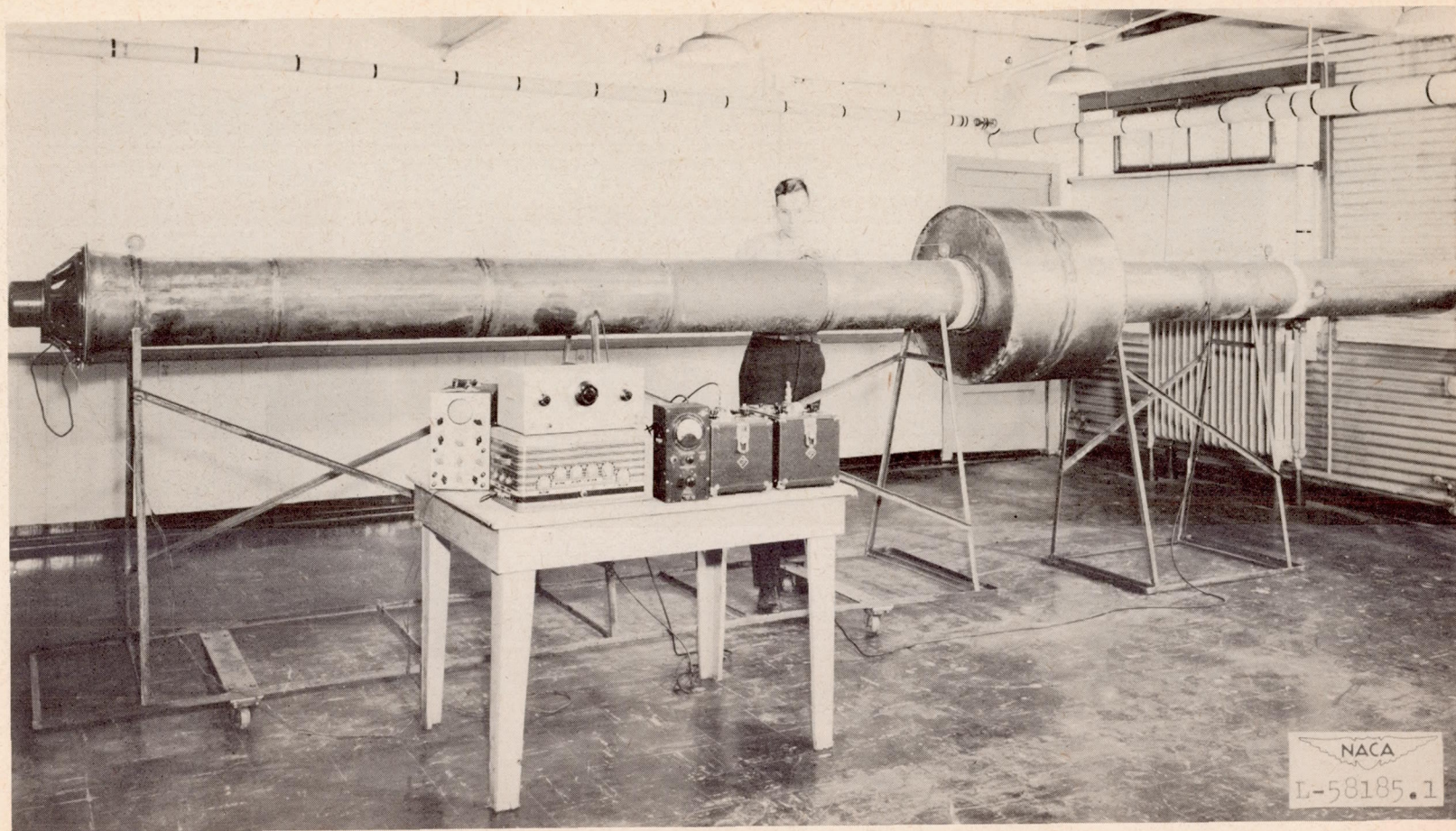
Figure 5.- Apparatus used for testing mufflers designed for a 12-inch exhaust pipe.
