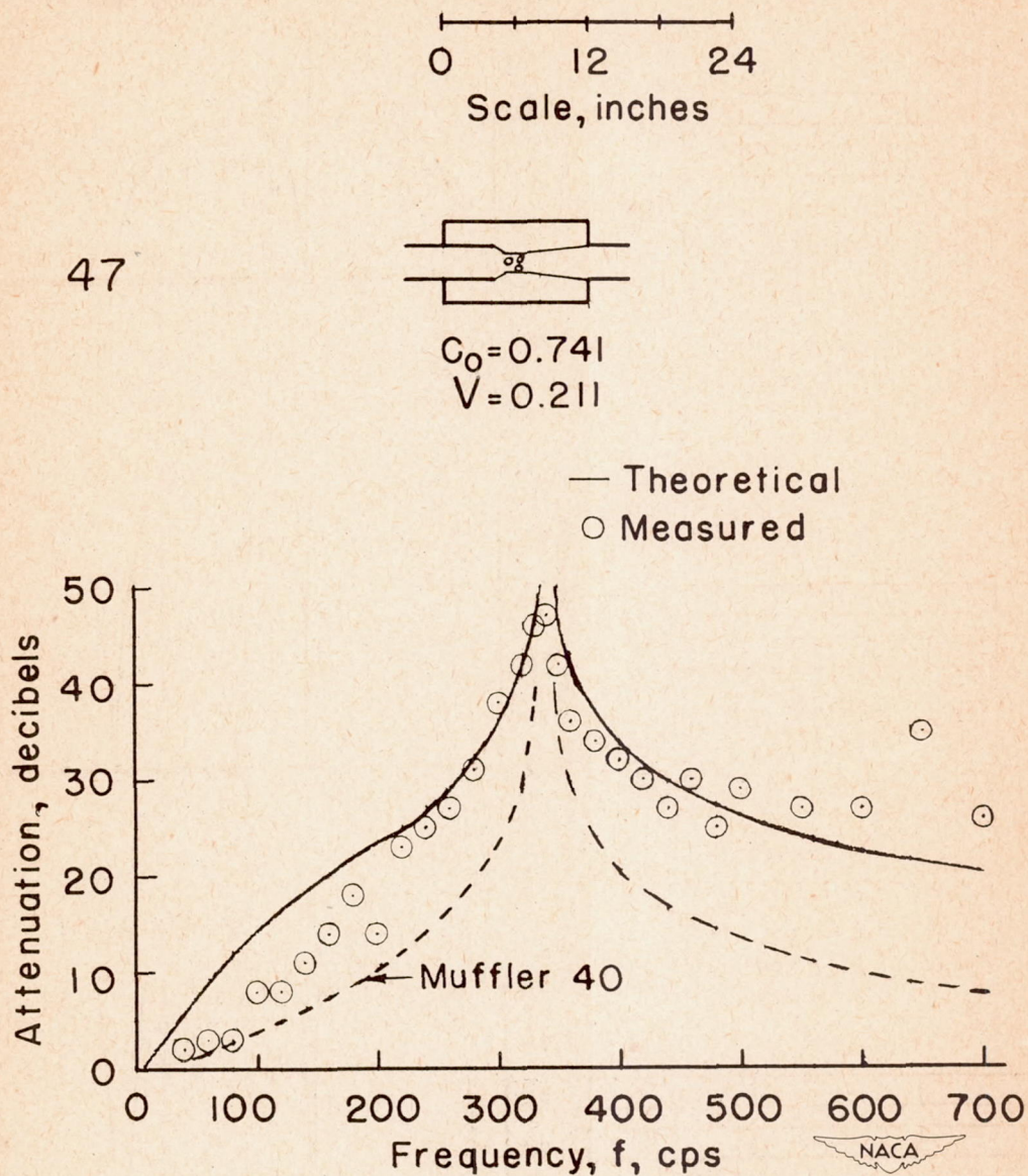
(d) Effect of venturi-shape contraction in central tube. Equation (B10).
