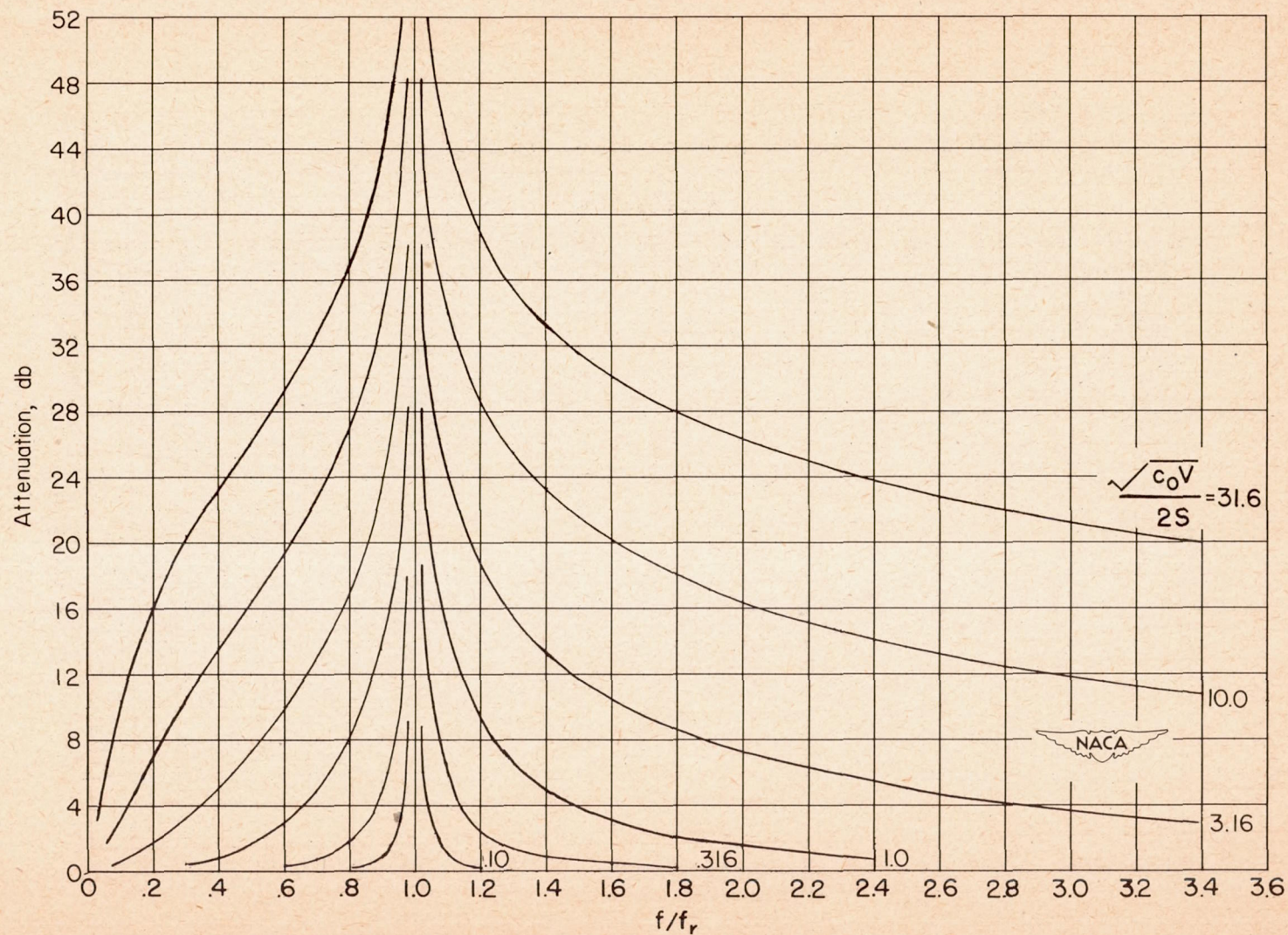
Figure 20.- Single-chamber-resonator design curves.
