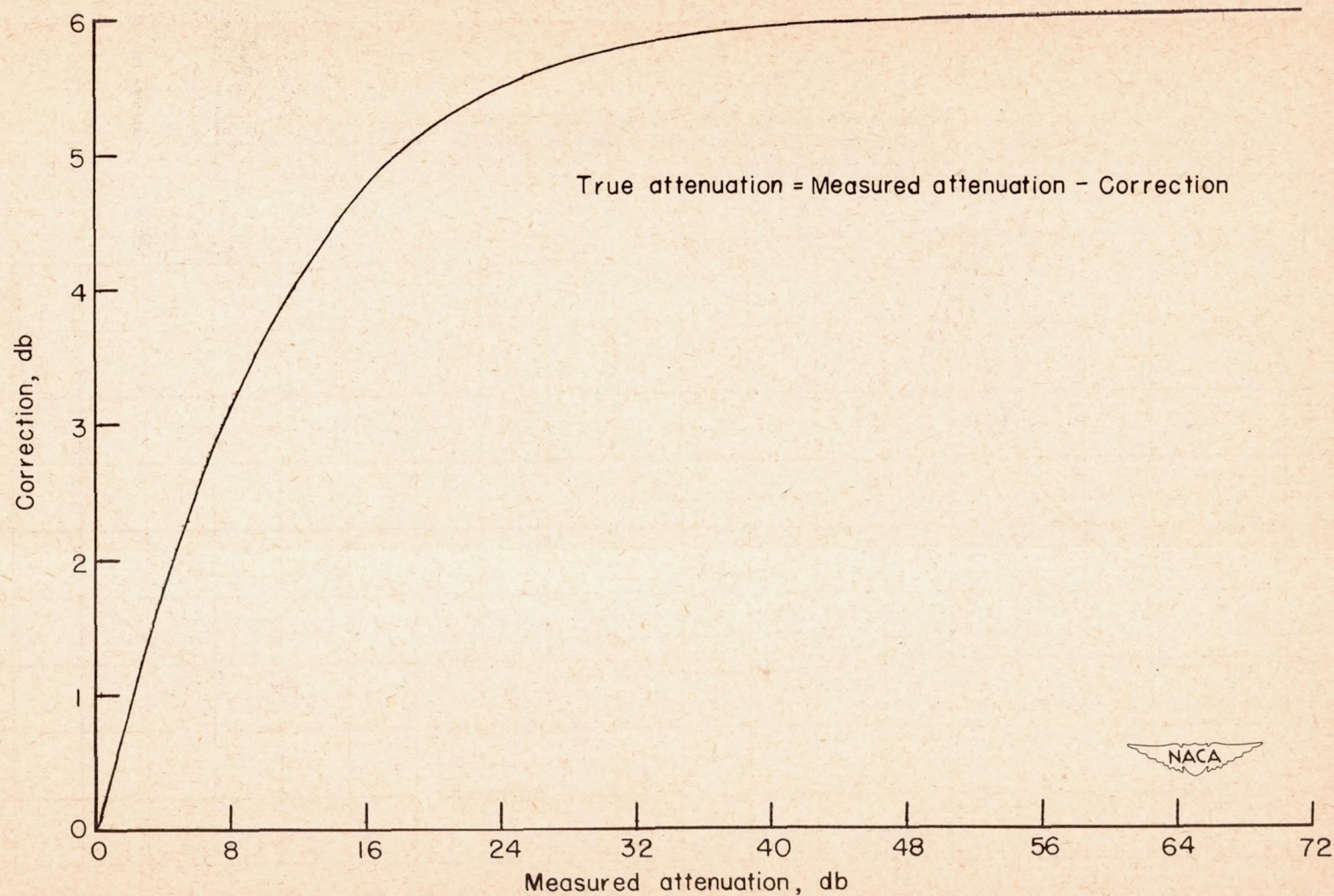
Figure 7.- Corrections to measured attenuation.
