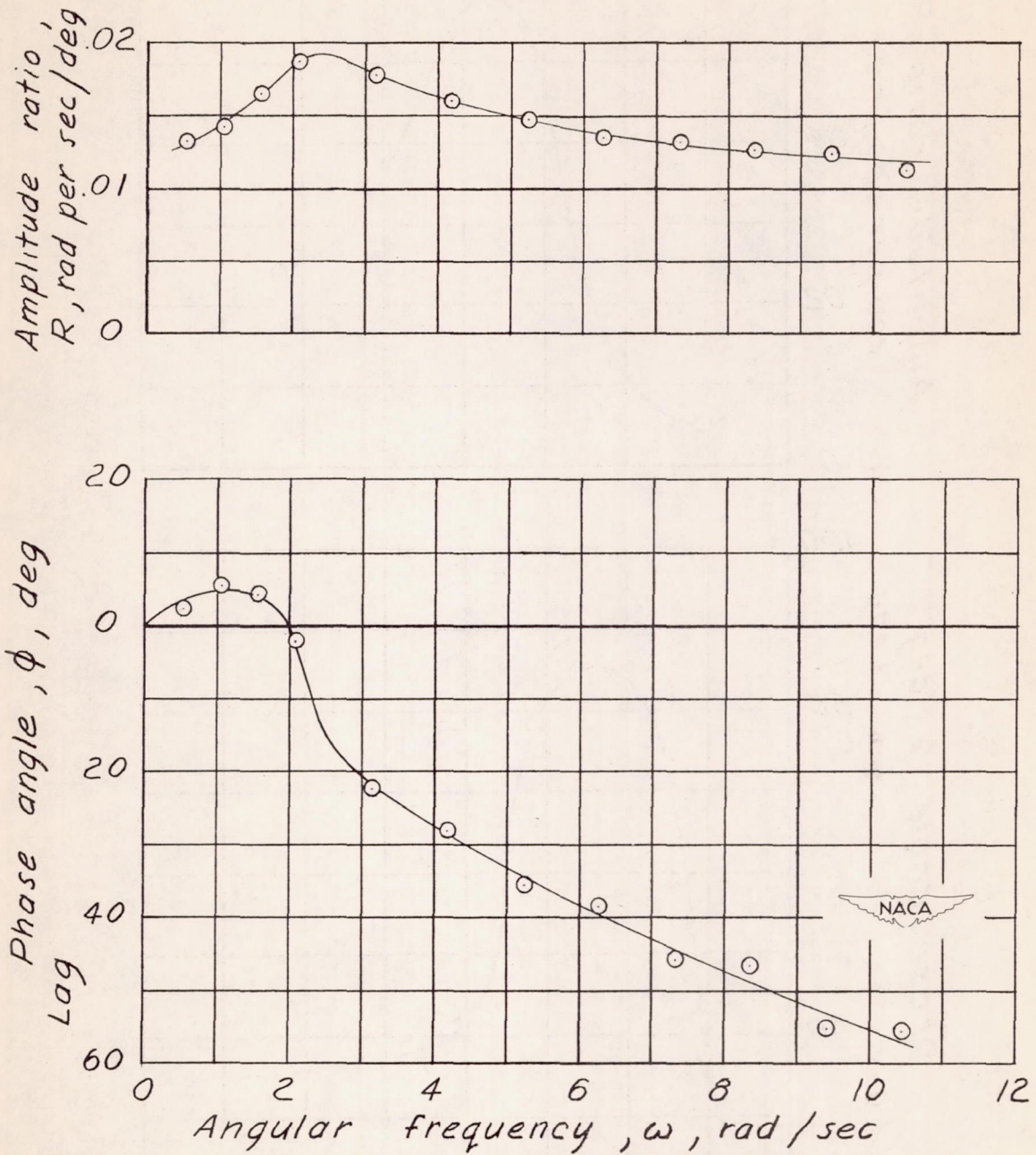
Figure 25.- Frequency response of rolling velocity to aileron deflection of a Douglas DC-3 airplane in the clean condition at an indicated airspeed of 160 mph.
