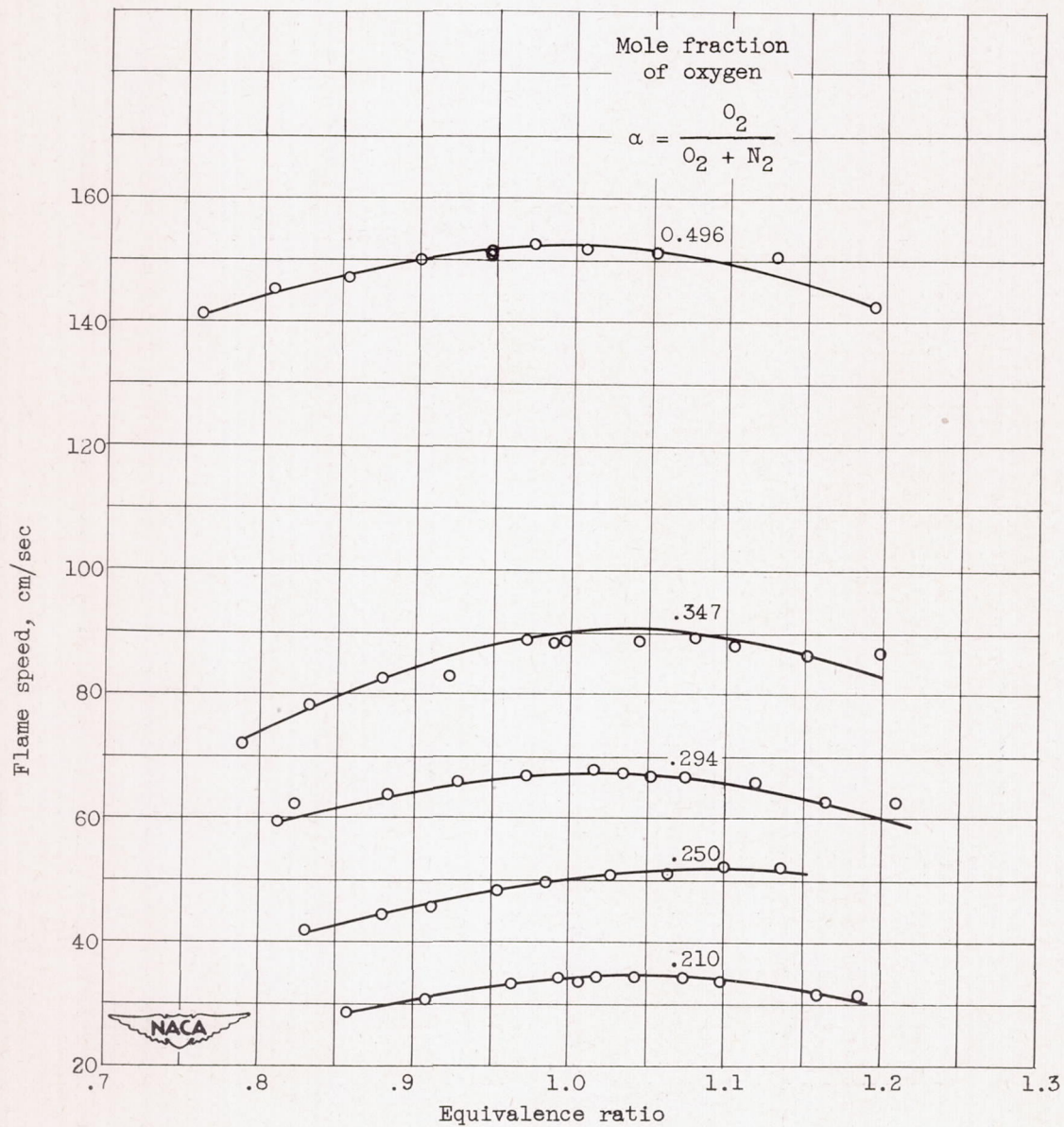
Figure 3. - Flame speeds of 2,2,4-trimethylpentane-oxygen-nitrogen mixtures.
