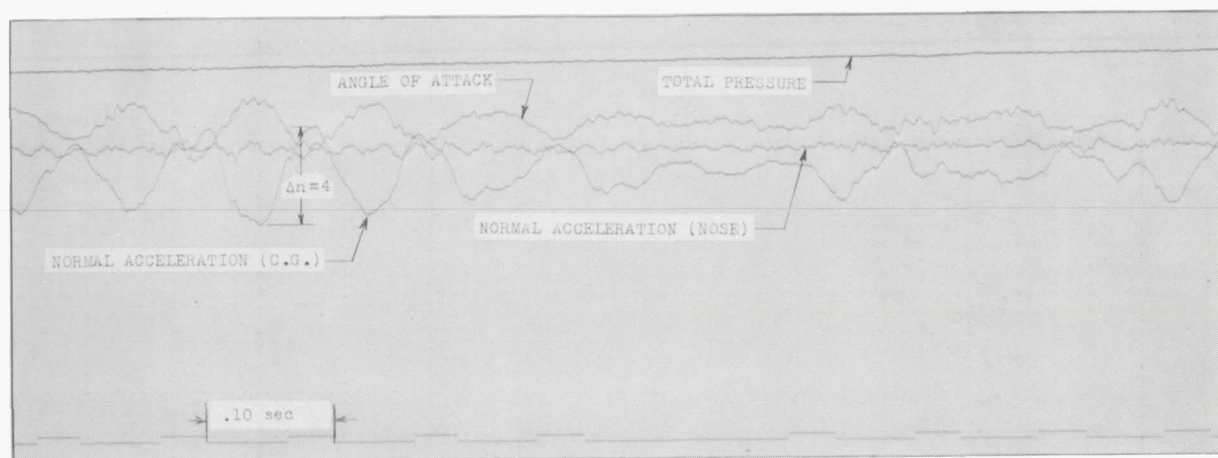
(b) Rough air at M = 0.90 ; altitude, 2,700 feet.
