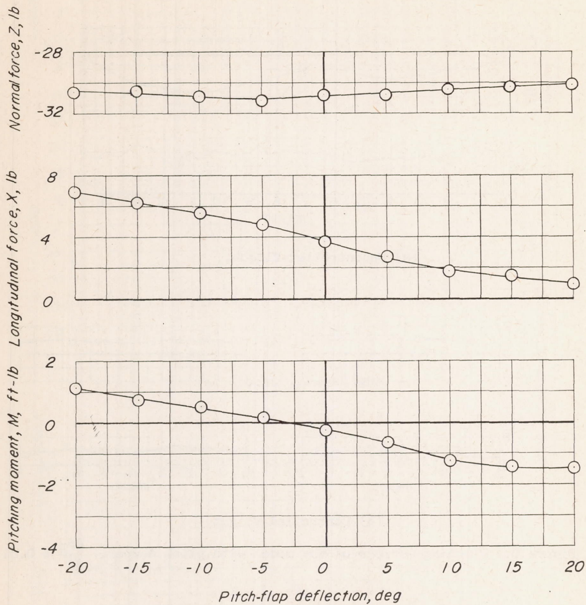
Figure 9.- Pitch control effectiveness from force tests of model.
