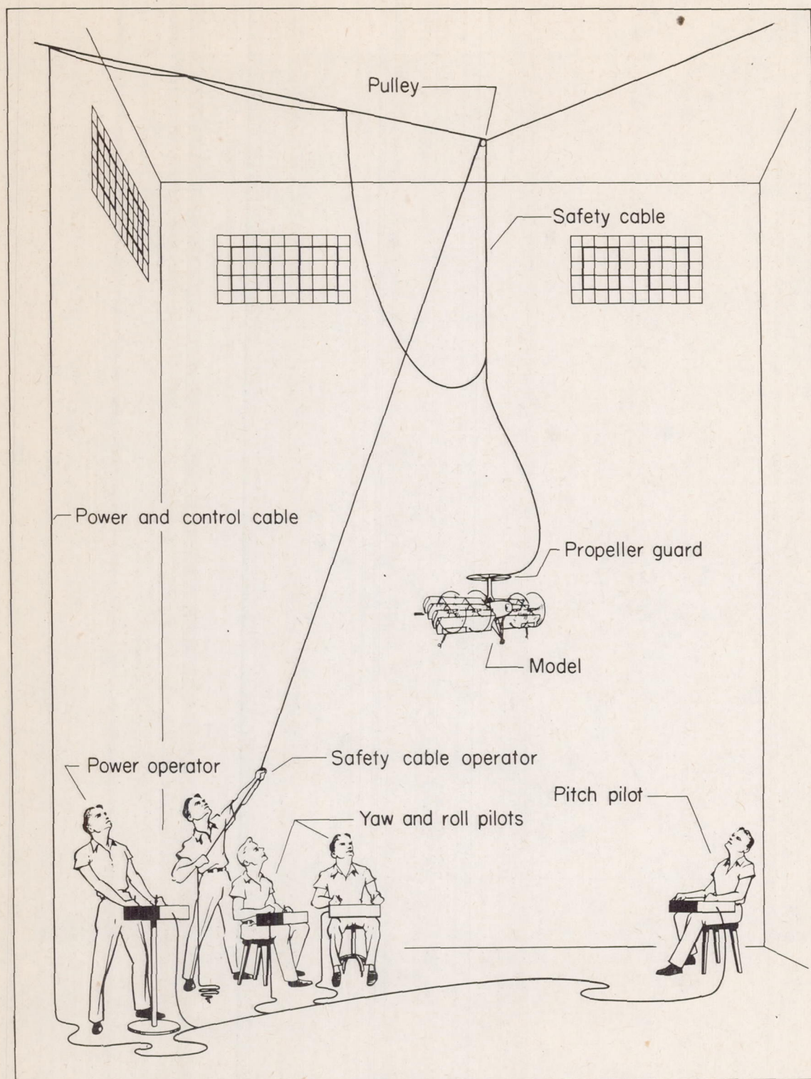
Figure 5.- Test setups used in flight testing hovering models.
