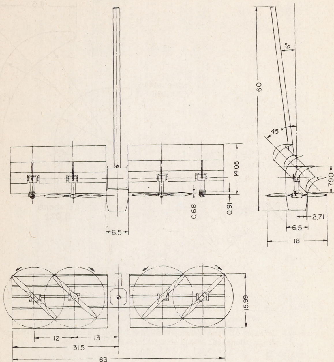
Figure 3.- Three-view sketch of cascade-wing model. All dimensions are in inches.
