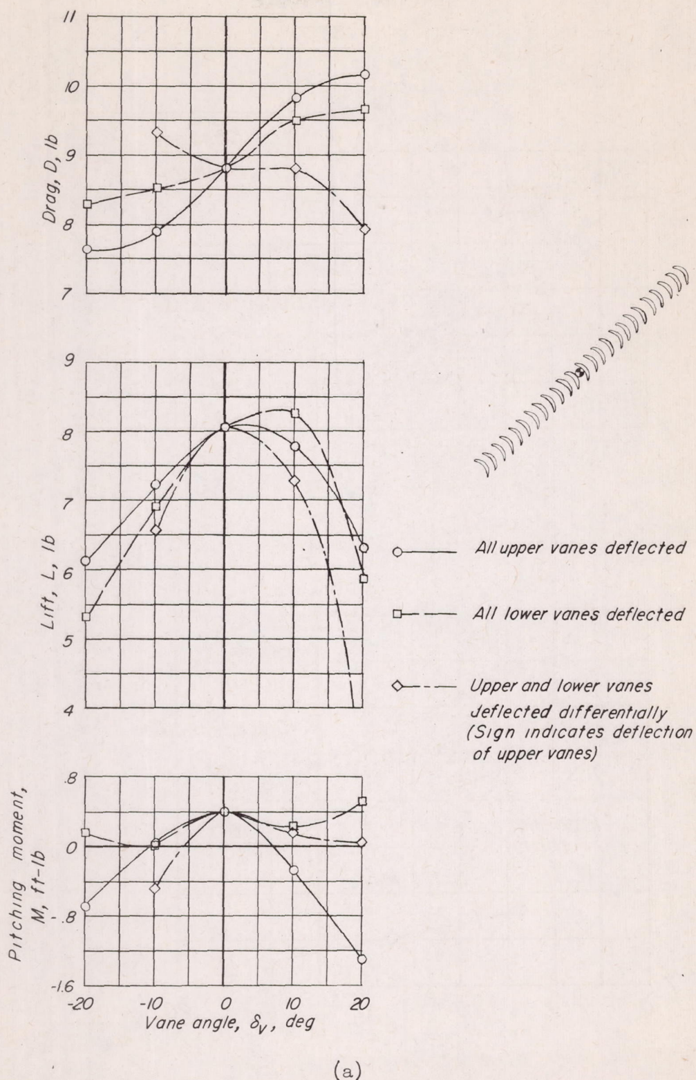
Figure 18.- Control effectiveness. Cascade angle (defined in fig. 17) = 45^\circ .
