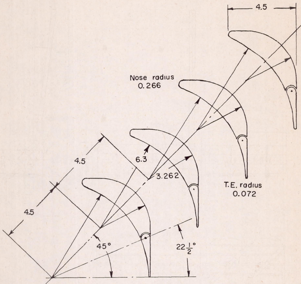
Figure 4.- Details of wing arrangement and airfoil section. All four wings identical. All dimensions are in inches.
