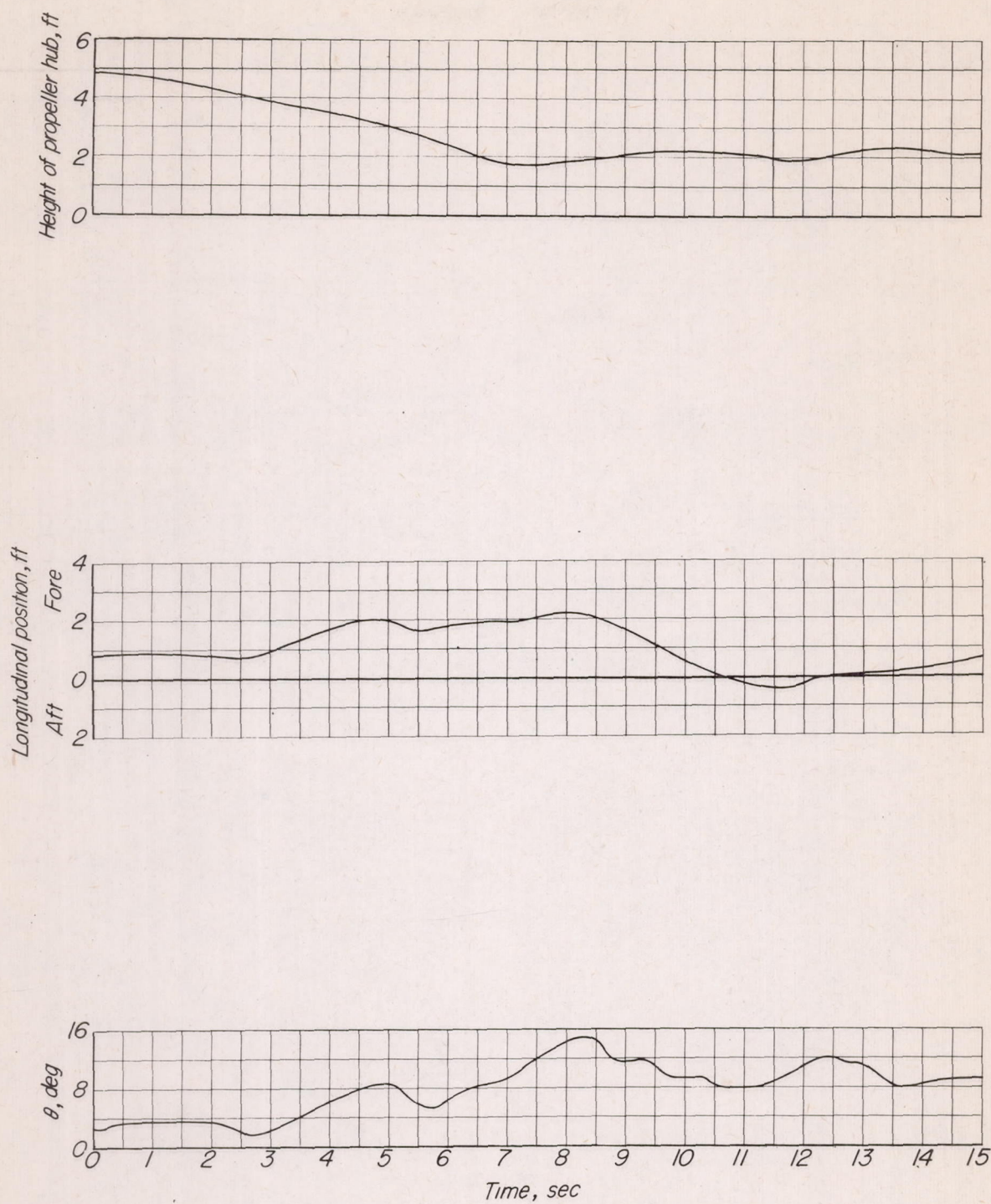
Figure 14.- Controlled flight near the ground with pitch damper. \frac{d\delta_p}{d\dot{\theta}} = 0.6 .
