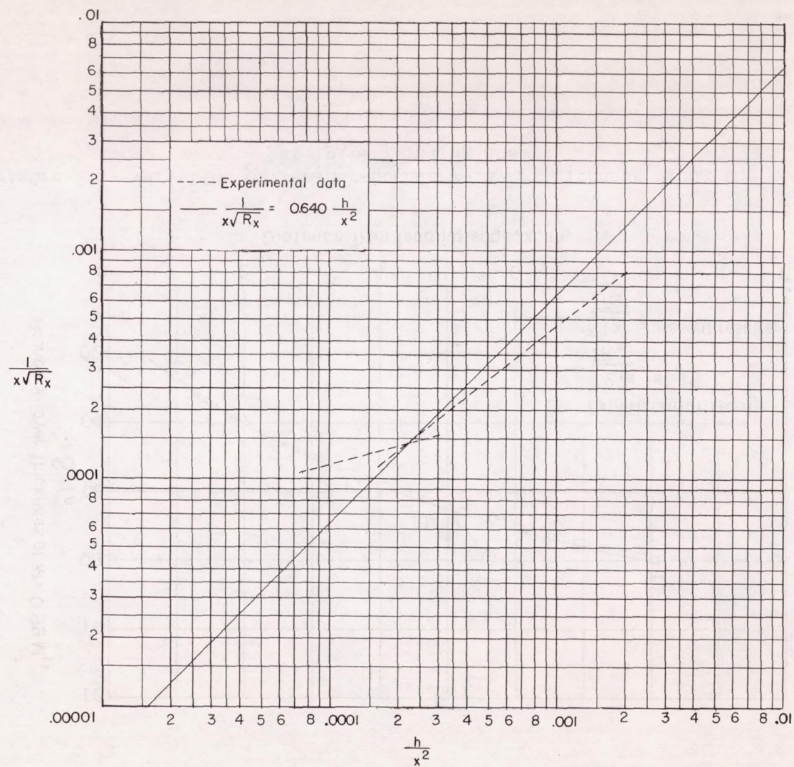
Figure 19.- Variation of 1/x\sqrt{R_x} as a function of h/x^2 .
