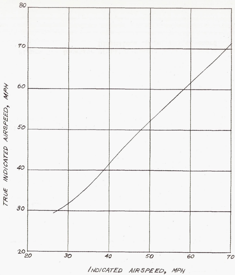
Figure 6.- Airspeed calibration.
