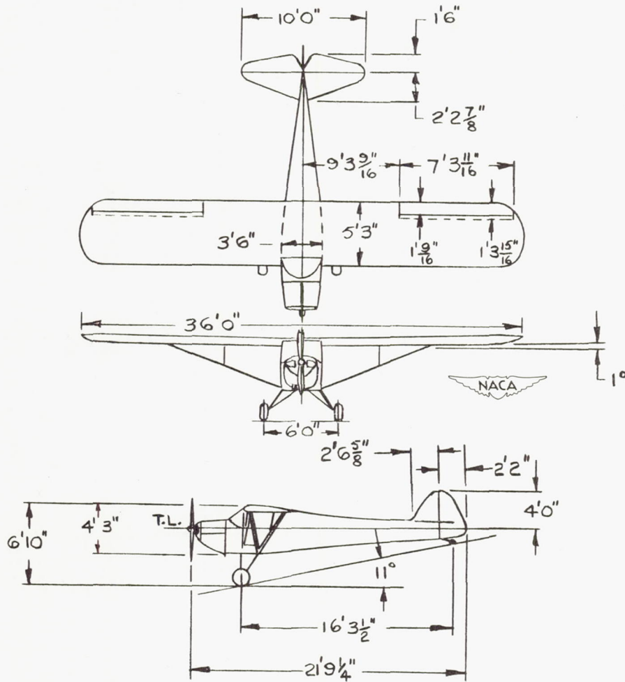
Figure 1.- Three-view drawing of test airplane.
