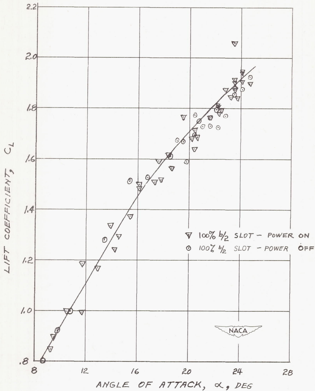
(b) Full-span slot.
