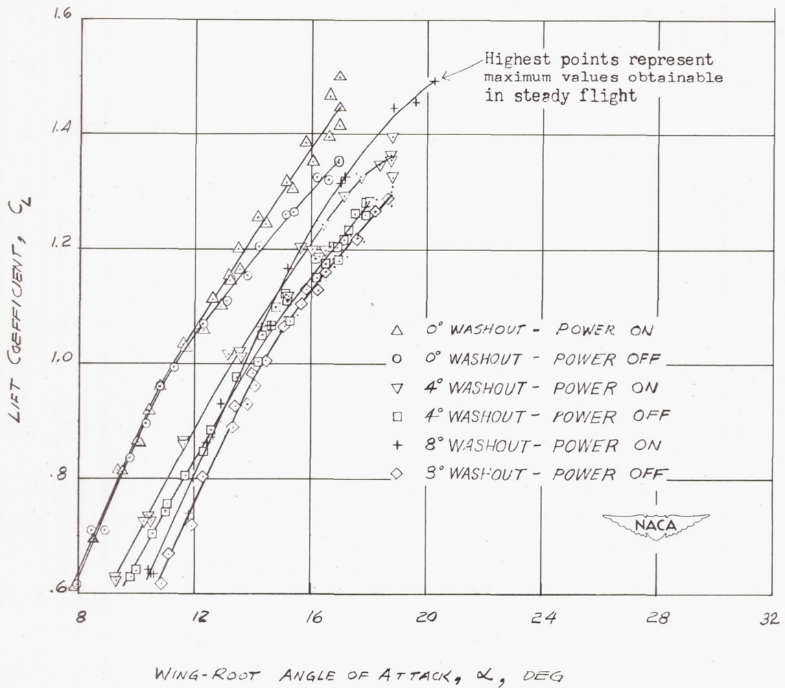
Figure 8.- Airplane lift characteristics for 0°, 4°, and 8° of washout.
