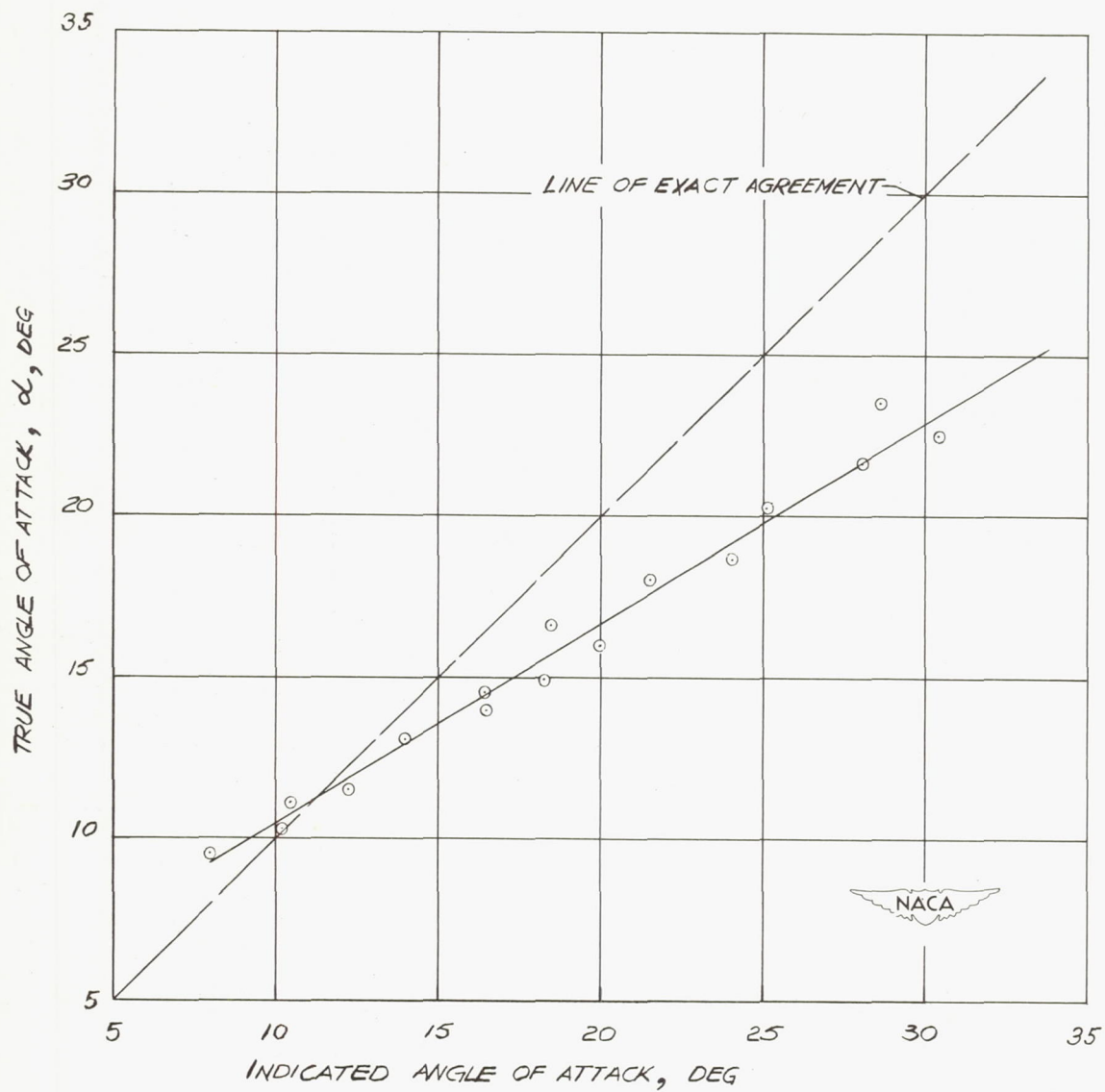
Figure 7.- Angle-of-attack-indicator calibration.
