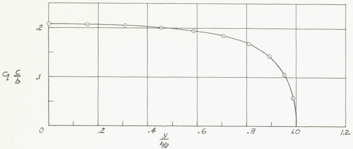
(a) Computed span loading. \alpha = 16.3^\circ ; C_L = 1.328 .
