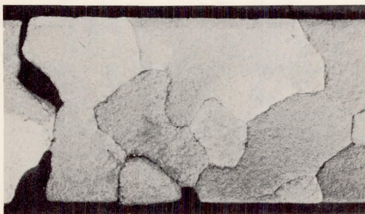
Figure 4.- Intergranular attack on a slow-cooled specimen. Aluminum III, cooled from 647^{\circ}\text{C} at 4.5^{\circ}\text{C} per hour and exposed 1 day to 20 percent hydrochloric acid. 6X.
