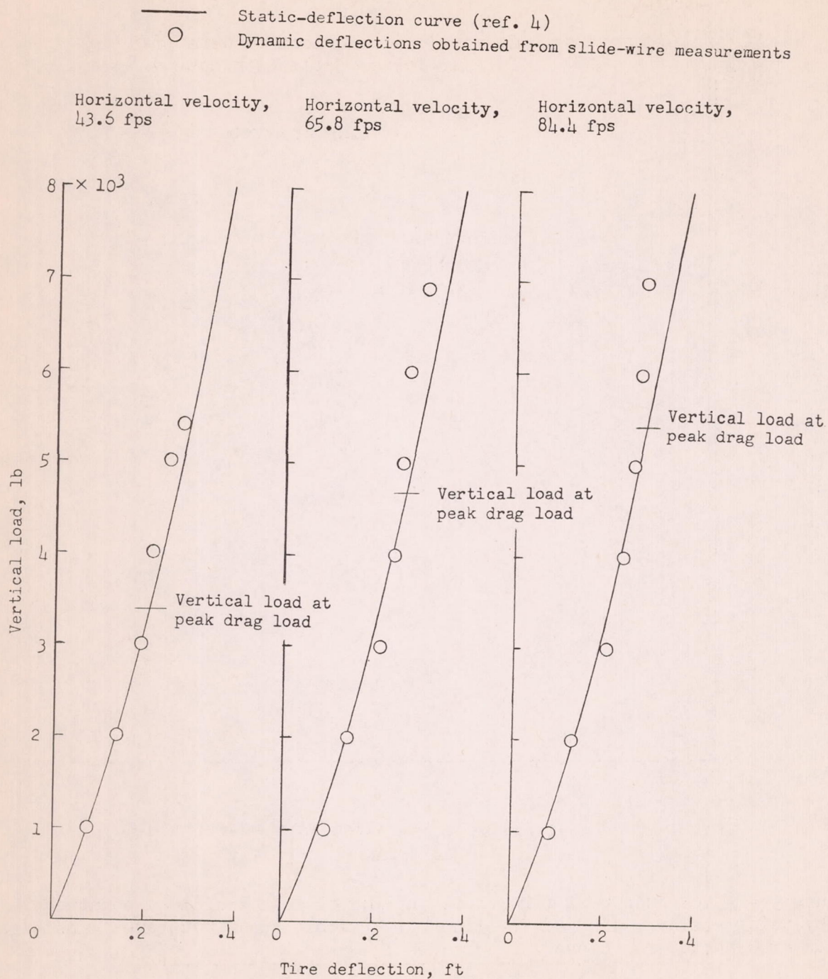
Figure 8.- Comparison of dynamic and static deflection at various horizontal velocities and a vertical velocity of 7.5 feet per second.
