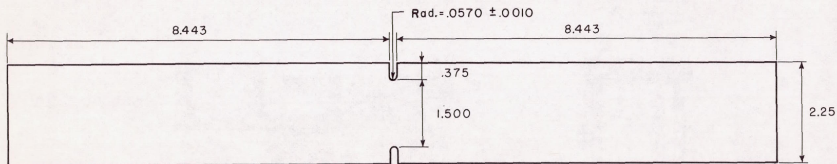
Figure 1.- Notched fatigue test specimen with K_T = 4.0 .
