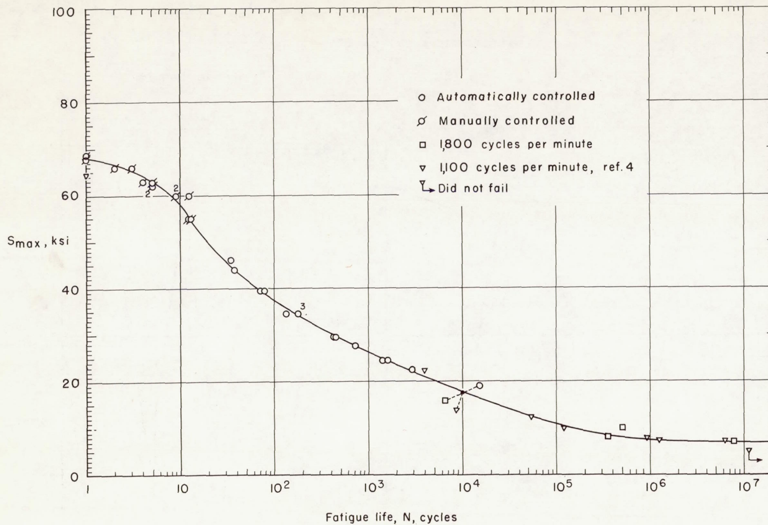
Figure 4.- Results of axial-load fatigue tests on notched 24S-T3 aluminum-alloy sheet specimens. K_T = 4.0 ; R = -1 .
