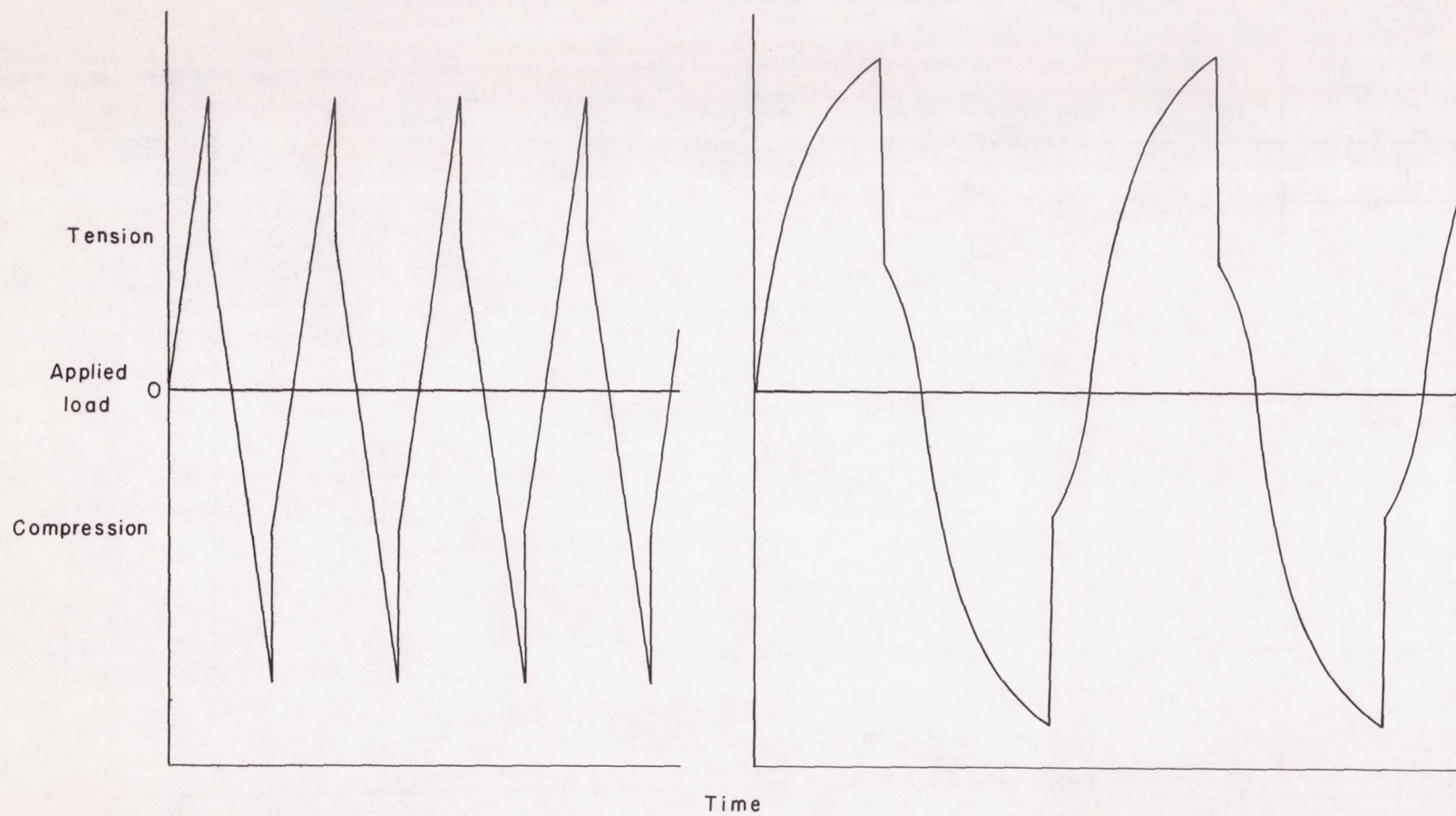
Figure 3.- Typical load-time curves.
