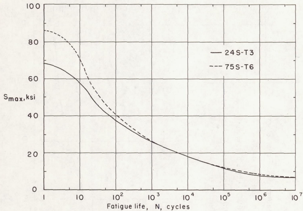
Figure 6.- Comparison of S-N curves for notched 24S-T3 and 75S-T6 aluminum-alloy sheet specimens. K_T = 4.0 ; R = -1 .
