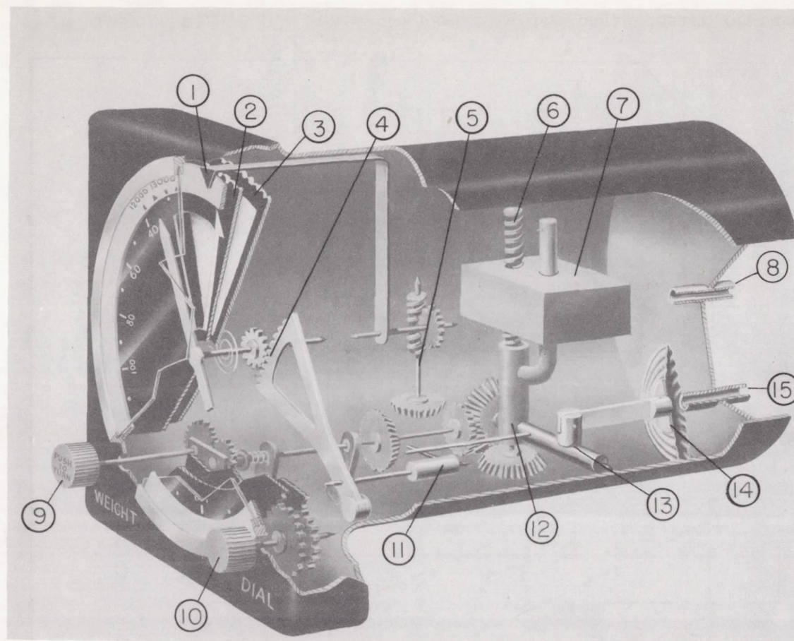
Figure 3.- Illustrative arrangement of take-off indicator.
