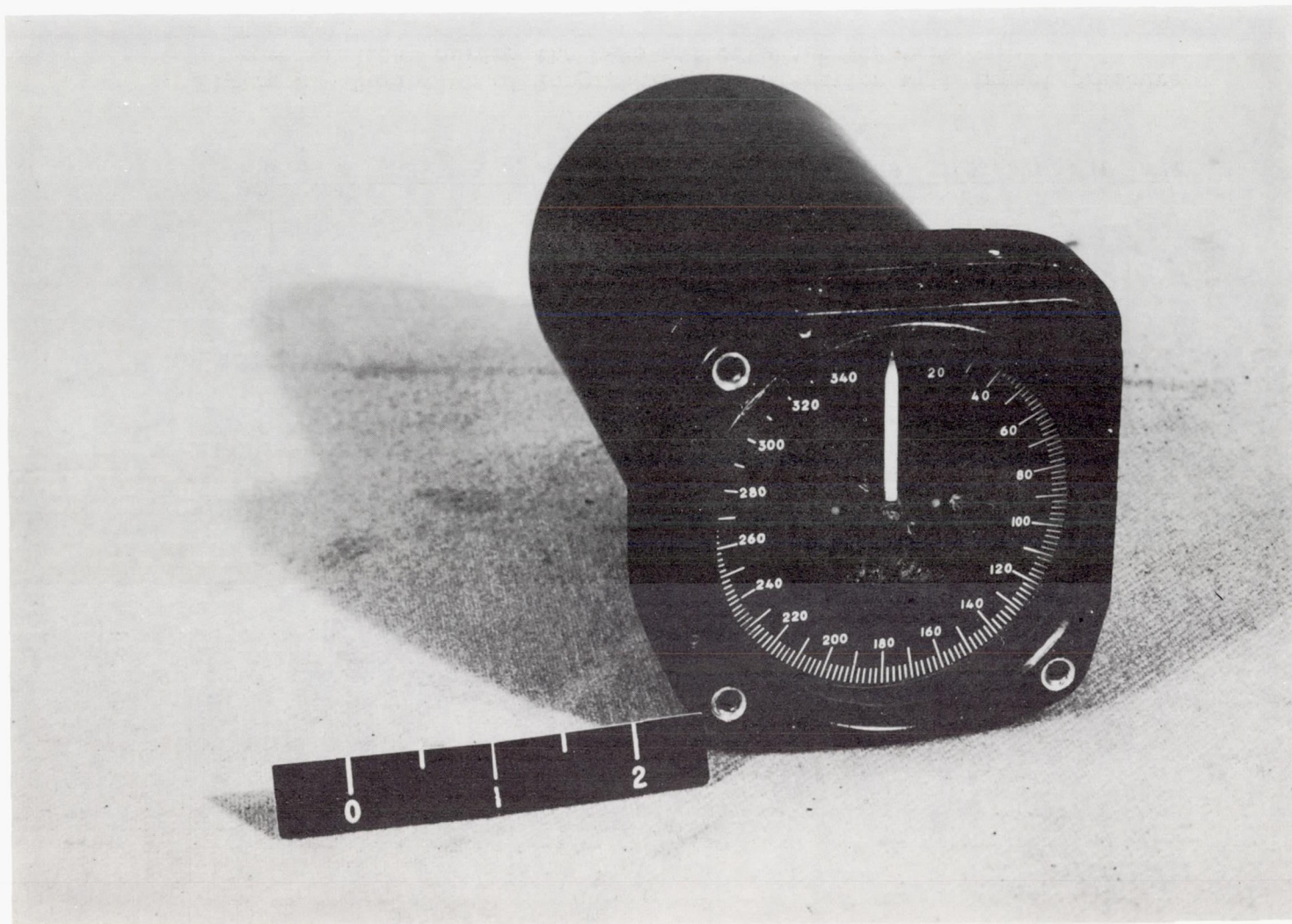
Figure 7.- Photograph of simplified prototype take-off indicator.
