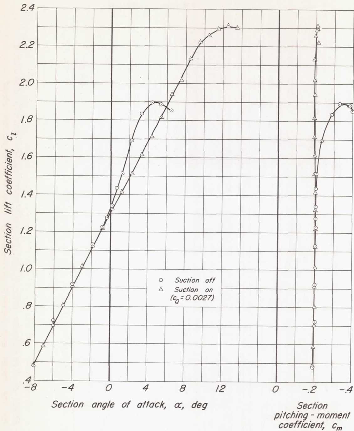
Figure 17.- Lift and moment characteristics of the model with tapered permeability from 0- to 1-percent chord and a 0.2-chord split flap deflected 60^\circ ; V_0 = 133 fps.
