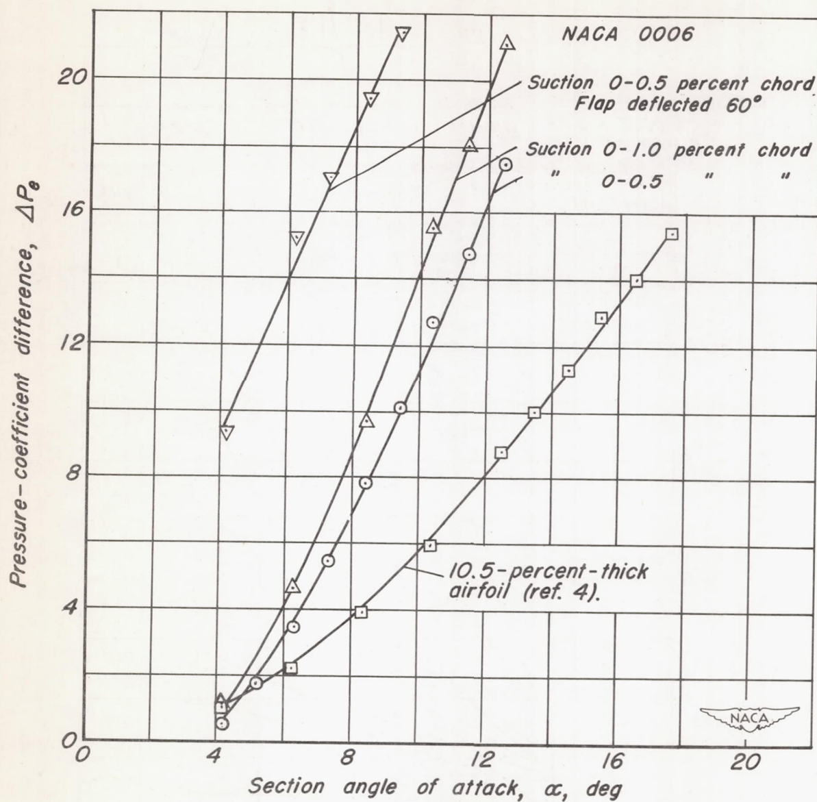
Figure 22.-Comparison of the pressure-coefficient difference between the leading and trailing edges of the porous area on the NACA 0006 and the symmetrical 10.5-percent-thick airfoils; c_Q = 0.0016 ; V_0 = 162 fps.
