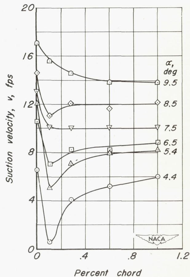
Figure 18.- Flow requirements and stall-point suction-velocity distributions for the model with tapered permeability from 0- to 1-percent chord and a 0.2-chord split flap deflected 60^\circ ; V_0 = 133 fps.
