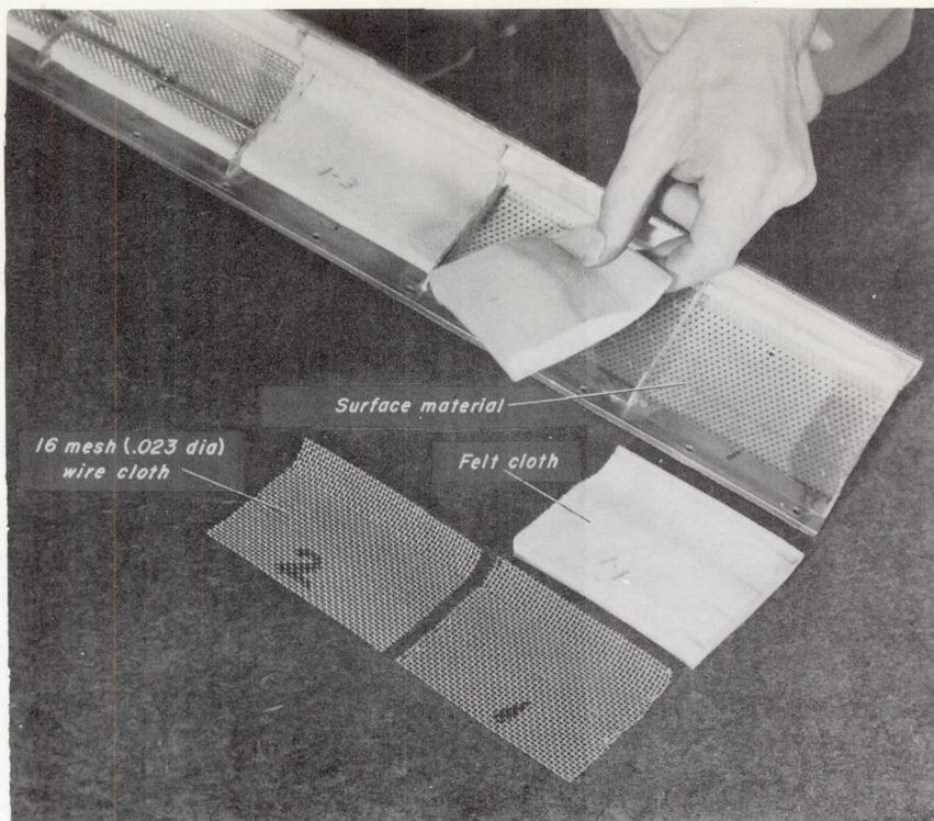
(a) Arrangement of the permeable material in the leading edge.
