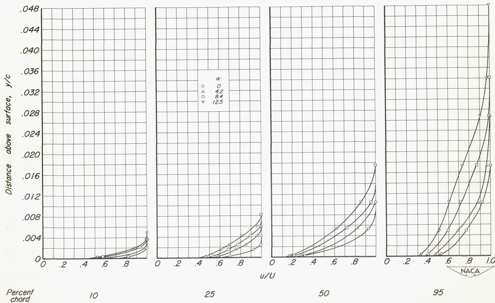
Figure 14.-Boundary-layer velocity profiles for the model with tapered permeability from 0-to 1-percent chord; c_0=0.0016 ; V_0=162 fps.
