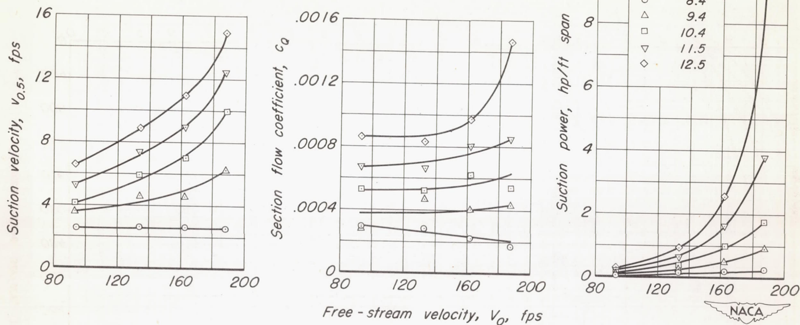
Figure 15.-Effect of free-stream velocity on the stall-point suction requirements of the model with tapered permeability from 0- to 1-percent chord.
