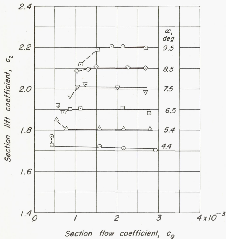
Figure 18.- Flow requirements and stall-point suction-velocity distributions for the model with tapered permeability from 0- to 1-percent chord and a 0.2-chord split flap deflected 60^\circ ; V_0 = 133 fps.
