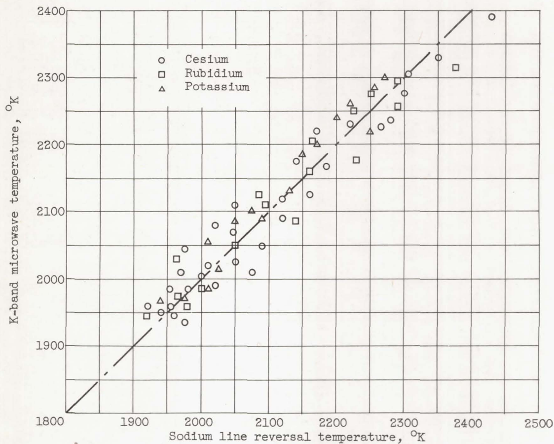
(a) K-band microwaves, obtained for experimental ionization potentials for cesium, rubidium, and potassium.
