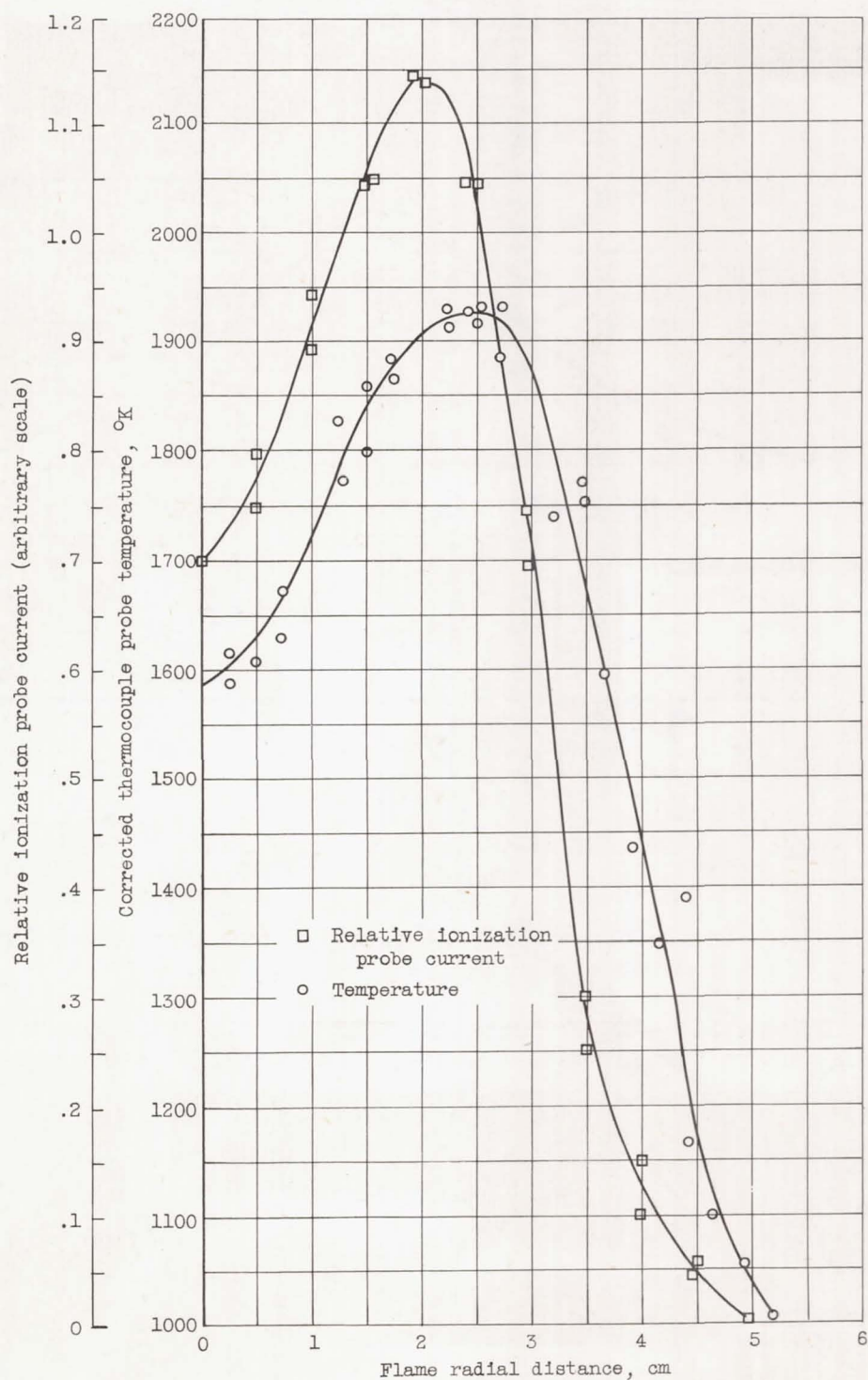
Figure 10. - Typical plots of relative ionization probe current and thermocouple probe temperature across blast burner flame.
