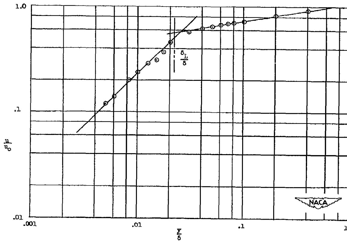
Figure 2.- Agreement between assumed and experimental profiles from reference 10. R_\delta = 12,200 .
