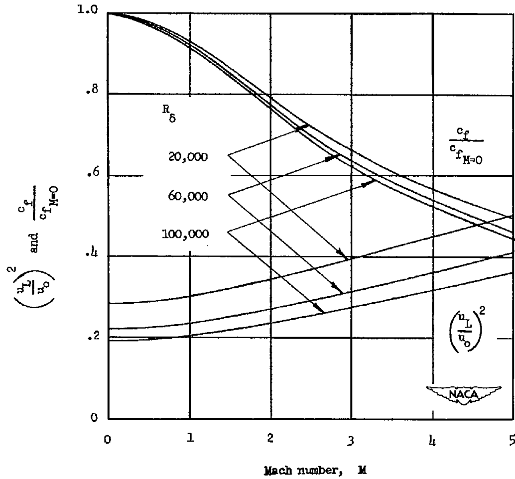
Figure 4.- Plot of \frac{c_f}{c_{f_{M=0}}} and \left(\frac{u_L}{u_0}\right)^2 against Mach number as determined from equations (24) and (25).
