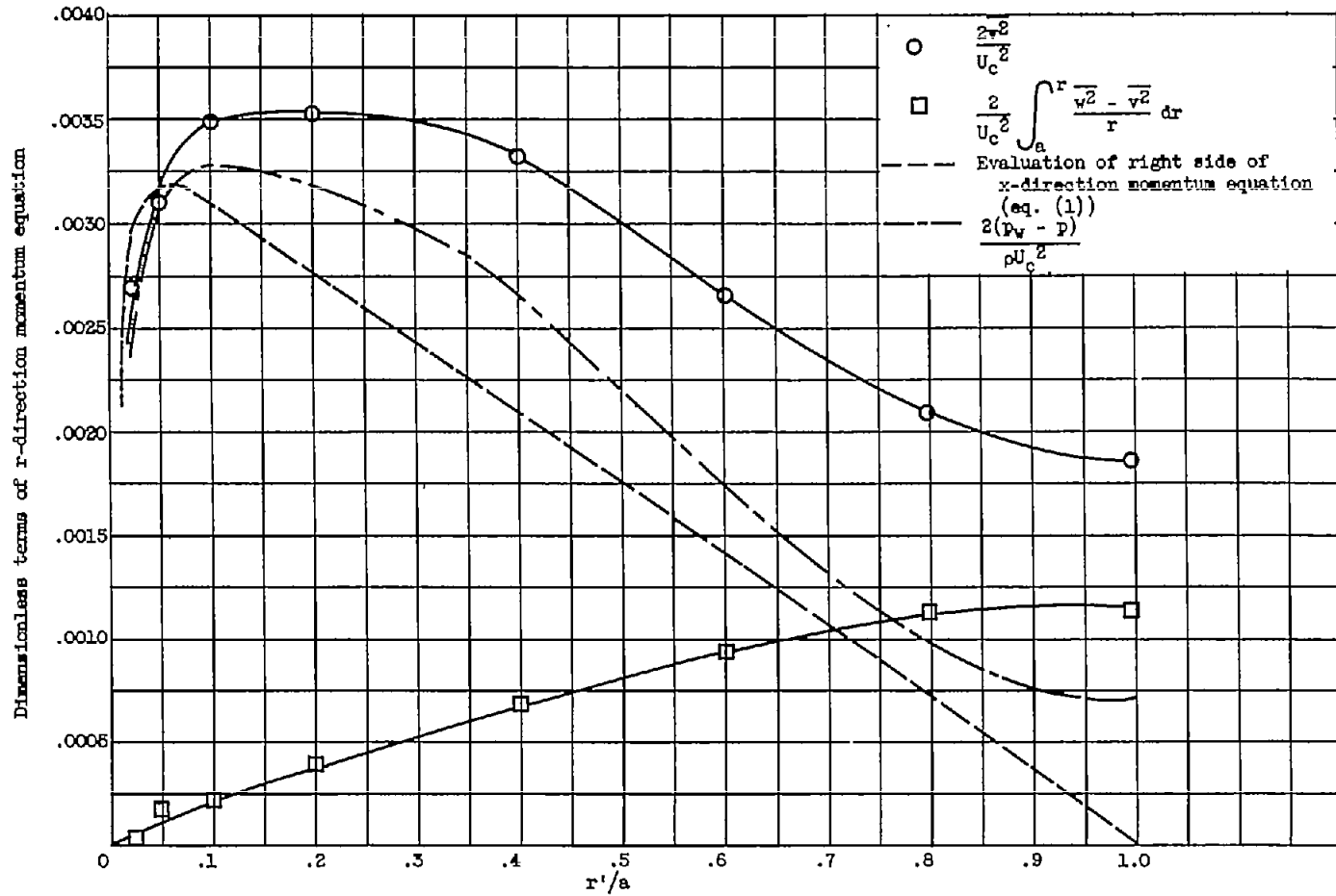
(a) Reynolds number, 25,000.
