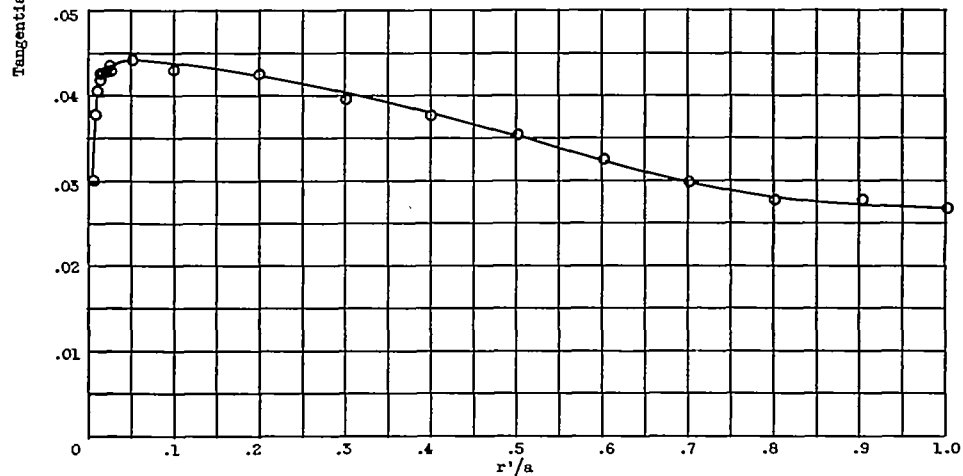
(b) Reynolds number, 50,000.
