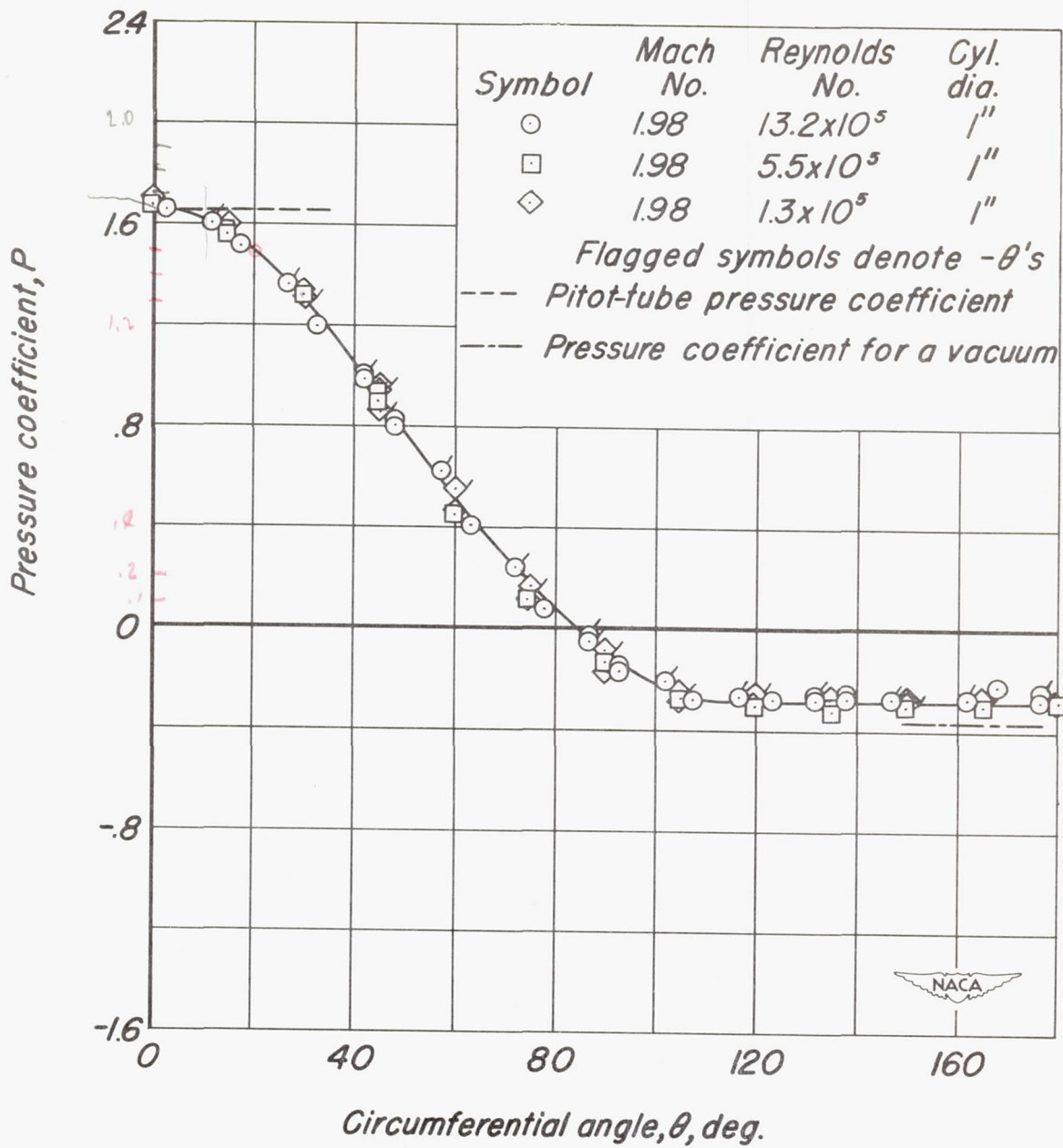
(d) Effects of Reynolds number at a Mach number of 1.98.
