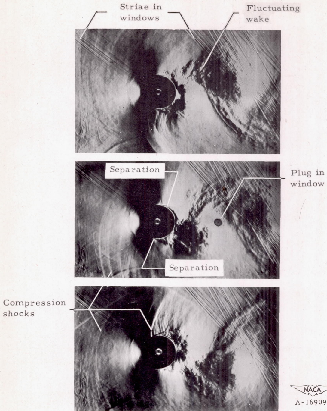
Figure 3. - Schlieren pictures of the flow about a 1.97-inch cylinder in the Ames 1- by 3 1 / 2 -foot wind tunnel at a Mach number of 0.51.
