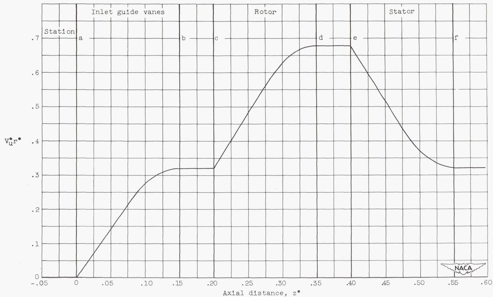
Figure 3. - Prescribed variation of tangential velocity along casing.
