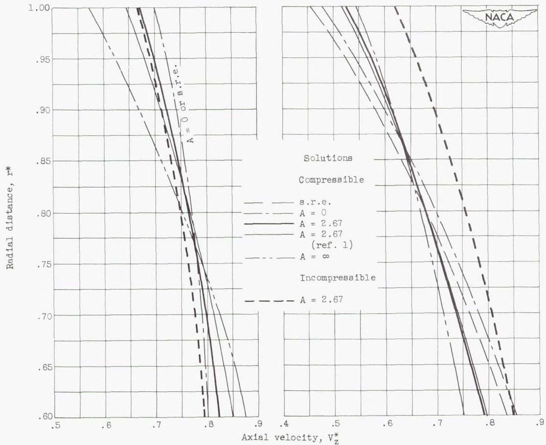
Figure 12. - Radial variation of axial velocity in front of and behind rotor. A , aspect ratio; s.r.e., simplified-radial-equilibrium.
