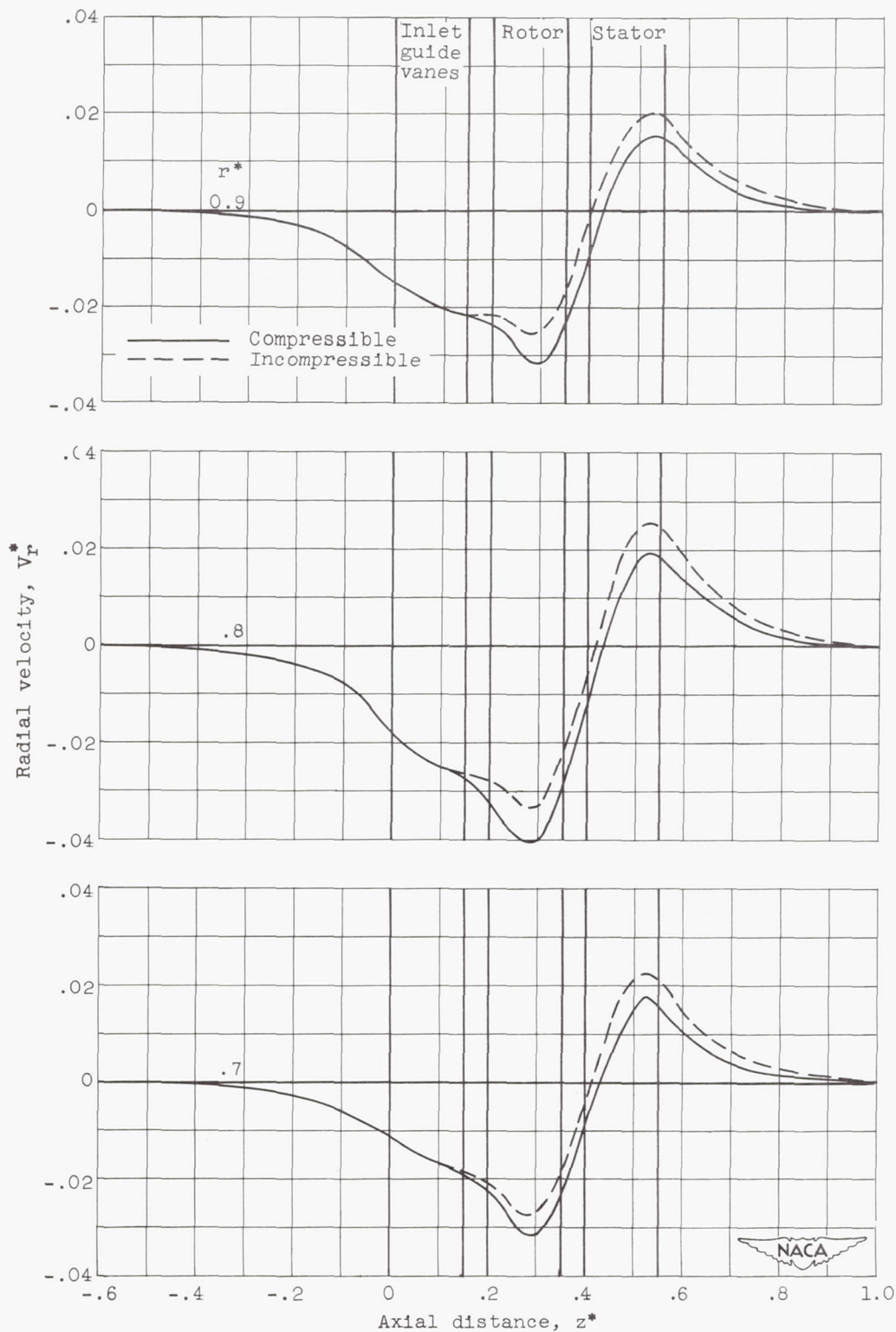
Figure 7. - Variation of radial velocity.
