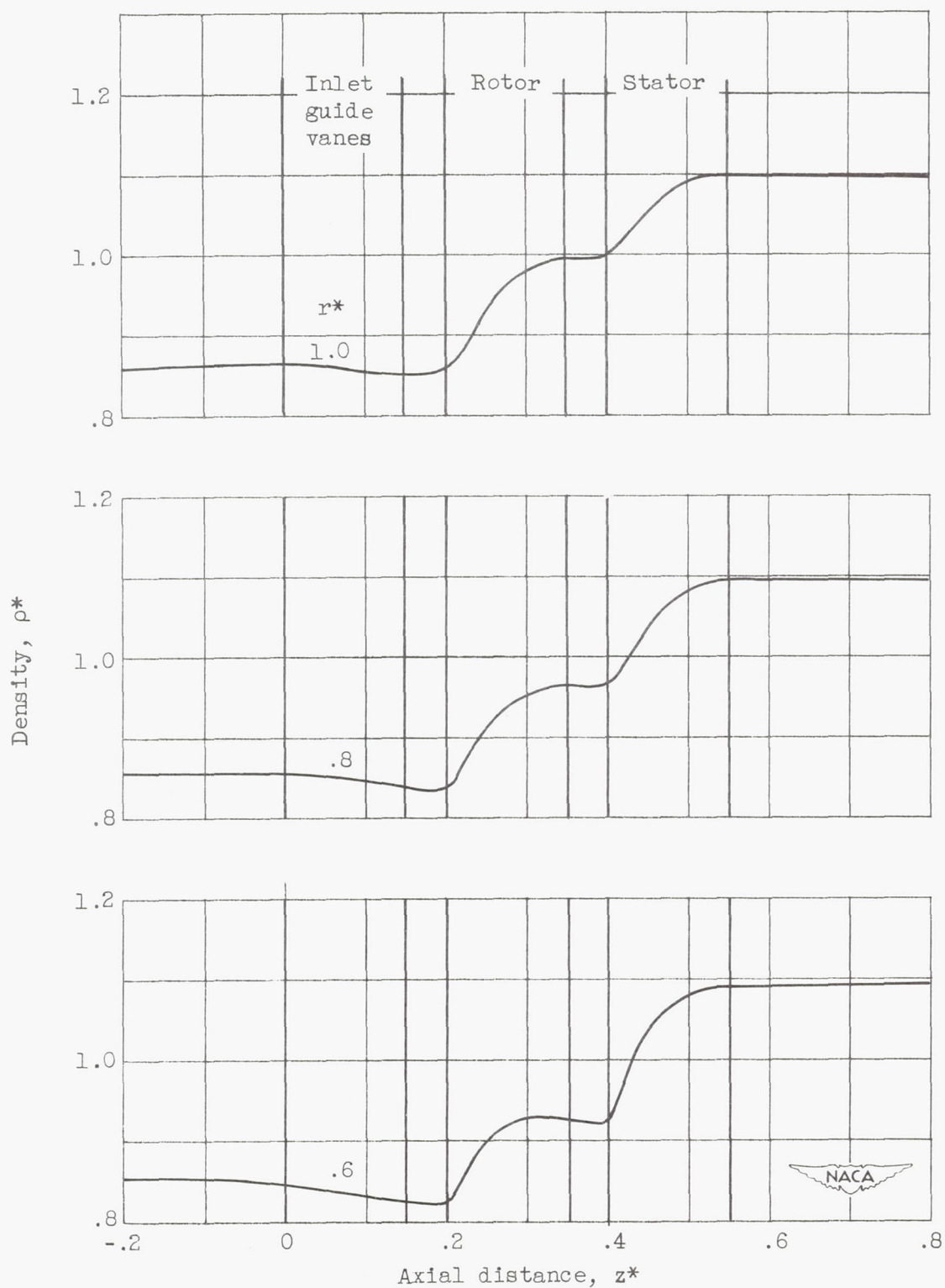
Figure 8. - Variation of density.
