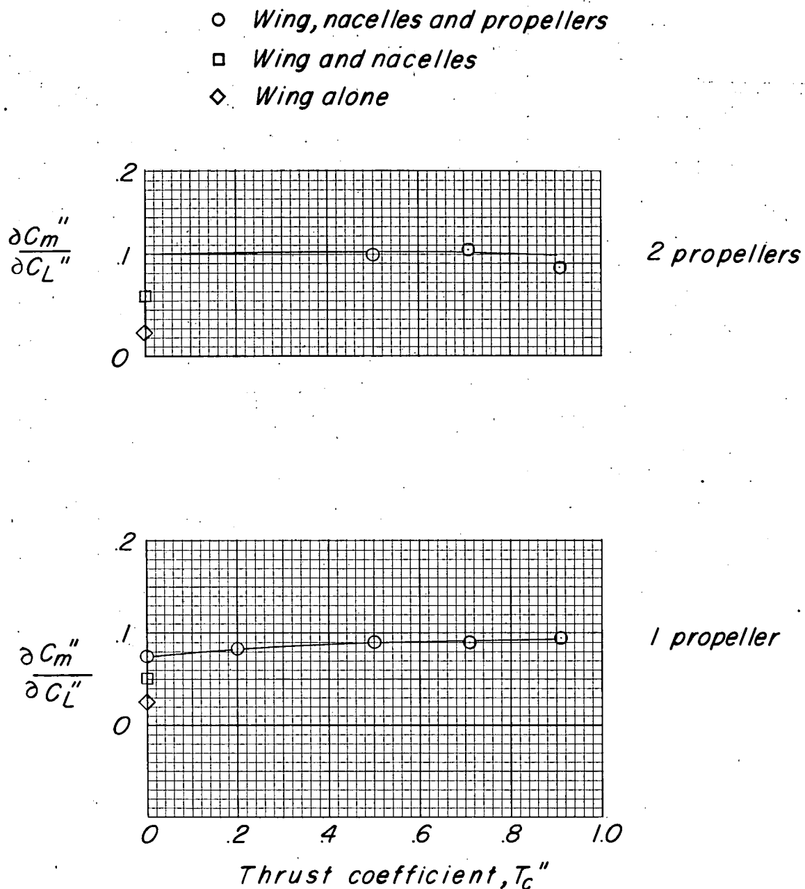
Figure 21.- Variation with thrust coefficient of longitudinal-stability parameter \partial C_m''/\partial C_L'' near zero angle of attack.
