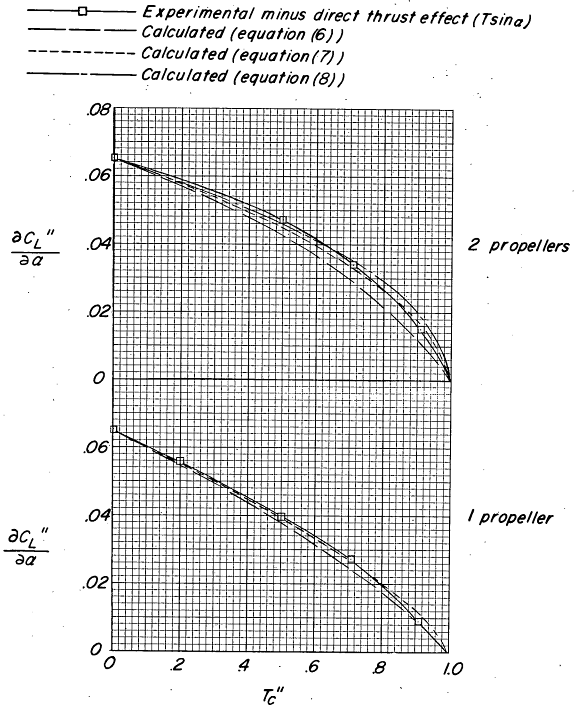
Figure 22.- Variation of \partial C_L''/\partial \alpha with thrust coefficient near \alpha = 0^\circ .
