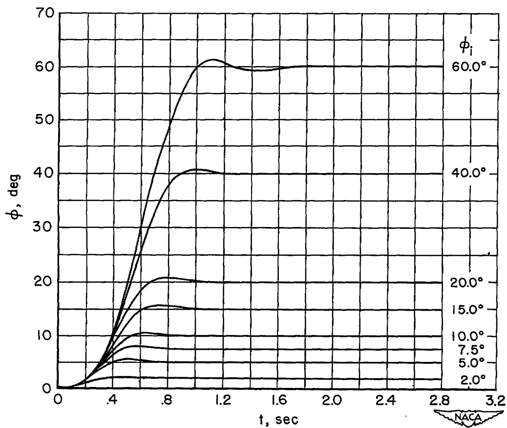
Figure 8.— Response of modified roll-control system to step commands with K_{\phi} as a nonlinear function of error.
