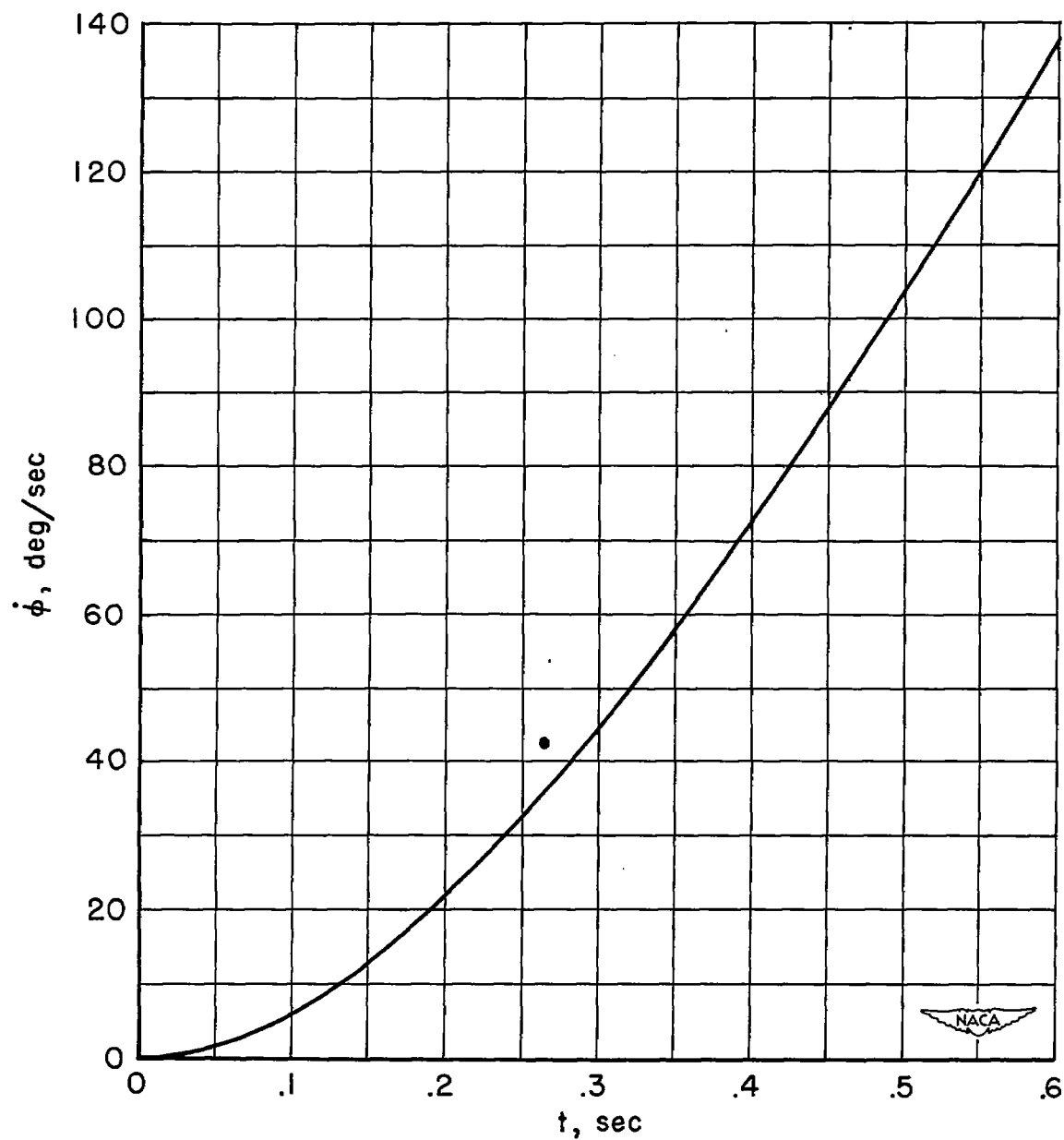
Figure 6.— Rolling-velocity response to a constant rate (50° per sec) aileron input.
