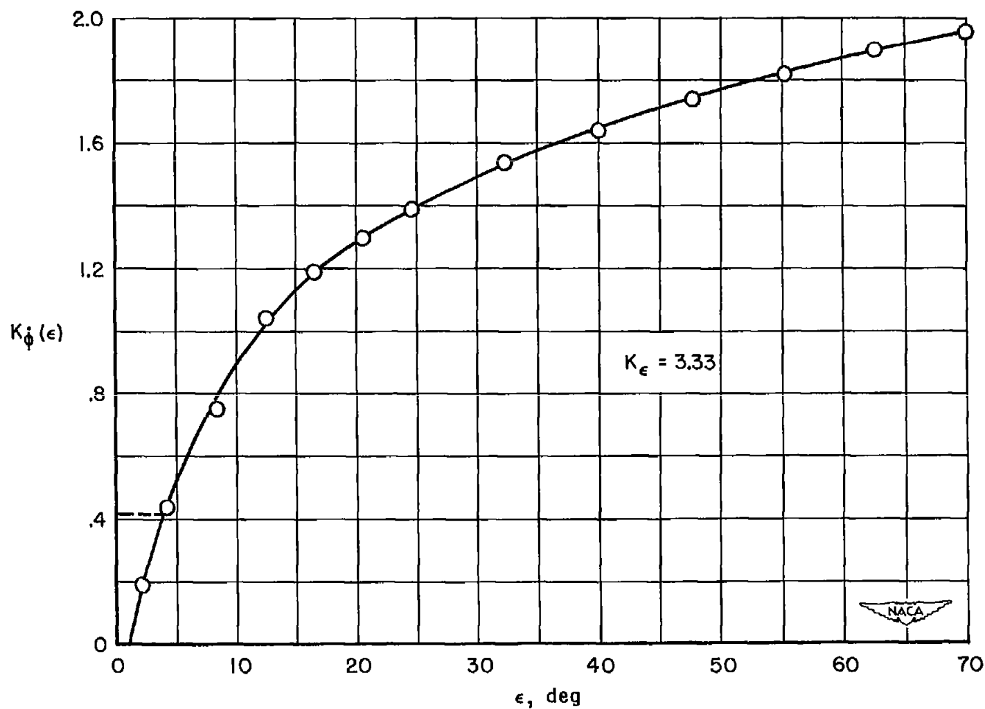
Figure 9.— Optimum nonlinear function K_{\phi}^*(\epsilon) for the roll-control system.
