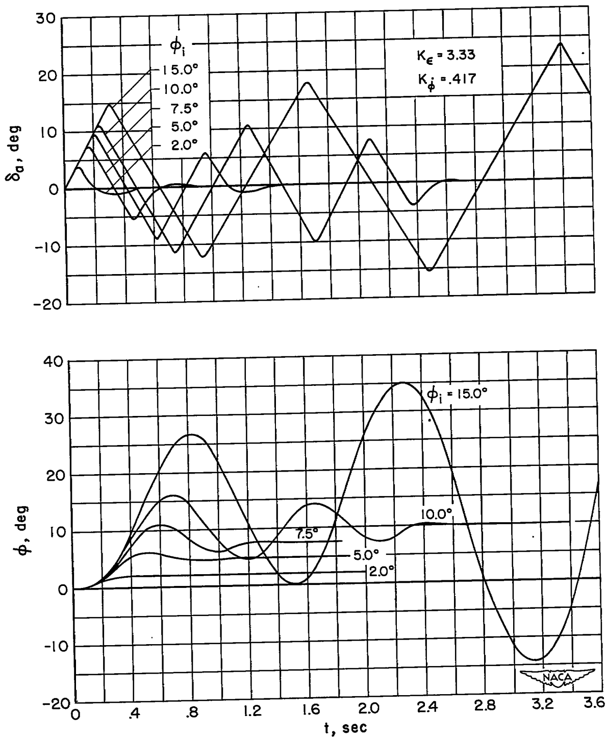
Figure 3.— Response of basic roll-control system to step commands with aileron rate limited to 50^\circ per sec.
