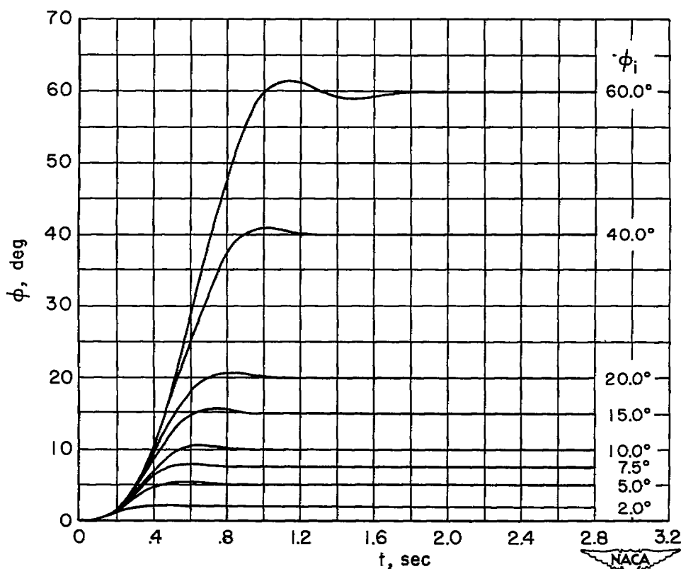
Figure 10.- Response of modified roll-control system to step commands with K_{\phi} as a nonlinear function of error.
