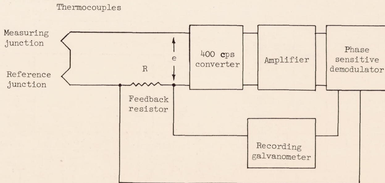
Figure 5.- Block diagram of electronic temperature recorder.
