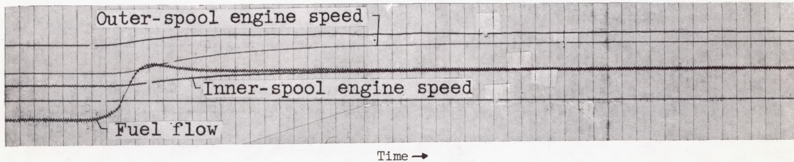
Figure 2. - Transient data for change in fuel flow at constant exhaust-nozzle area.
