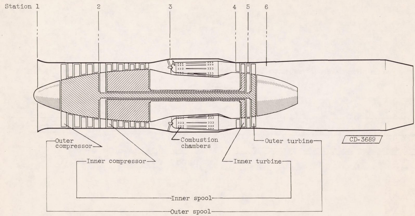
Figure 1. - Two-spool engine.
