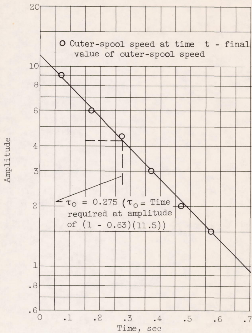
Figure 5. - Semilog plot of outer-spool speed response to exhaust-nozzle area at constant fuel flow.
