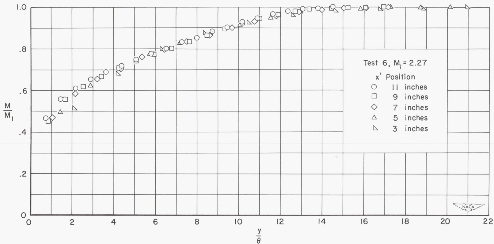
Figure 4.- Typical boundary-layer distributions showing similarity of profiles.
