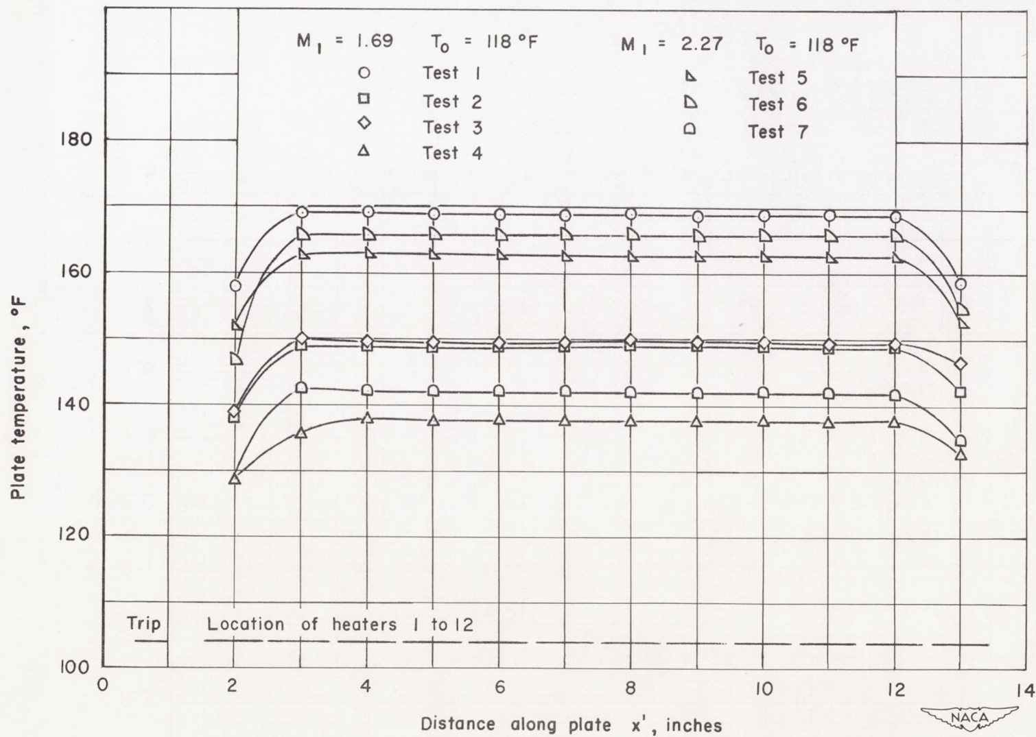
Figure 3.- Typical temperature distributions along flat-plate model.
