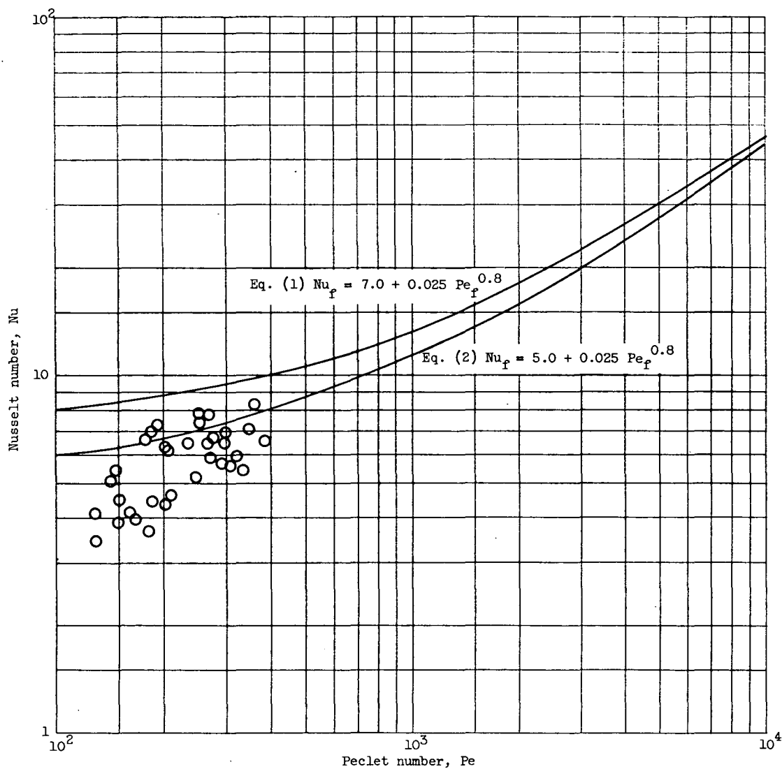
Figure 32. - Re-evaluated data of Doody and Younger (refs. 14 and 15) for heat transfer to mercury with small sodium additions in round tubes.
