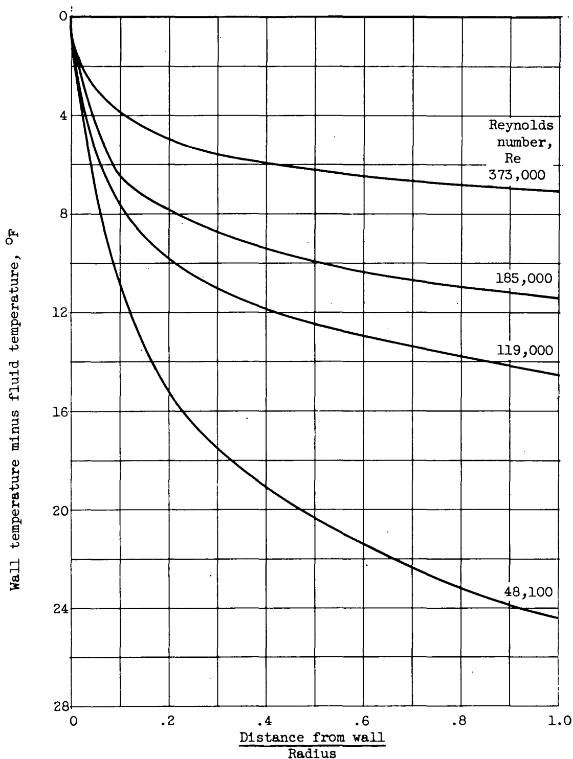
Figure 4. - Theoretical predictions of Martinelli (ref. 27) for fully developed temperature profiles for heat transfer to liquid metals in round tubes. Prandtl number, 0.022.
