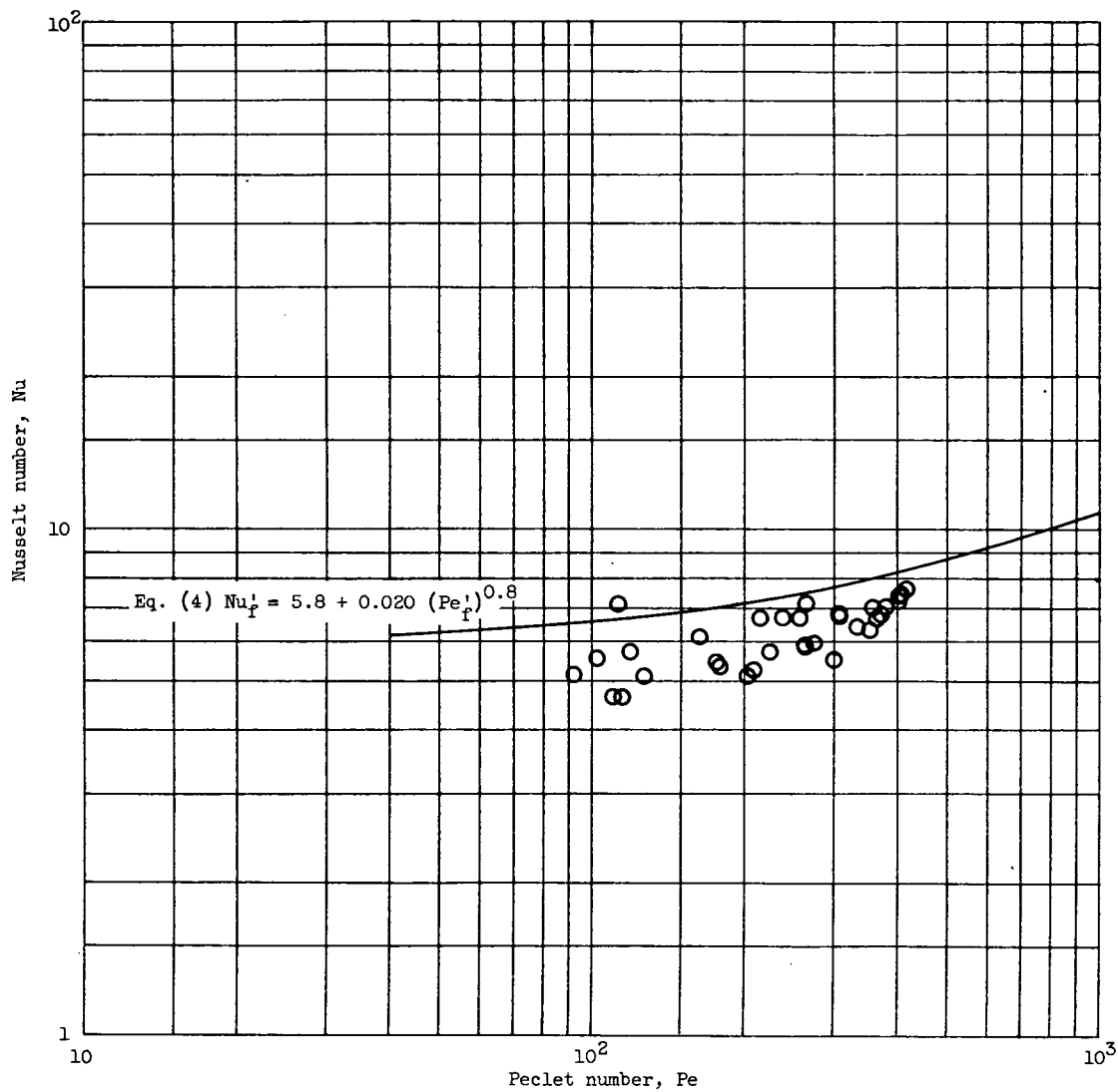
Figure 17. - Concluded. Re-evaluated data of Lyon (ref. 6) for average heat transfer to a sodium-potassium alloy in annuli.
