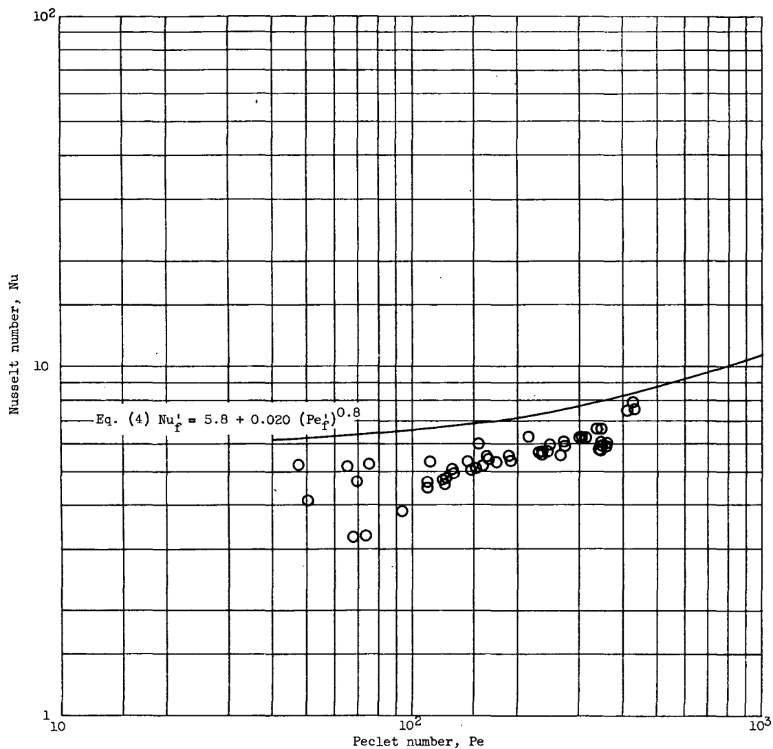
Figure 17. - Continued. Re-evaluated data of Lyon (ref. 6) for average heat transfer to a sodium-potassium alloy in annuli.
