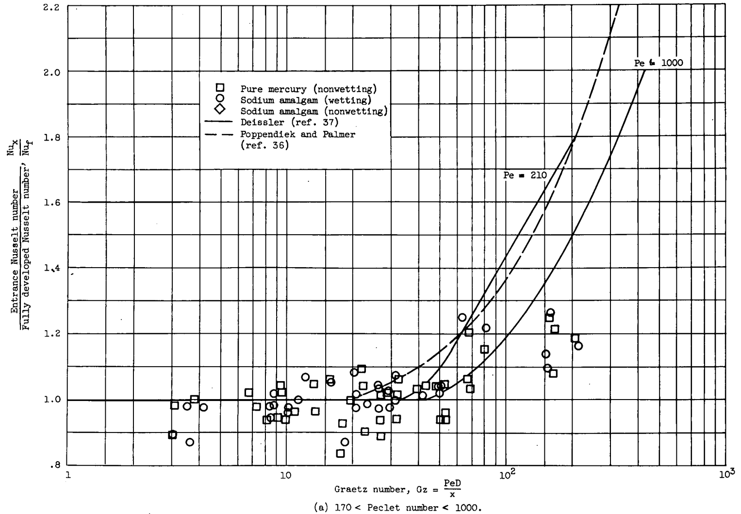
Figure 44. - Data of Stromquist (ref. 21) for entrance region heat transfer to mercury, with and without sodium additions, in round tubes.
