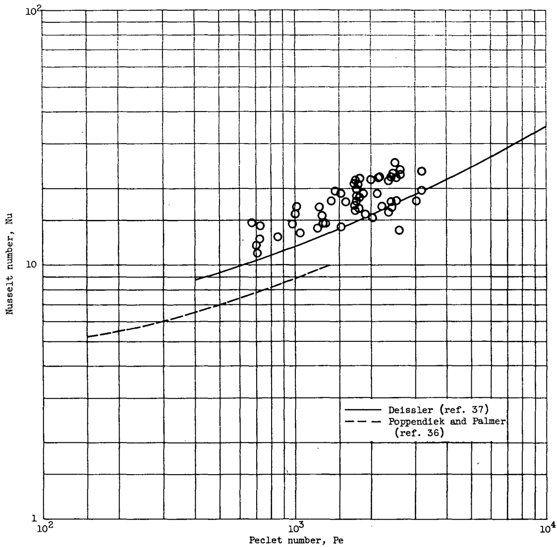
Figure 36. - Data of Johnson, Hartnett, and Clabaugh (refs. 17 and 18) for entrance region heat transfer to lead-bismuth eutectic in round tubes.
