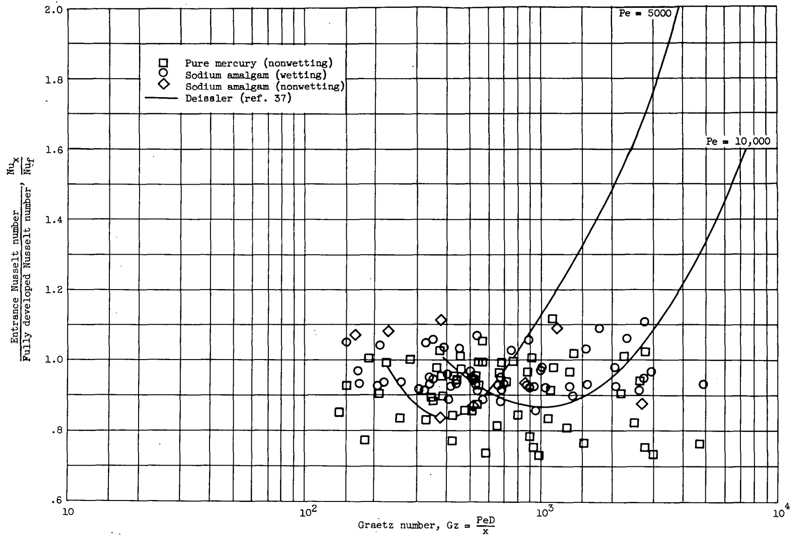
Figure 44. - Concluded. Data of Stromquist (ref. 21) for entrance region heat transfer to mercury, with and without sodium additions, in round tubes.
