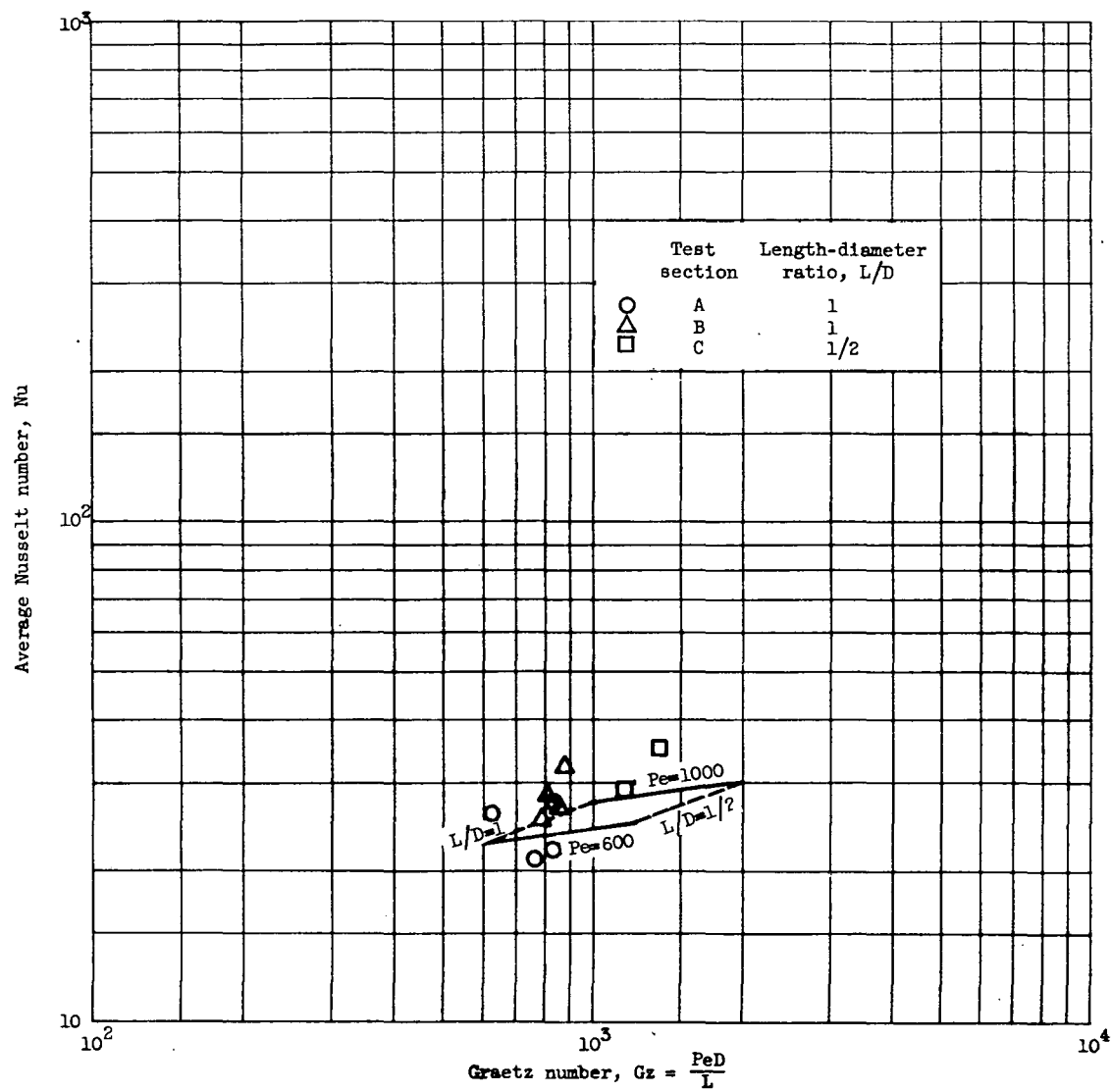
Figure 52. - Data of Poppendiek and Harrison (ref. 26) for average heat transfer to mercury in very short round tubes compared with prediction of Deissler (ref. 37).
