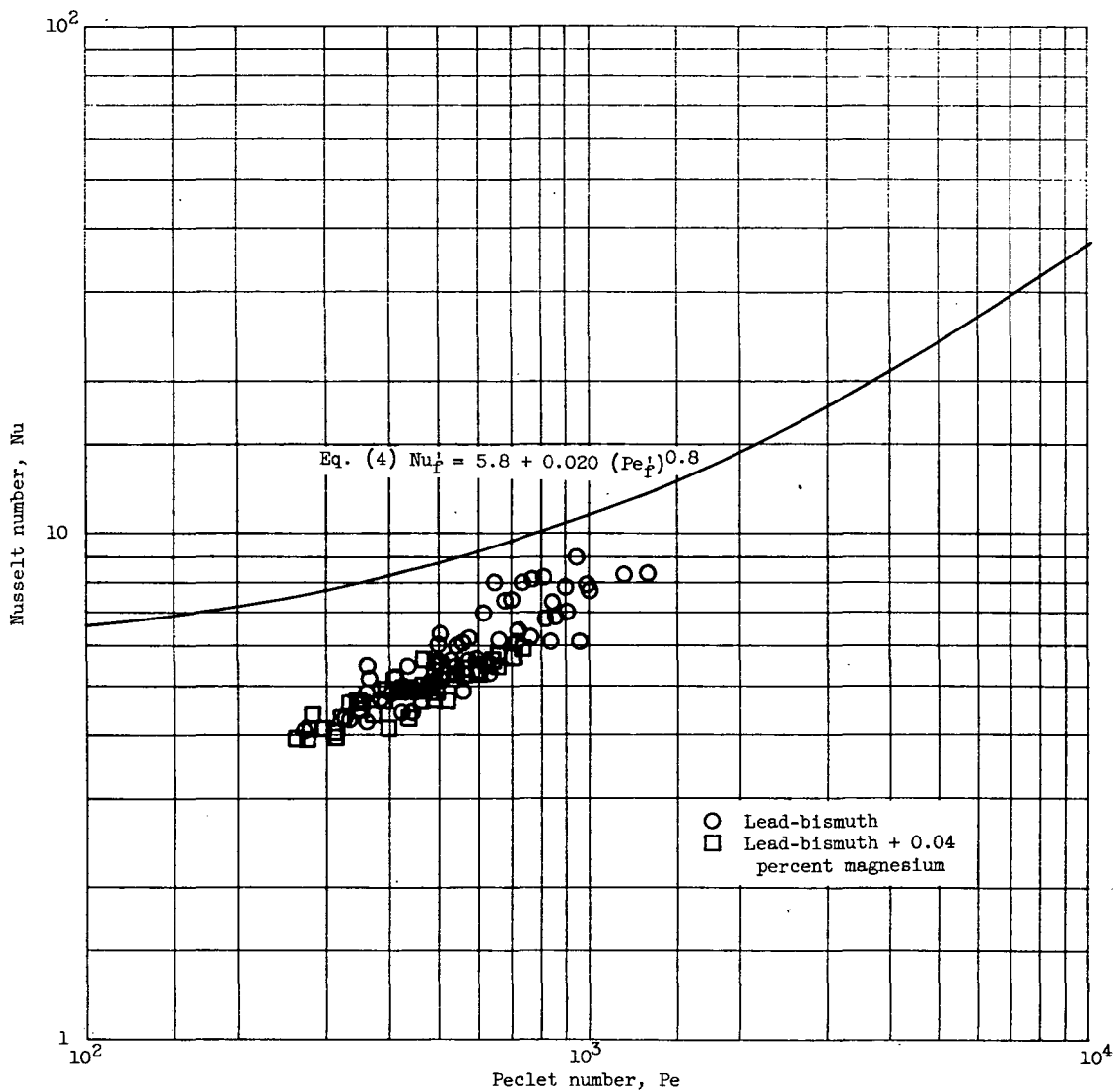
Figure 34. - Data of Lubarsky (ref. 16) for average heat transfer to lead-bismuth eutectic in annuli. Length-diameter ratio, 322.
