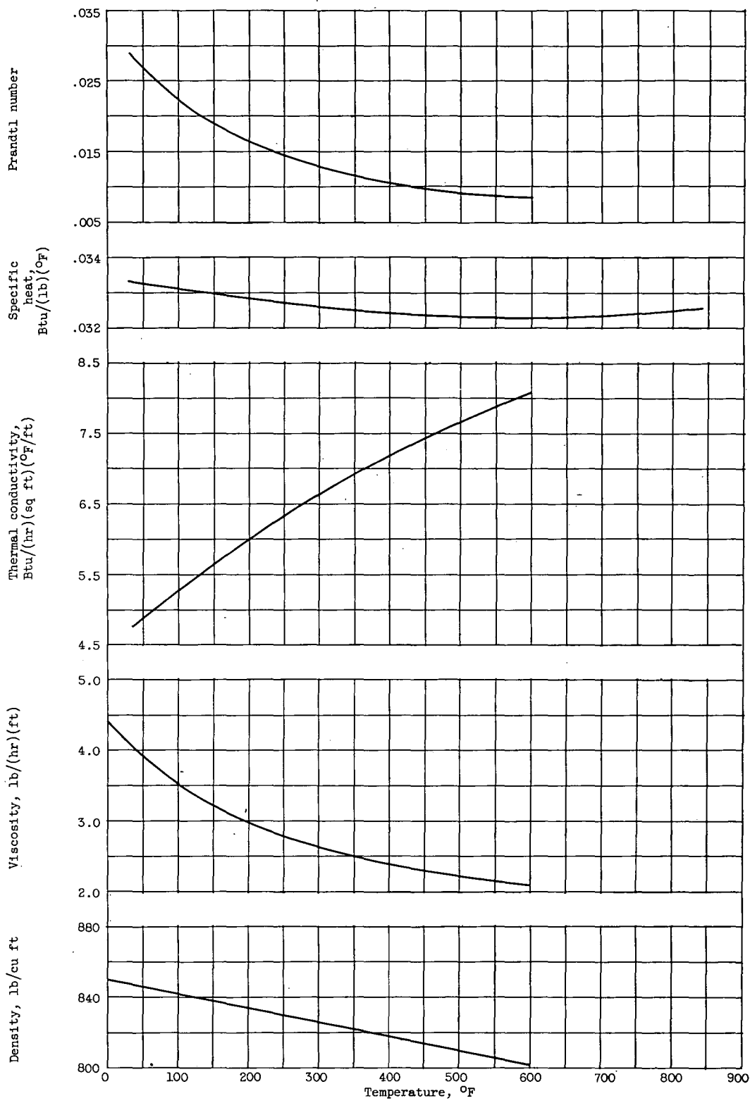
Figure 7. - Physical properties of mercury (ref. 28).
