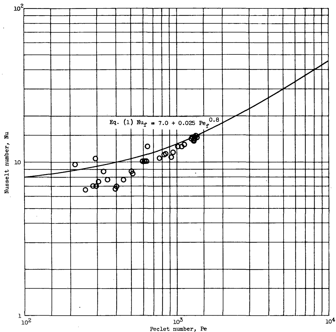
Figure 16. - Continued. Re-evaluated data of Lyon (ref. 6) for average heat transfer to a sodium-potassium alloy in round tubes.
