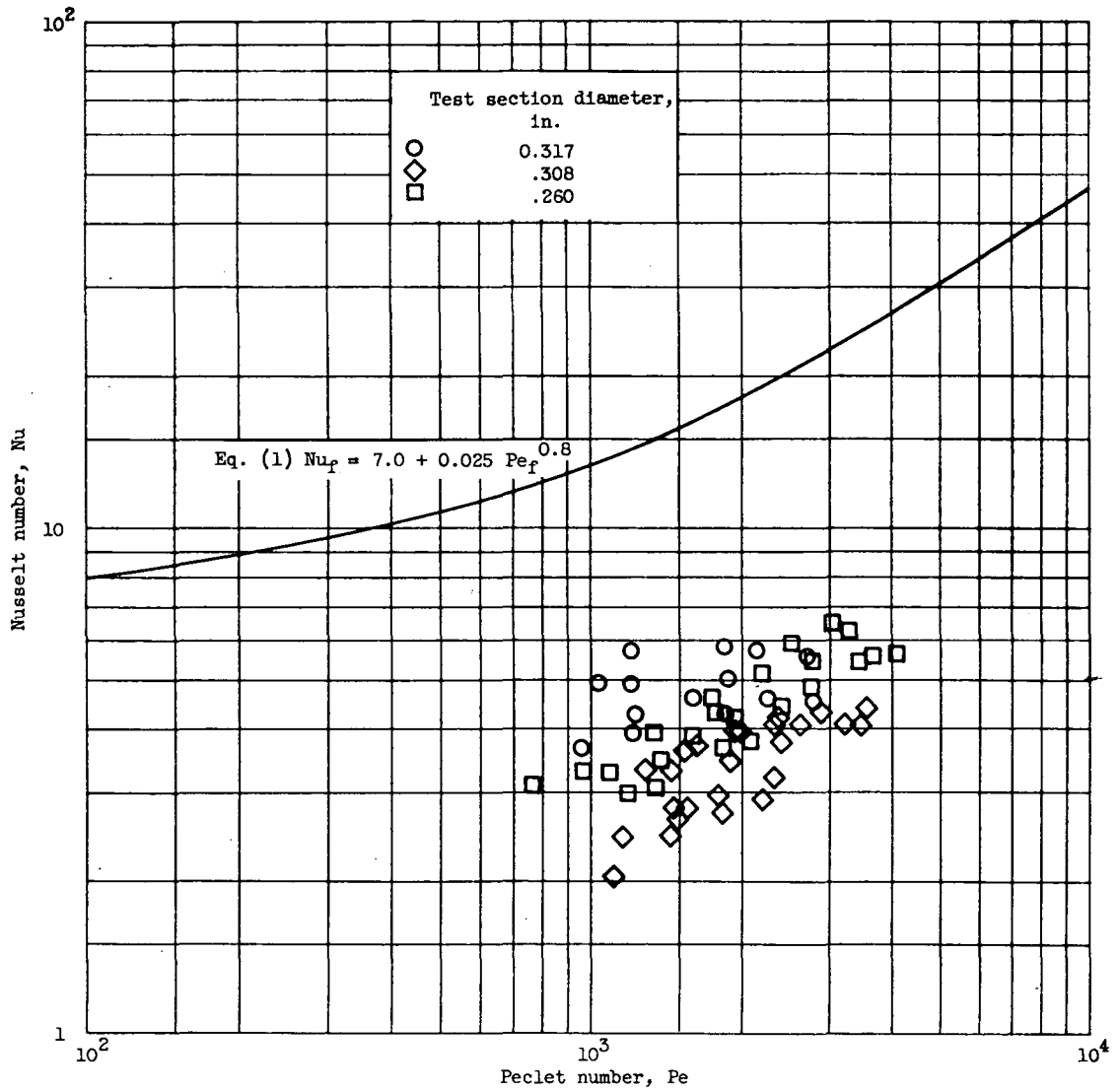
Figure 14. - Re-evaluated data of Elser (ref. 4) for fully developed heat transfer to mercury in round tubes.
