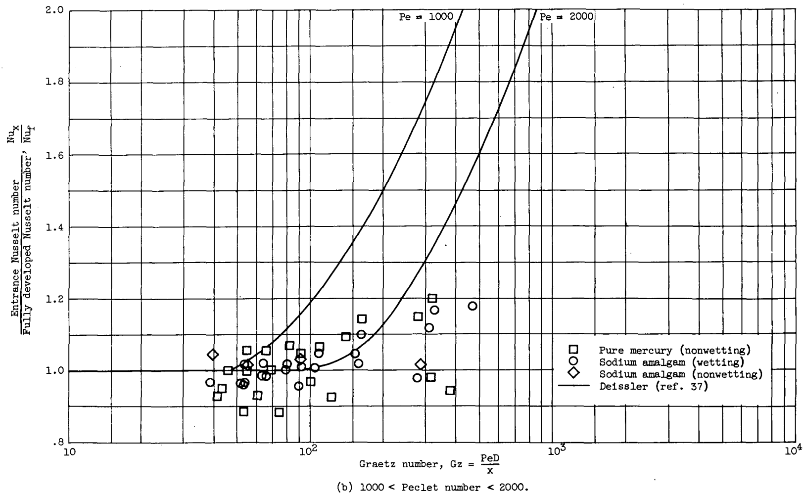
Figure 44. - Continued. Data of Stromquist (ref. 21) for entrance region heat transfer to mercury, with and without sodium additions, in round tubes.
