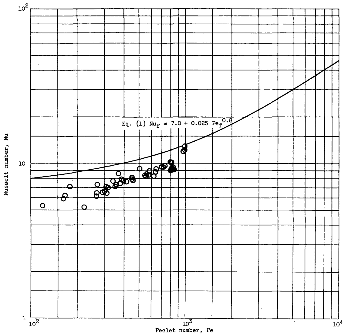
Figure 16. - Continued. Re-evaluated data of Lyon (ref. 6) for average heat transfer to a sodium-potassium alloy in round tubes.
