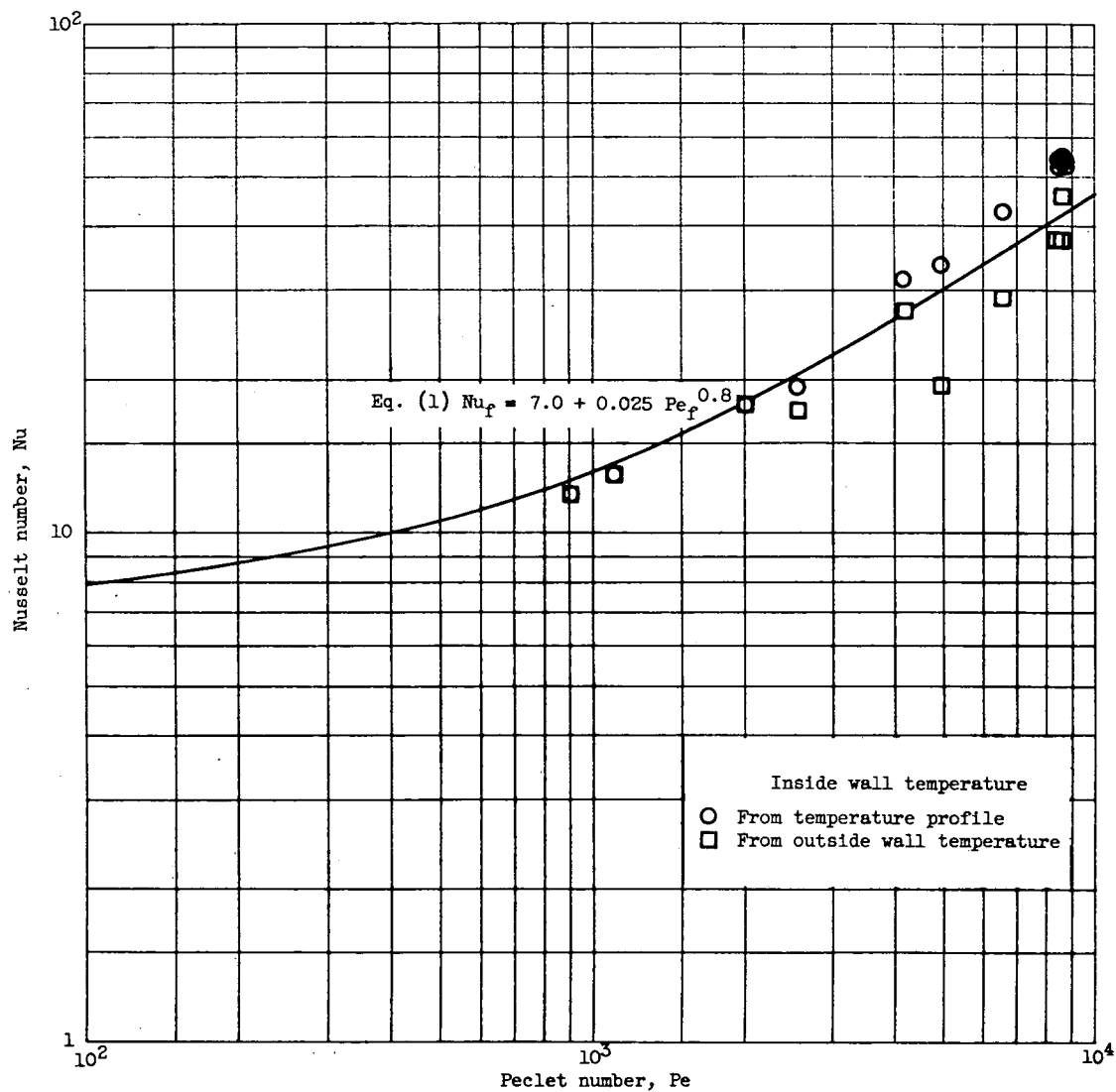
Figure 39. - Data of Isakoff and Drew (refs. 19 and 20) for fully developed heat transfer to mercury in round tubes.
