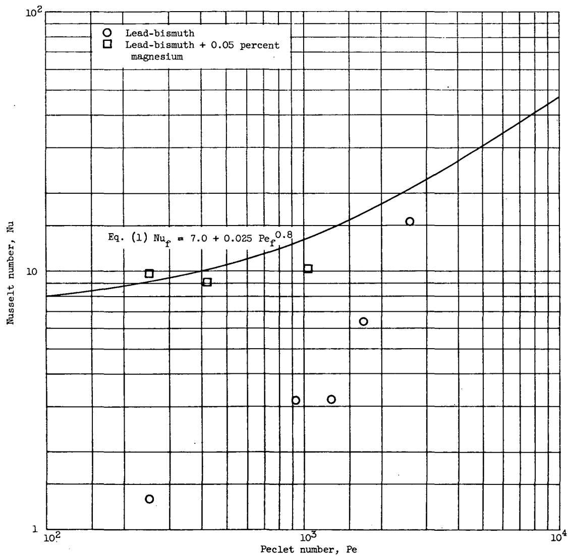
Figure 18. - Re-evaluated data of Untermeyer for fully developed heat transfer to lead-bismuth, with and without magnesium addition, in round tubes.
