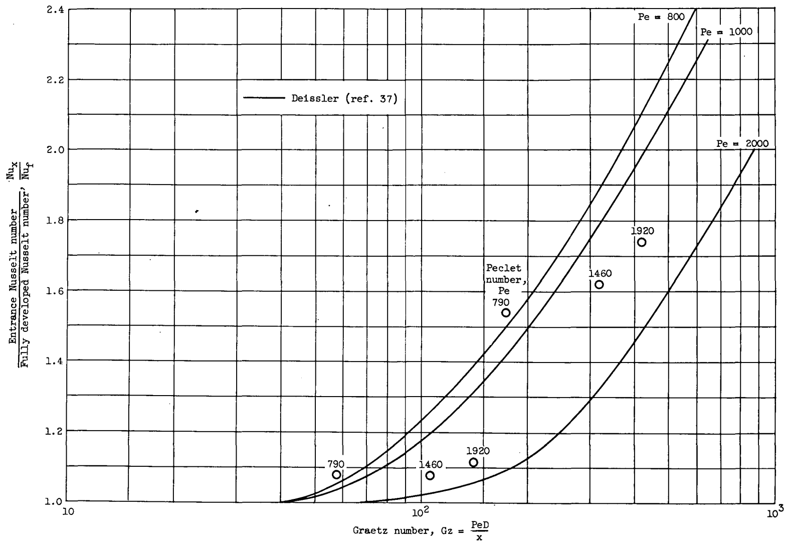
Figure 27. - Data of Seban (ref. 11) for entrance region heat transfer to lead-bismuth eutectic in round tubes.
