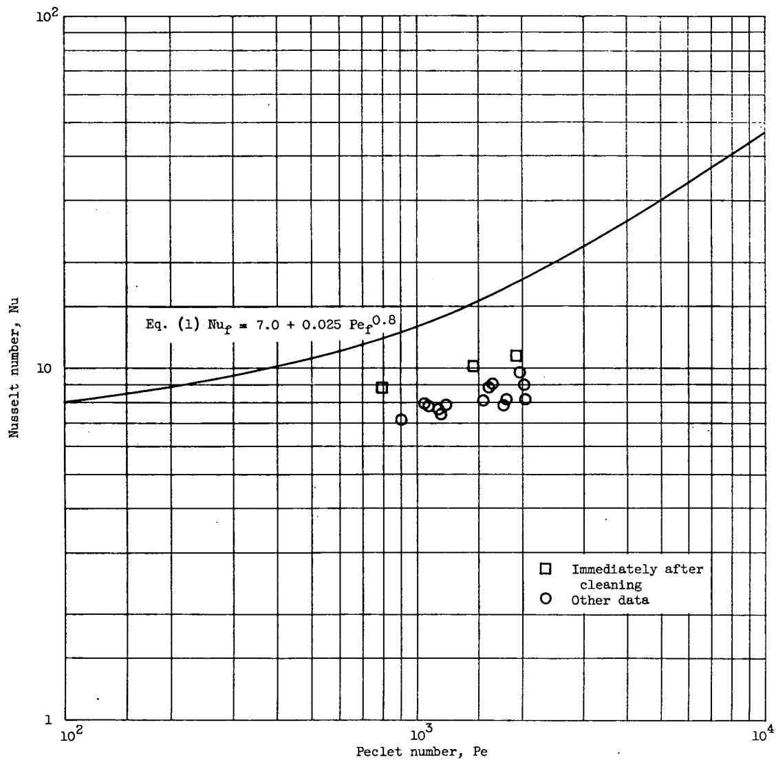
Figure 26. - Data of Seban (ref. 11) for fully developed heat transfer to lead-bismuth eutectic in round tubes.
