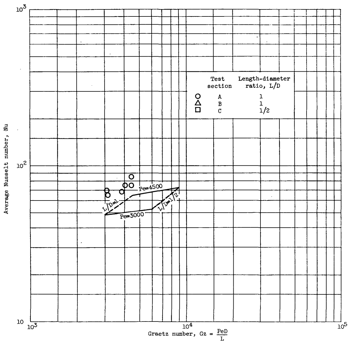
Figure 52. - Concluded. Data of Poppendiek and Harrison (ref. 26) for average heat transfer to mercury in very short round tubes compared with prediction of Deissler (ref. 37).
