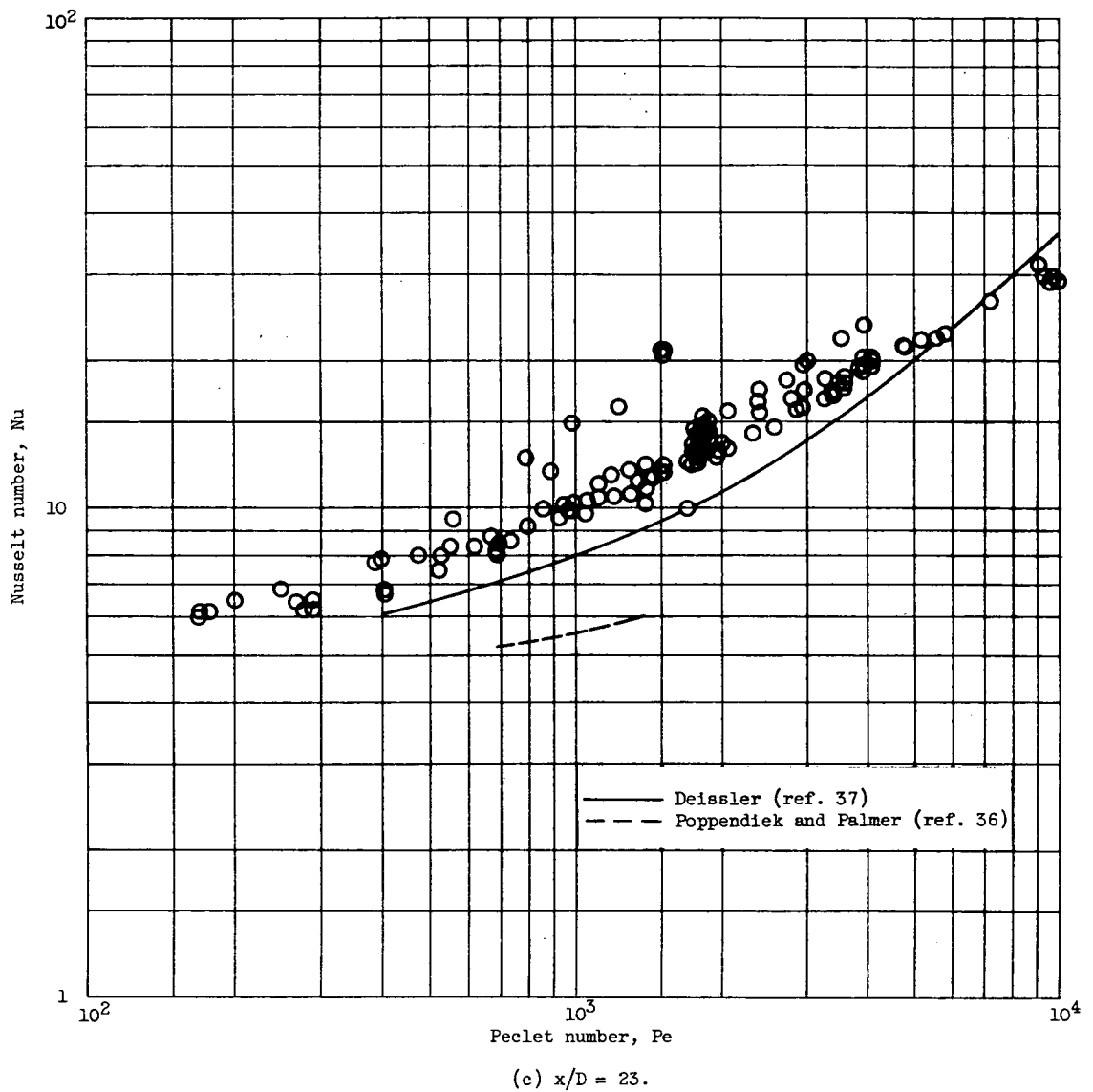
Figure 47. - Concluded. Data of Johnson, Hartnett, and Clabaugh (ref. 24) for entrance region heat transfer to mercury in round tubes.
