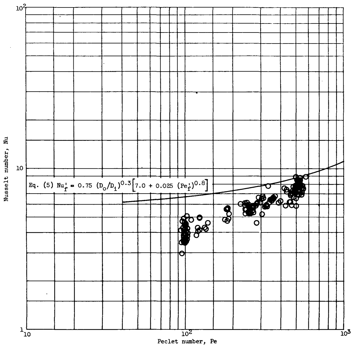
Figure 17. - Re-evaluated data of Lyon (ref. 6) for average heat transfer to a sodium-potassium alloy in annuli.
