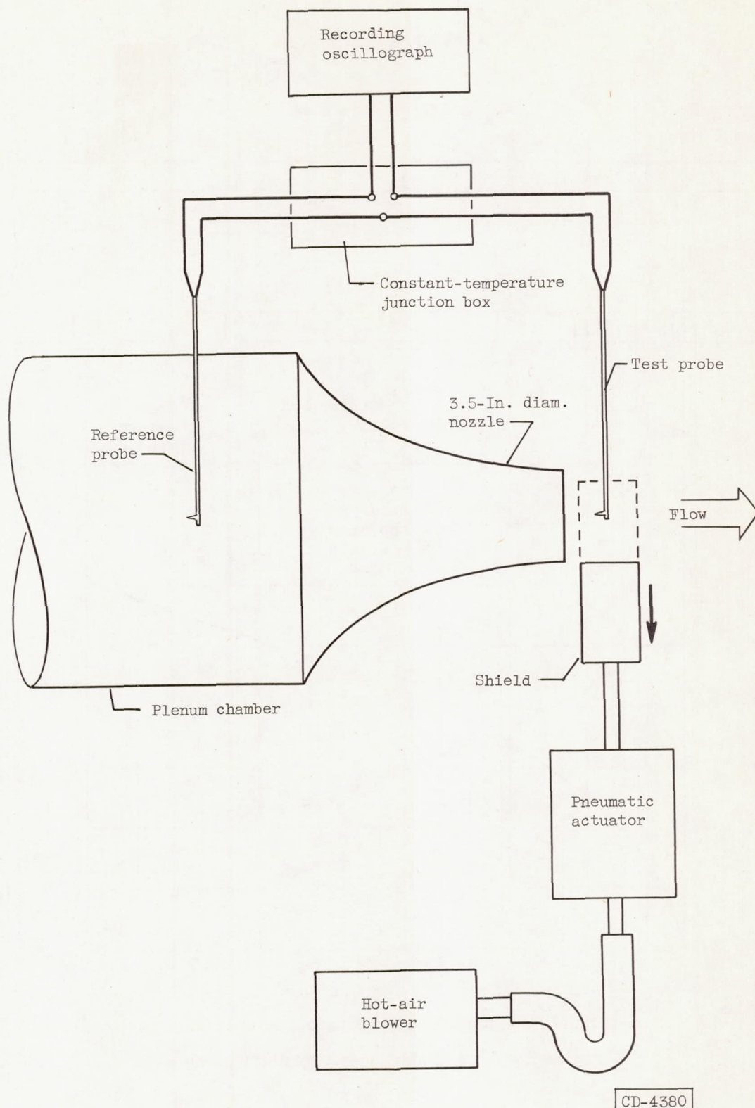
Figure 2. - Time-response apparatus.
