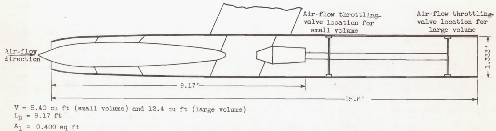
(d) 16-inch ram-jet engine (diffuser illustrated in fig. 3(f)) employed in 8- by 6-foot supersonic-tunnel experiments.
