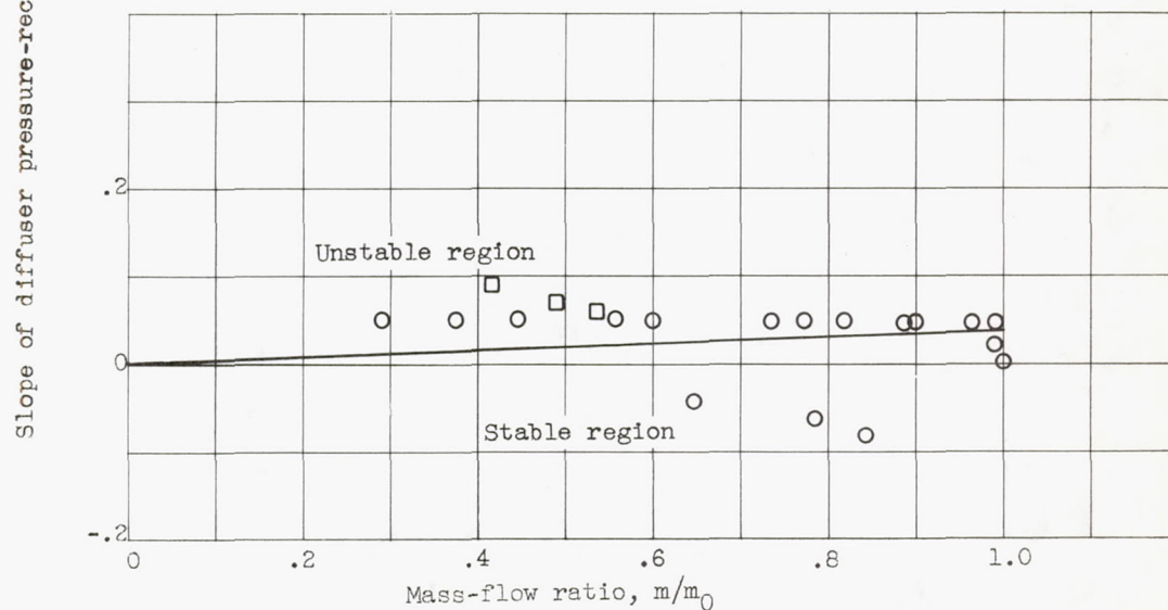
(b) Free-stream Mach number, 1.99.
