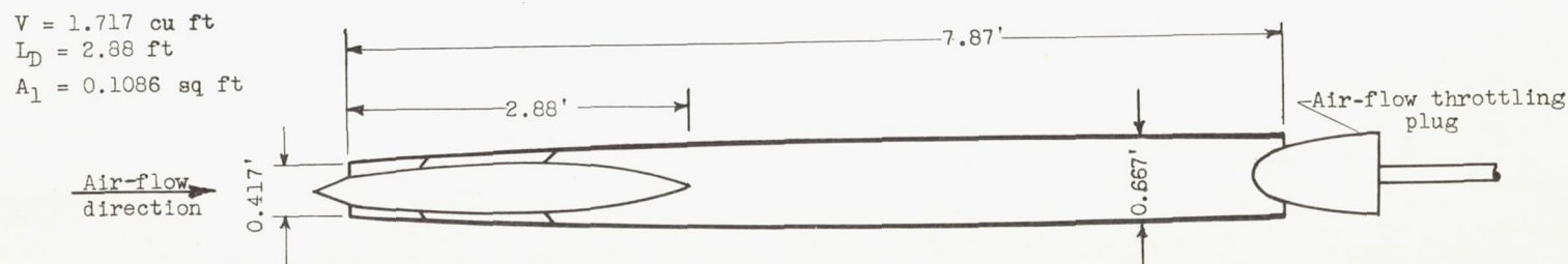
(b) 8-inch ram-jet engine (diffuser illustrated in fig. 3(b)) employed in 20-inch supersonic tunnel experiments.
