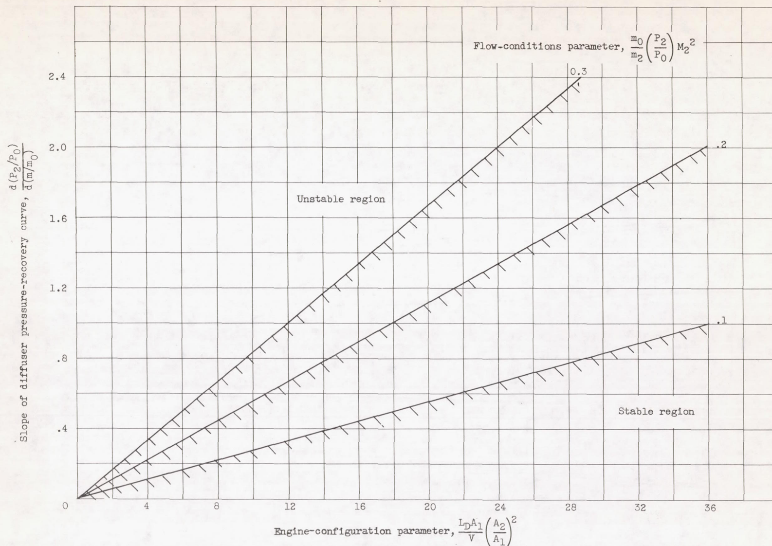
Figure 2. - Theoretical stability criterions without heat addition; \gamma_2 = 1.4 .
