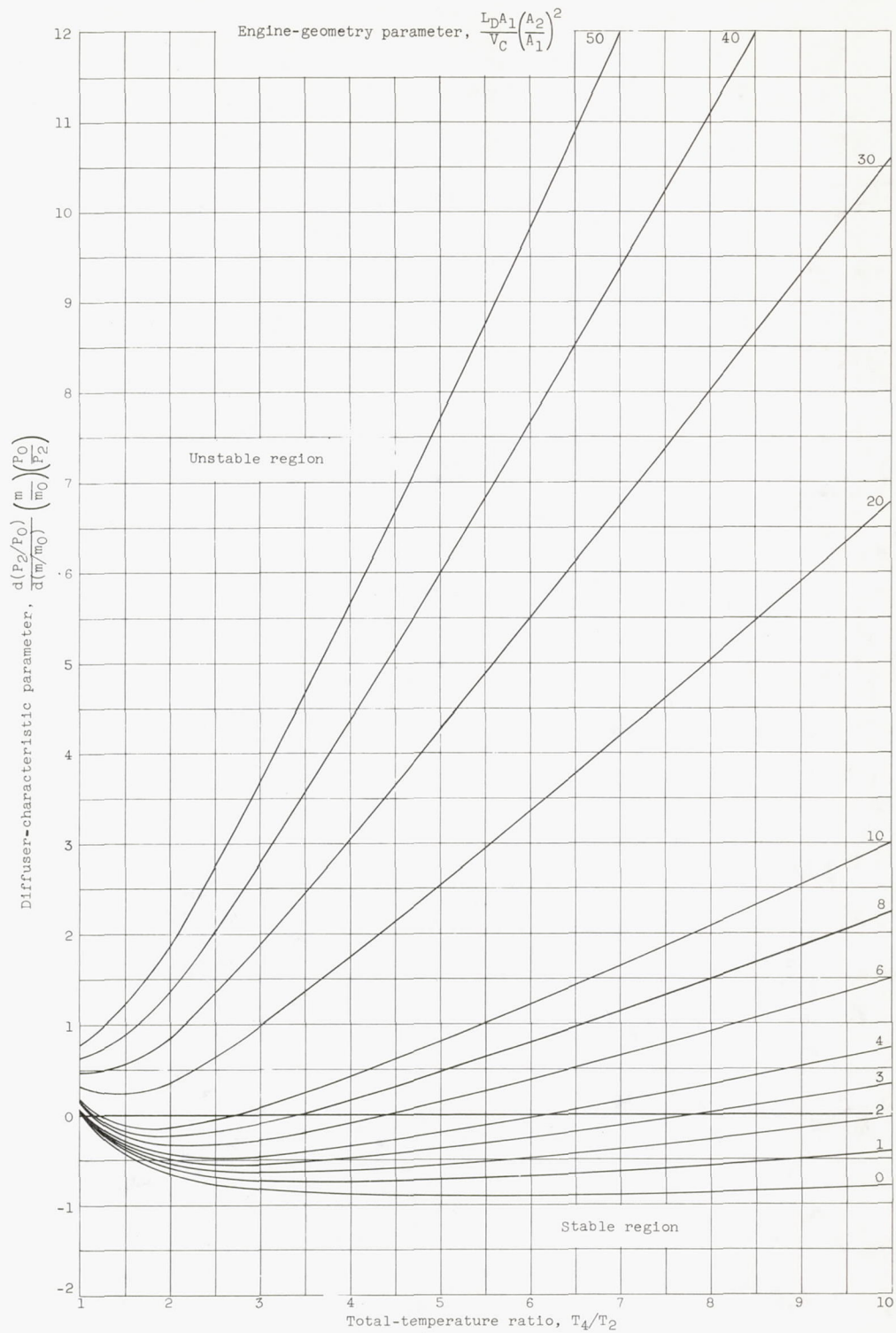
Figure 16. - Theoretical stability criterions with heat addition. V_D/V_C = 0 ; \gamma_2 = 1.4 ; \gamma_4 = \gamma_2 - 0.03 ( - 1).
