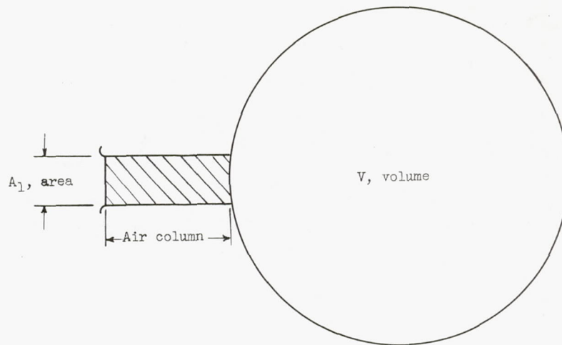
(a) Helmholtz resonator.
