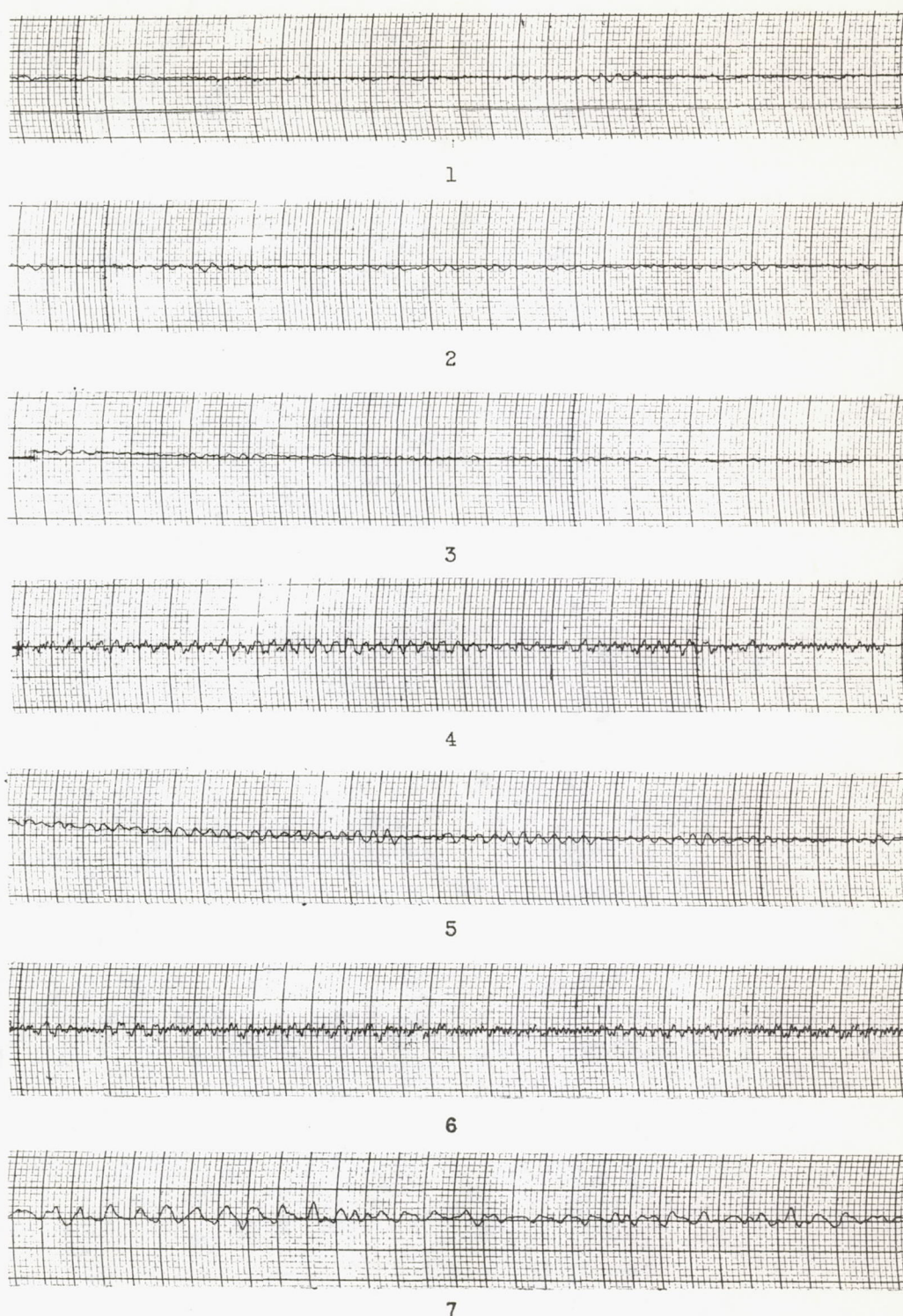
Figure 20. - Pressure oscillation traces in 16-inch ram jet at various mass-flow ratios using gasoline as fuel. Free-stream Mach number, 1.77.
