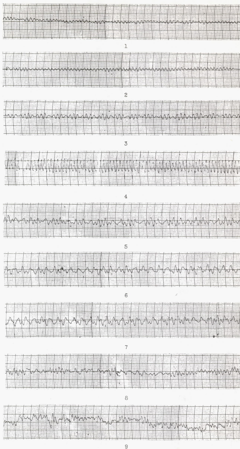
Figure 23. - Pressure oscillation traces in 16-inch ram jet at various mass-flow ratios using kerosene - propylene-oxide fuel blend. Free-stream Mach number, 1.58.
