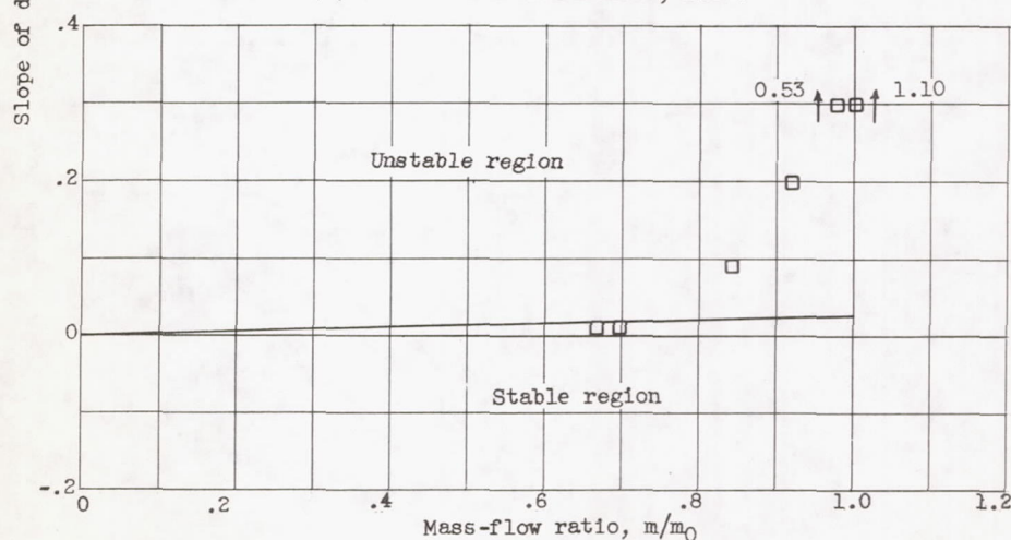
(c) Free-stream Mach number, 2.00.
