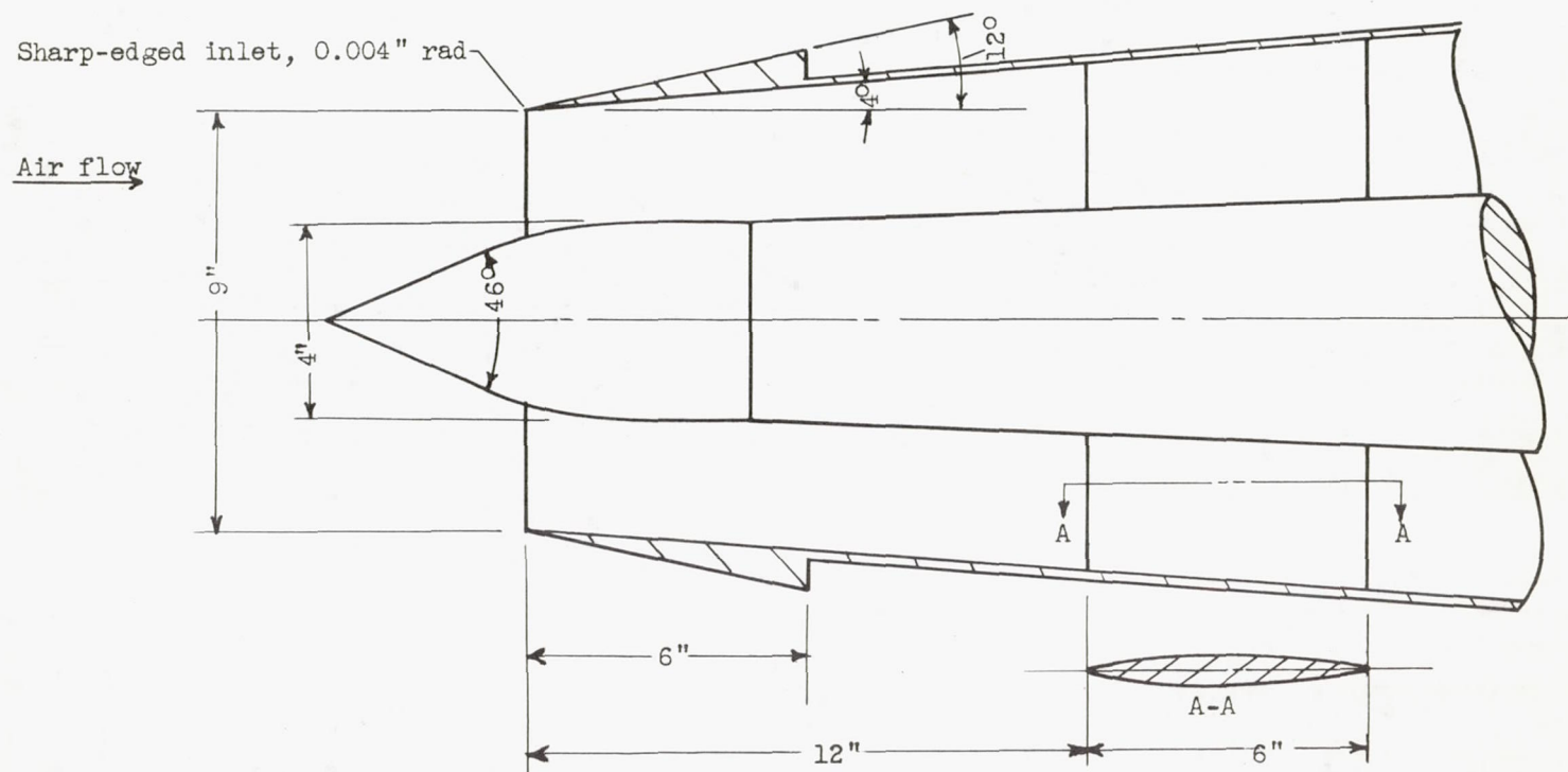
(a) Diffuser employed on 16-inch ram jet studied in supersonic free jet. All external supersonic compression.
