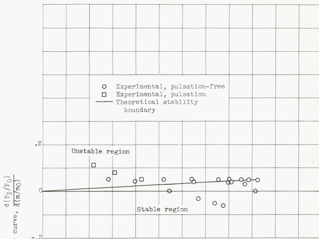
(a) Free-stream Mach number, 1.79.
