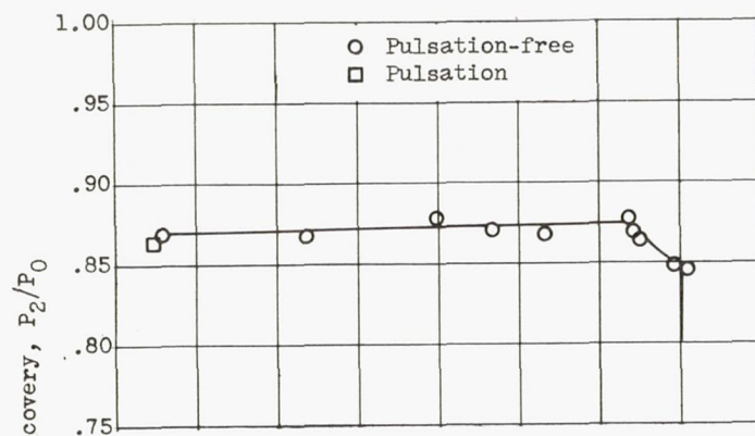
(a) Spike projection, 4.18 inches.
