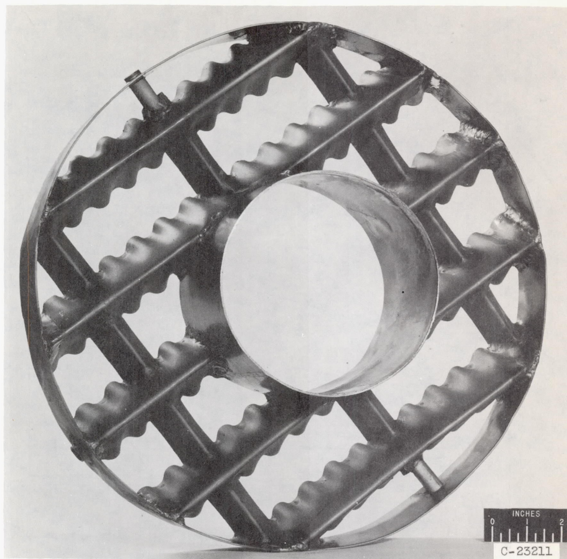
(a) Upstream view of corrugated-gutter flame holder.
