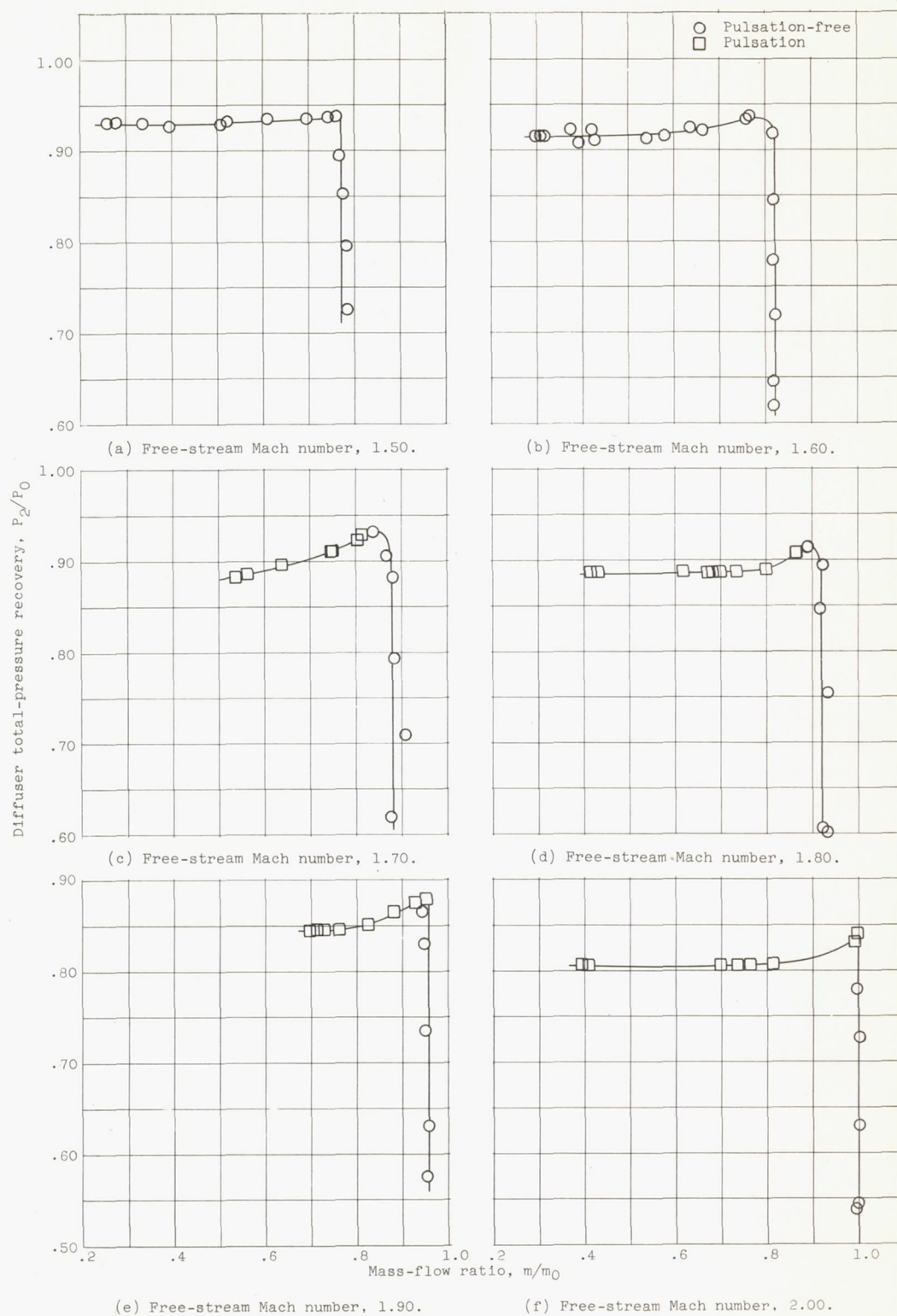
Figure 7. - Diffuser pressure recovery as function of engine mass-flow ratio for ram jet with small volume showing occurrence of flow pulsations at various free-stream Mach numbers; 16-inch ram jet in 8- by 6-foot supersonic tunnel.
