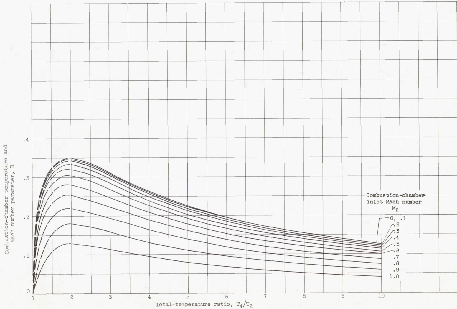
(b) Combustion-chamber temperature and Mach number parameter, R .
