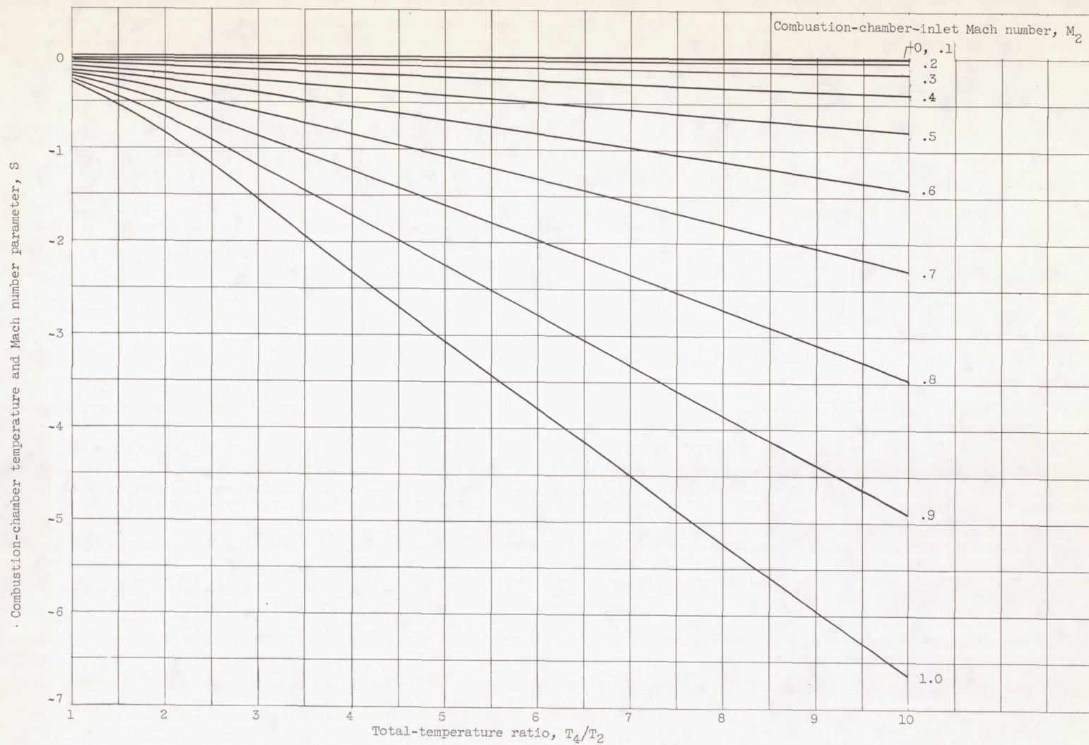
(c) Combustion-chamber temperature and Mach number parameter, S .
