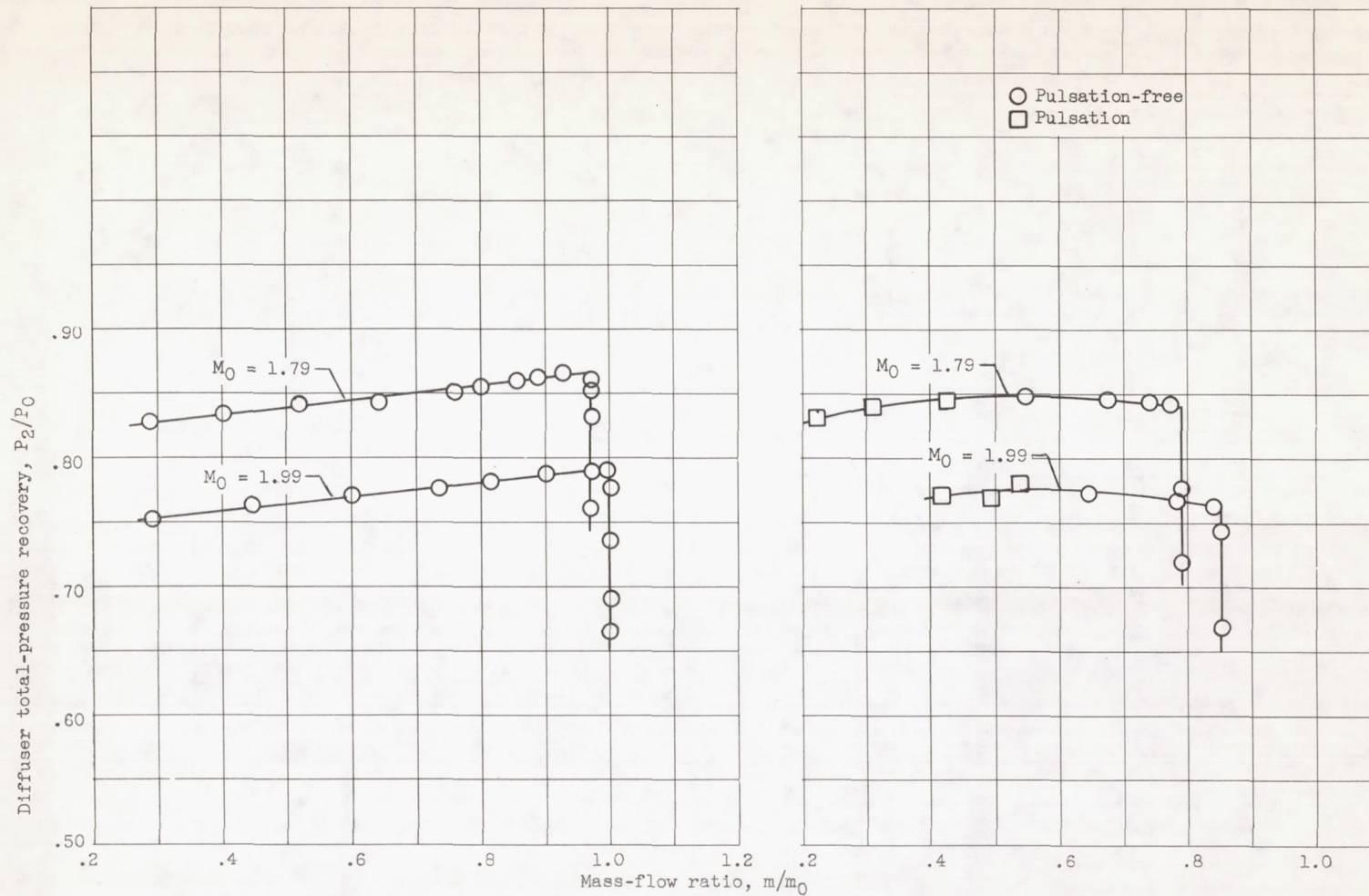
(c) Single-shock 50^\circ cone; external compression; sharp-edged inlet; 8- by 6-foot supersonic tunnel.
