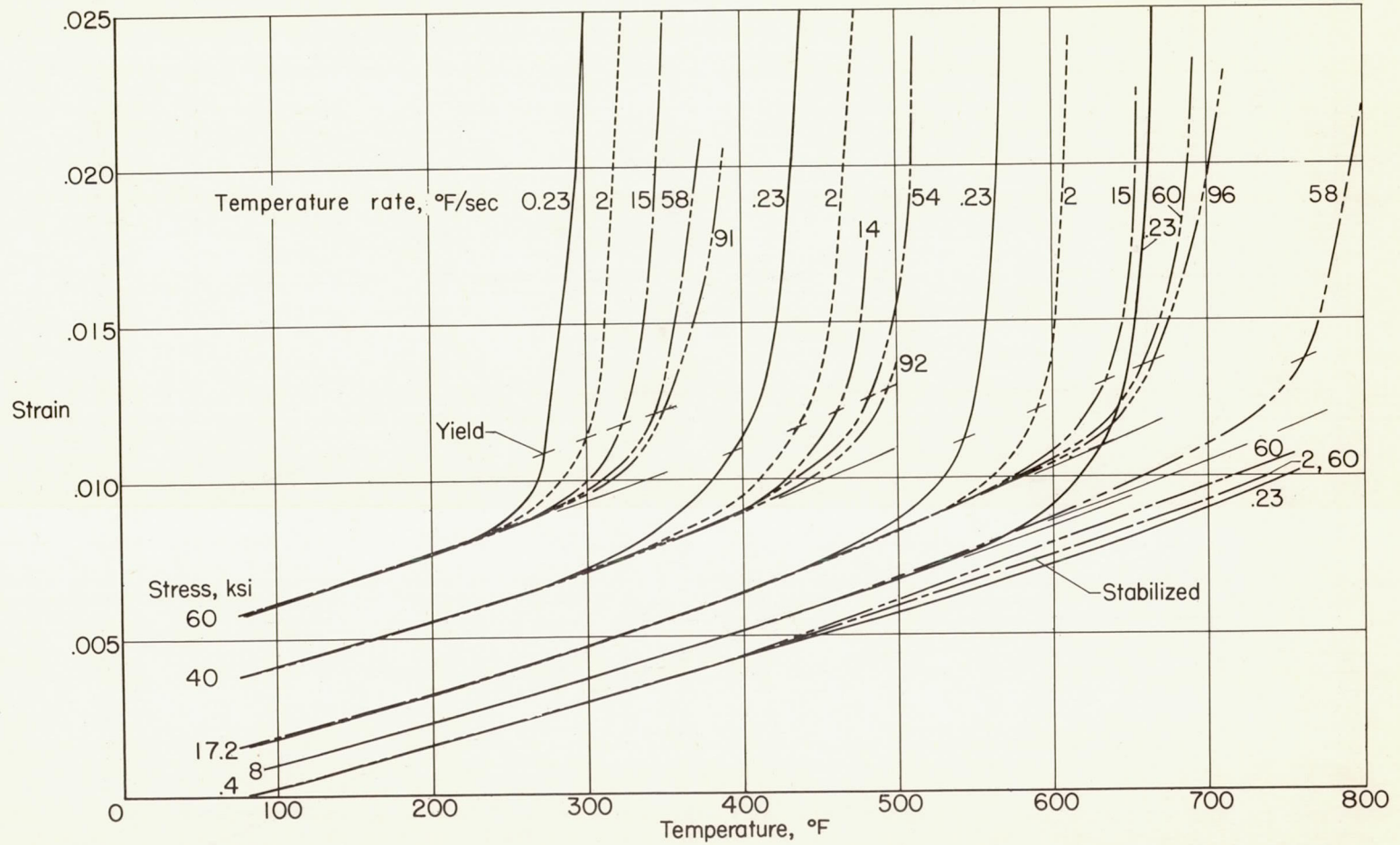
Figure 10.- Strain-temperature histories of 7075-T6 aluminum alloy for temperature rates from 0.2° F to 100° F per second for various stresses.
