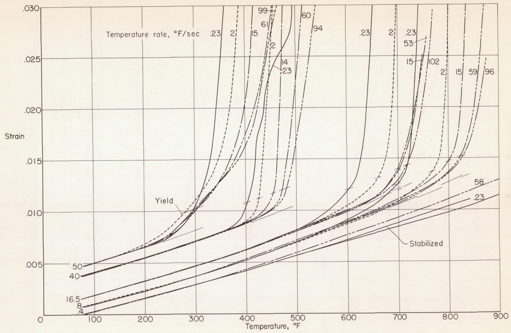
Figure 11.- Strain-temperature histories of 2024-T3 aluminum alloy for temperature rates from 0.2° F to 100° F per second for various stresses.
