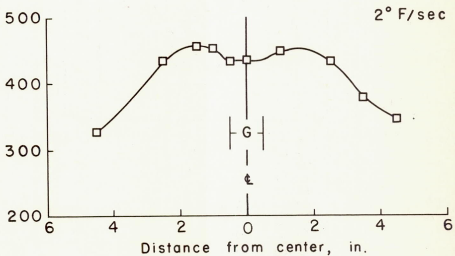
Figure 6.- Temperature gradients along length of rapid-heating specimen for temperature rates of 2° F and 110° F per second. Gage length is designated as G.
