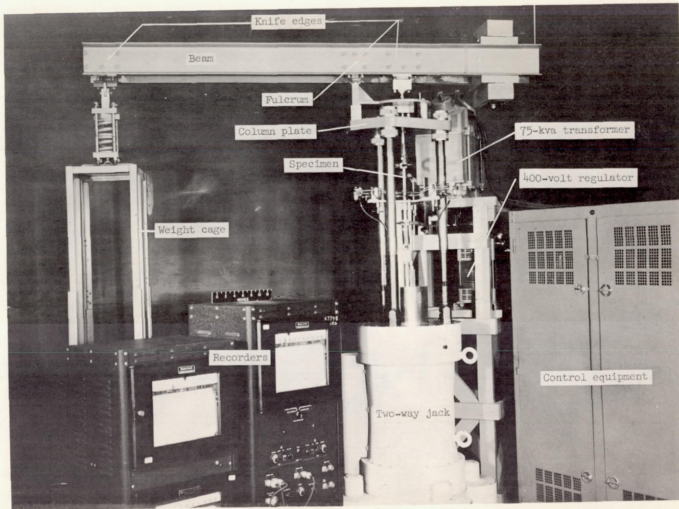
Figure 2.- General arrangement of loading, heating, controlling, and recording equipment for rapid-heating tests.
