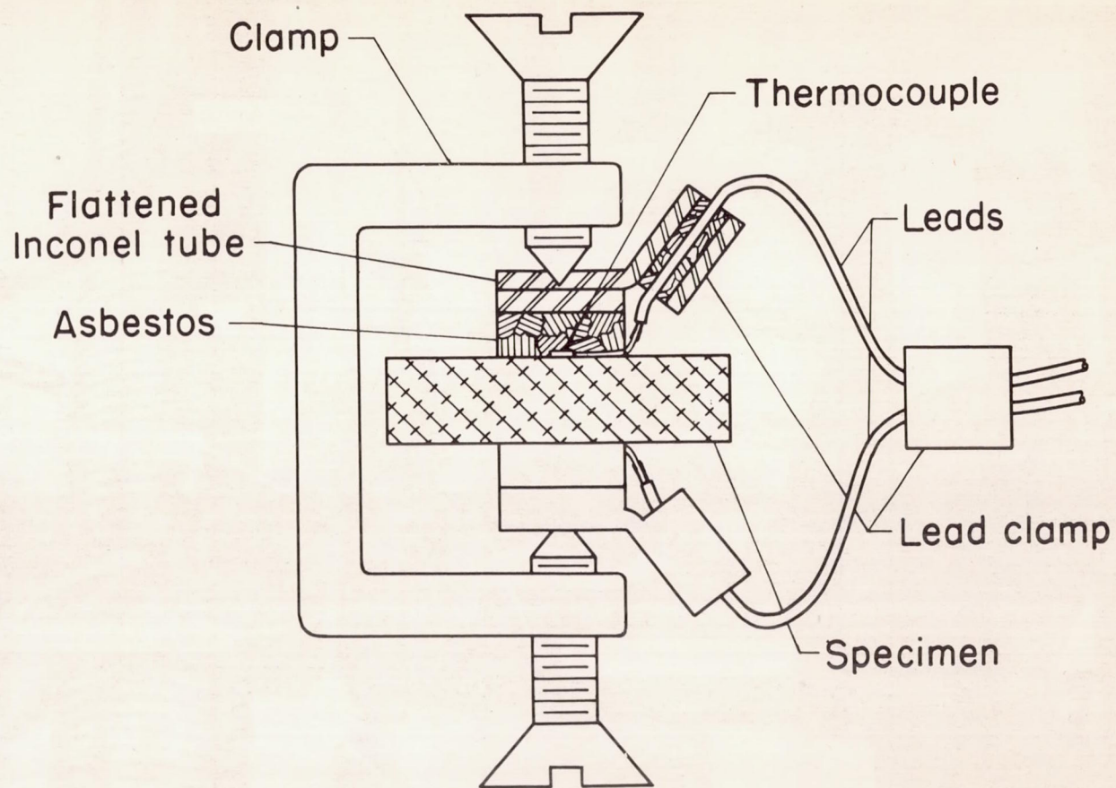
Figure 5.- Arrangement of specimen, thermocouple, and mounting clamp at midposition.
