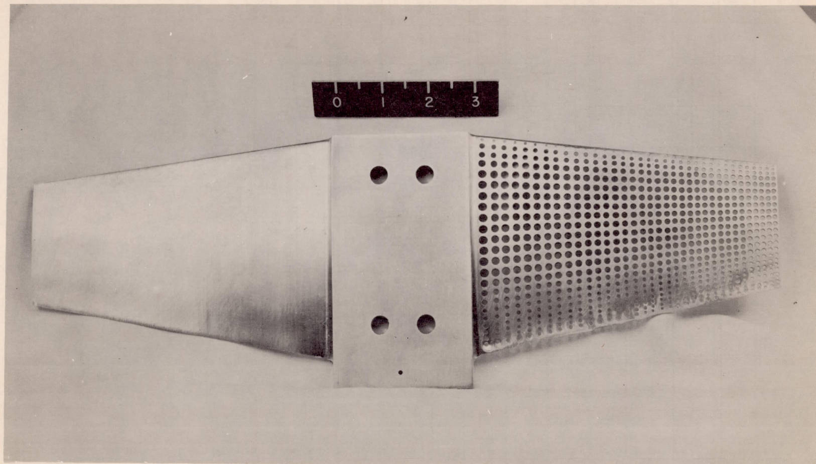
Figure 10.- Tapered-wing model showing one panel drilled. L-83459
