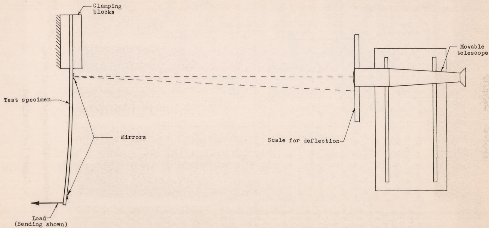
Figure 2.- Schematic diagram of stiffness-measuring setup.
