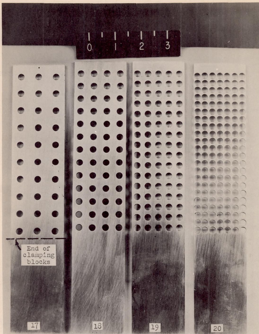
(a) Specimens with square patterns. L-83458.1
