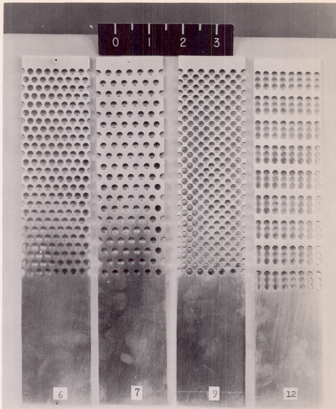
(b) Specimens with staggered patterns. L-83457.1
