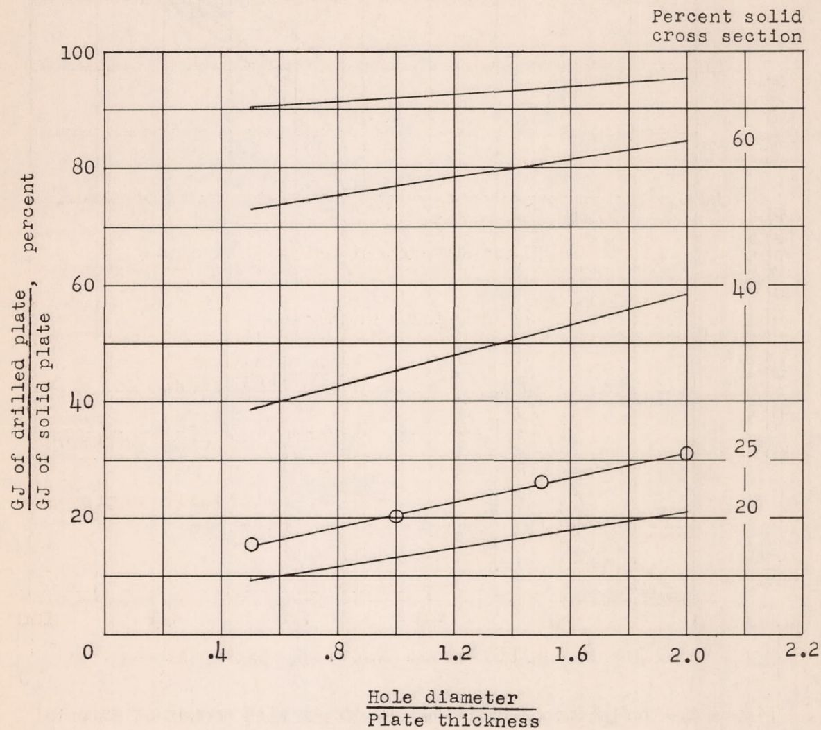
Figure 6.- Effect of ratio of hole diameter to plate thickness on torsional stiffness.
