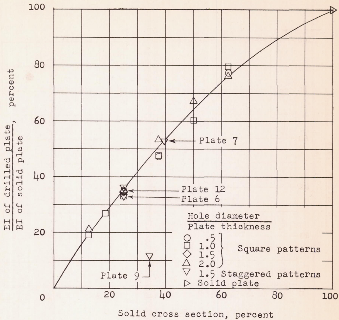
Figure 3.- Variation of bending stiffness with amount of material remaining.
