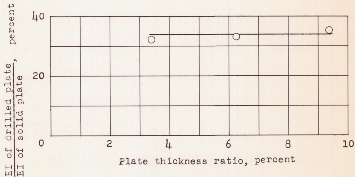
(b) Bending stiffness.
