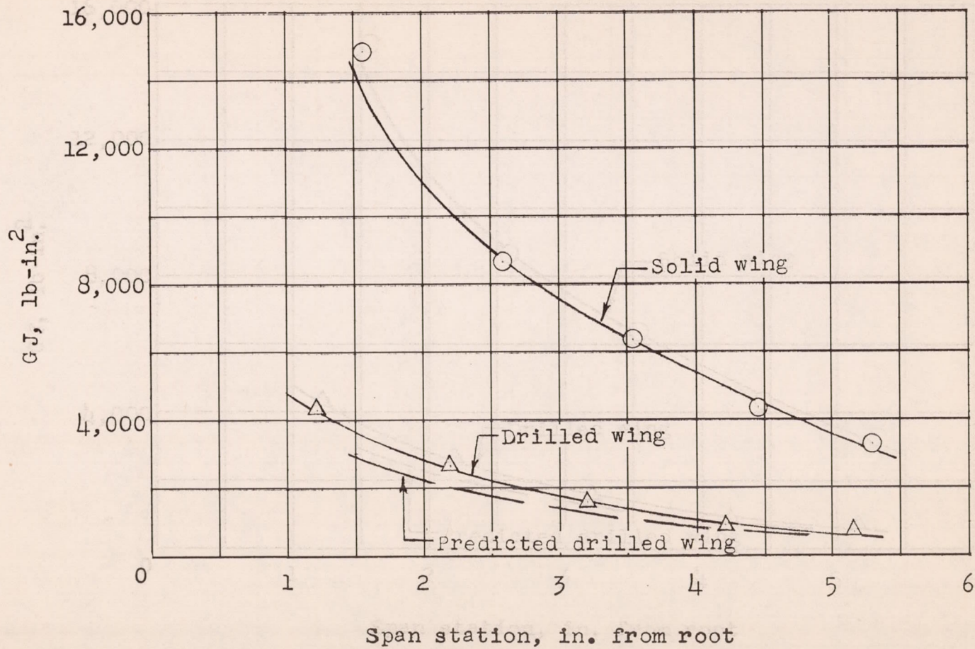
Figure 12.- Torsional stiffnesses of solid and drilled wings.
