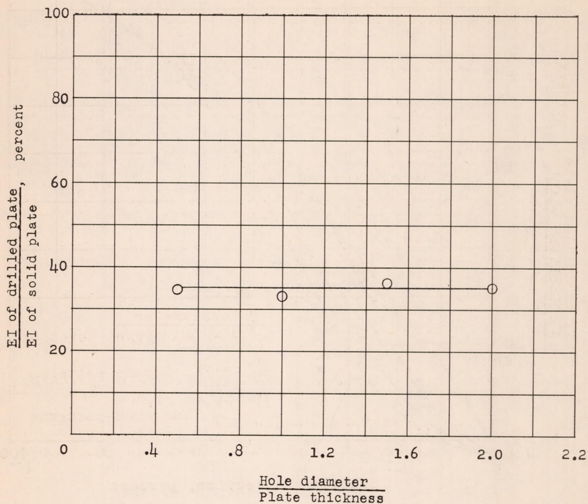
Figure 4.- Effect of ratio of hole diameter to plate thickness on bending stiffness. 25 percent solid cross section.
