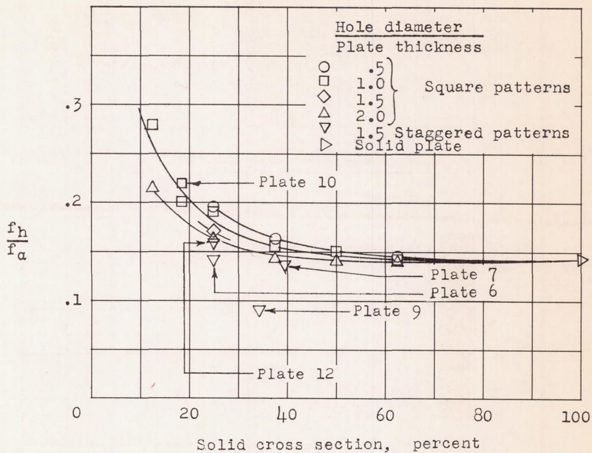
Figure 9.- Variation of frequency ratio with amount of material remaining.
