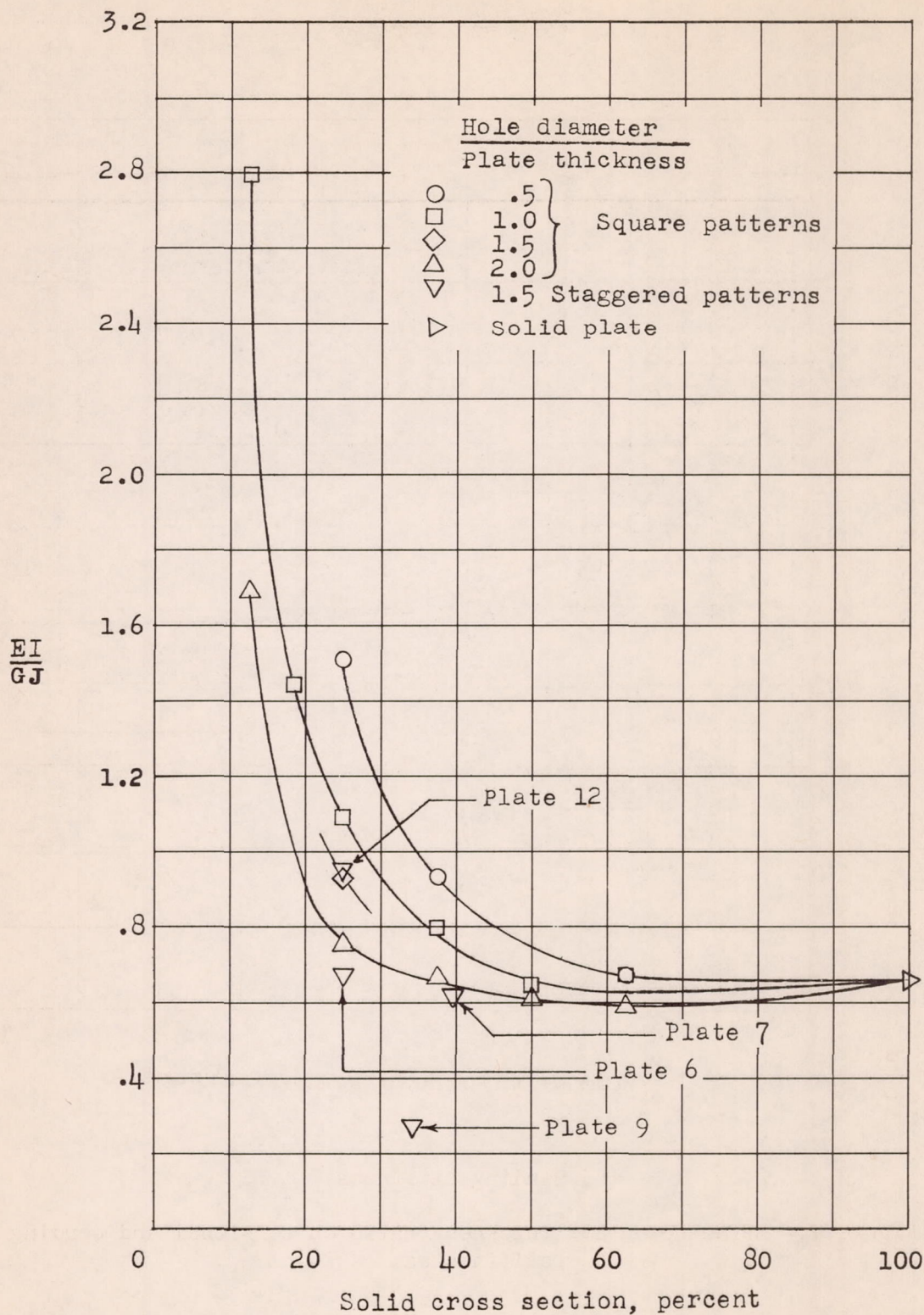
Figure 8.- Variation of ratio of bending to torsional stiffness with amount of material remaining.
