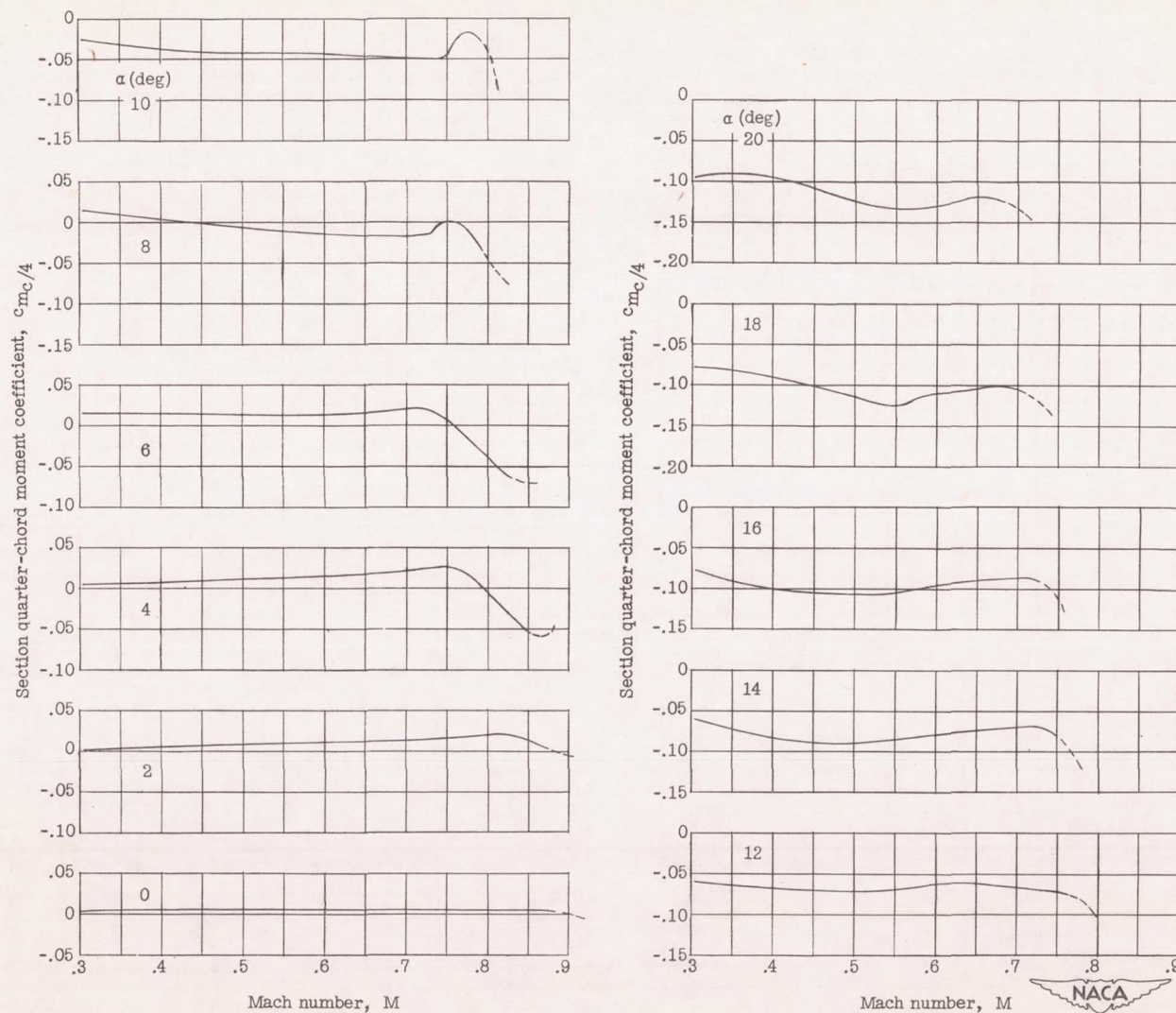
(a) NACA 16-006 airfoil.
