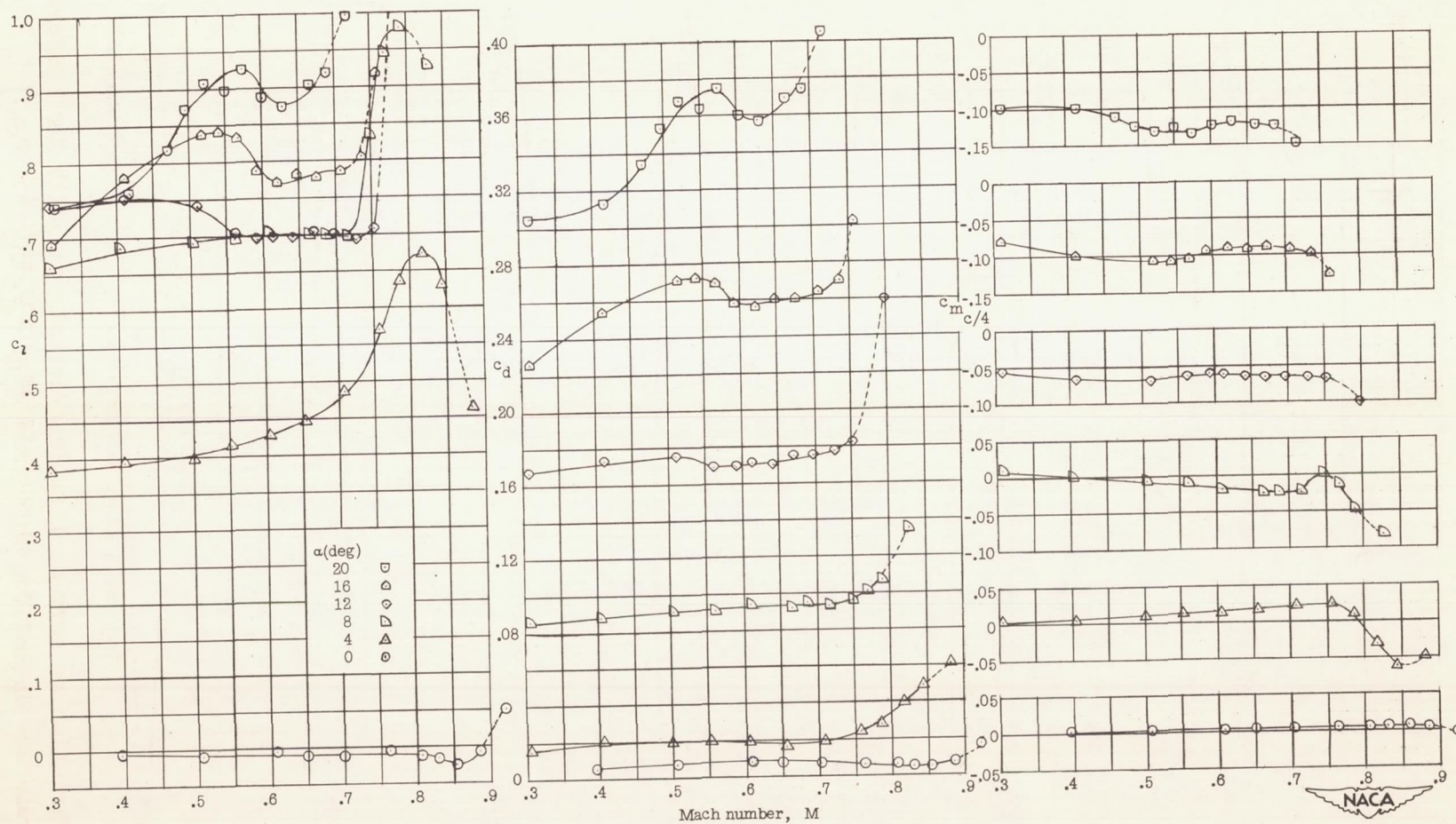
Figure 2.- Representative variations with Mach number of the force characteristics of the NACA 16-006 airfoil. (Curves are dashed for data from (M_{ch} - 0.030) to M_{ch} .)
