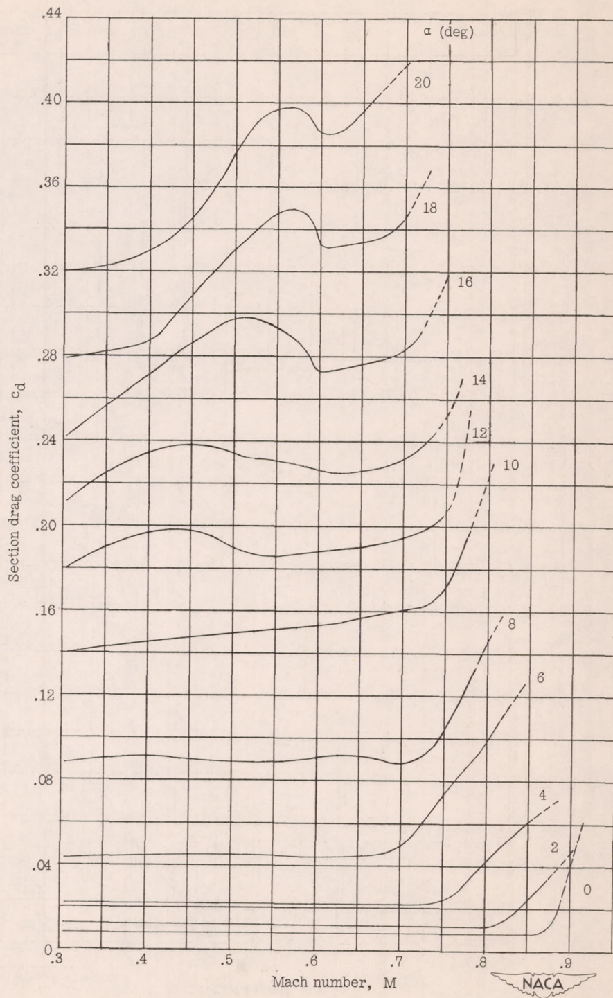
(b) NACA 66-006 airfoil.
