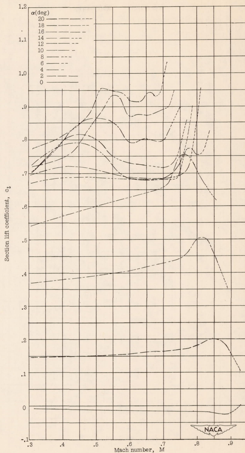
(e) C-5 airfoil.
