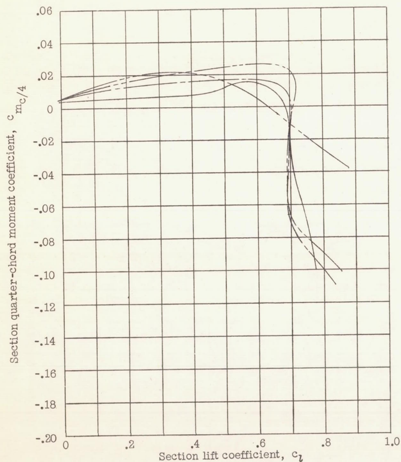
(a) NACA 16-006 airfoil.
