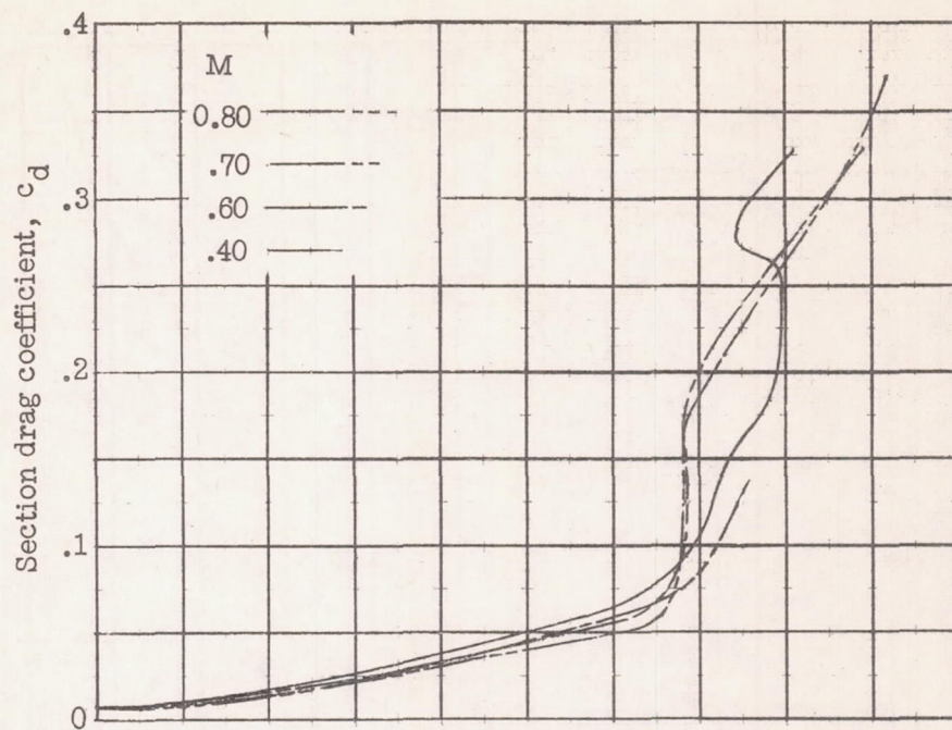
(e) C-5 airfoil.
