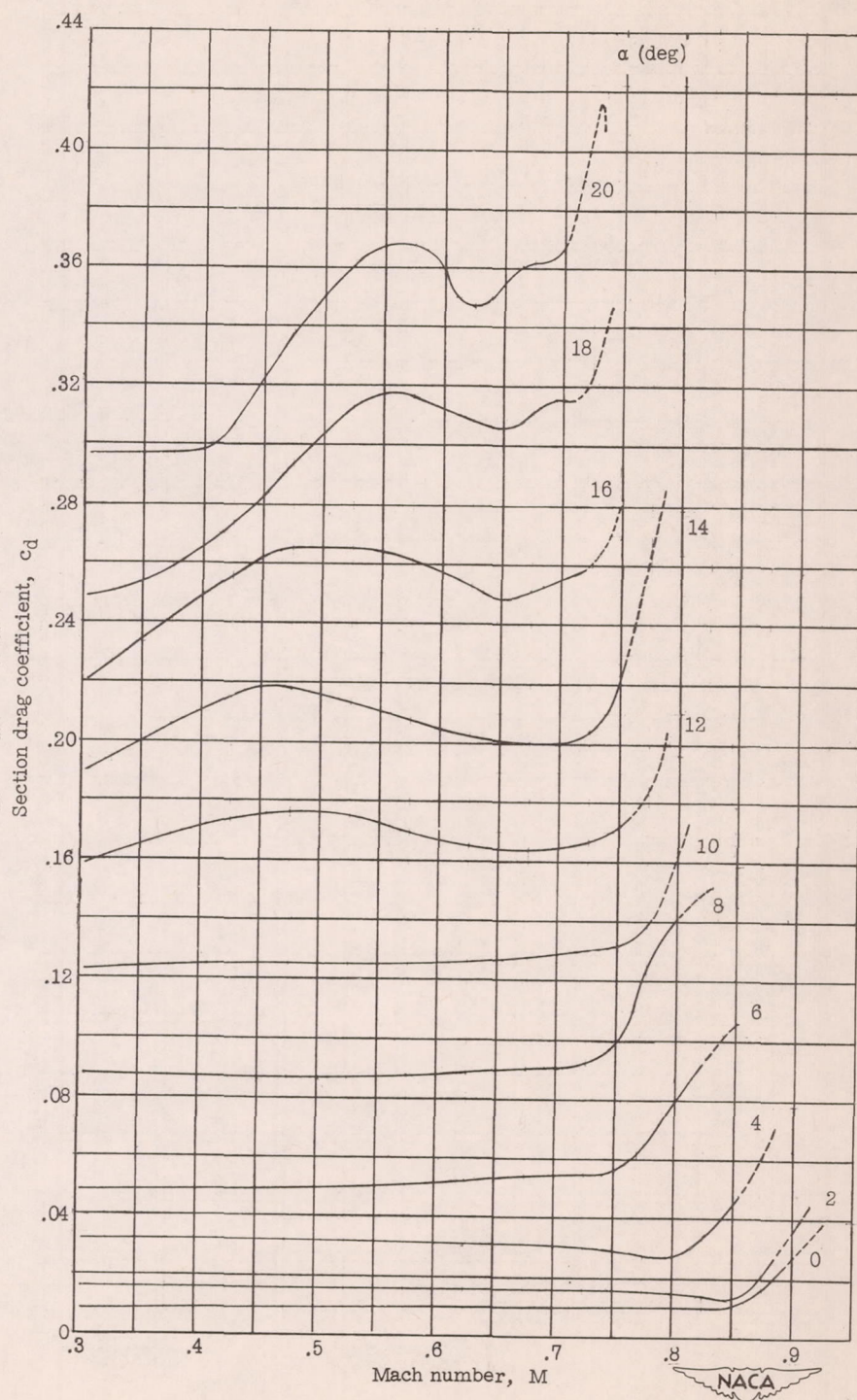
(f) C-7 airfoil.
