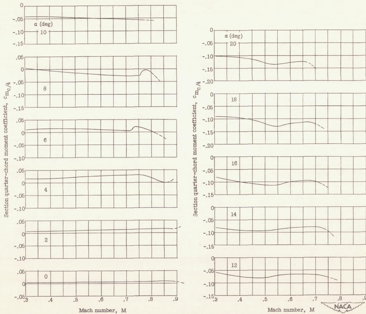
(e) C-5 airfoil.
