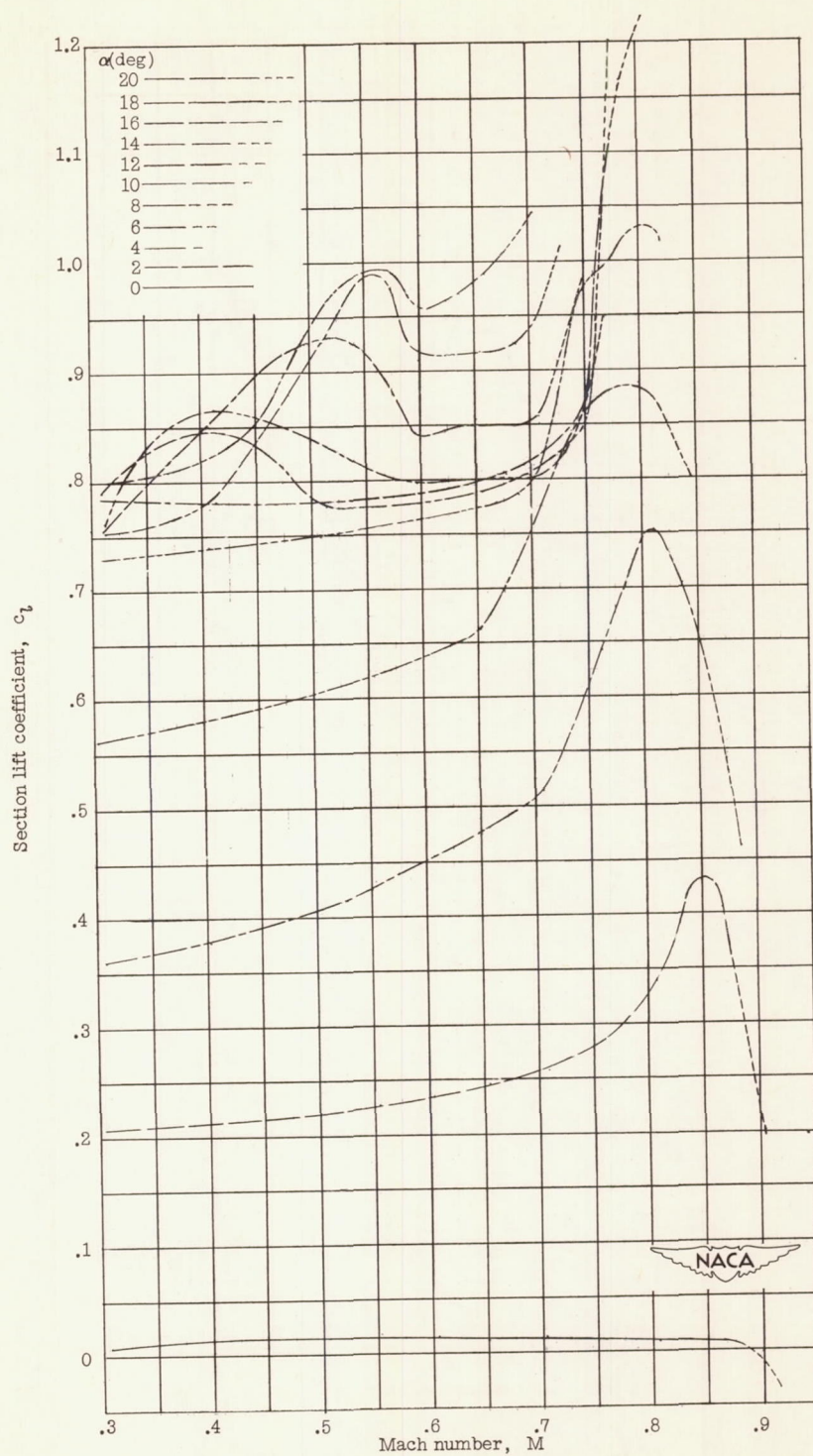
(b) NACA 66-006 airfoil.
