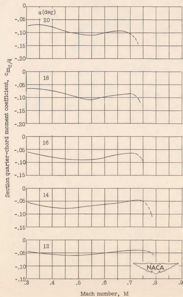
(f) C-7 airfoil.
