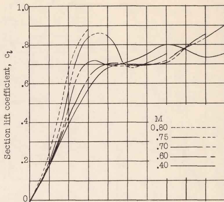
(a) NACA 16-006 airfoil.
