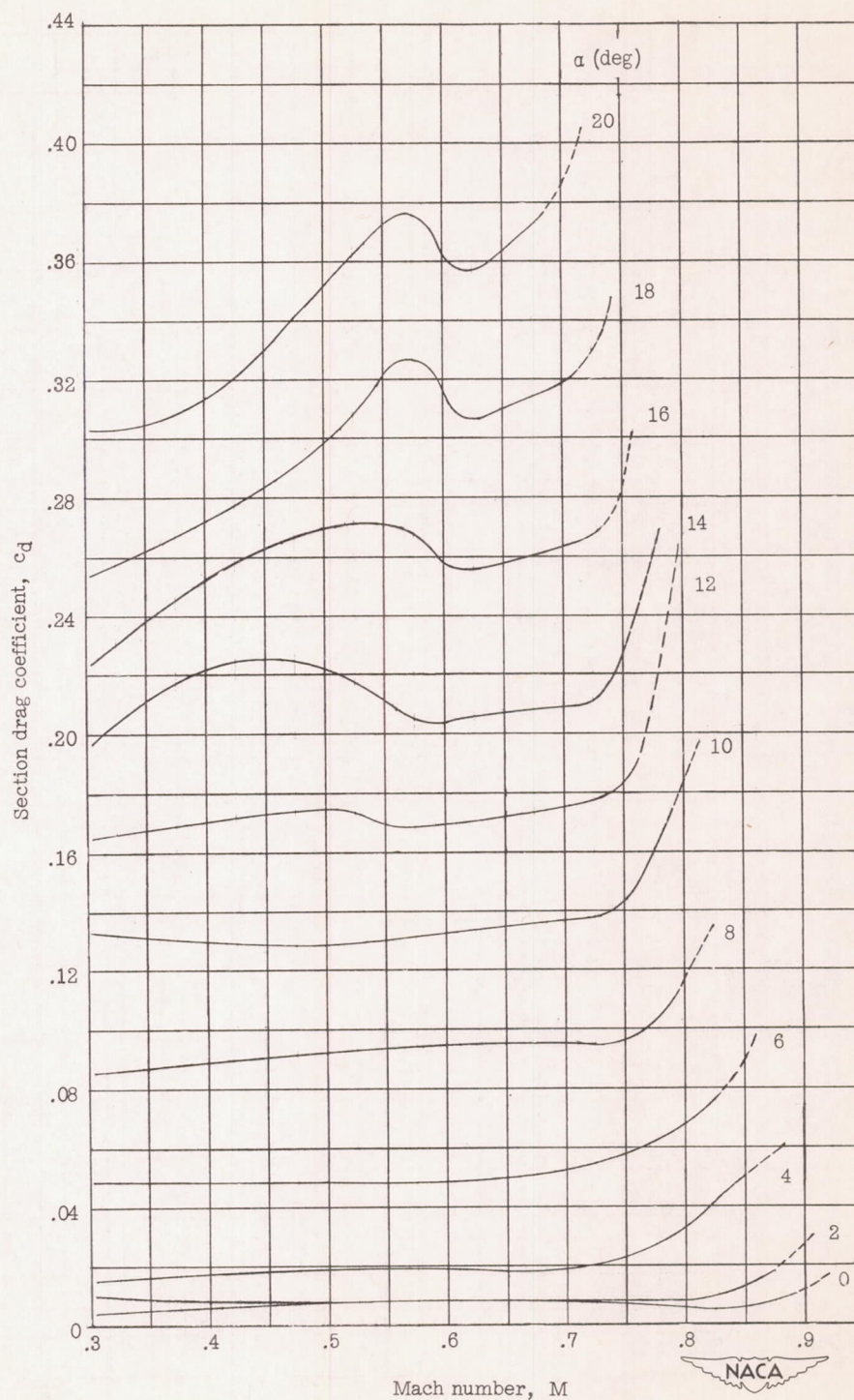
(a) NACA 16-006 airfoil.
