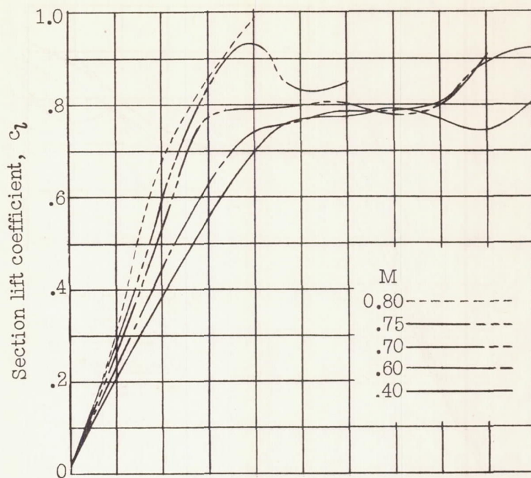
(c) NACA 0006-63 airfoil.
