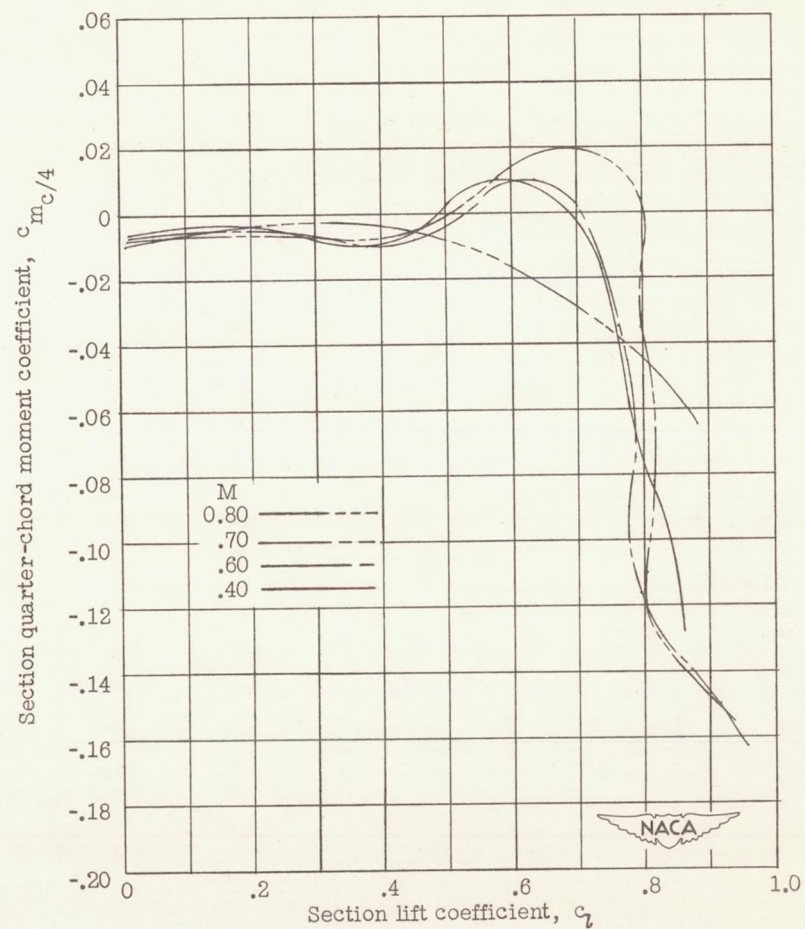
(b) NACA 66-006 airfoil.
