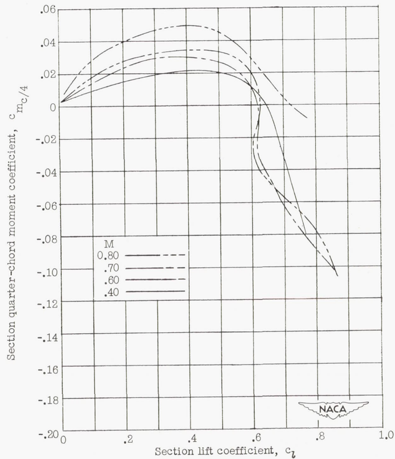
(f) C-7 airfoil.
