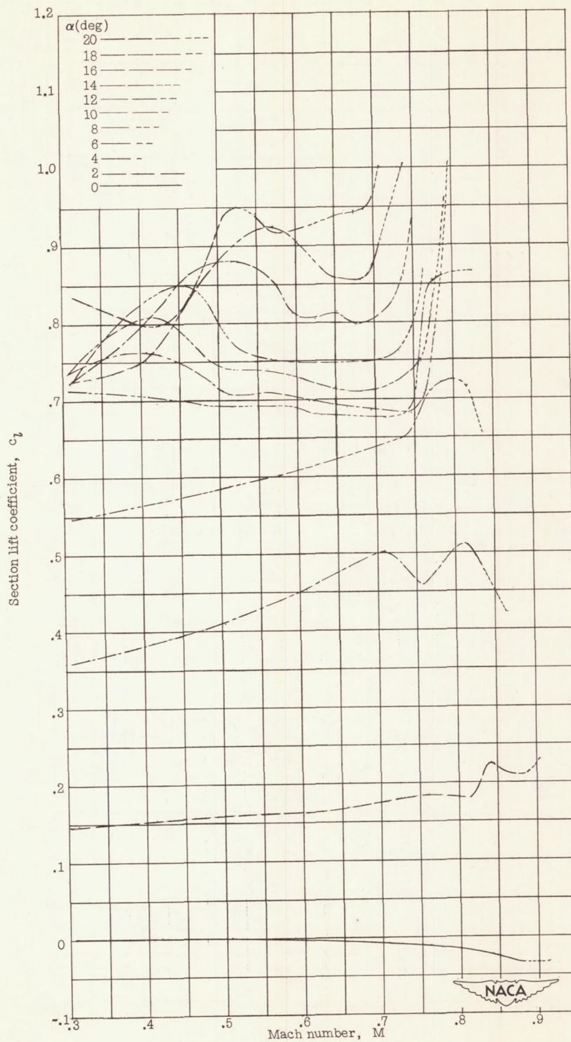
(h) W-7 airfoil.
