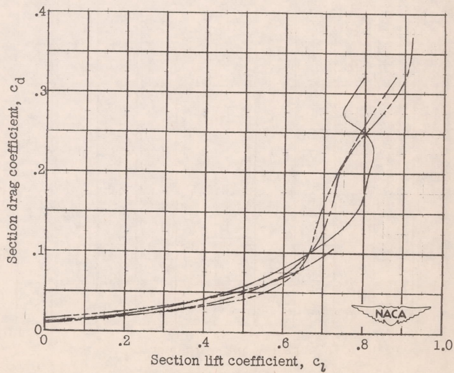
(h) W-7 airfoil.
