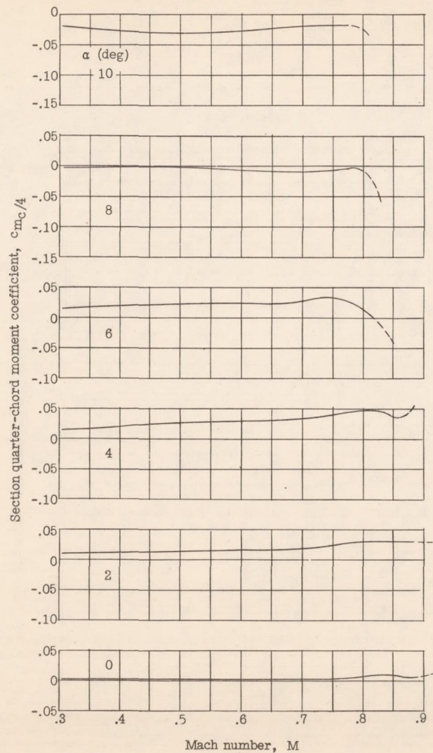
(f) C-7 airfoil.
