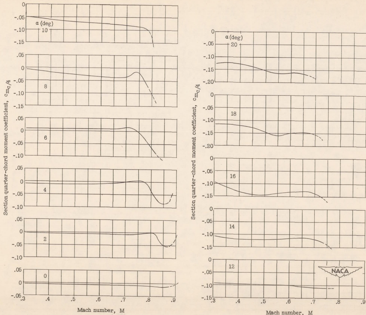
(b) NACA 66-006 airfoil.
