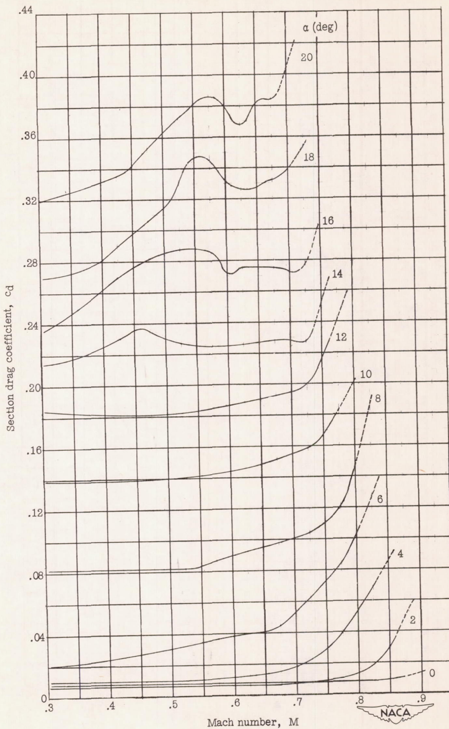
(c) NACA 0006-63 airfoil.
