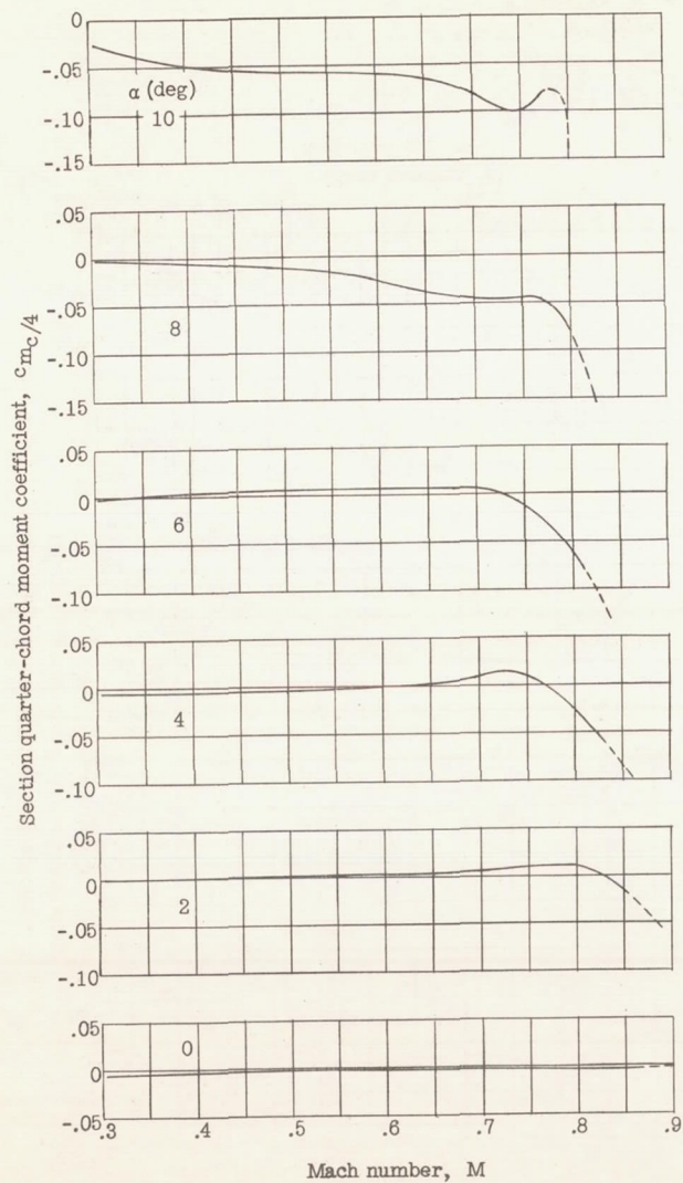
(c) NACA 0006-63 airfoil.
