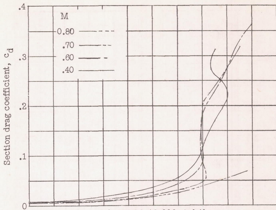
(a) NACA 16-006 airfoil.
