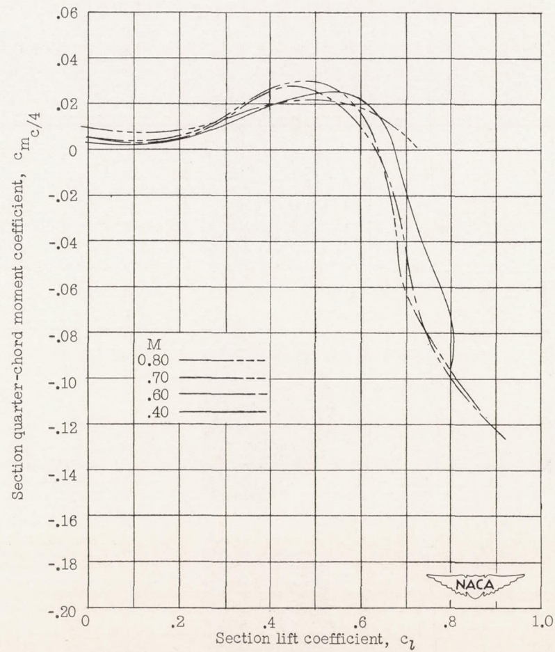
(h) W-7 airfoil.
