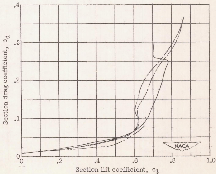
(f) C-7 airfoil.
