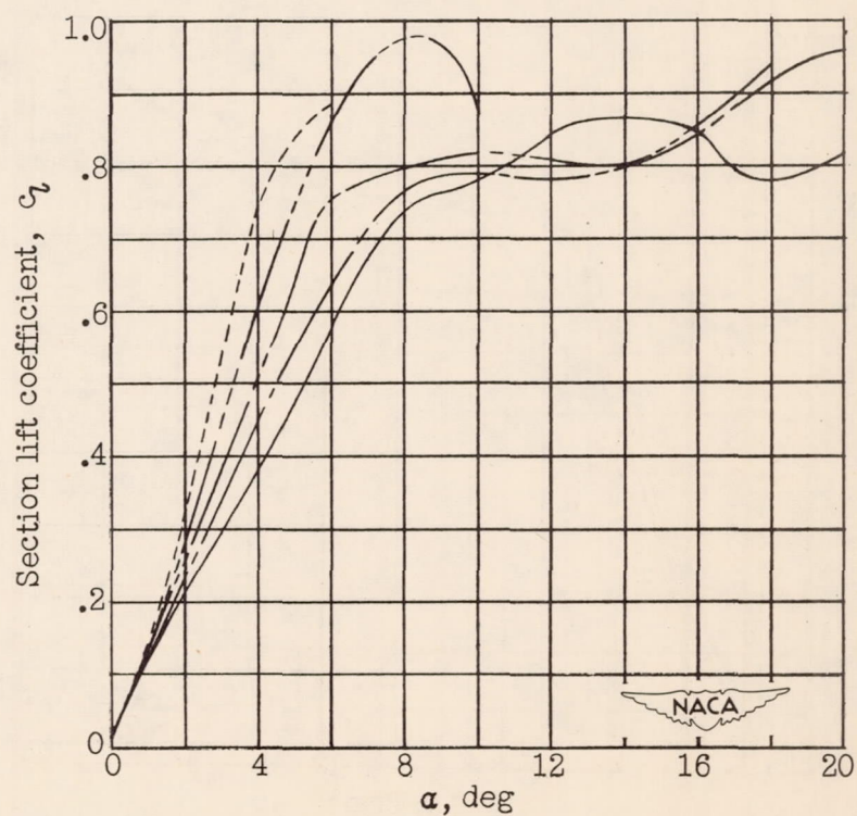
(b) NACA 66-006 airfoil.
