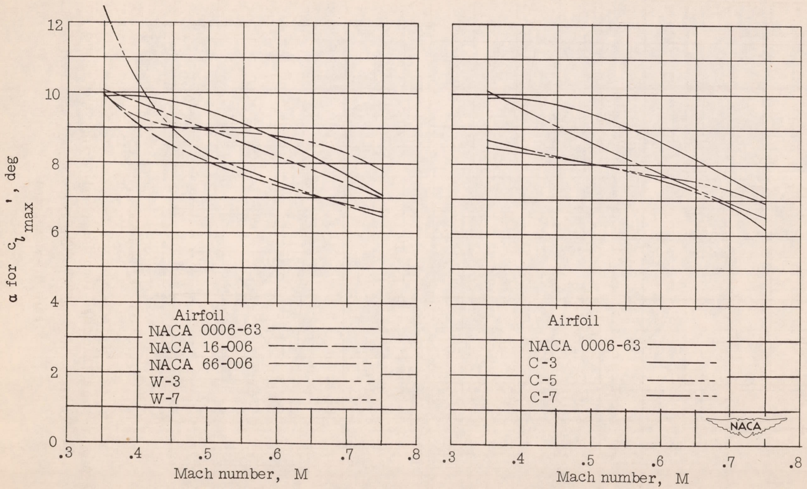
Figure 6.- Variation of angle of attack for effective maximum section lift coefficient with Mach number.
