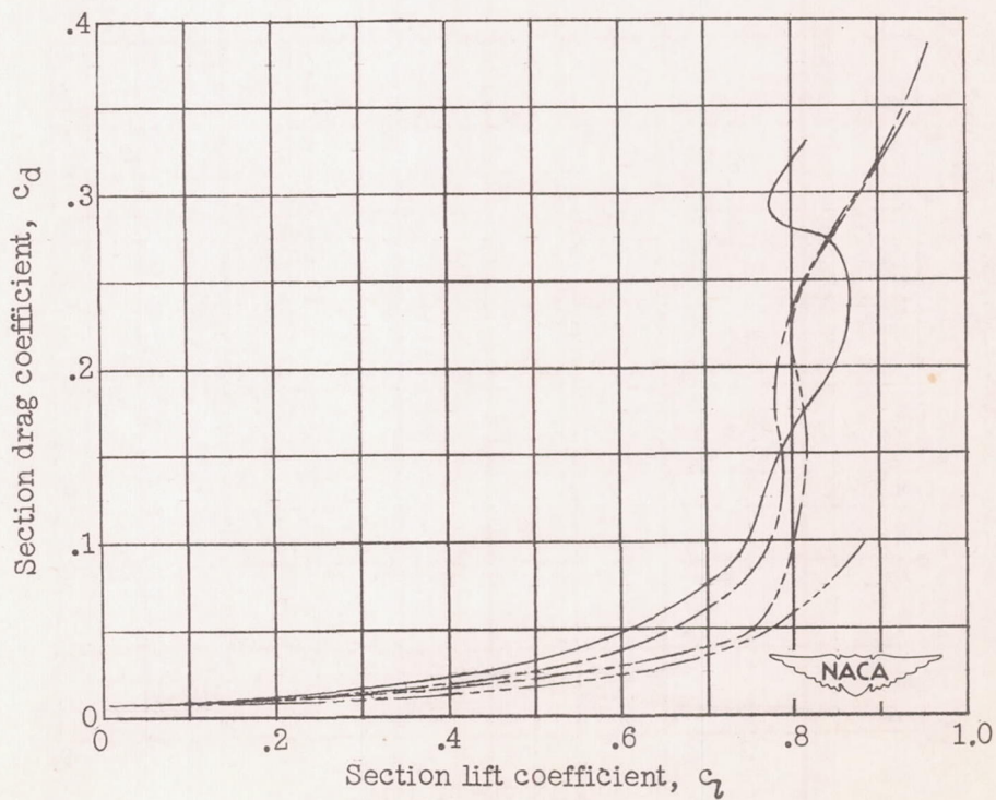
(b) NACA 66-006 airfoil.
