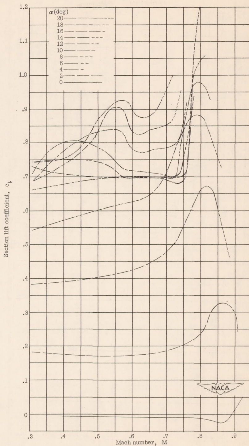
(a) NACA 16-006 airfoil.
