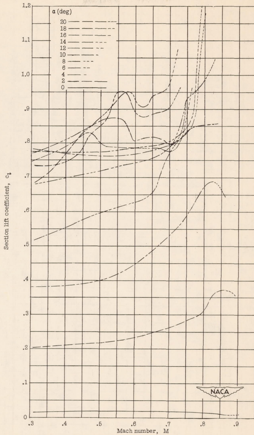
(c) NACA 0006-63 airfoil.
