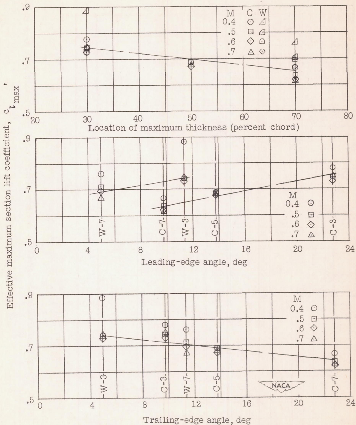
(b) Effect of maximum-thickness location, leading-edge angle, and trailing-edge angle.
