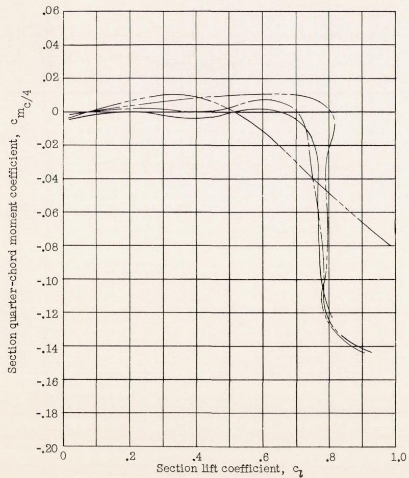
(c) NACA 0006-63 airfoil.
