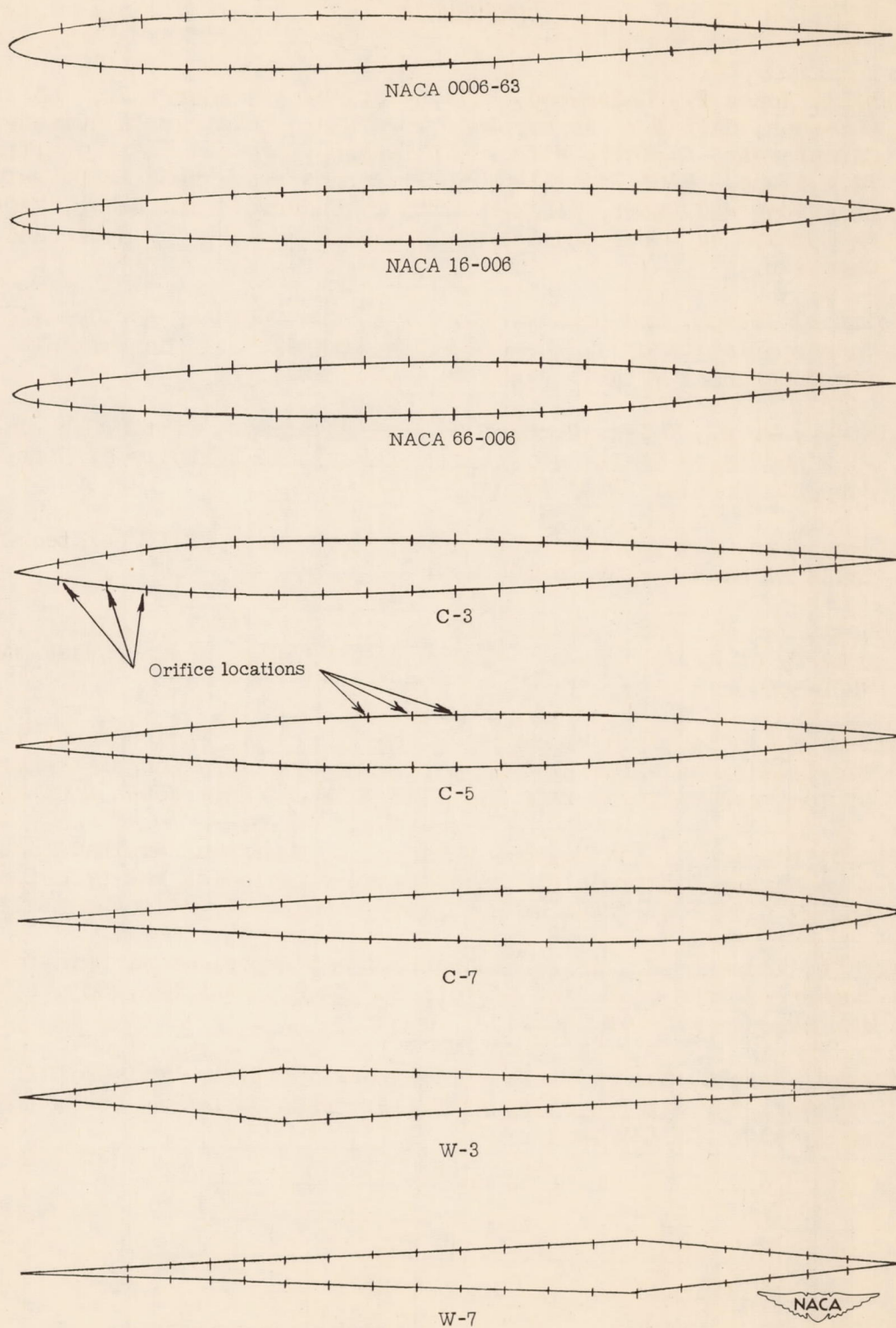
Figure 1.- Airfoil profiles and static-pressure-orifice locations.
