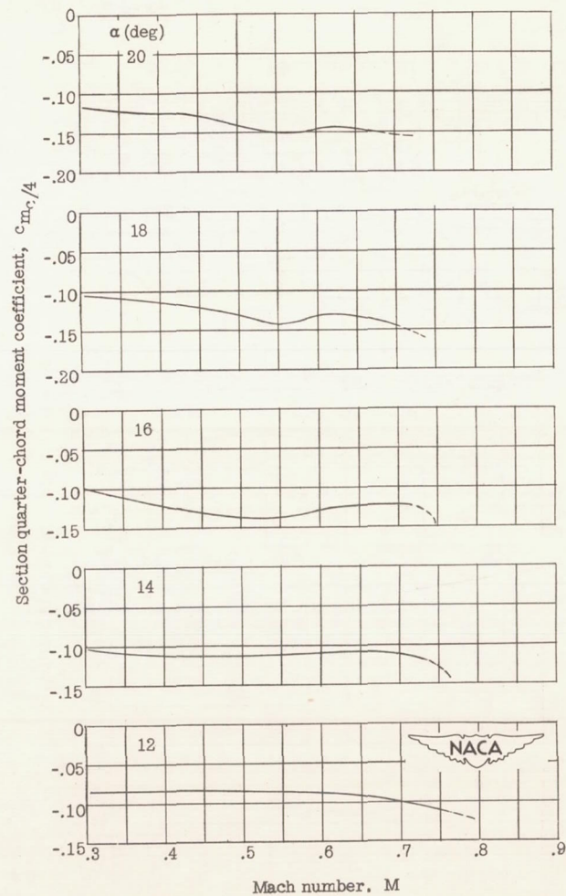
(c) NACA 0006-63 airfoil.
