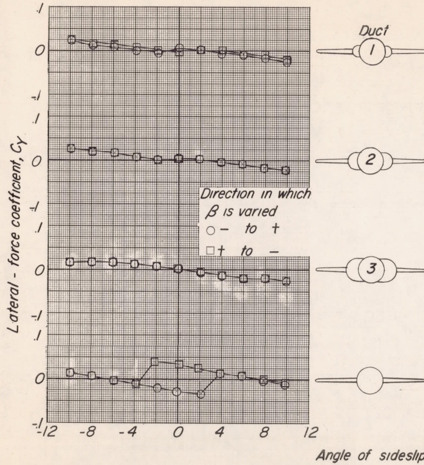
(a) Configuration FW_2 .
