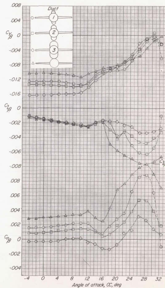
(b) Vertical air ducts.
