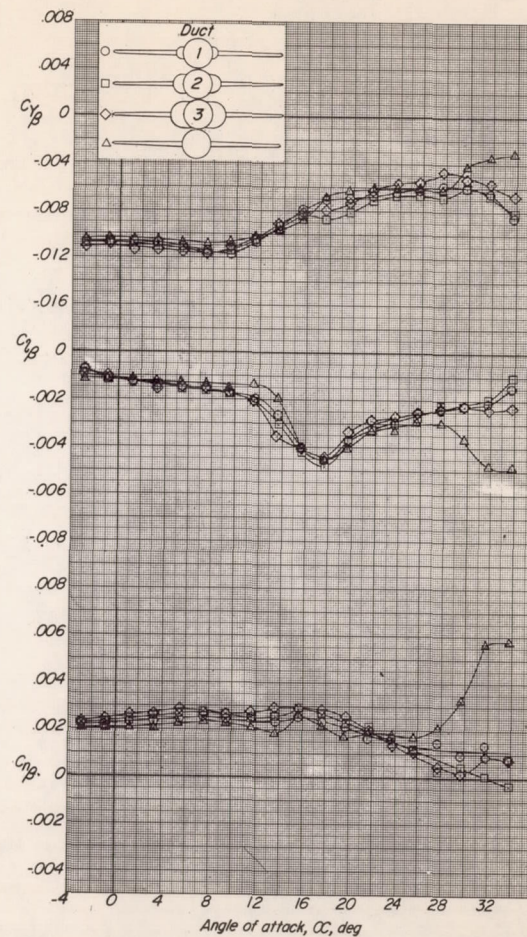
(b) Configuration FW_{4V} .
