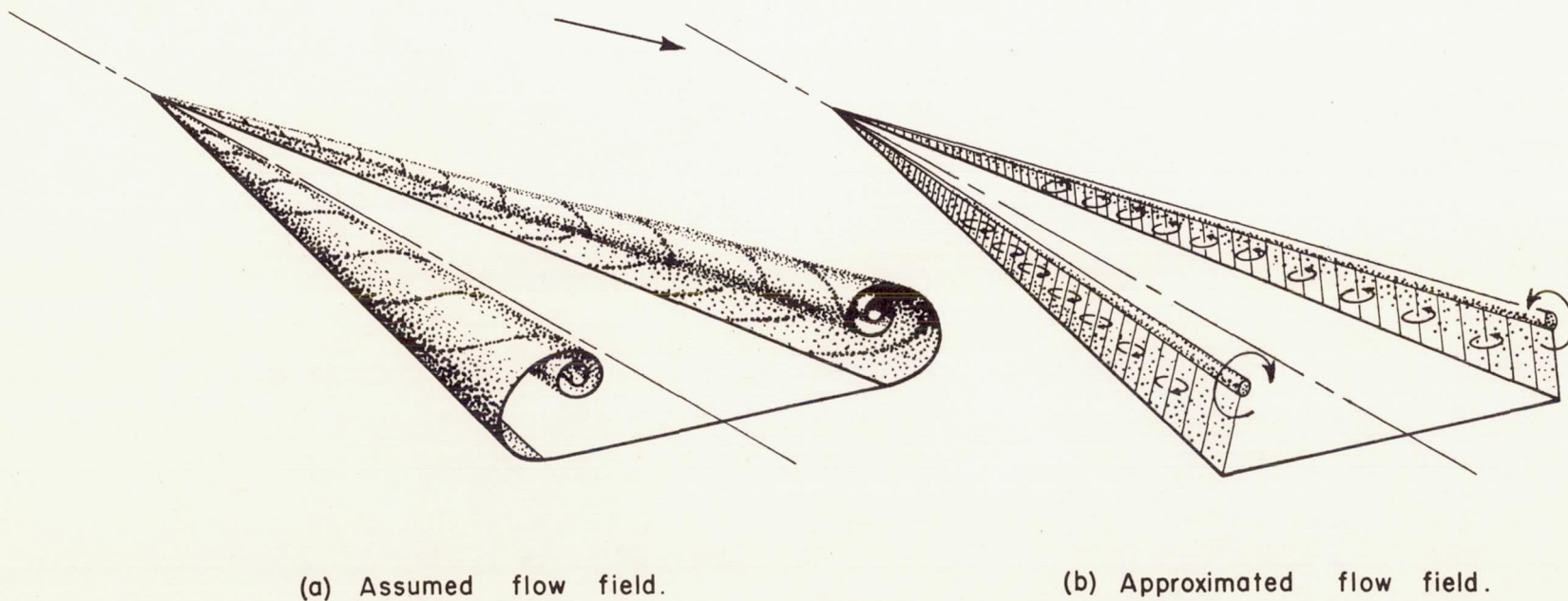
Figure 1.- Schematic drawings of separated flow over slender delta wings.
