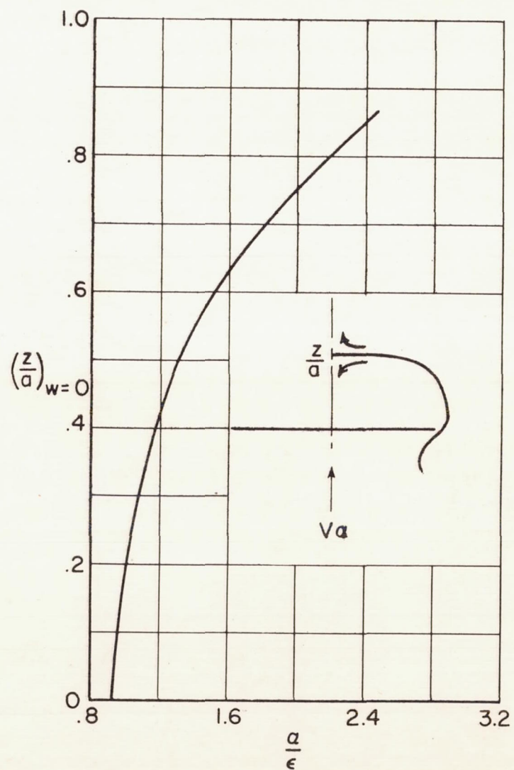
Figure 9.- Stagnation-point locations.
