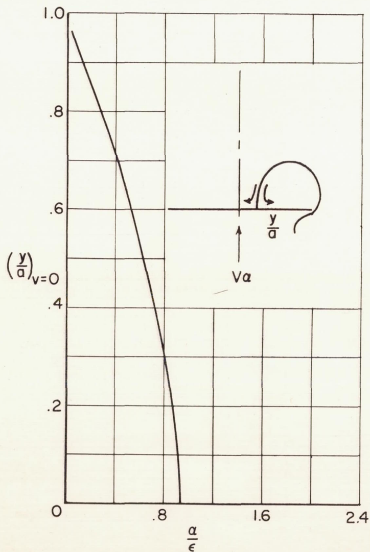
Figure 9.- Stagnation-point locations.
