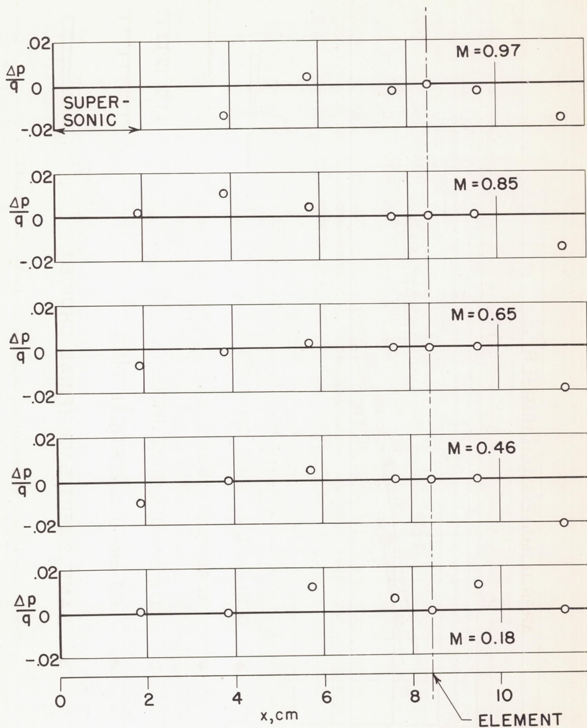
Figure 6.- Pressure distributions at subsonic speeds.
