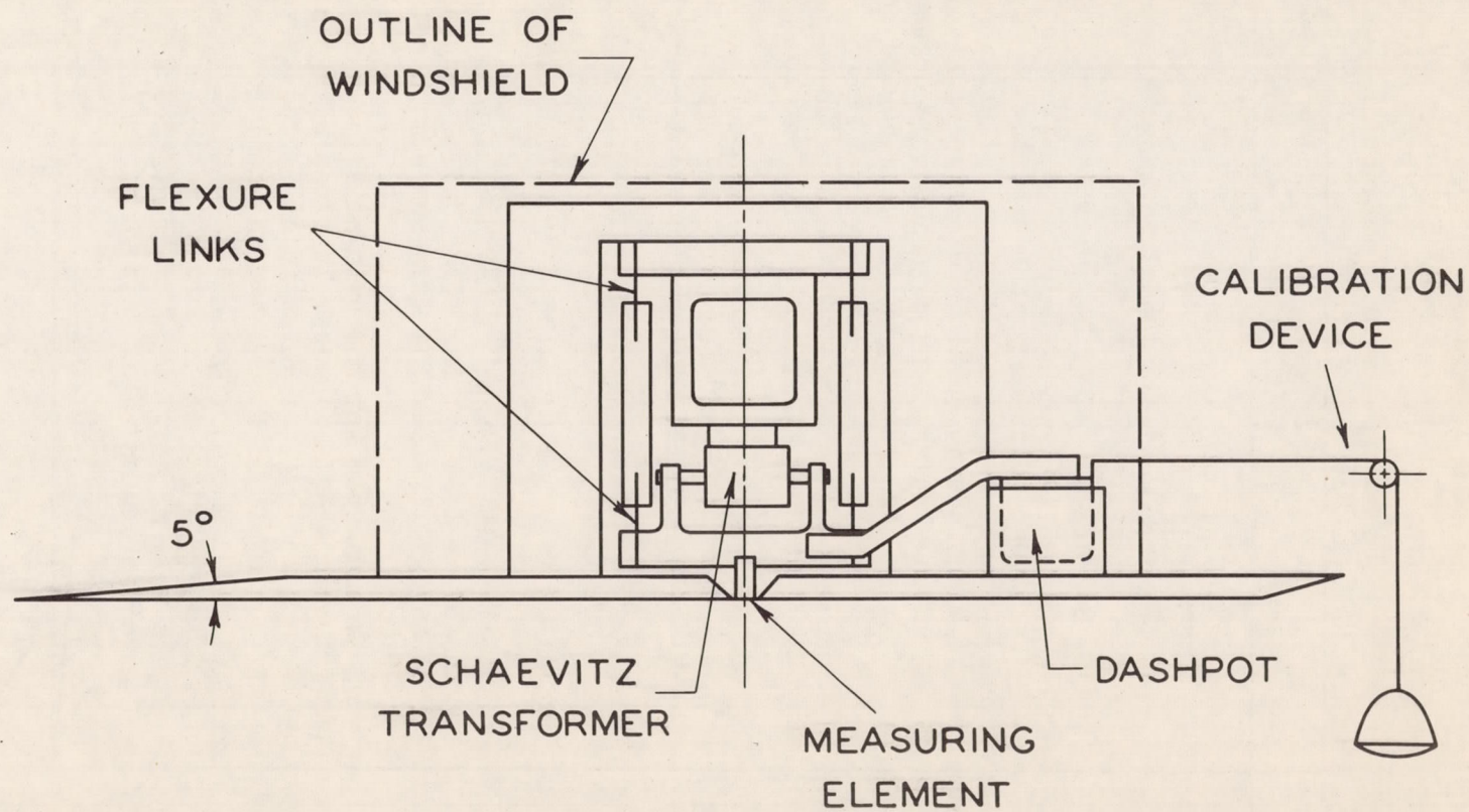
Figure 1.- Skin-friction meter.
