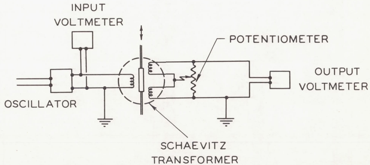
Figure 4.- Electrical circuit.
