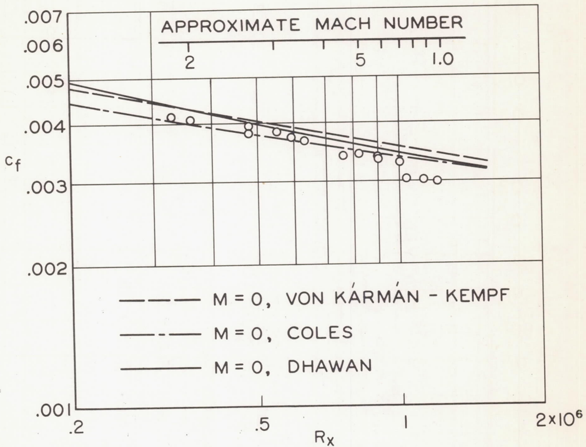
Figure 8.- Subsonic measurements.
