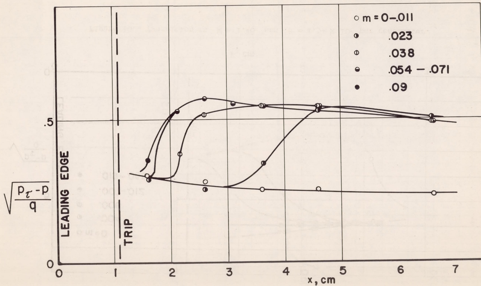
Figure 11.- Transition at M = 1.76 and R = 1.15 \times 10^5 per centimeter.
