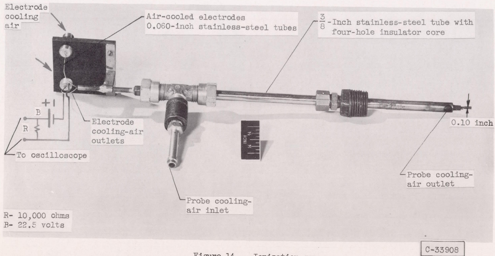
Figure 14. - Ionization gap.
