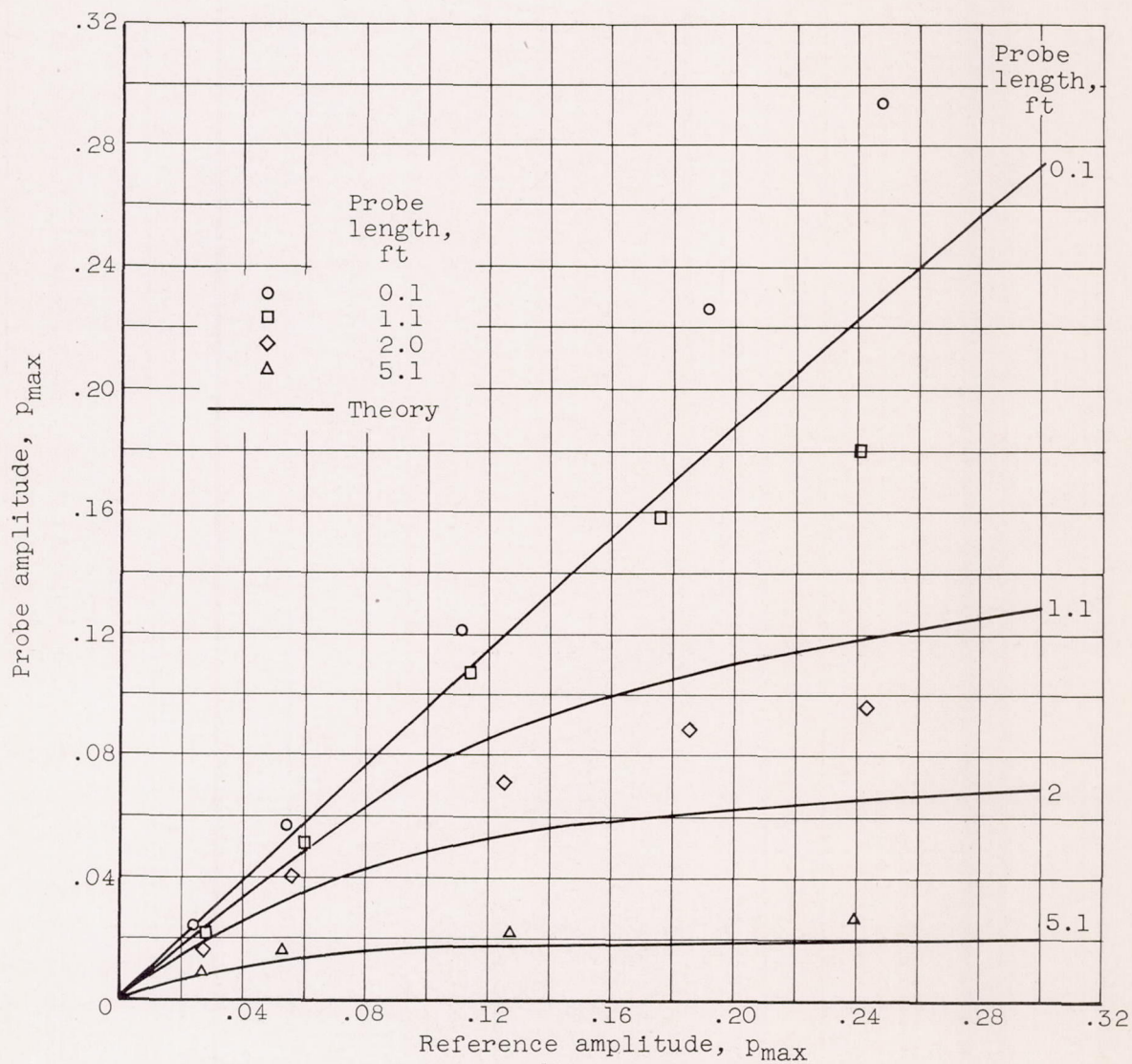
Figure 12. - Concluded. Probe-microphone calibration.
