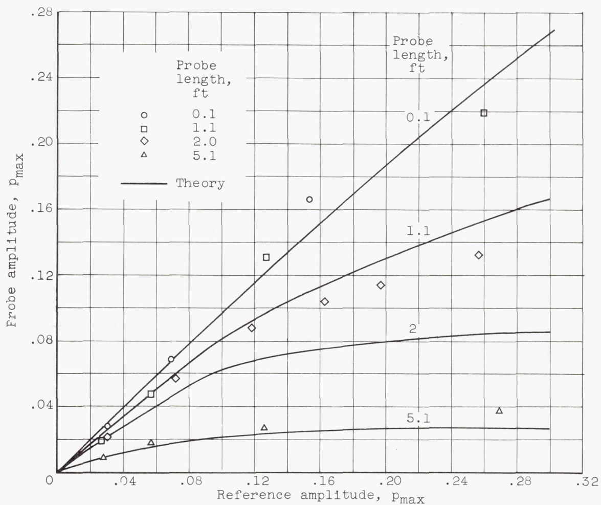
Figure 12. - Continued. Probe-microphone calibration.
