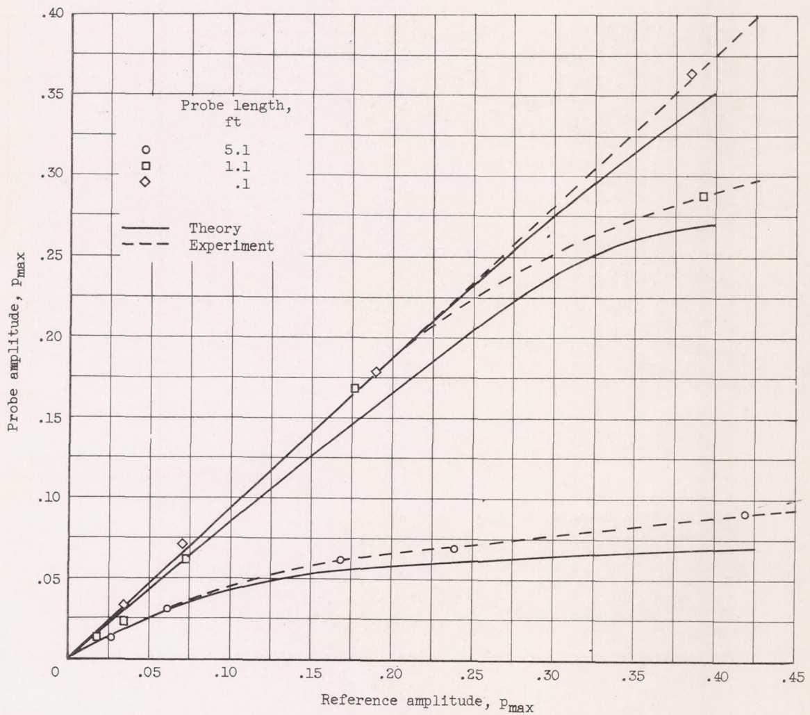
Figure 12. - Probe-microphone calibration.
