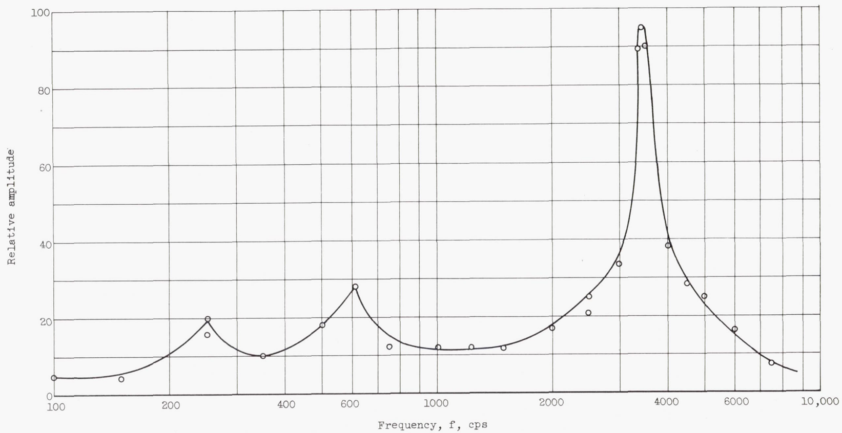
Figure 18. - Concluded. Examples of spectra at wall downstream of flameholders.
