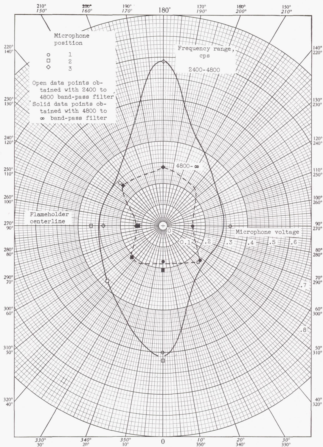
Figure 22. - Microphone voltages about circumference of screeching combustor 1\frac{1}{2} inches downstream of V-gutter.
