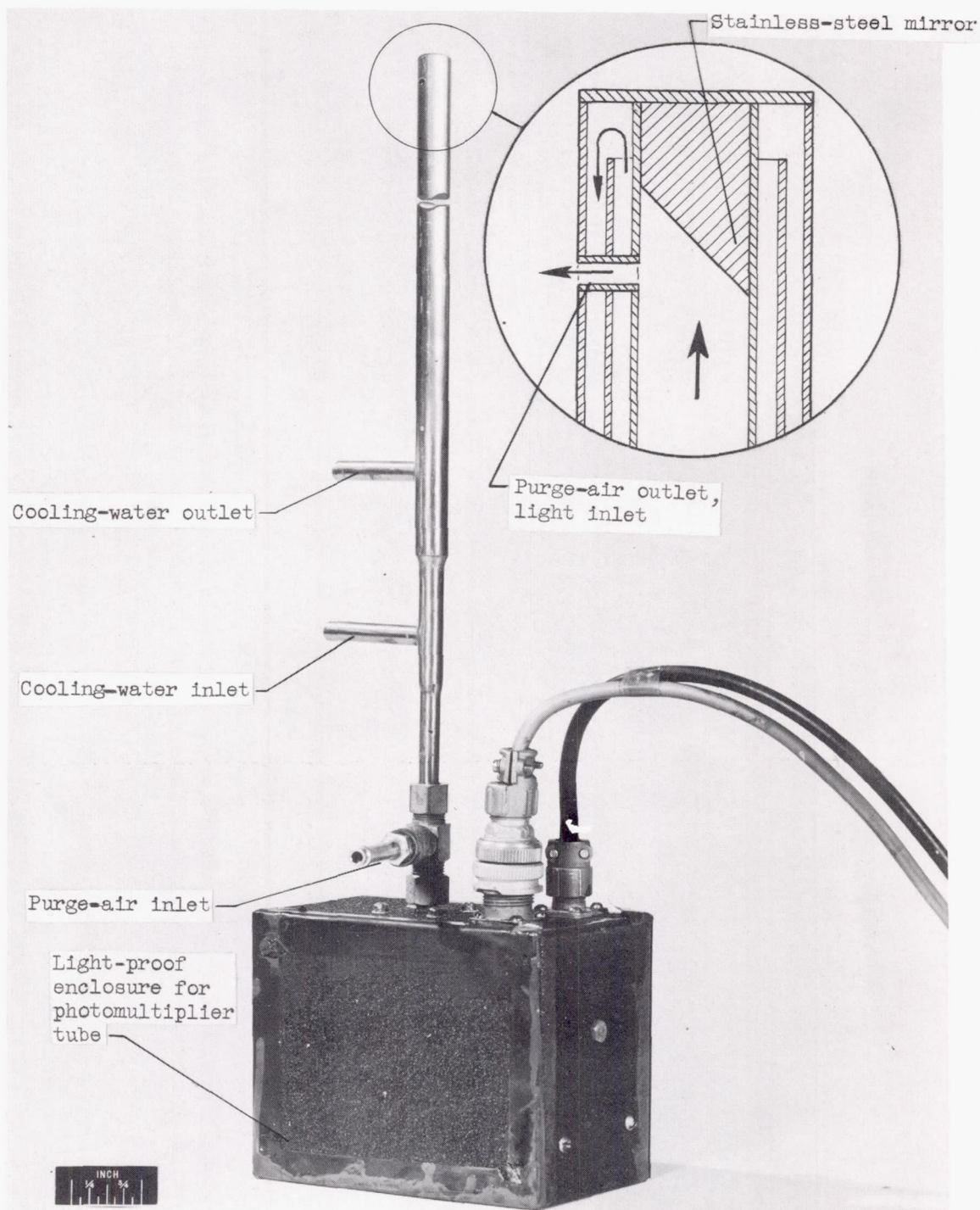
Figure 15. - Photocell probe.
