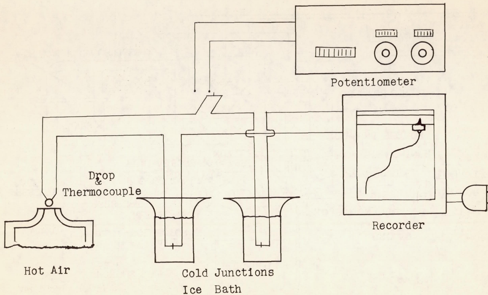
Figure 2.- Schematic diagram of temperature-recording system.
