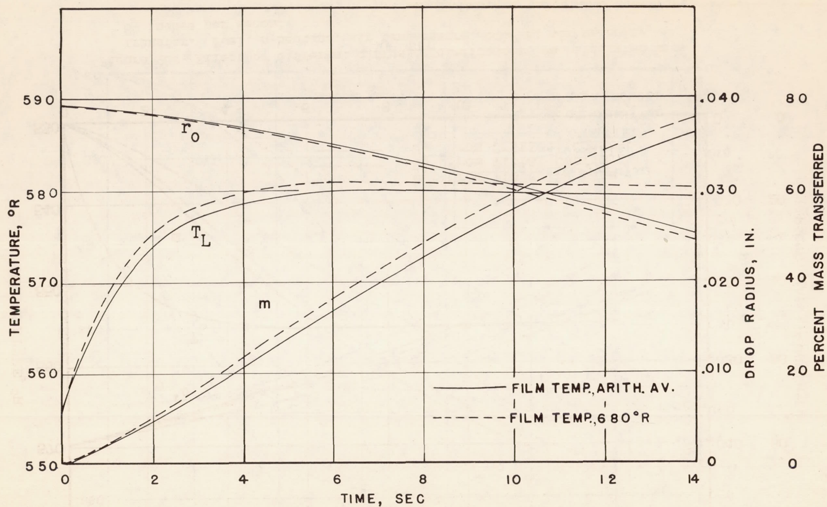
Figure 25.- Effect of film temperature averaging on physical properties. Fuel, n-octane; air temperature, 680° R.
