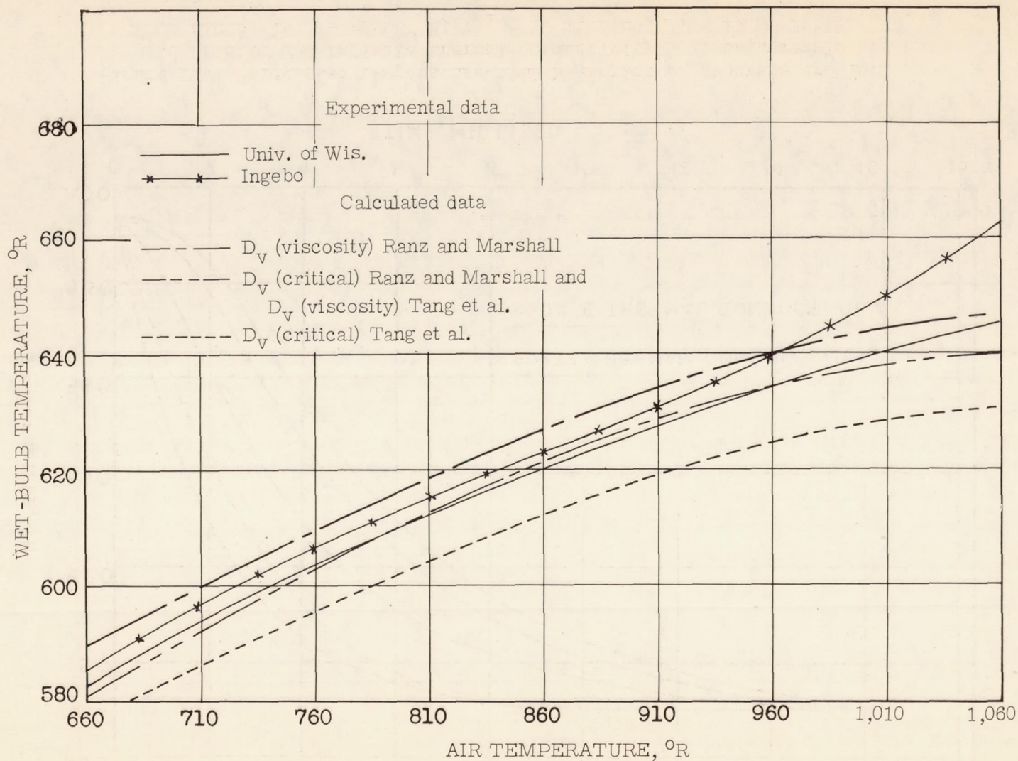
Figure 21.- Experimental and calculated wet-bulb temperatures of n-octane for different air temperatures.
