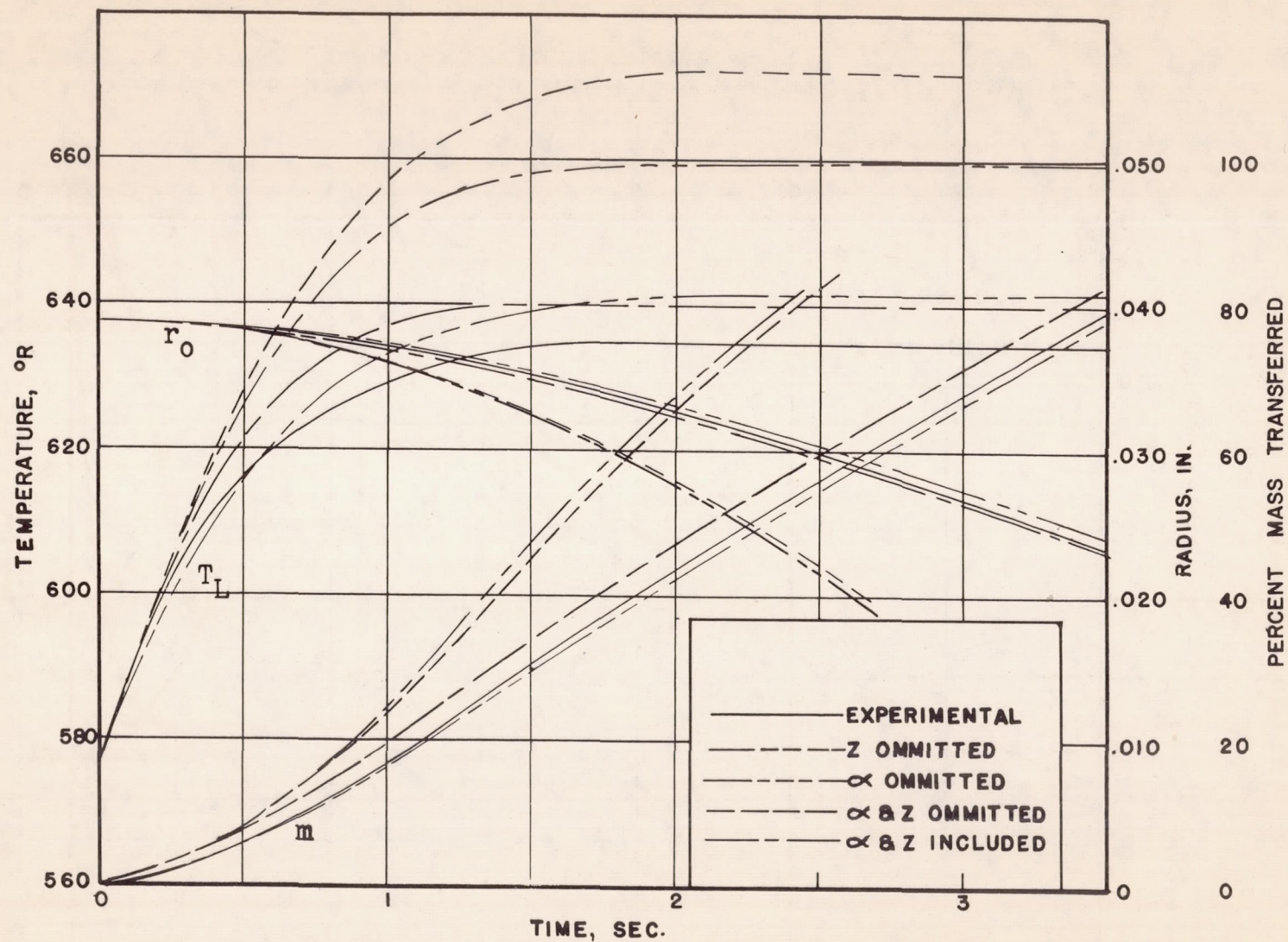
Figure 24.- Effect of \alpha and Z factors on calculated histories.
