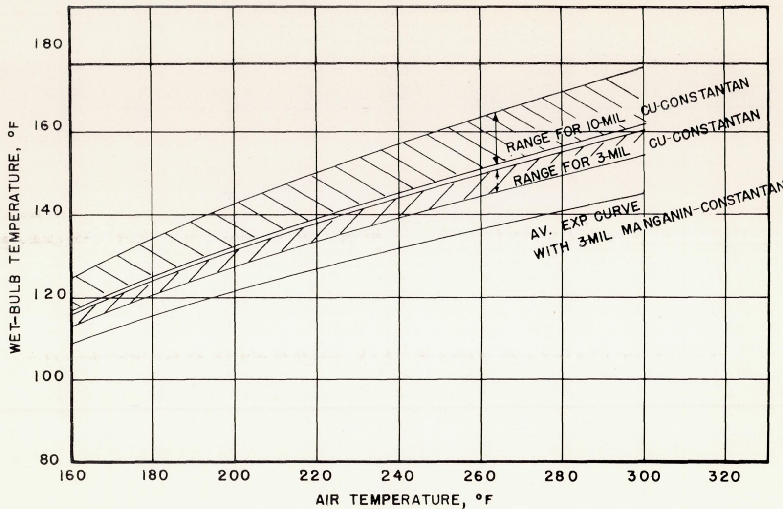
Figure 10.- Experimental wet-bulb temperatures for n-octane using different thermocouples and air temperatures.
