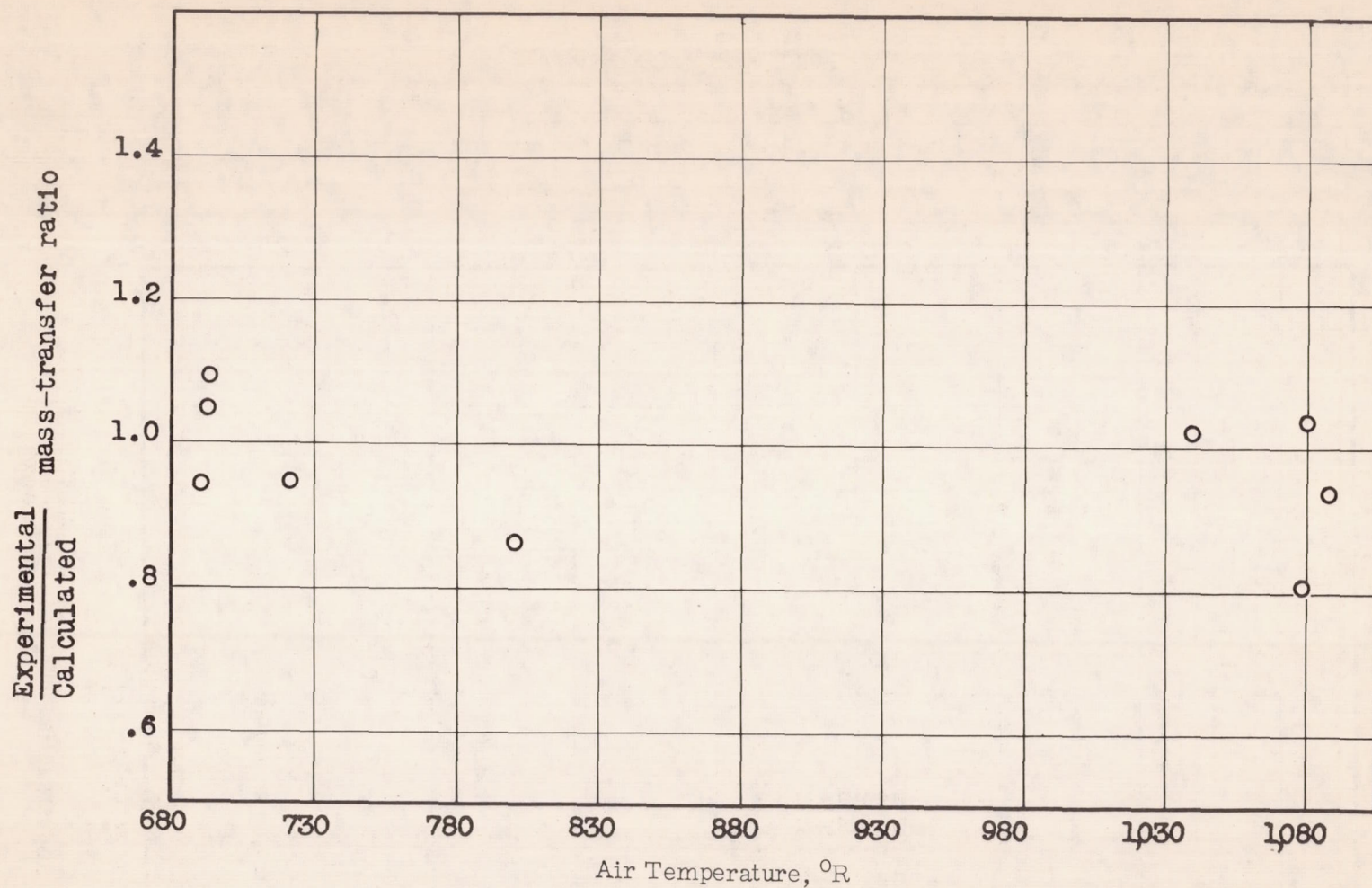
(a) Mass transfer during steady-state portion of temperature history.
