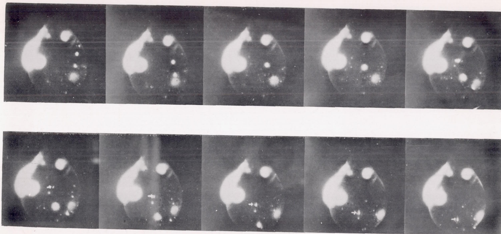
Figure 7.- High-speed photographs of internal circulation in drops. L-89339 Cetane drop in 6-foot-per-second upward air stream; frames 0.005 second apart.
