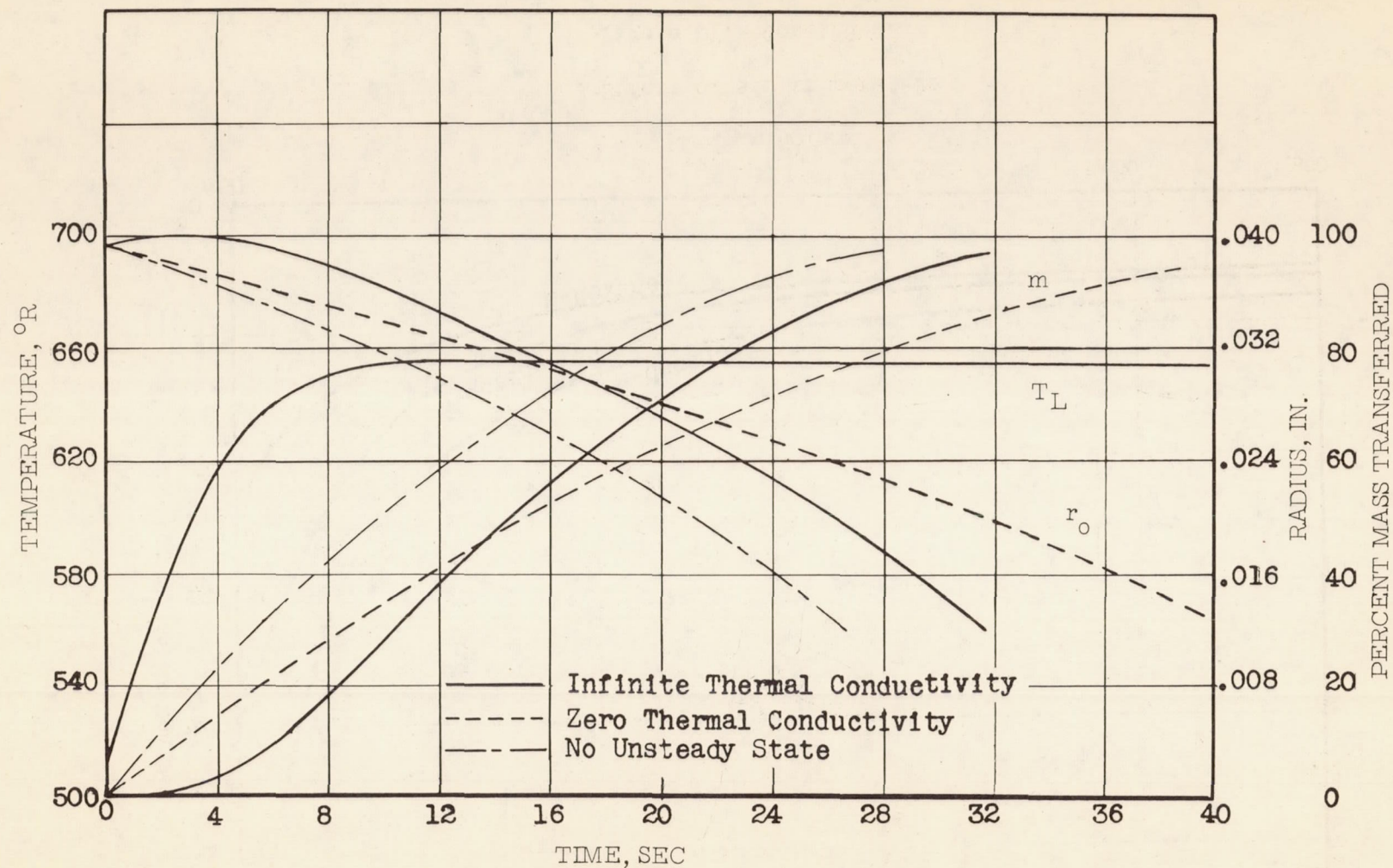
Figure 28.- Results of different calculation techniques. Fuel, n-octane; air temperature, 1,000° R; air velocity, 90 inches per second.
