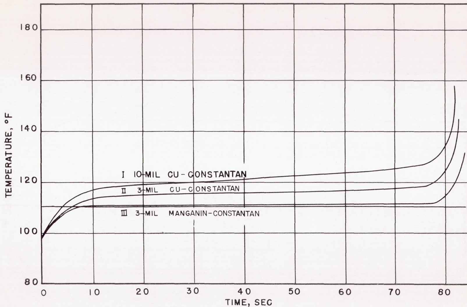
Figure 9.- Experimental time-temperature curves using water on different thermocouples in 300° F air blast.
