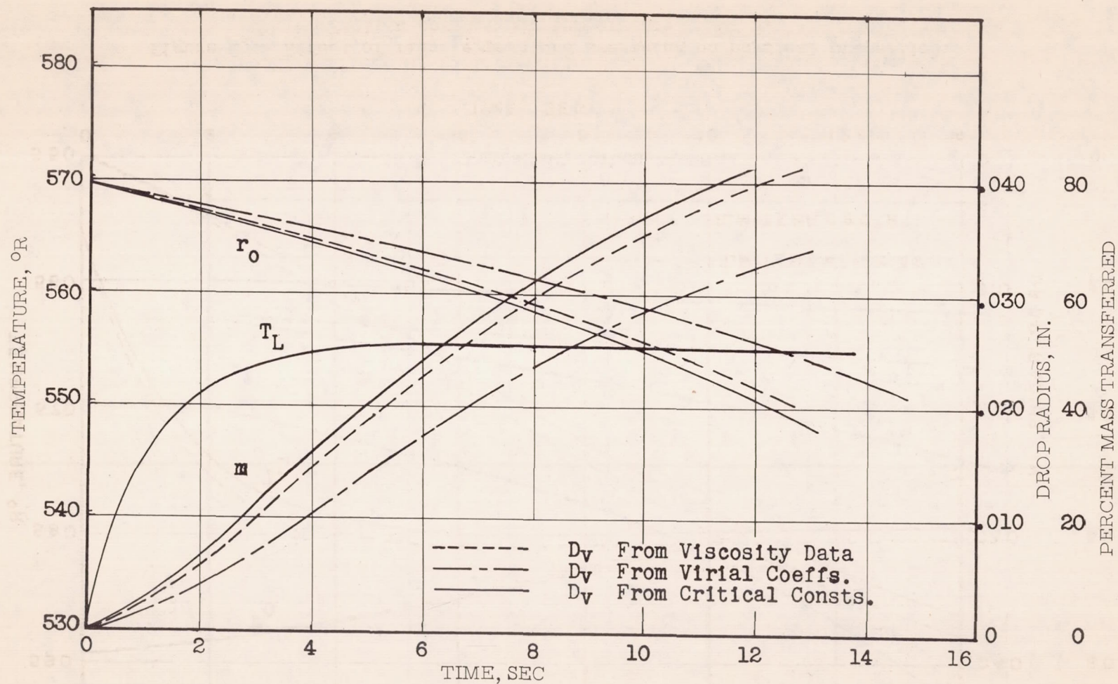
Figure 26.- Effect of different diffusion coefficients on calculated mass transfer. Fuel, n-heptane; air temperature, 676° R; air velocity, 84 inches per second.
