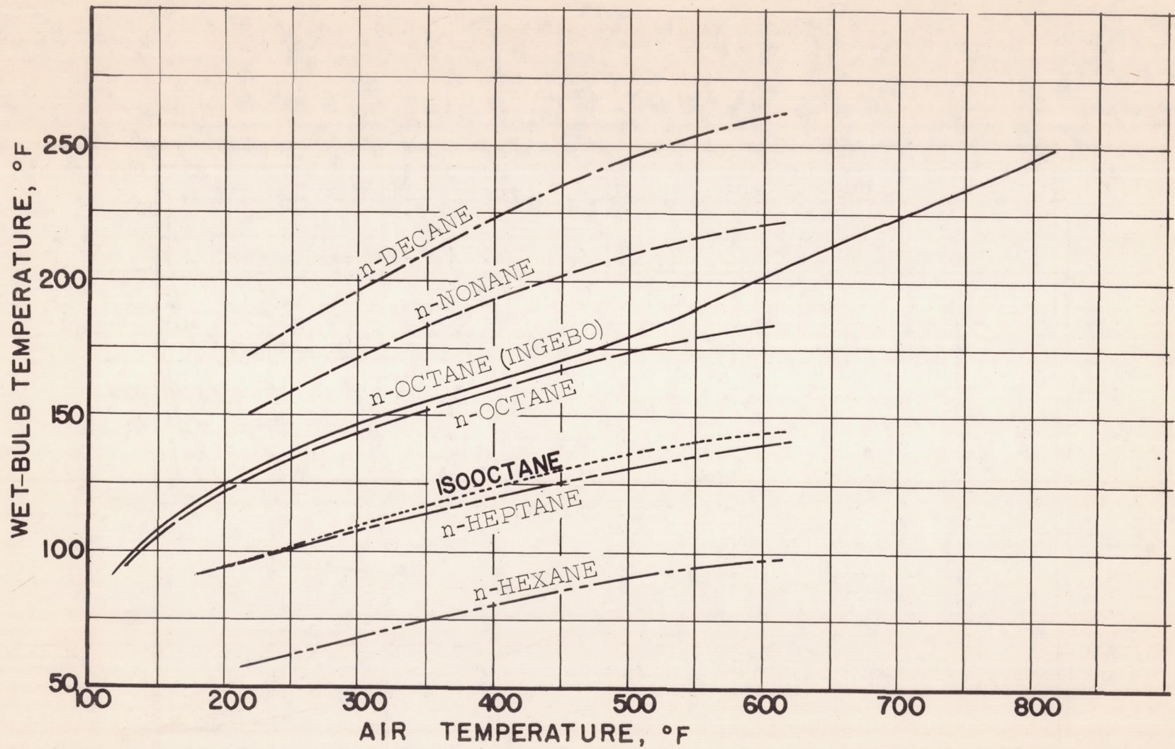
Figure 13.- Wet-bulb temperatures for given fuels.
