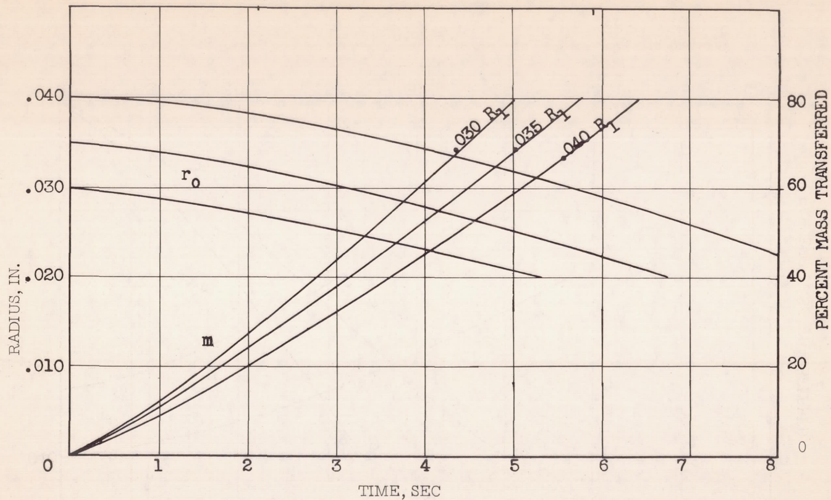
Figure 16.- Experimental droplet histories with different initial radii. Air temperature, 680^{\circ} R; air velocity, 90 inches per second.
