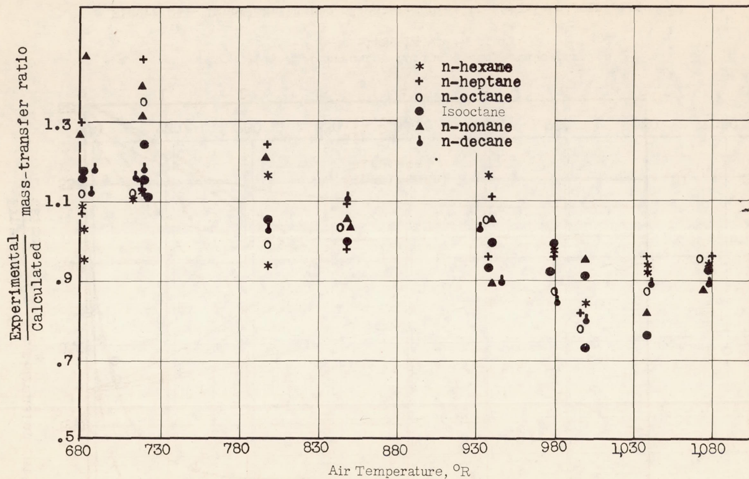
(b) Mass transfer calculated from experimental temperature histories for heating-up period.
