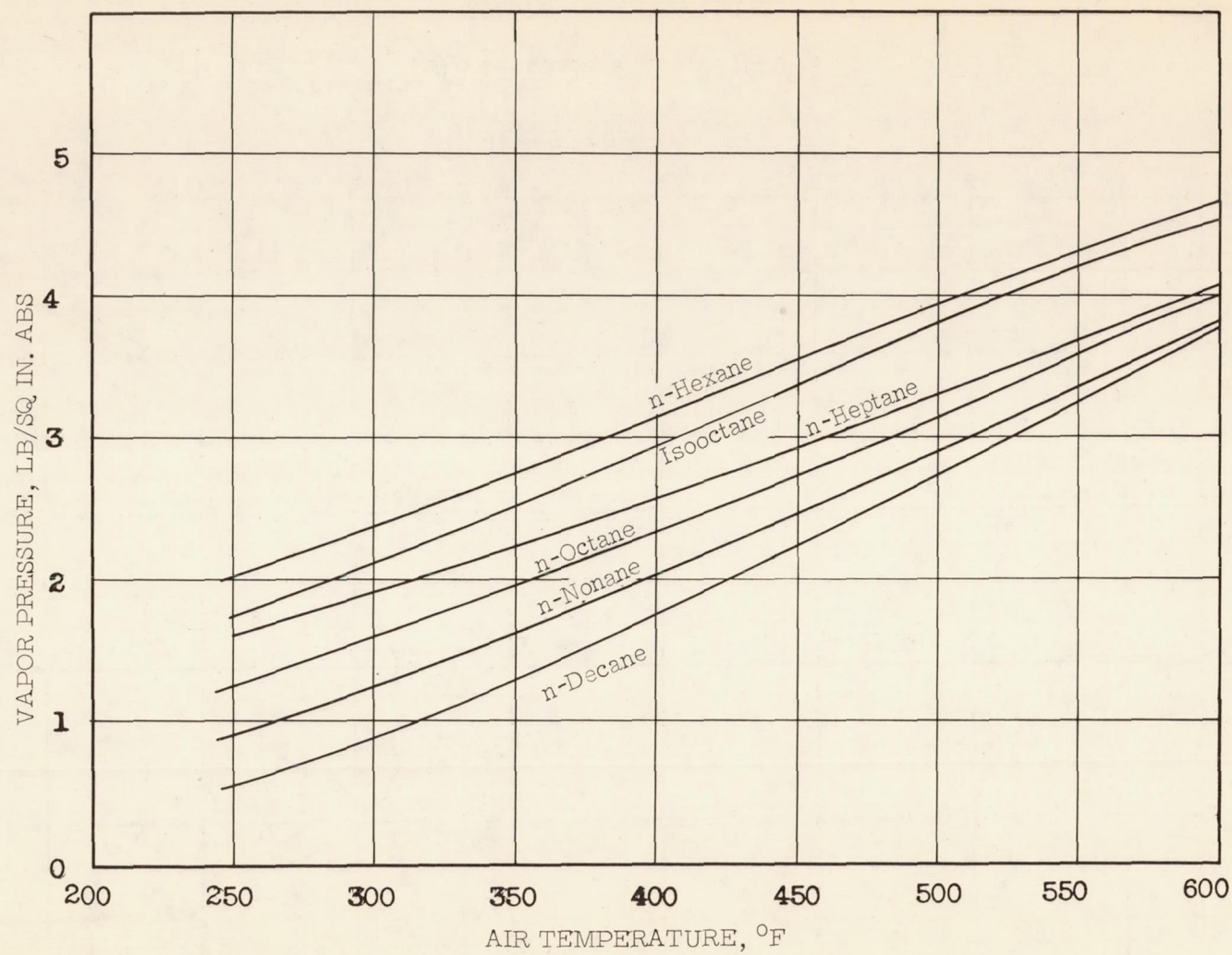
Figure 15.- Vapor pressure at wet-bulb temperature against air temperature.
