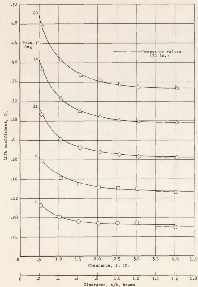
(a) Mean wetted length l_m = 2 inches ( l_m/b = 0.8 ).
