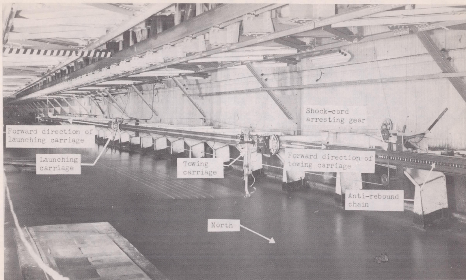
Figure 13.- General view of Langley tank no. 2 monorail.
