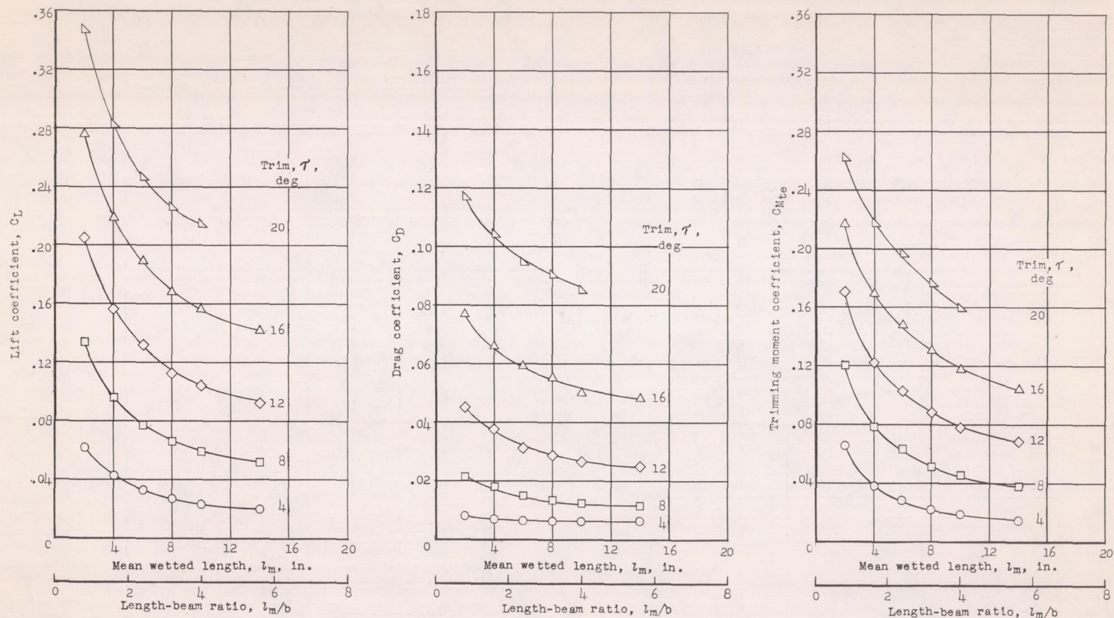
Figure 5.- Lift, drag, and trimming-moment coefficients for deep water (72 inches).
