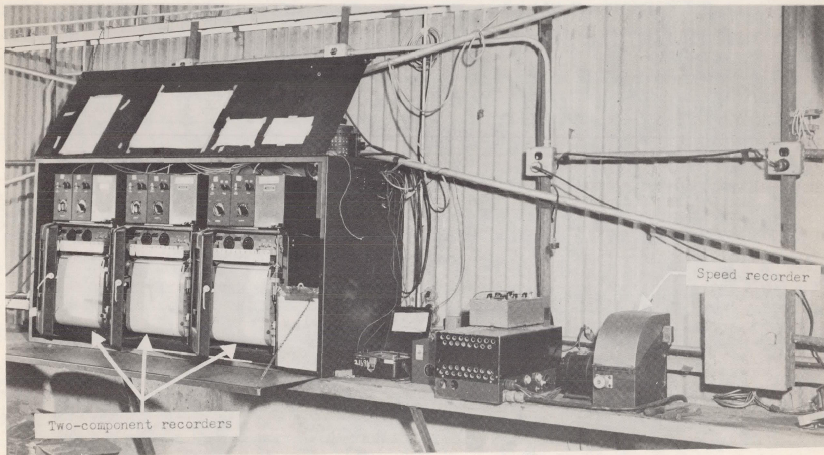
Figure 16. Photograph of recording instruments. L-76498.1
