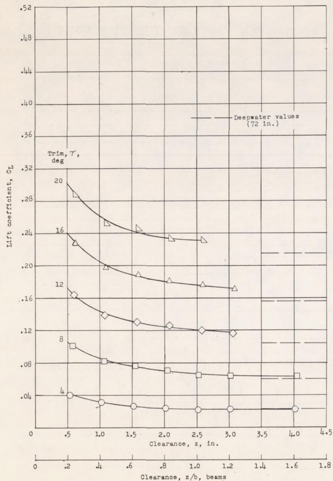
(e) Mean wetted length l_m = 10 inches ( l_m/b = 4.0 ).
