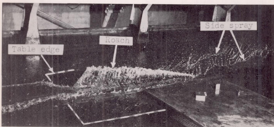
(c) Shallow-water roach further developed.
