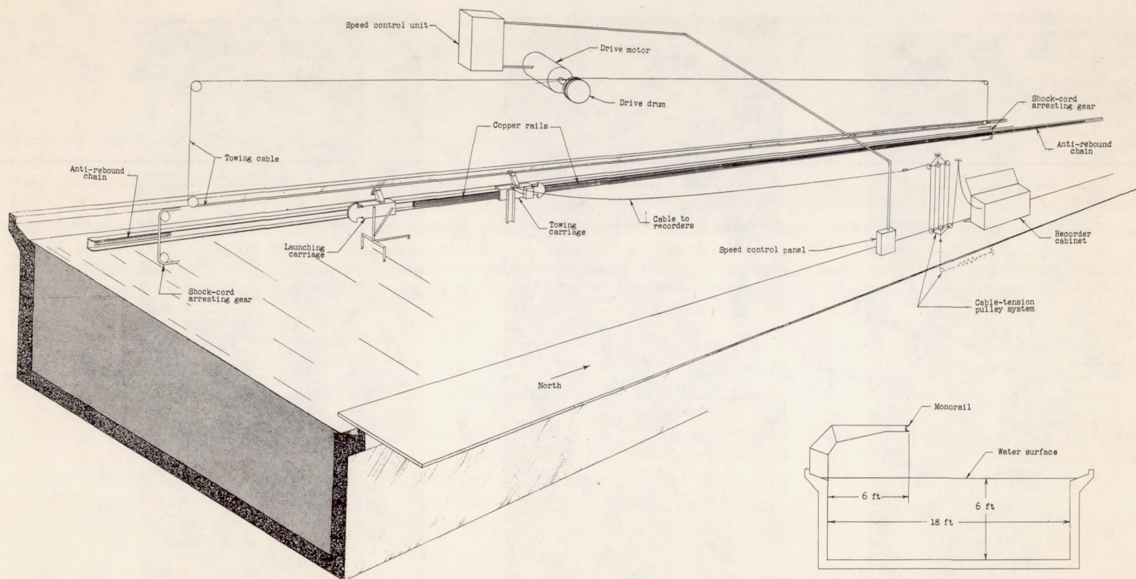
Figure 12.- Schematic sketch of monorail system.
