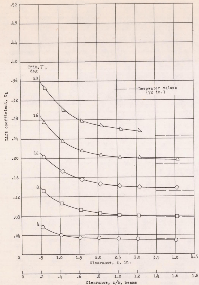
(c) Mean wetted length l_m = 6 inches ( l_m/b = 2.4 ).
