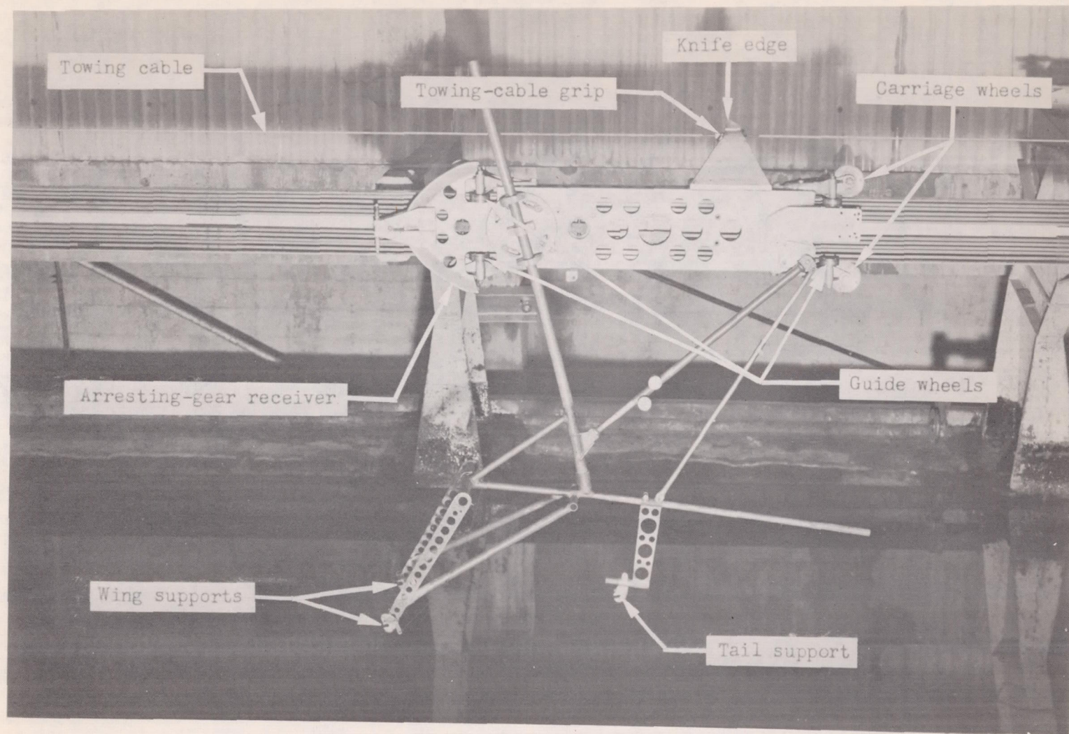
Figure 15.- Photograph of launching carriage. L-89558.1
