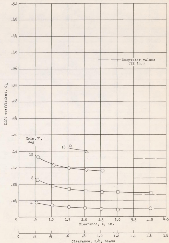
(f) Mean wetted length l_m = 14 inches ( l_m/b = 5.6 ).
