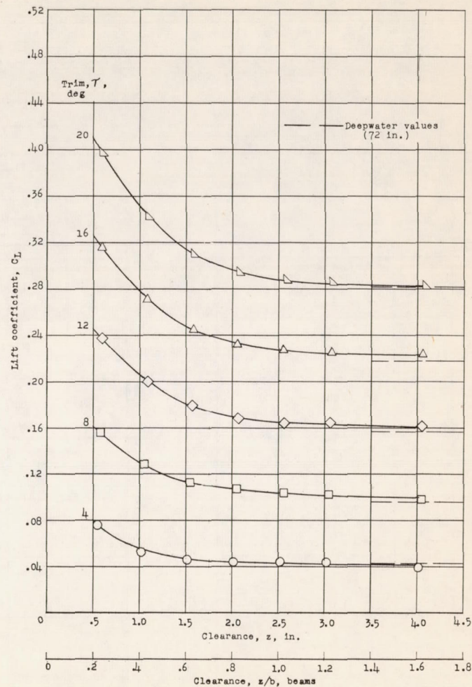
(b) Mean wetted length l_m = 4 inches ( l_m/b = 1.6 ).
