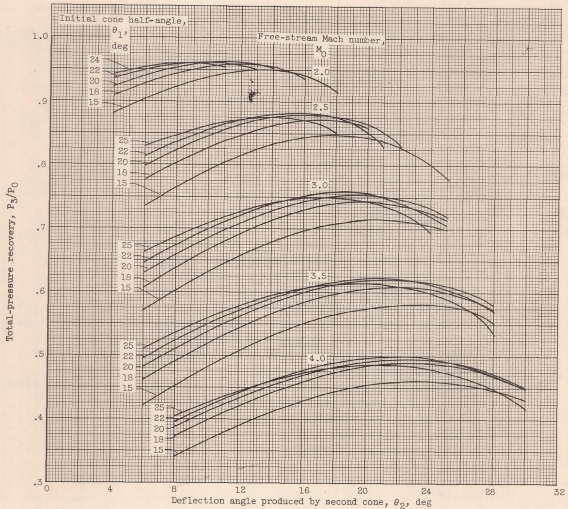
(a) Double-cone inlets; no internal contraction.
