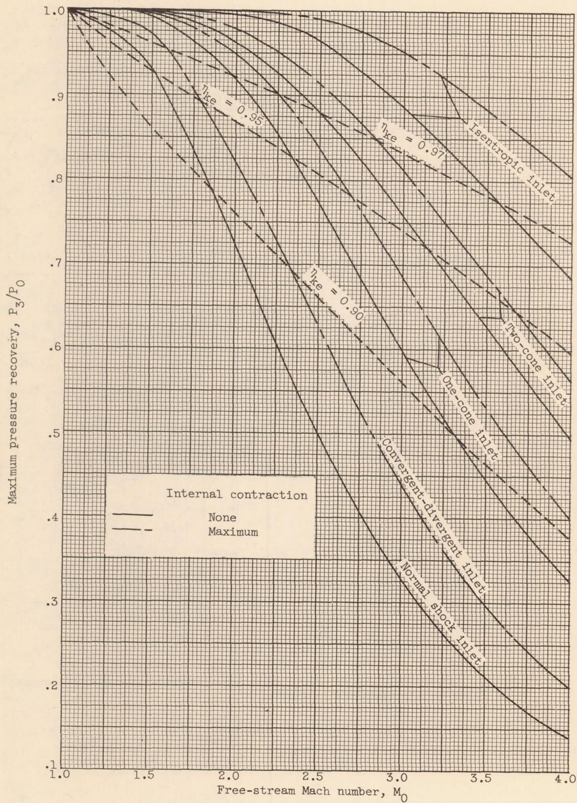
Figure 8. - Theoretical performance comparison of several types of supersonic inlets.
