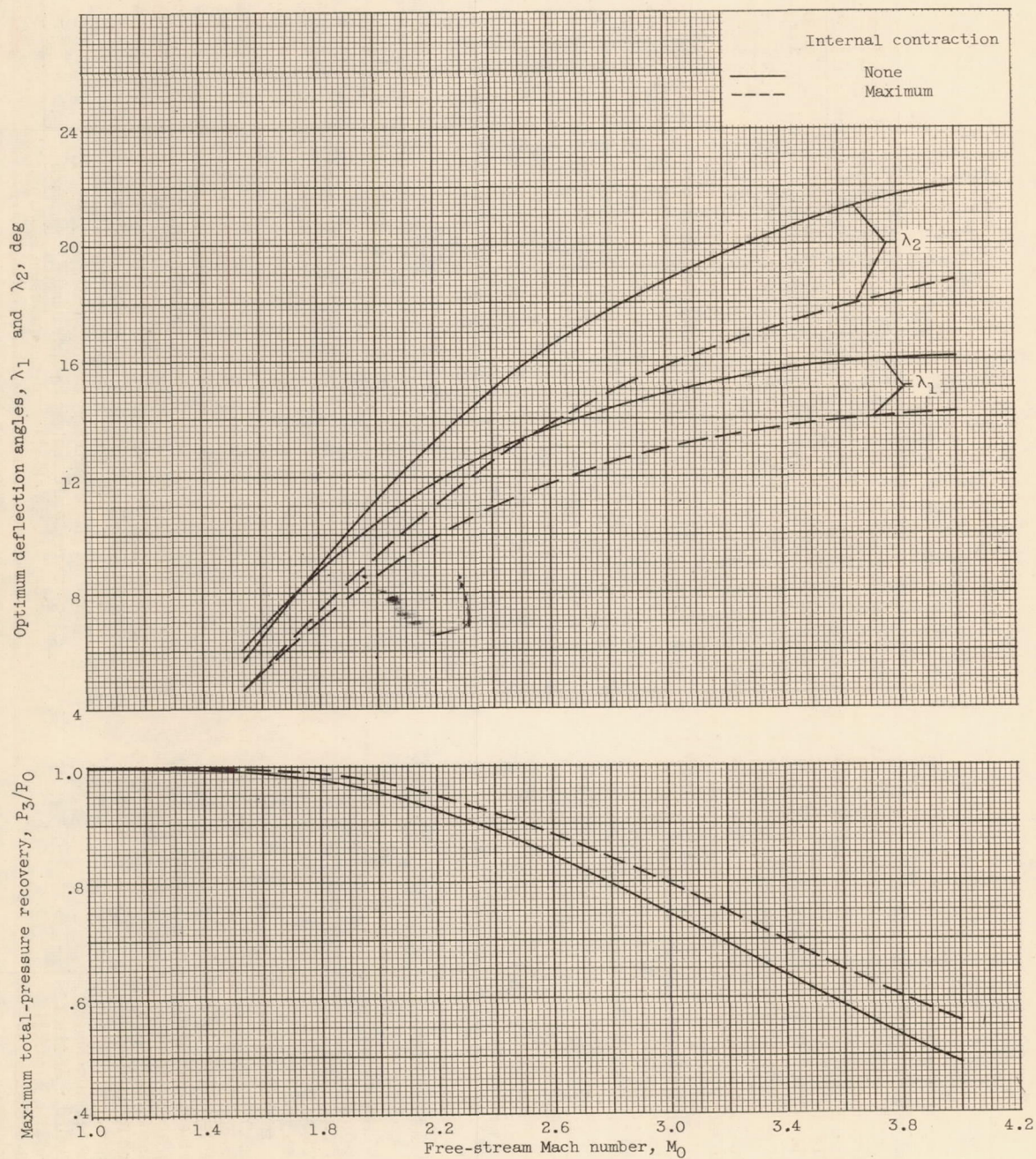
Figure 11. - Concluded. Optimum performance and angle combinations for double-oblique-shock supersonic inlets.
