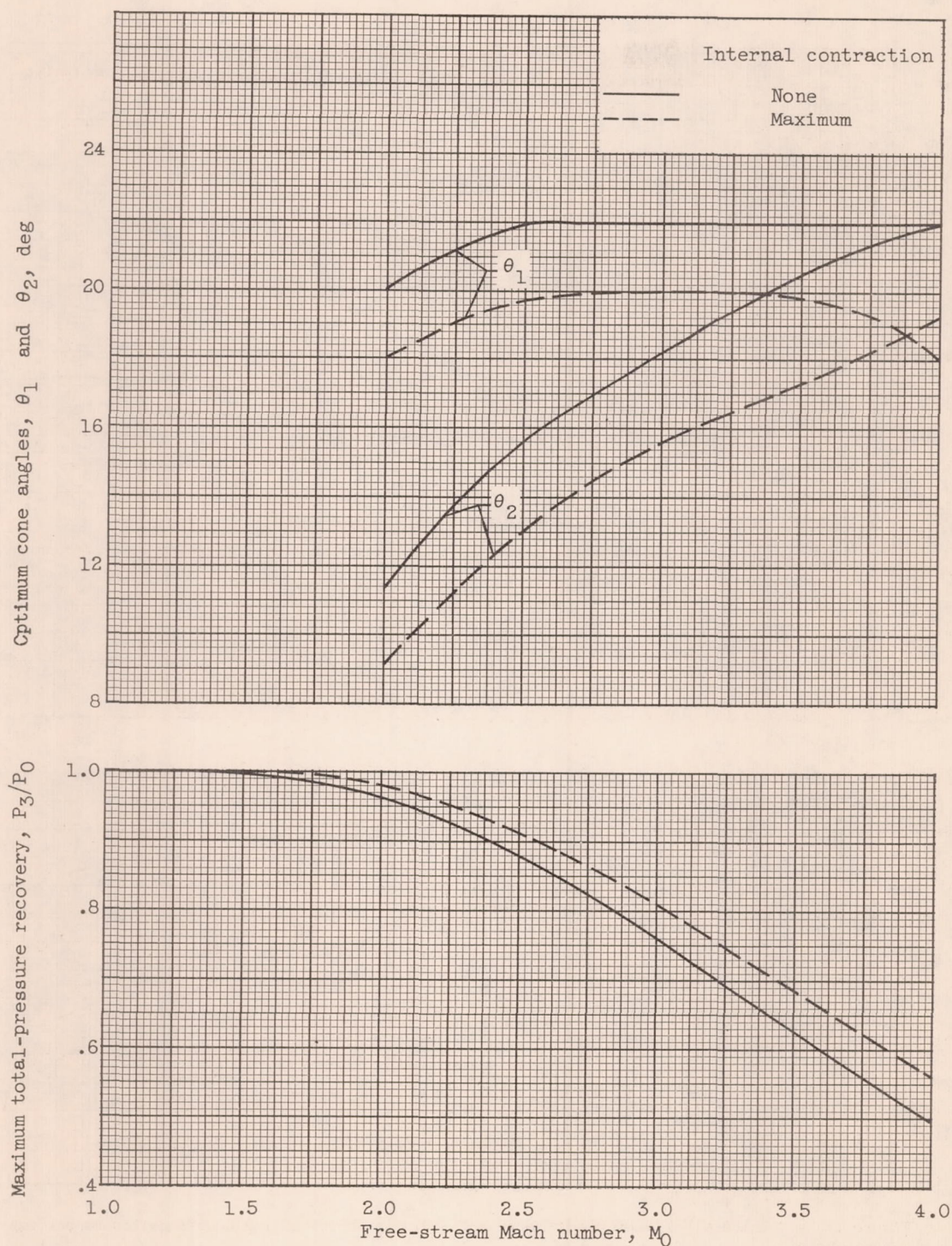
(a) Double-cone inlets.
