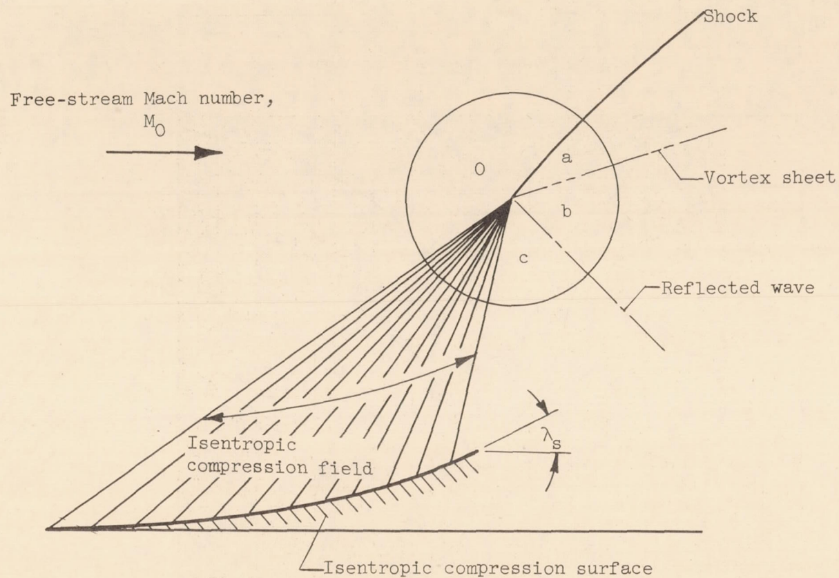
Figure 4. - Schematic representation of branch-shock structure to be analyzed for maximum isentropic flow turning.
