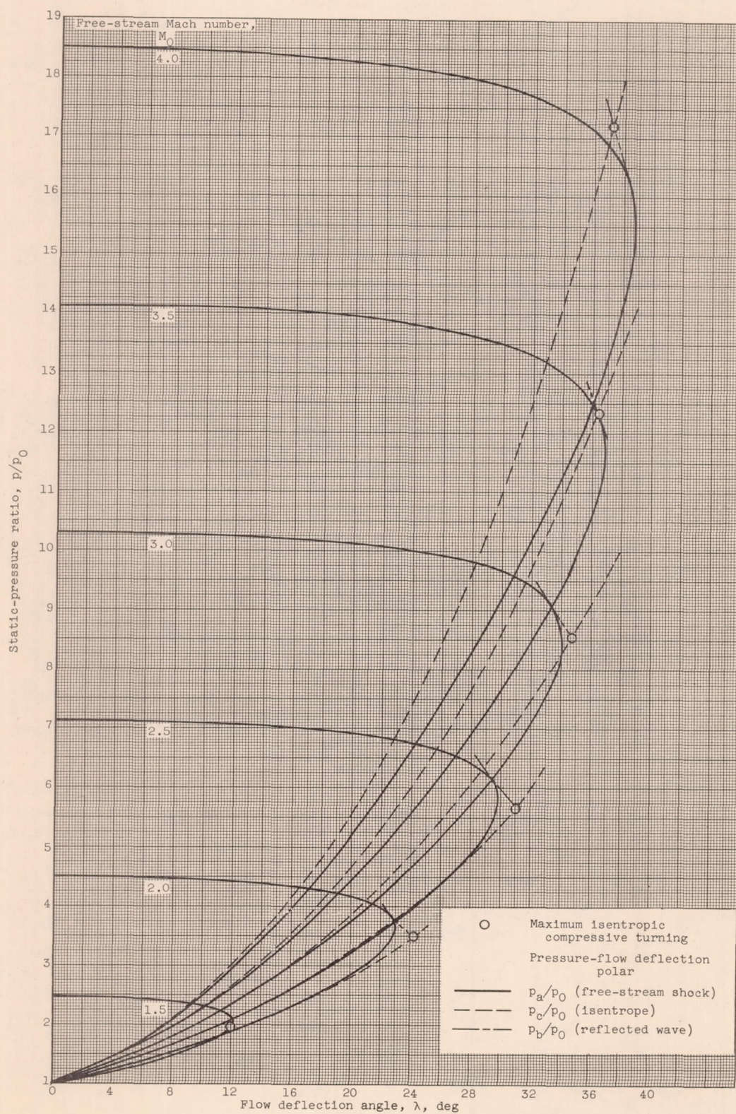
Figure 5. - Theoretical pressure-deflection polars.
