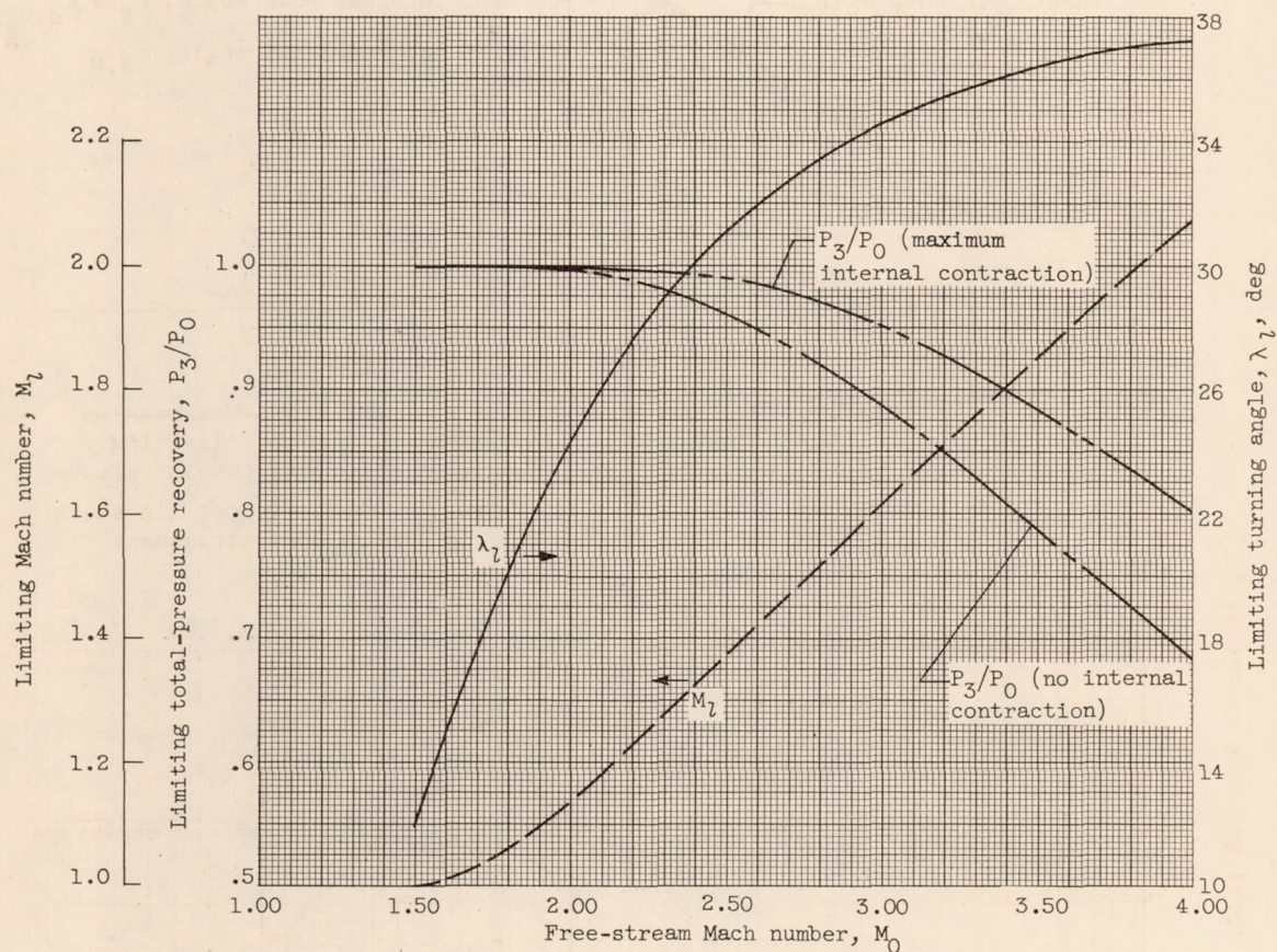
Figure 6. - Summary of aerodynamic parameters corresponding to compression limit based on shock-structure requirements.
