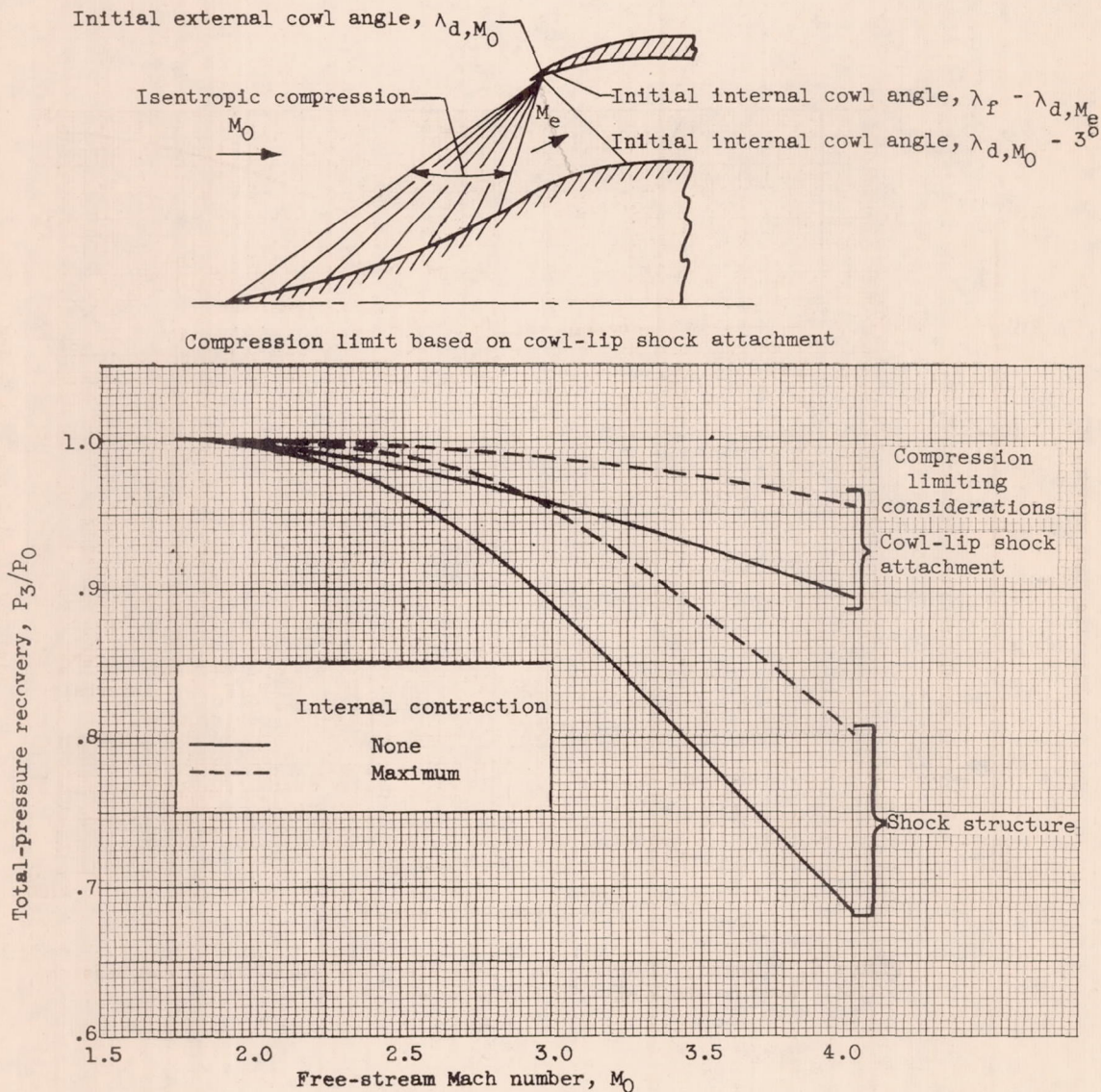
Figure 7. - Comparison of compression limits based on cowl-lip shock attachment and shock-structure considerations.
