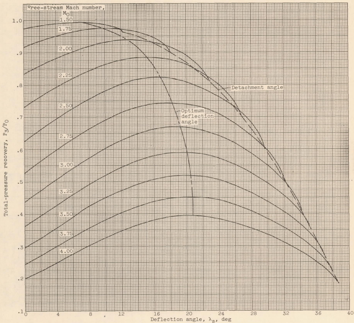
Figure 9. - Concluded. Theoretical performance of single-cone and single-wedge inlets.
