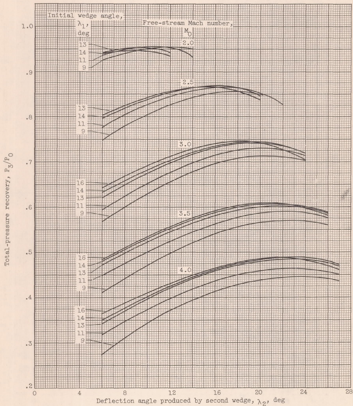
Figure 10. - Continued. Theoretical performance of double-cone and double-wedge inlets.
