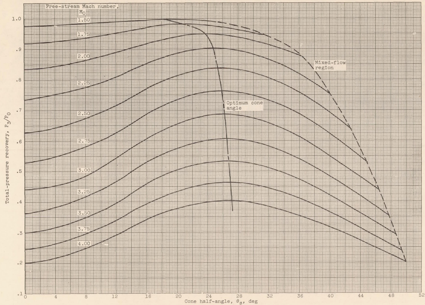
Figure 9. - Continued. Theoretical performance of single-cone and single-wedge inlets.
