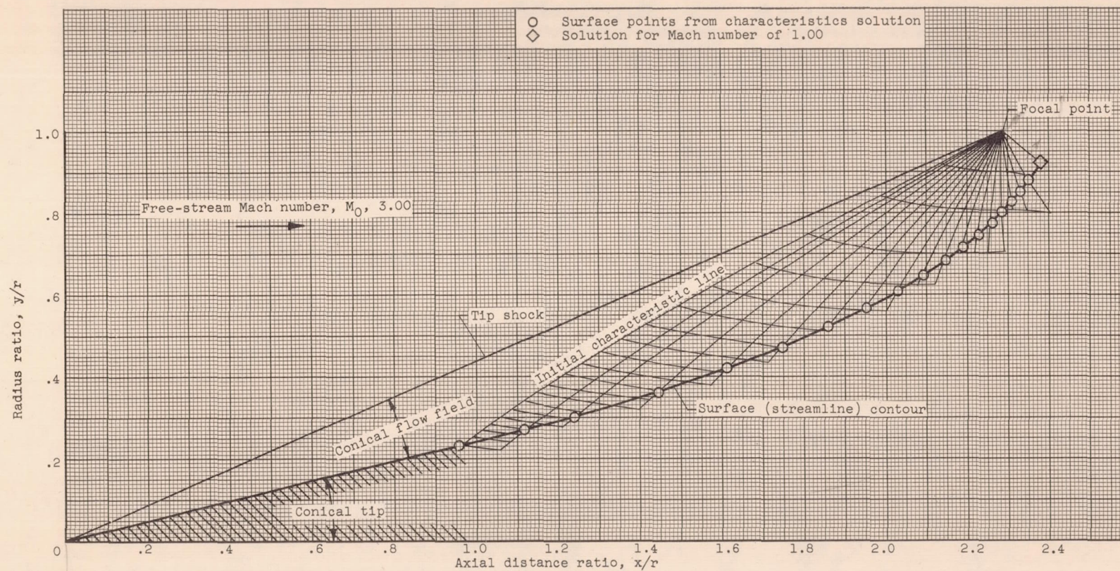
Figure 1. - Typical axisymmetric characteristics solution for isentropic spike.
