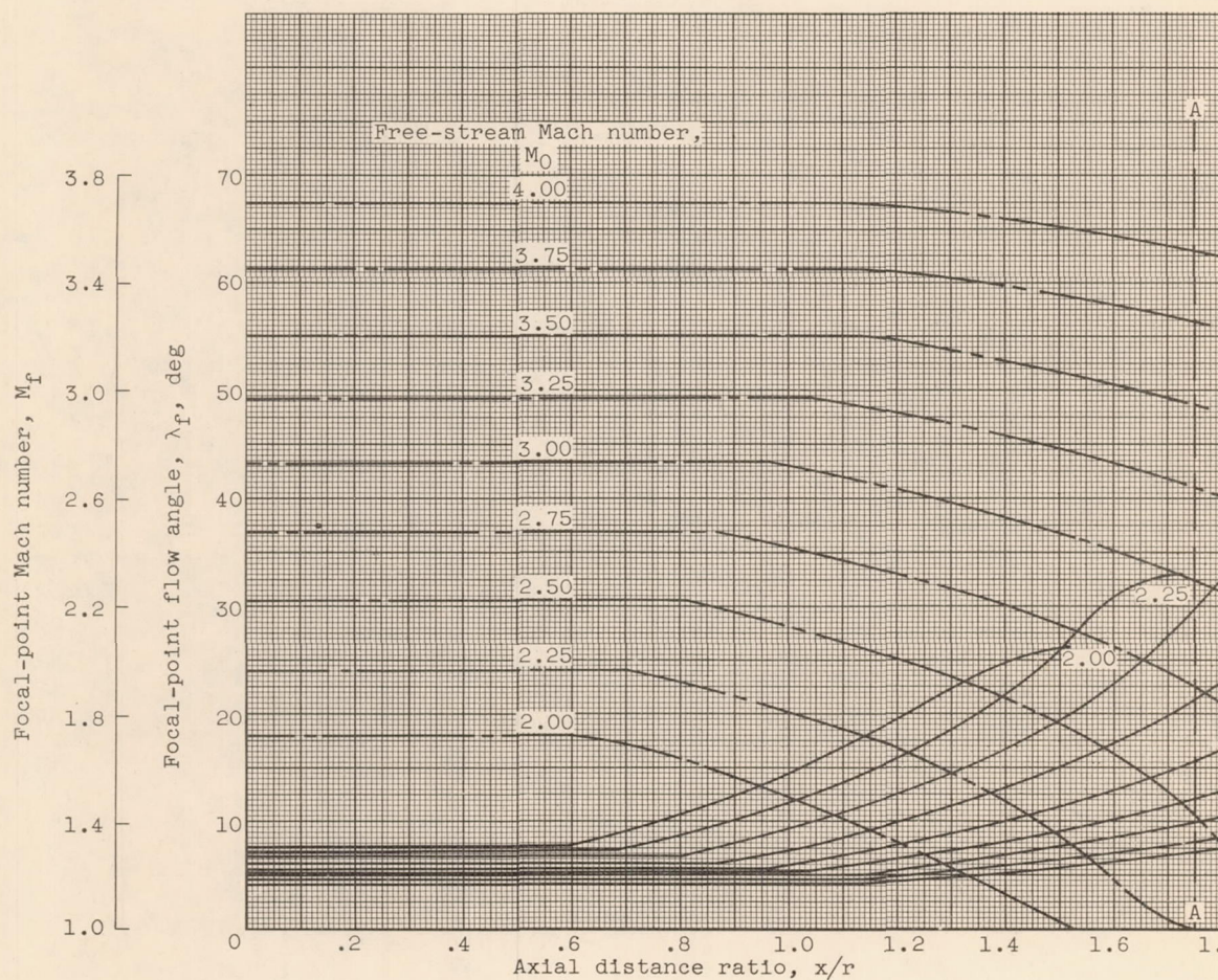
(c) Focal-point flow angle and Mach number.
