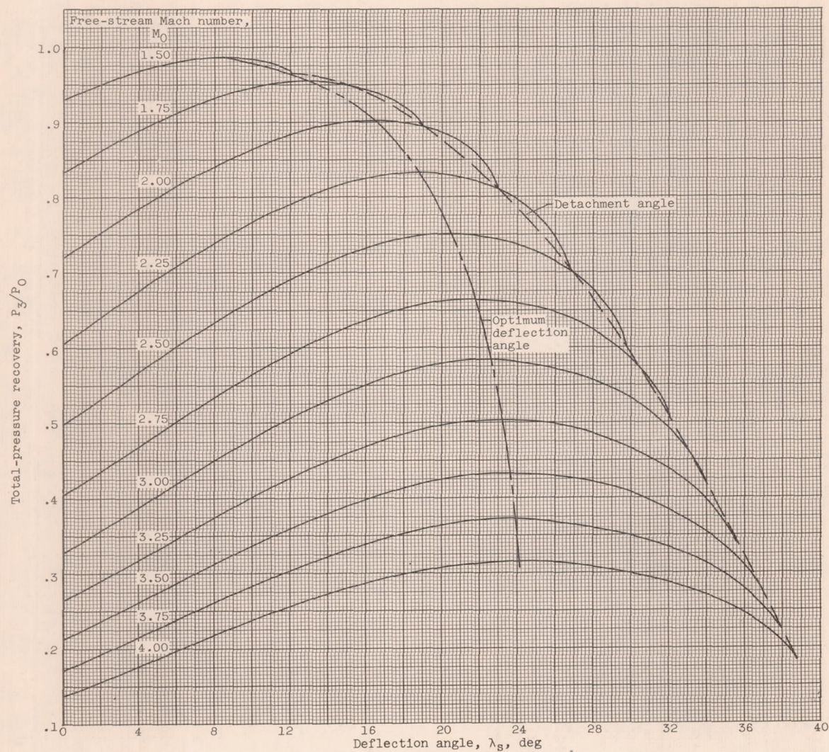
Figure 9. - Continued. Theoretical performance of single-cone and single-wedge inlets.
