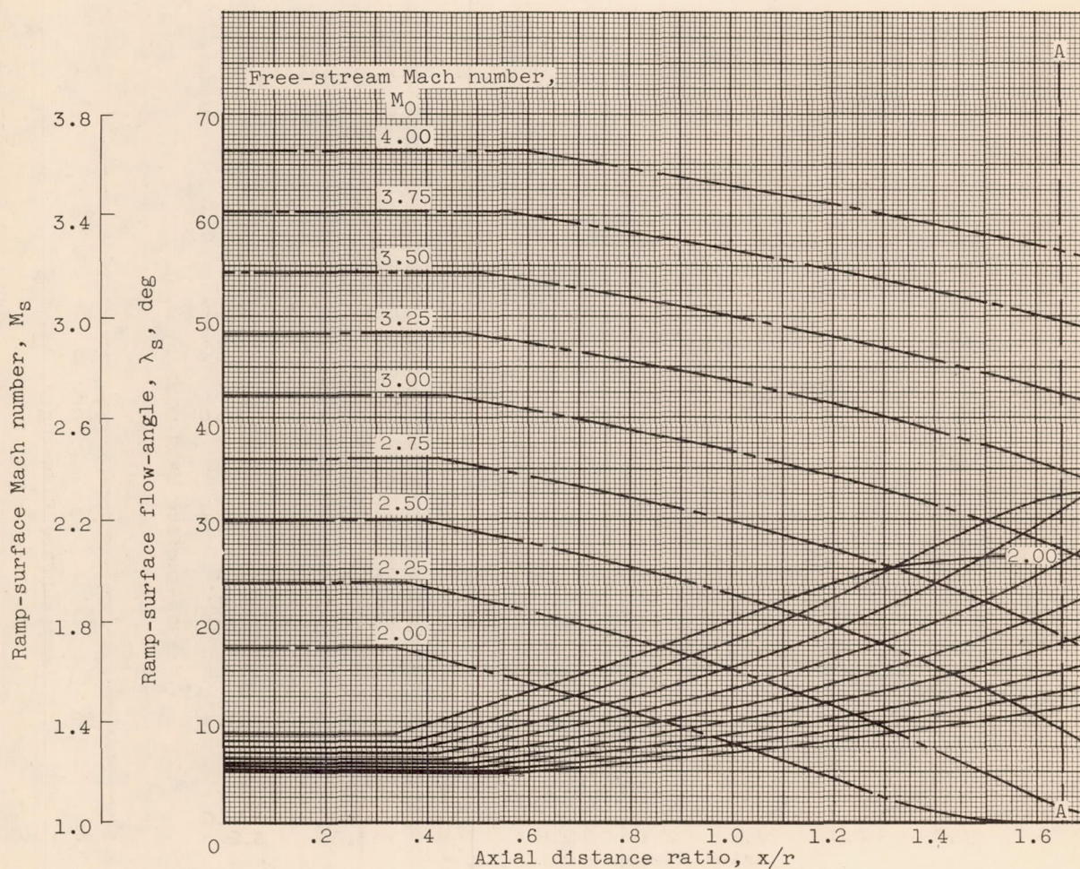
(b) Mach number and flow-angle variation.
