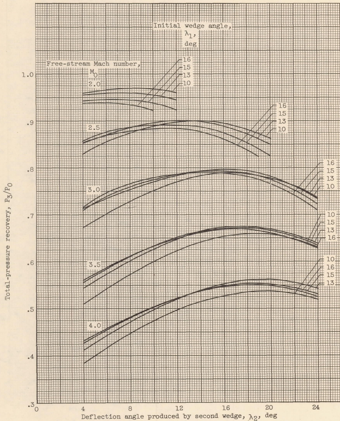
Figure 10. - Concluded. Theoretical performance of double-cone and double-wedge inlets.
