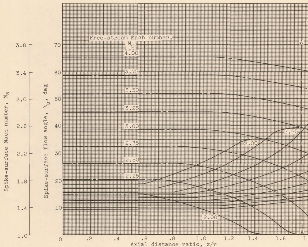
(b) Surface flow angle and Mach number.
