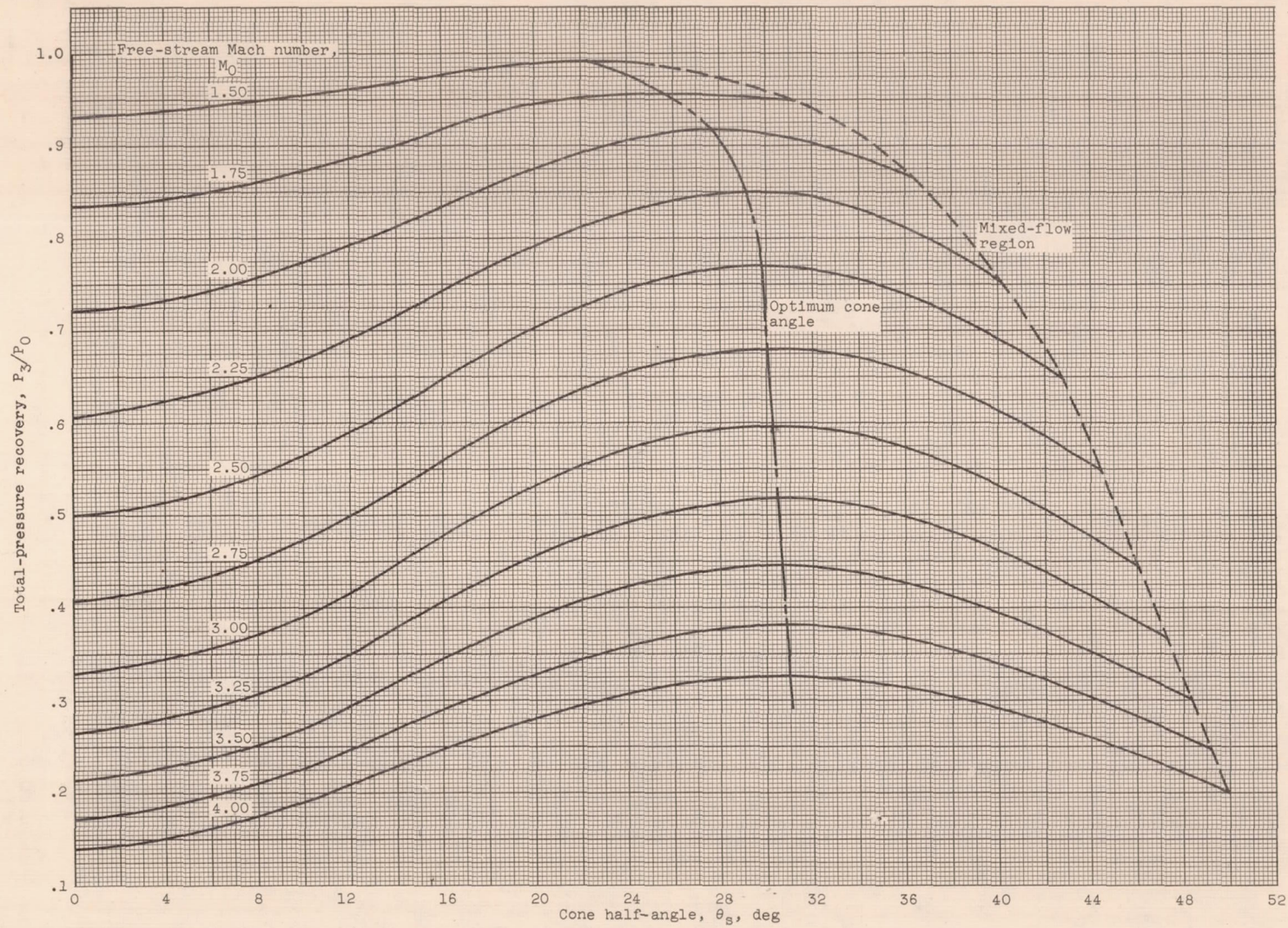
Figure 9. - Theoretical performance of single-cone and single-wedge inlets.
