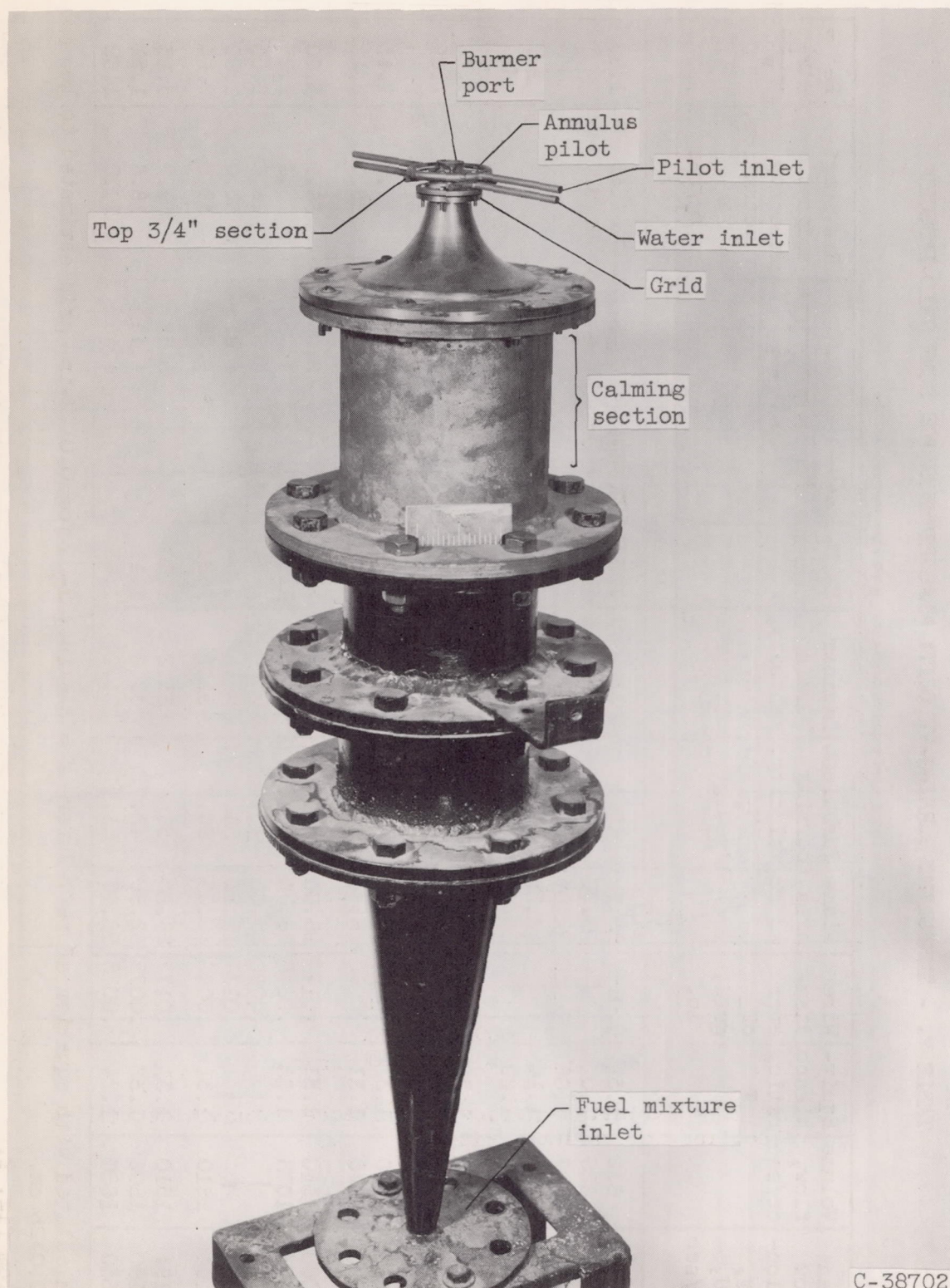
Figure 1. - 1/2-Inch nozzle burner.
