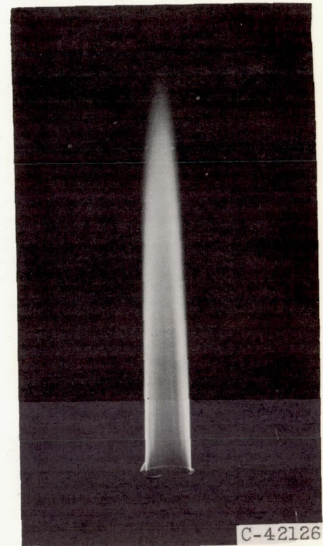
0.0090-Inch-wire grid; rms longitudinal velocity fluctuation, 28.4 cm/sec
