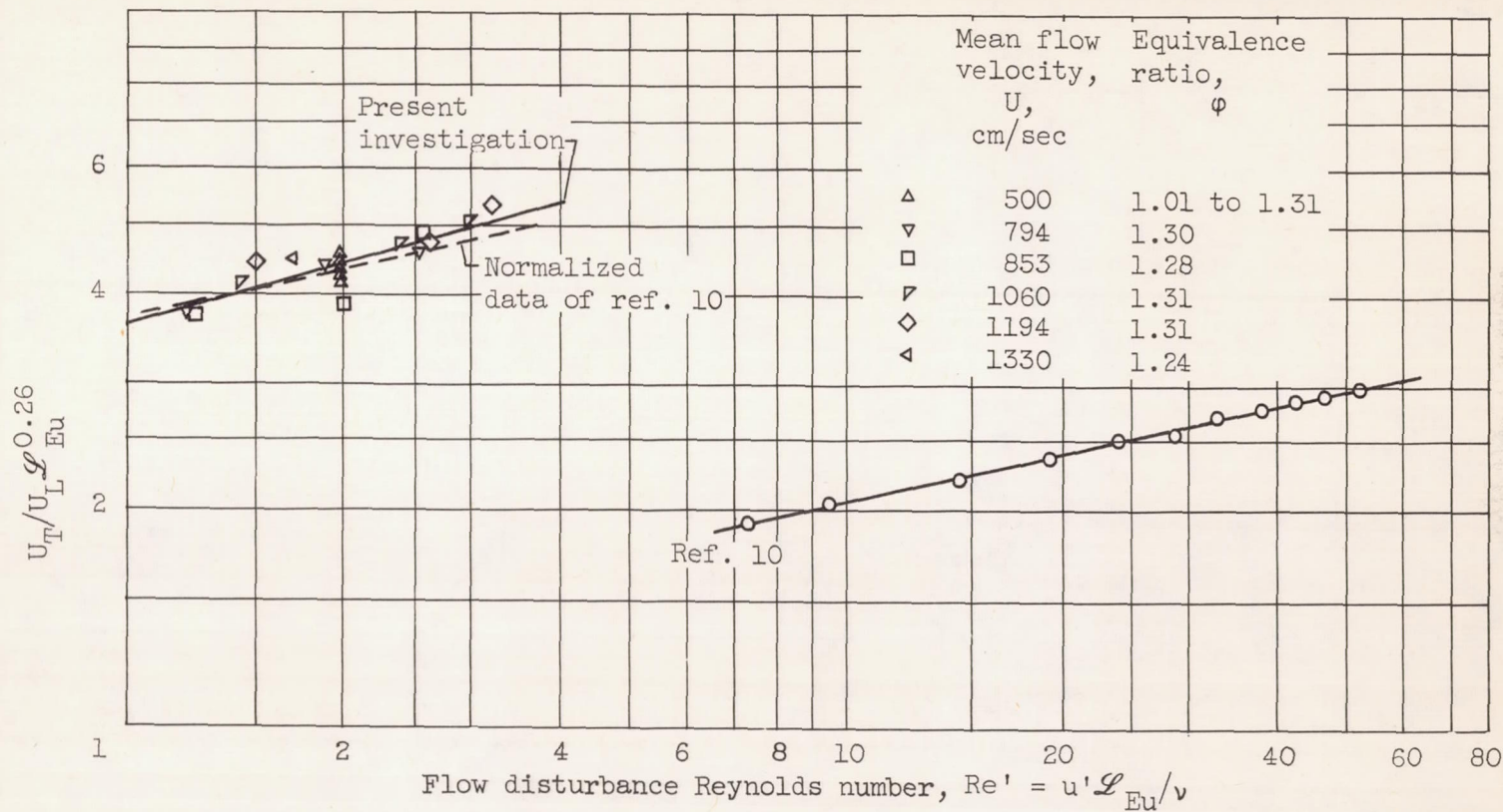
Figure 5. - Comparison of turbulent burning-velocity measurements of reference 10 with those from present investigation.
