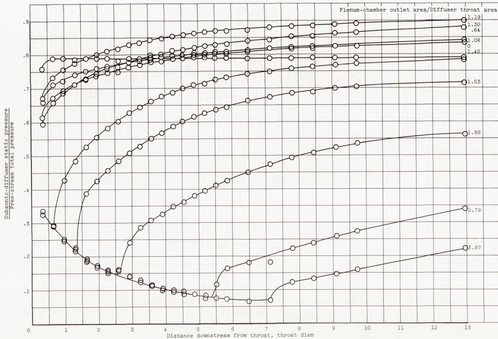
Figure 4. - Continued. Static-pressure distribution along subsonic diffuser. Free-stream Mach number, 1.85.
