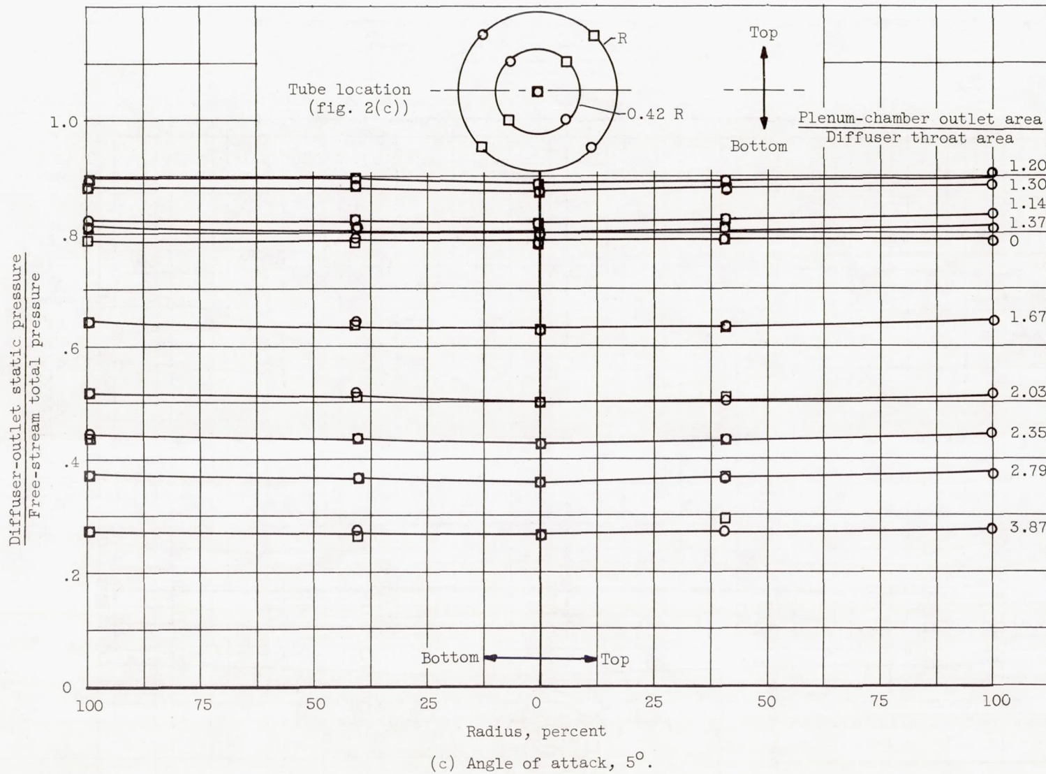
Figure 5. - Concluded. Static-pressure distribution across diffuser outlet. Free-stream Mach number, 1.85.
