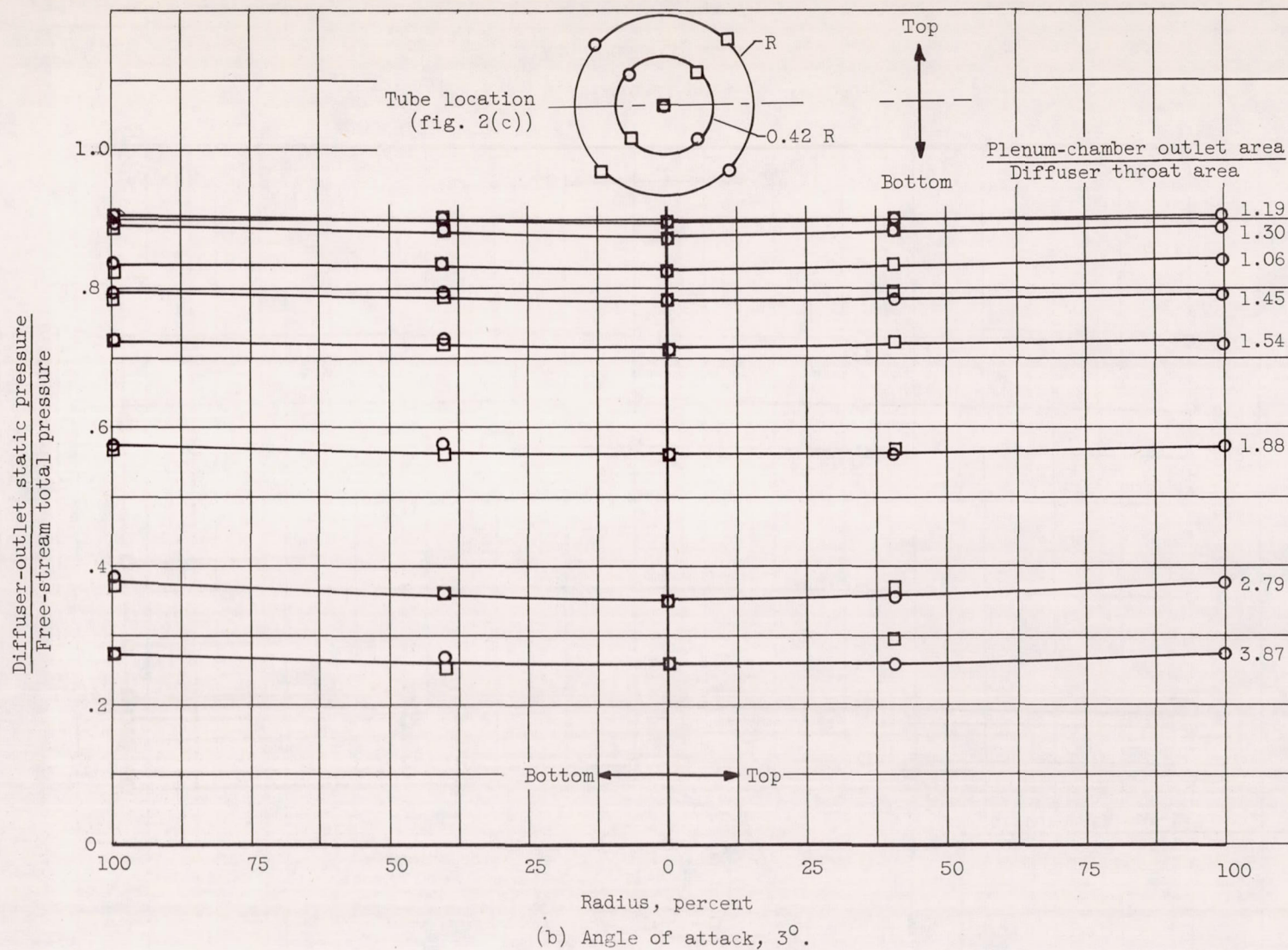
Figure 5. - Continued. Static-pressure distribution across diffuser outlet. Free-stream Mach number, 1.85.
