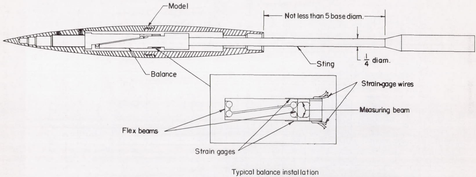
Figure 3.- Wire strain-gage balance.
