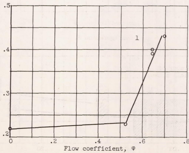
Figure 8. - Stall propagation rate as a function of flow coefficient.
