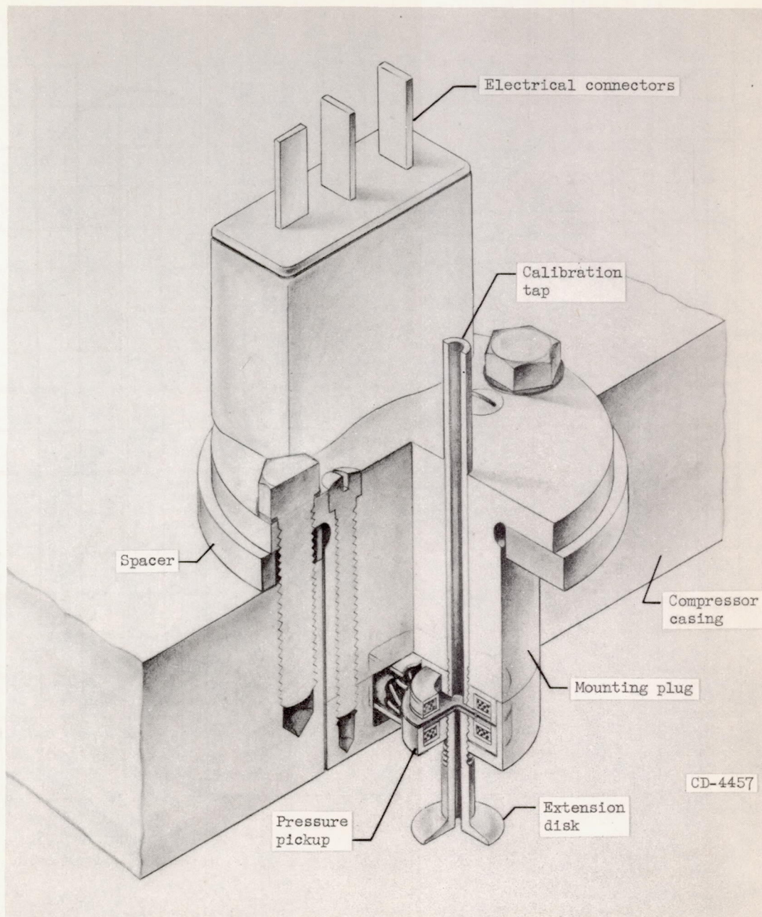
Figure 4. - Installation of pressure pickup in compressor casing.
