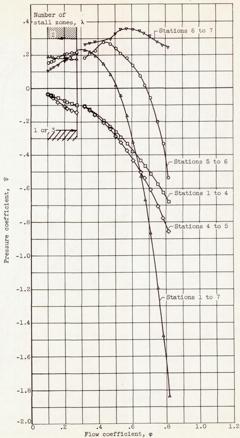
Figure 5. - Continued. Steady-state performance and rotating stall regions.
