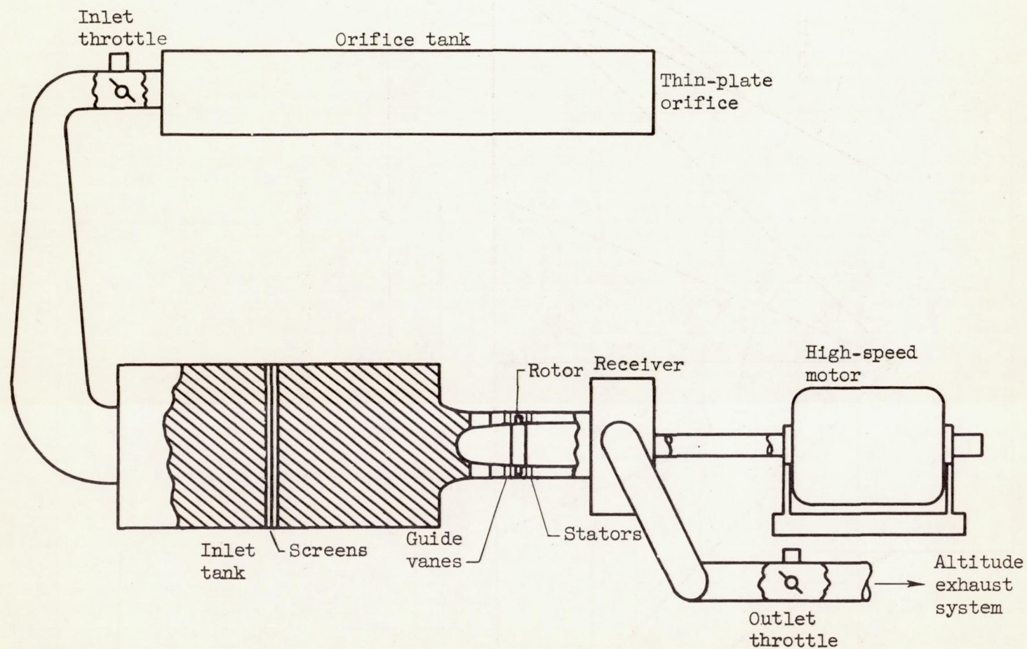
Figure 2. - Compressor installation.
