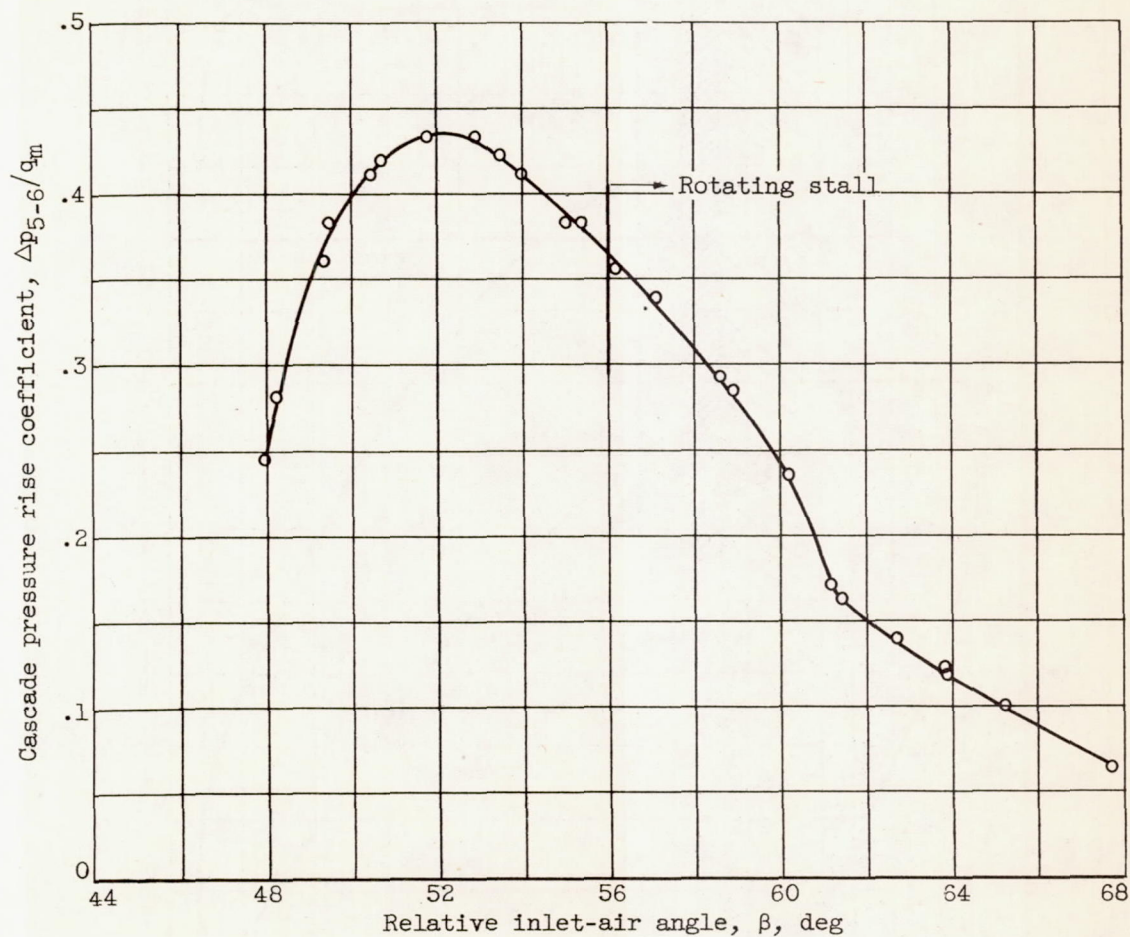
(a) Configuration 1. Guide-vane turning angle, -22.5^\circ ; no stators; corrected rotor speed, 8000 rpm.
