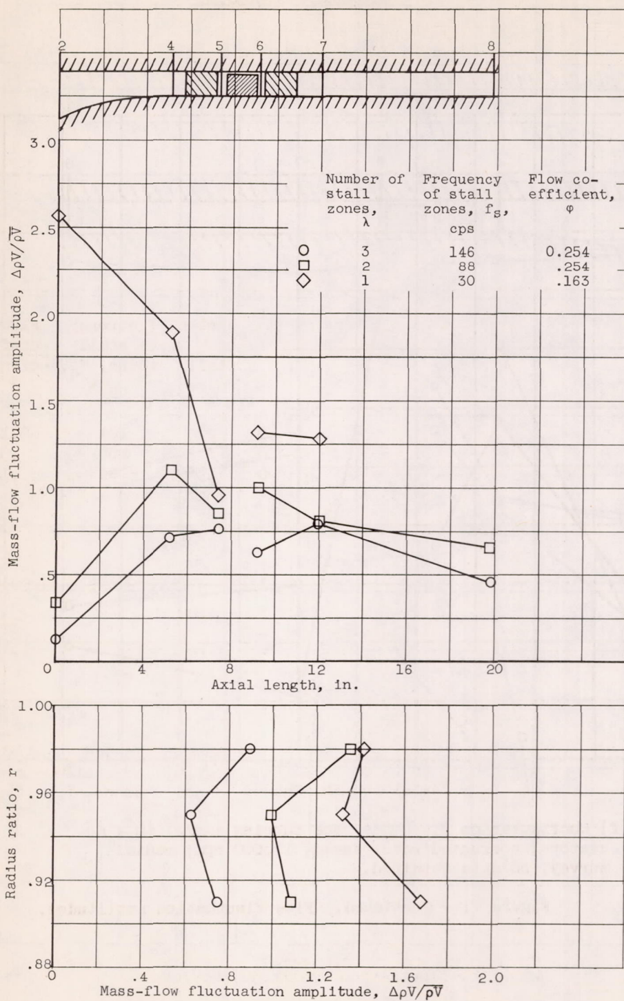
(g) Configuration 8. Guide-vane turning angle, 40^\circ ; stators; corrected rotor speed, 8000 rpm; radial survey at station 6; axial survey along stage axis.
