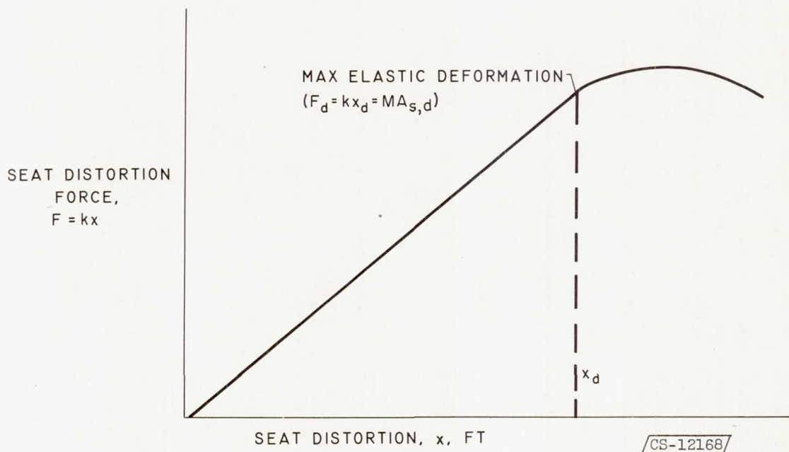
Figure 3. - Seat elasticity.
