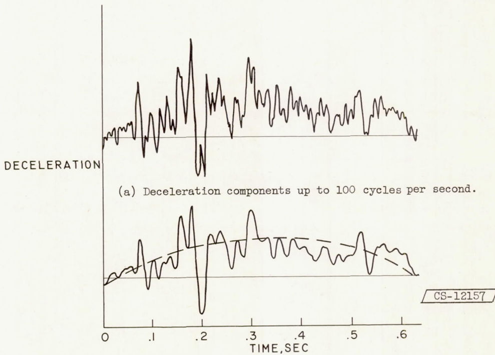
Figure 1. - Fuselage floor deceleration, longitudinal.
