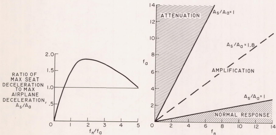
(a) Ratio of maximum seat to maximum airplane decelerations against frequency ratio.
