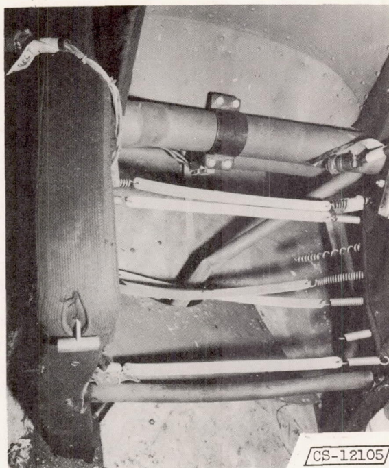
Figure 27. - Seat-pan failure.
