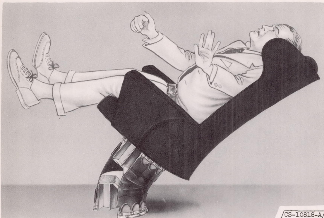
Figure 18. - Experimental duplex seat, impact from rear.
