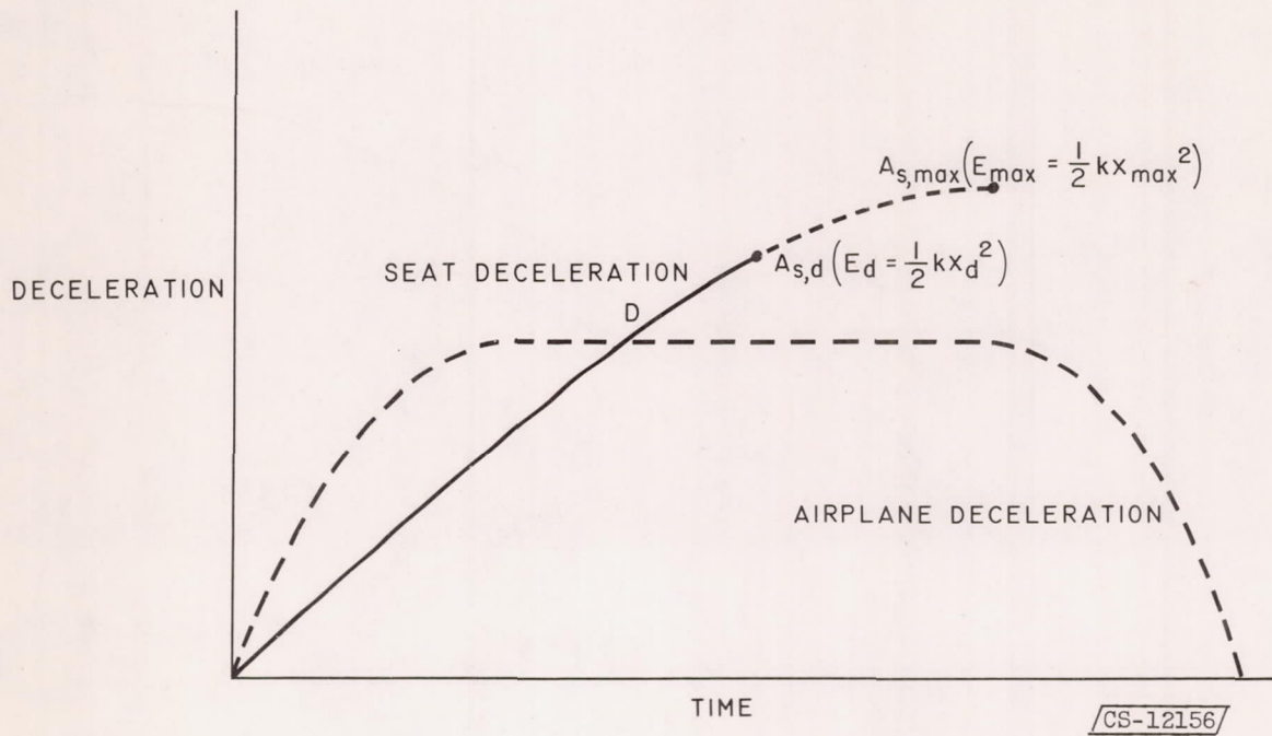
Figure 12. - Energy for seat failure.
