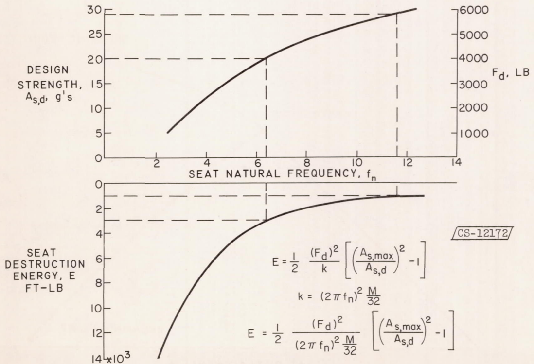
(b) Determination of seat-destruction energy requirement.
