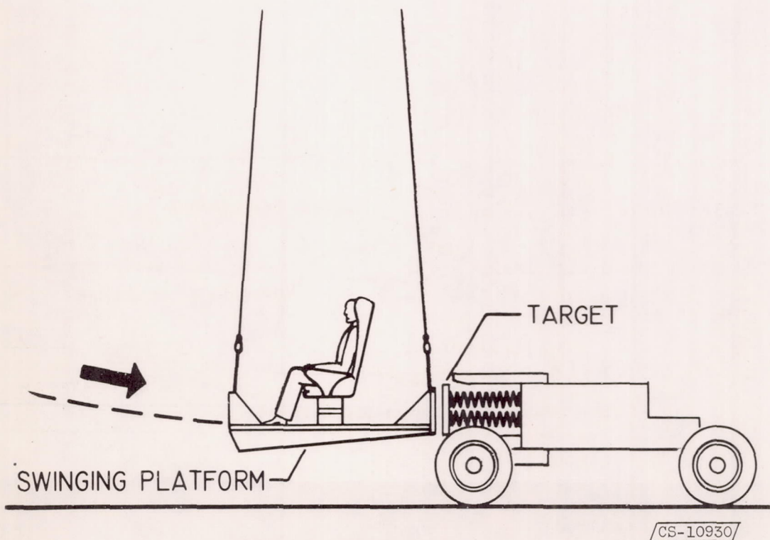
Figure 19. - Impact swing.
