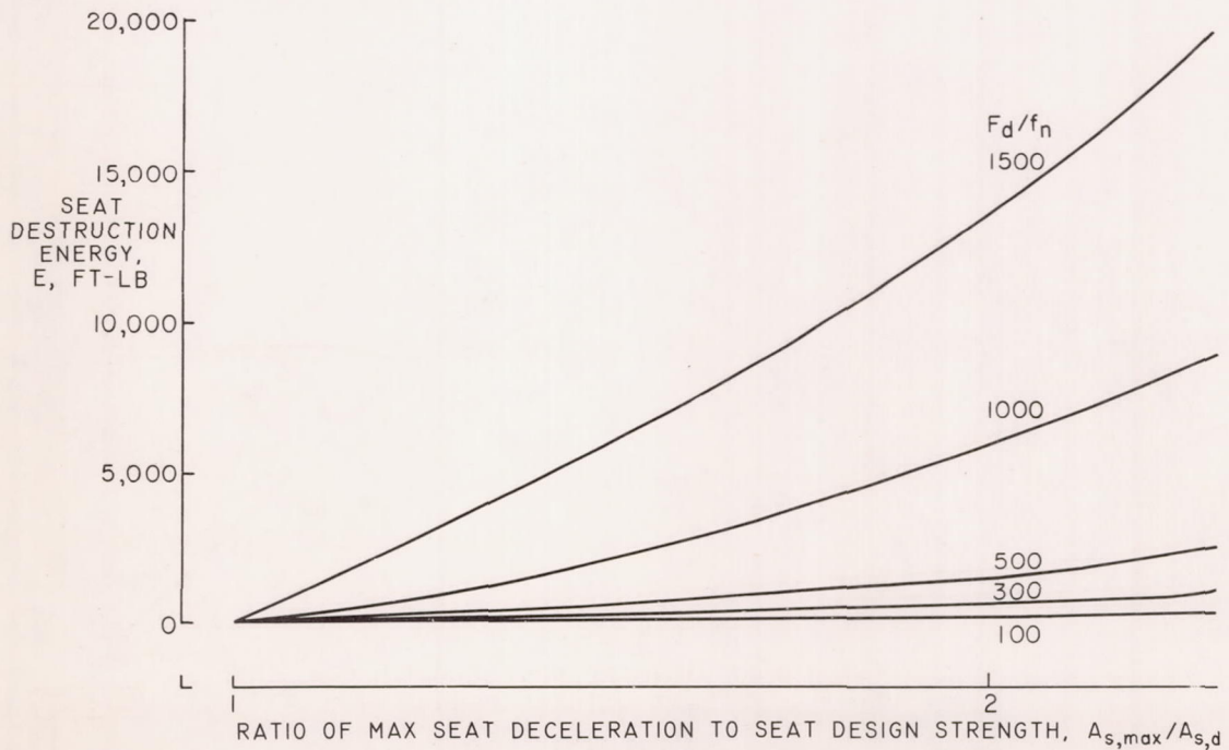
Figure 13. - Energy for seat destruction.
