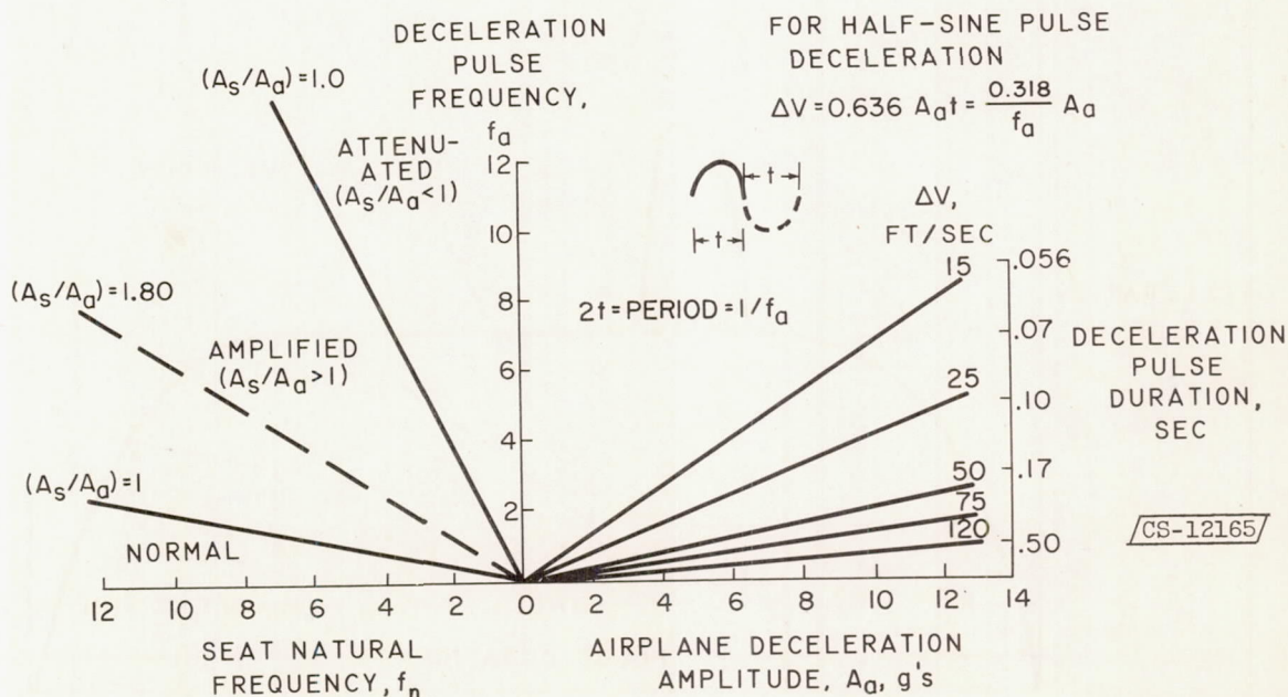
Figure 8. - Seat response, half-sine pulse.
