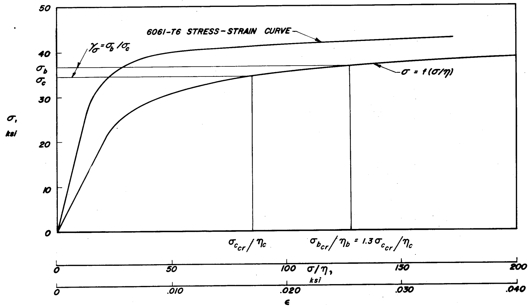
Figure 24.- Stress-strain curve for 6061-T6 aluminum alloy and derived curve of \sigma as a function of \sigma/\eta .
