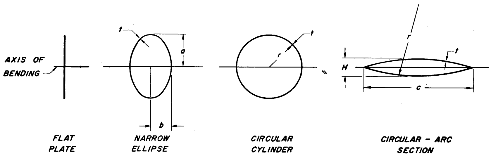
Figure 14.- Elliptic-cylinder geometry.
