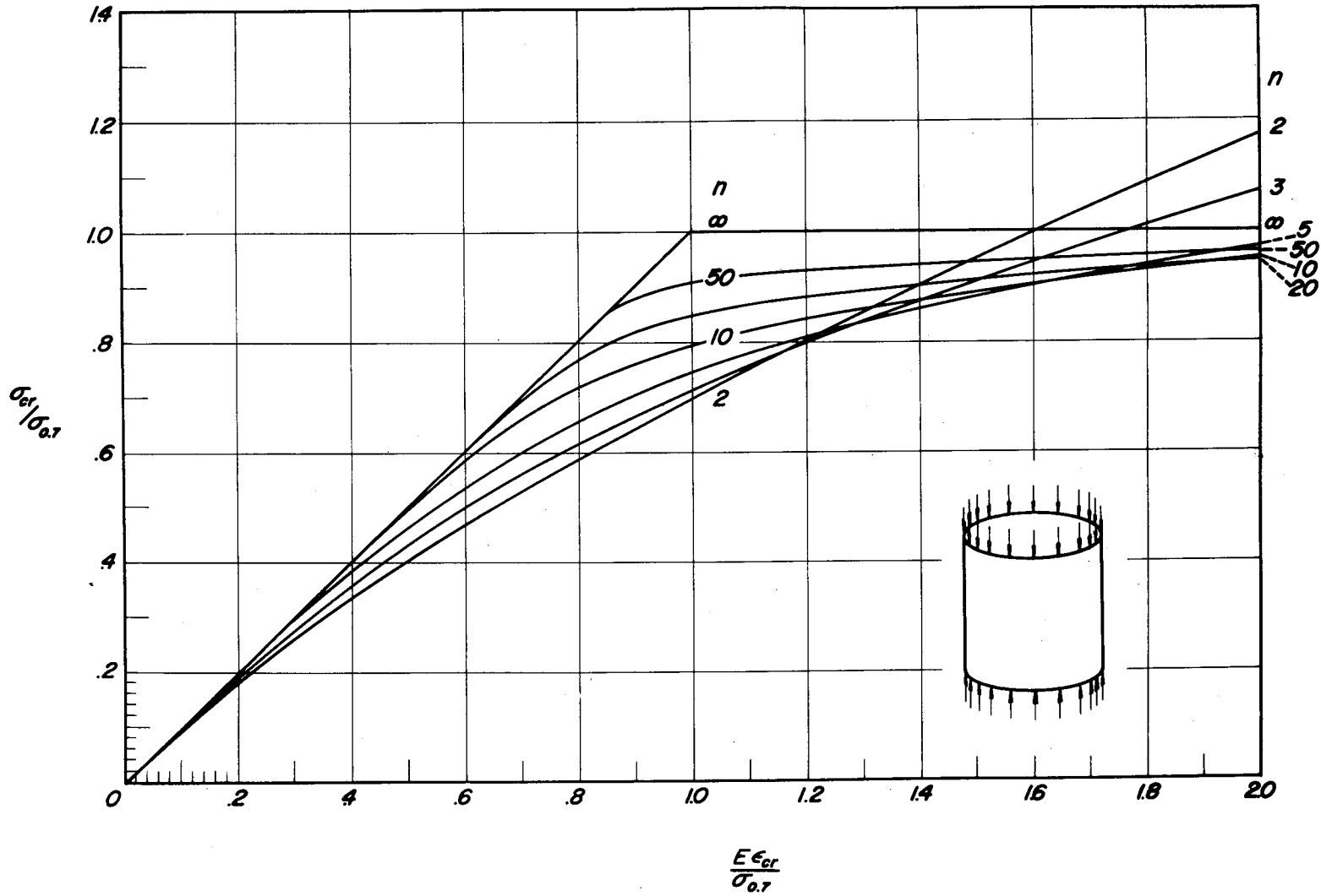
Figure 11.- Nondimensional buckling chart for axially compressed long circular cylinders.
