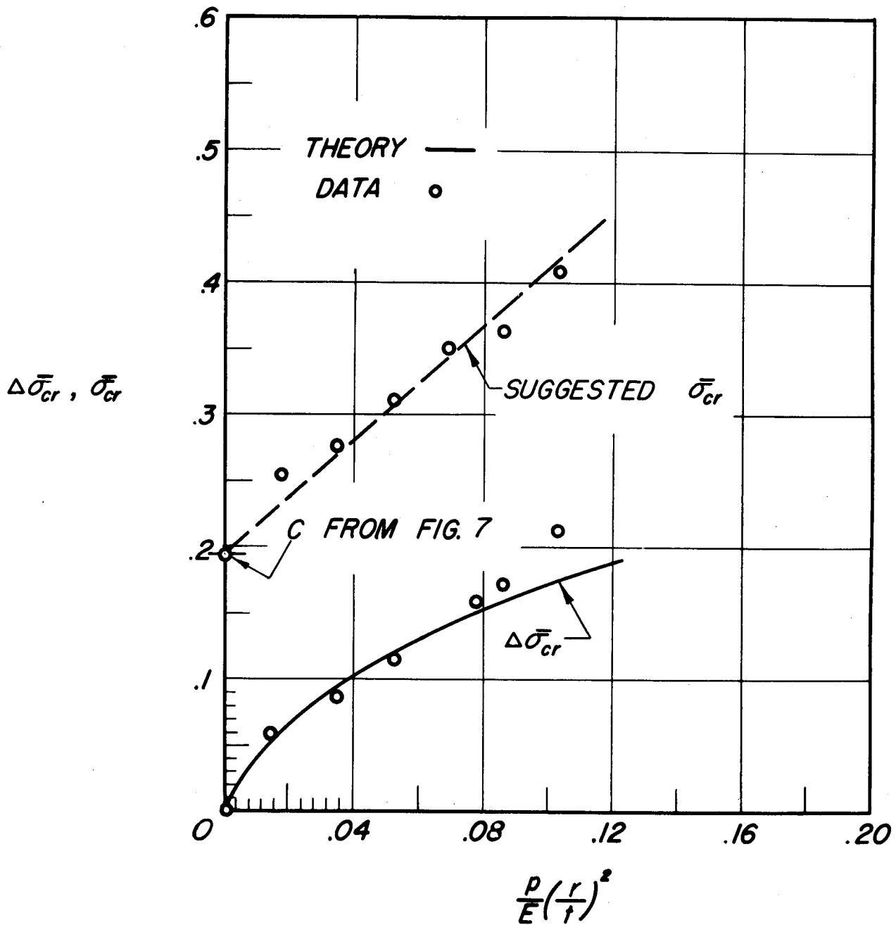
Figure 13.- Effect of internal pressure on axial-compressive-buckling stress of circular cylinders. \bar{\sigma}_{cr} = \frac{\sigma_{cr}r}{Et} .
