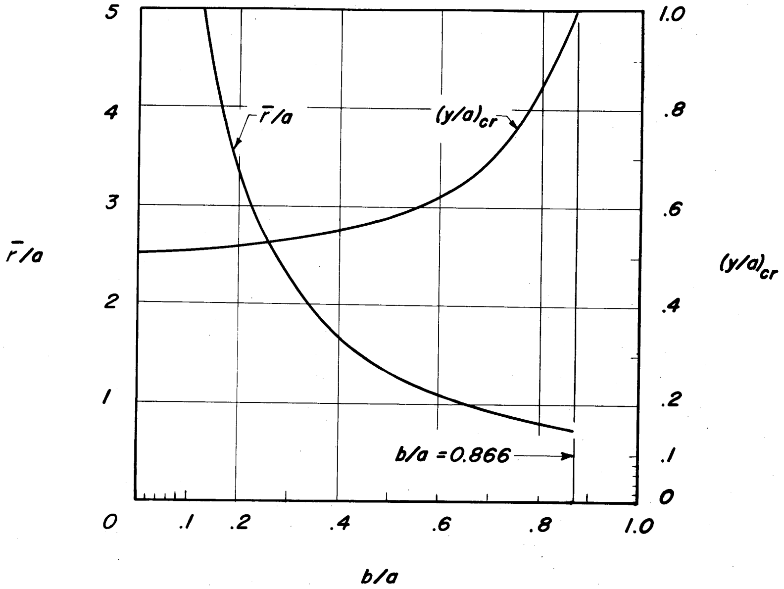
Figure 19.- Location and magnitude of critical radius of elliptic cylinder.
