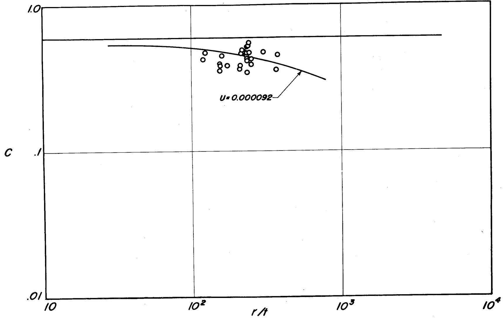
Figure 41.- Theoretical variation of C as a function of r/t for U = 0.000092 and comparison with elastic data of Schuette (ref. 65) for axially compressed curved plates.
