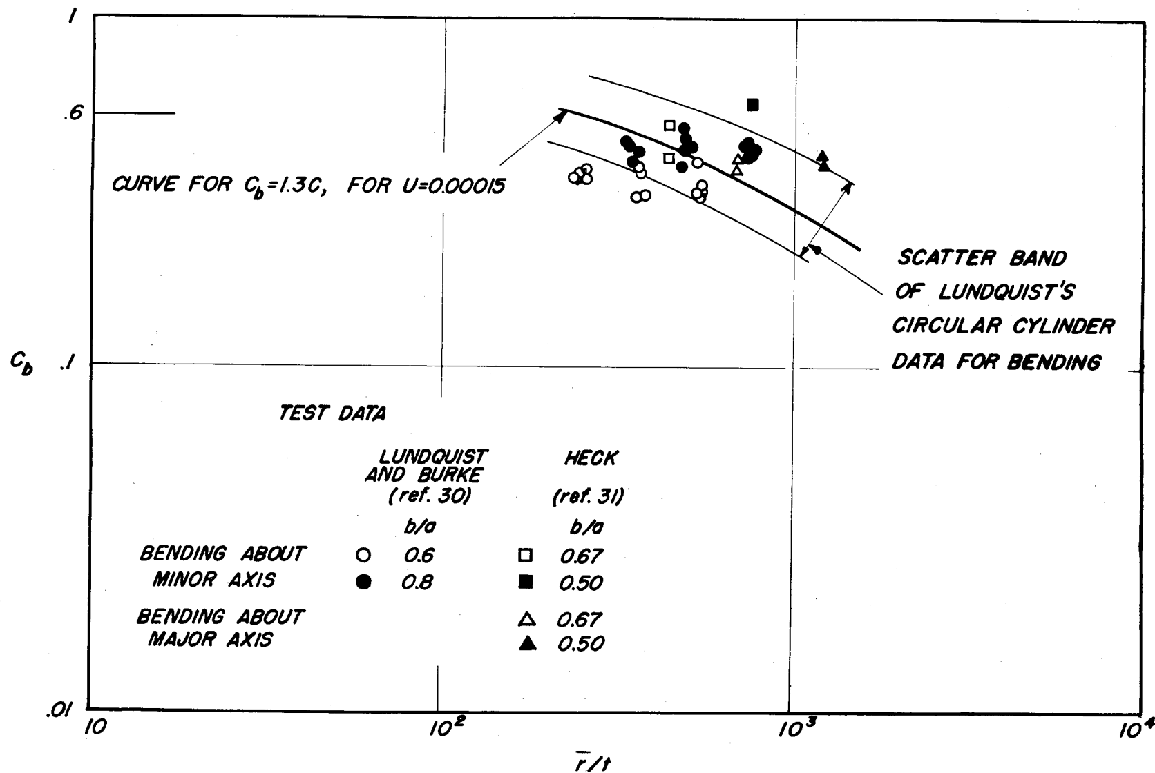
Figure 18.- Test data for long elliptic cylinders in bending.
