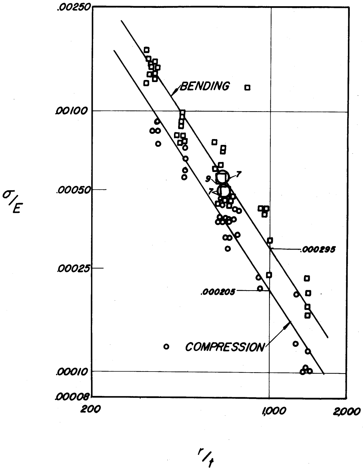
Figure 17.- Test data of Lundquist for long circular cylinders in axial compression and in bending (refs. 14 and 29).
