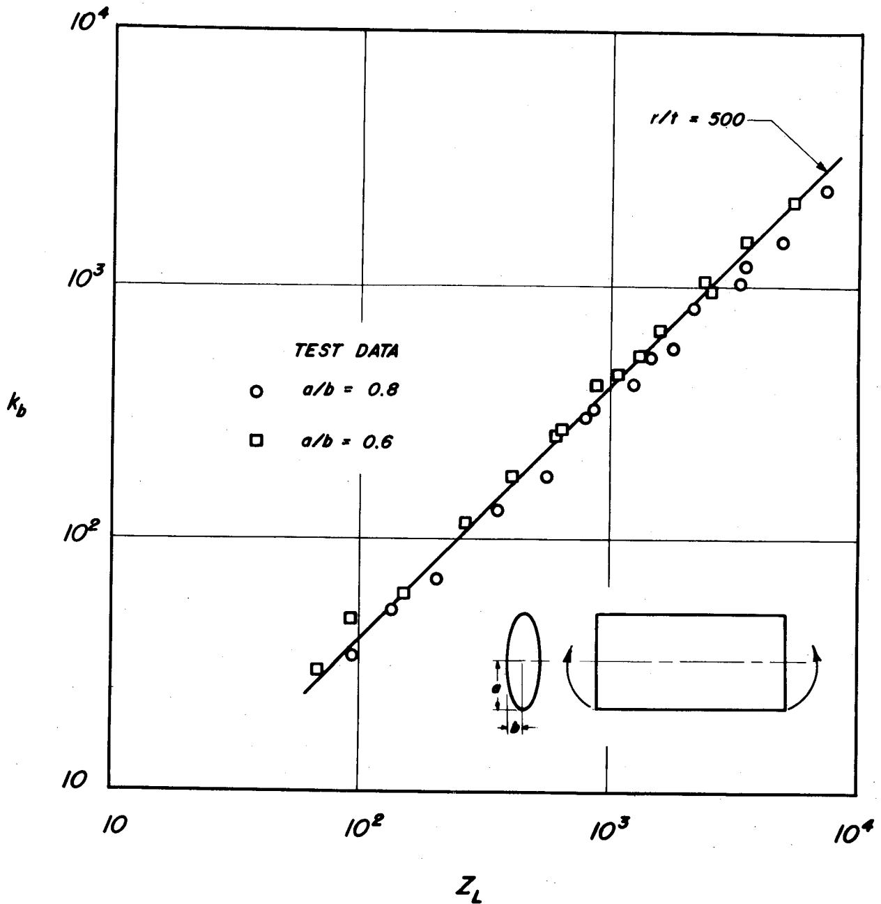
Figure 20.- Comparison of test data on elliptic cylinders with empirical curve for \bar{r}/t = 500 . For test data, 250 < \bar{r}/t < 750 .
