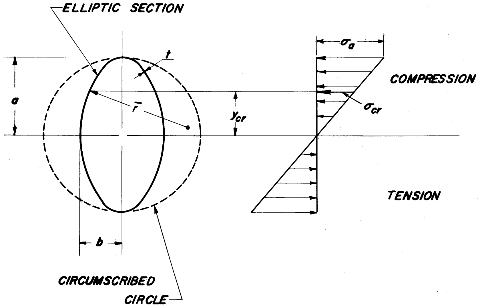
Figure 21.- Location of critical radius of curvature for elliptic cylinders in bending.
