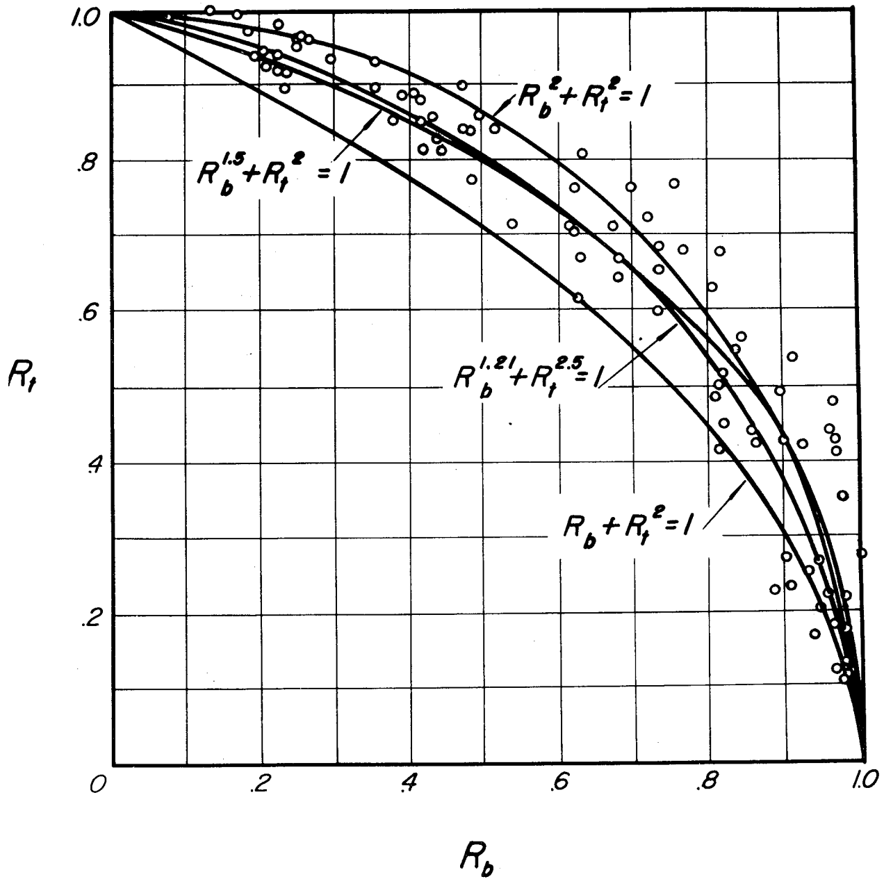
(c) Combined torsion and bending.
