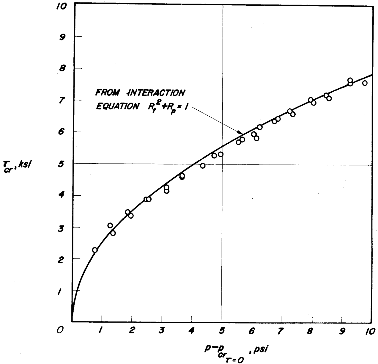
Figure 33.- Effect of internal pressure on torsional-buckling stress of long cylinders. Test results are from reference 43.
