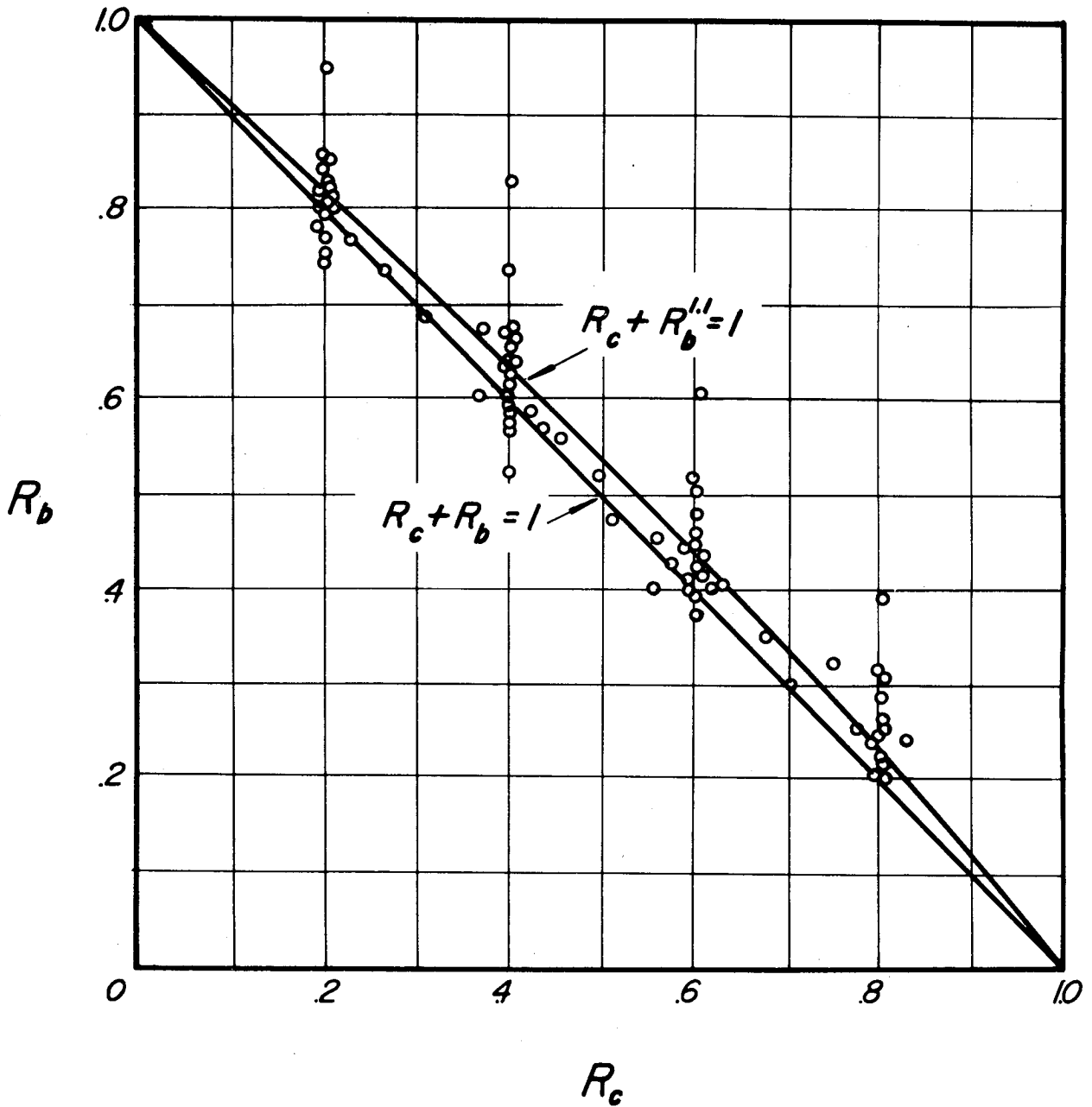
(a) Combined bending and compression.
