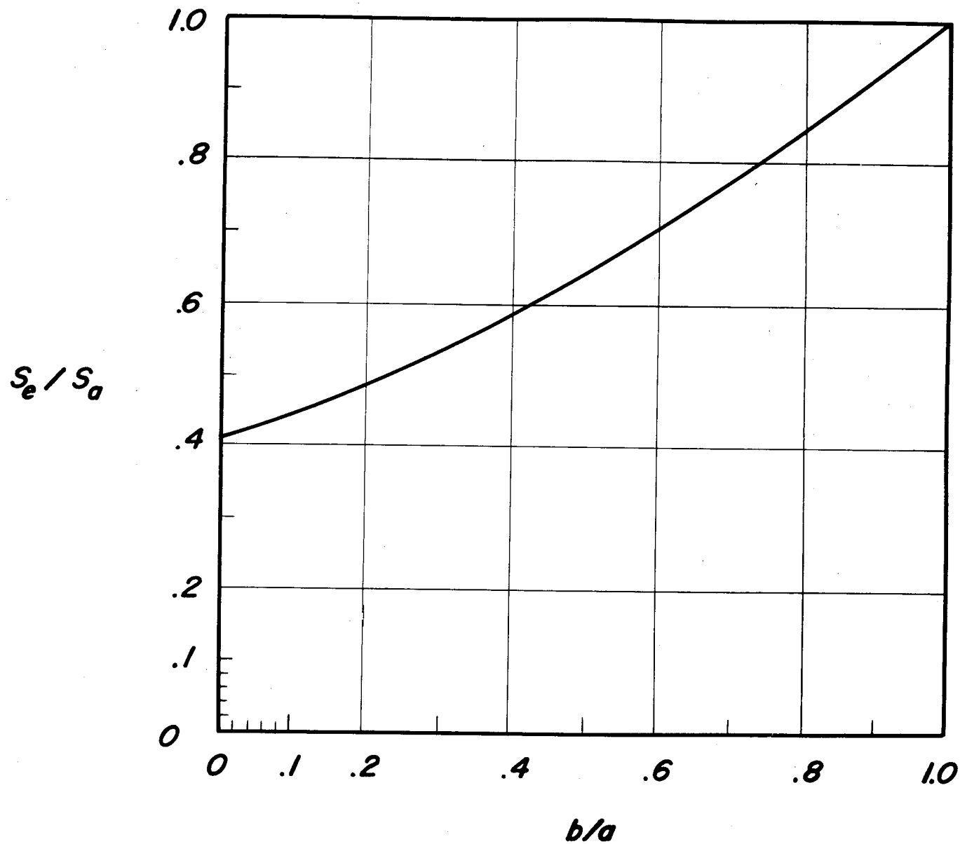
Figure 22.- Section modulus of elliptic cylinder.
