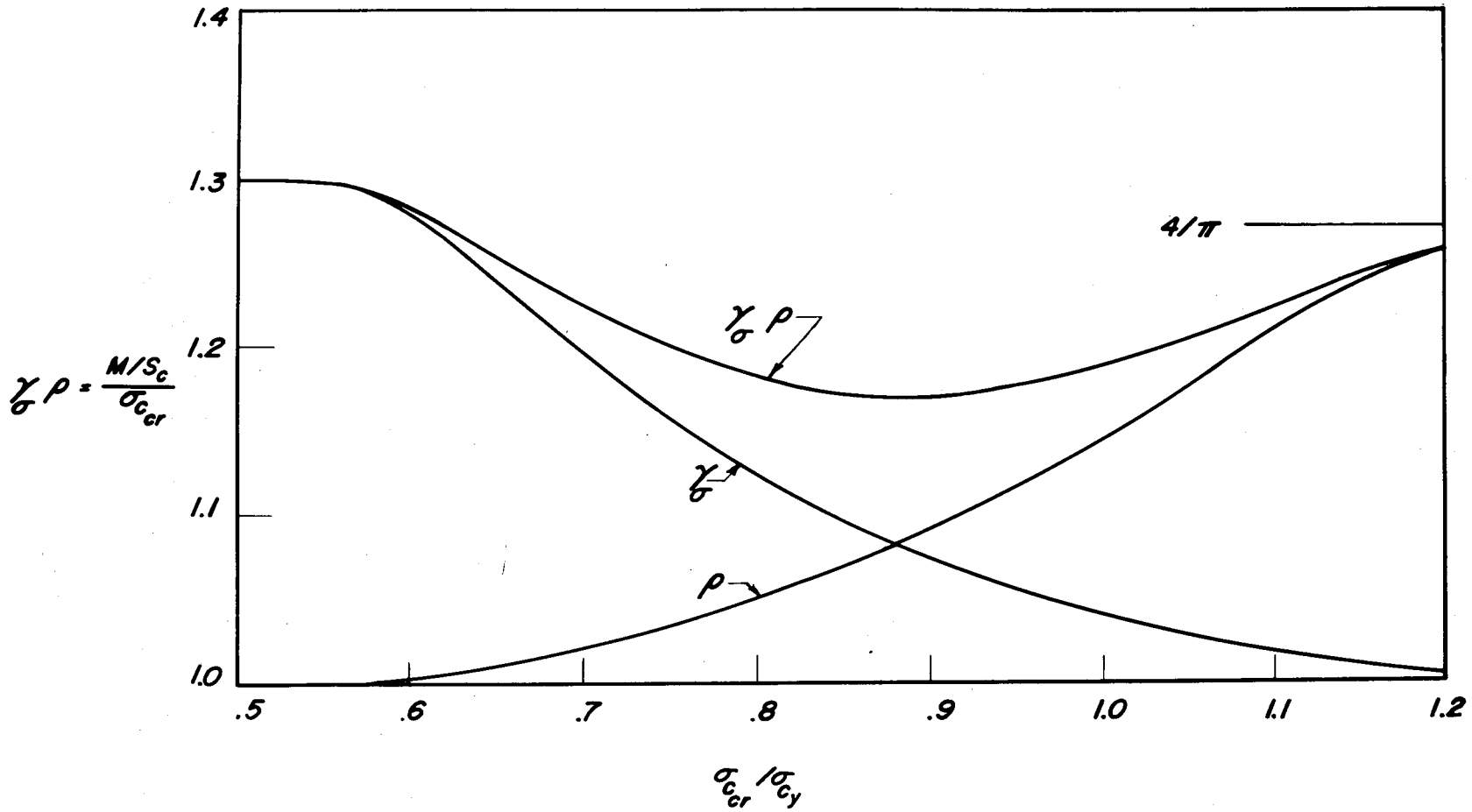
(a) Theoretical variation based on 6061-T6 aluminum-alloy data of figure 24. Figure 25.- Variation of (M/S_c)/\sigma_{cr} for long circular cylinders in bending.
