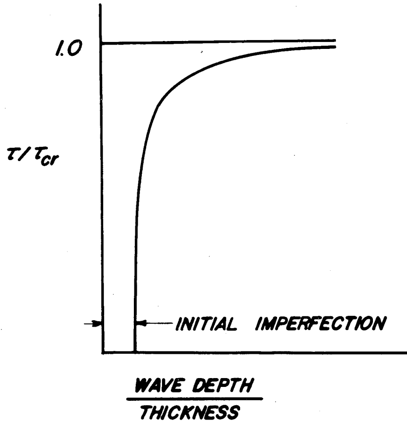
Figure 28.- Buckling stress as a function of buckle wave depth for circular cylinders in torsion. Curve taken from test data.
