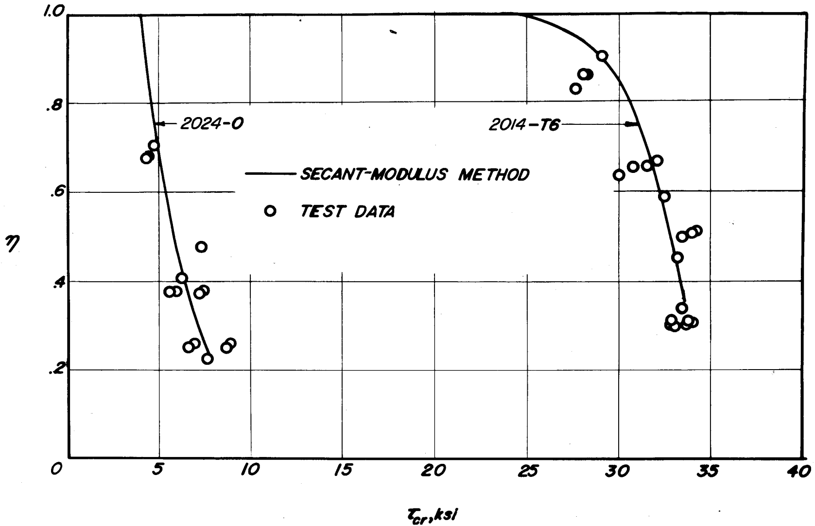
Figure 29.- Comparison of test data with plasticity-reduction factor for long flat plates in shear. Data from reference 44.
