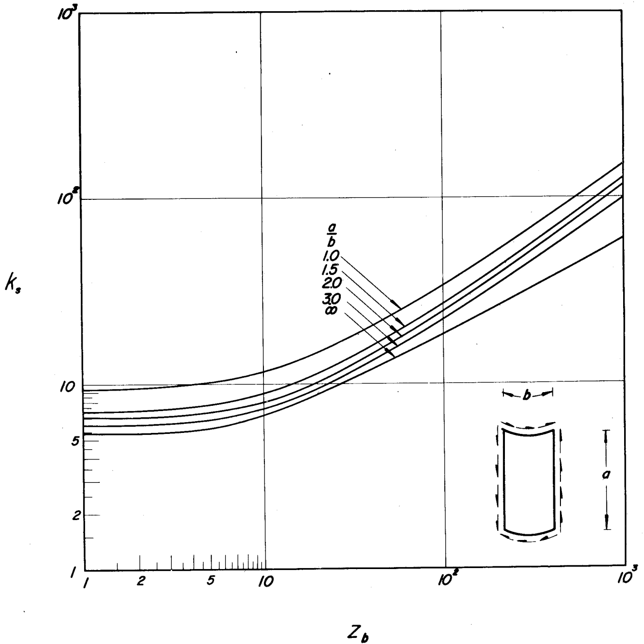
(a) Long simply supported plates.
