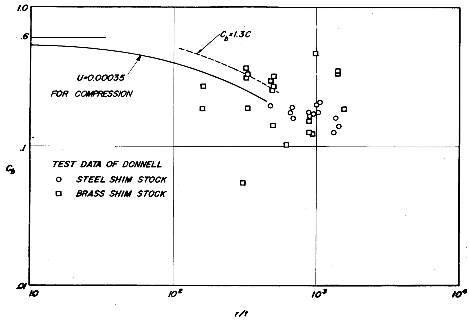
(b) Data of Donnell (ref. 8).
