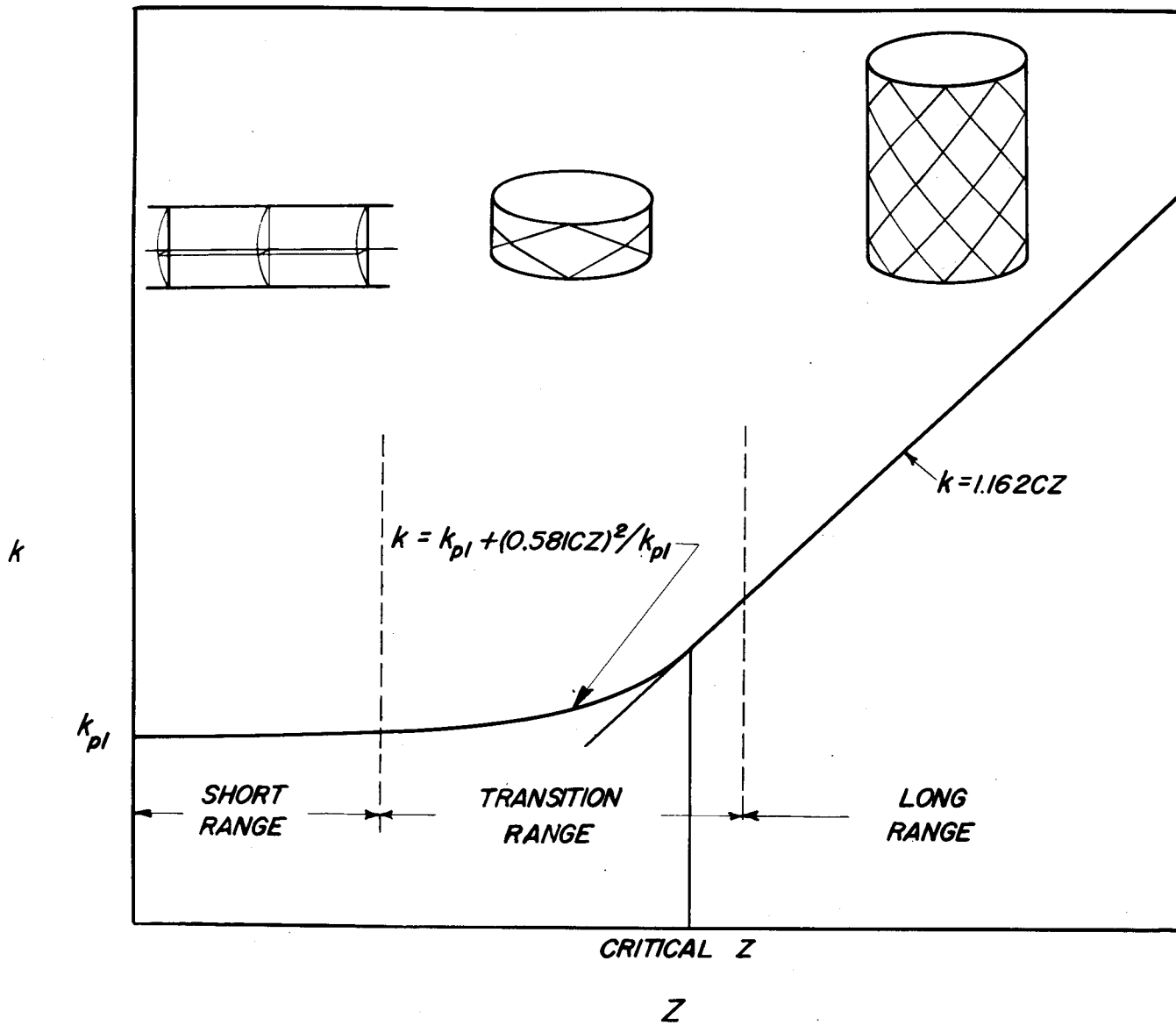
Figure 5.- Method of construction of curve for k as a function of Z . Typical buckle patterns shown for cylinder in each range of Z .
