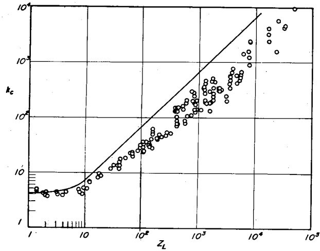
(a) Axial compression.
