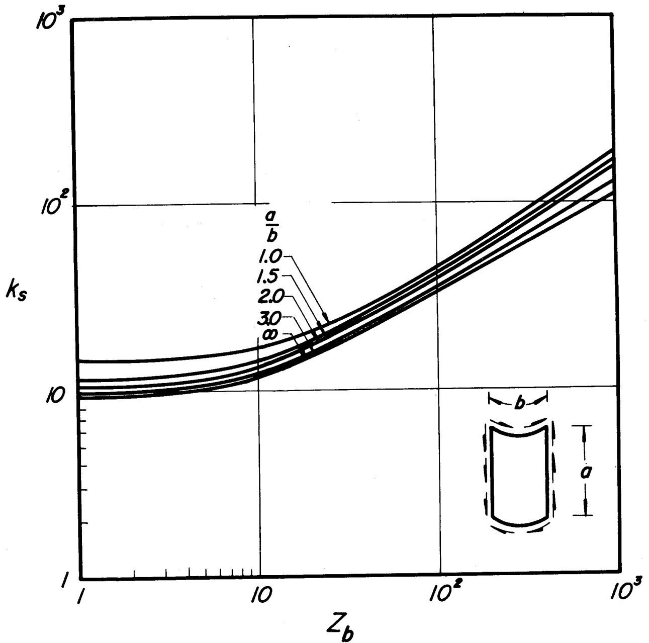
(b) Long clamped plates.
