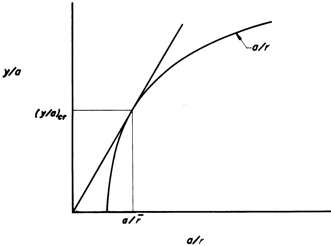
Figure 23.- Method for determining location and magnitude of critical radius of curvature.
