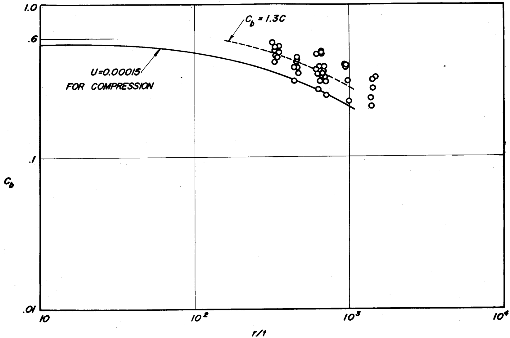
(a) Data of Lundquist for Duralumin sheet (ref. 29).
