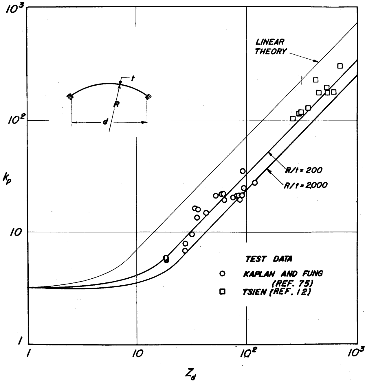
Figure 47.- Test data for spherical plates under external pressure compared with empirical theory.
