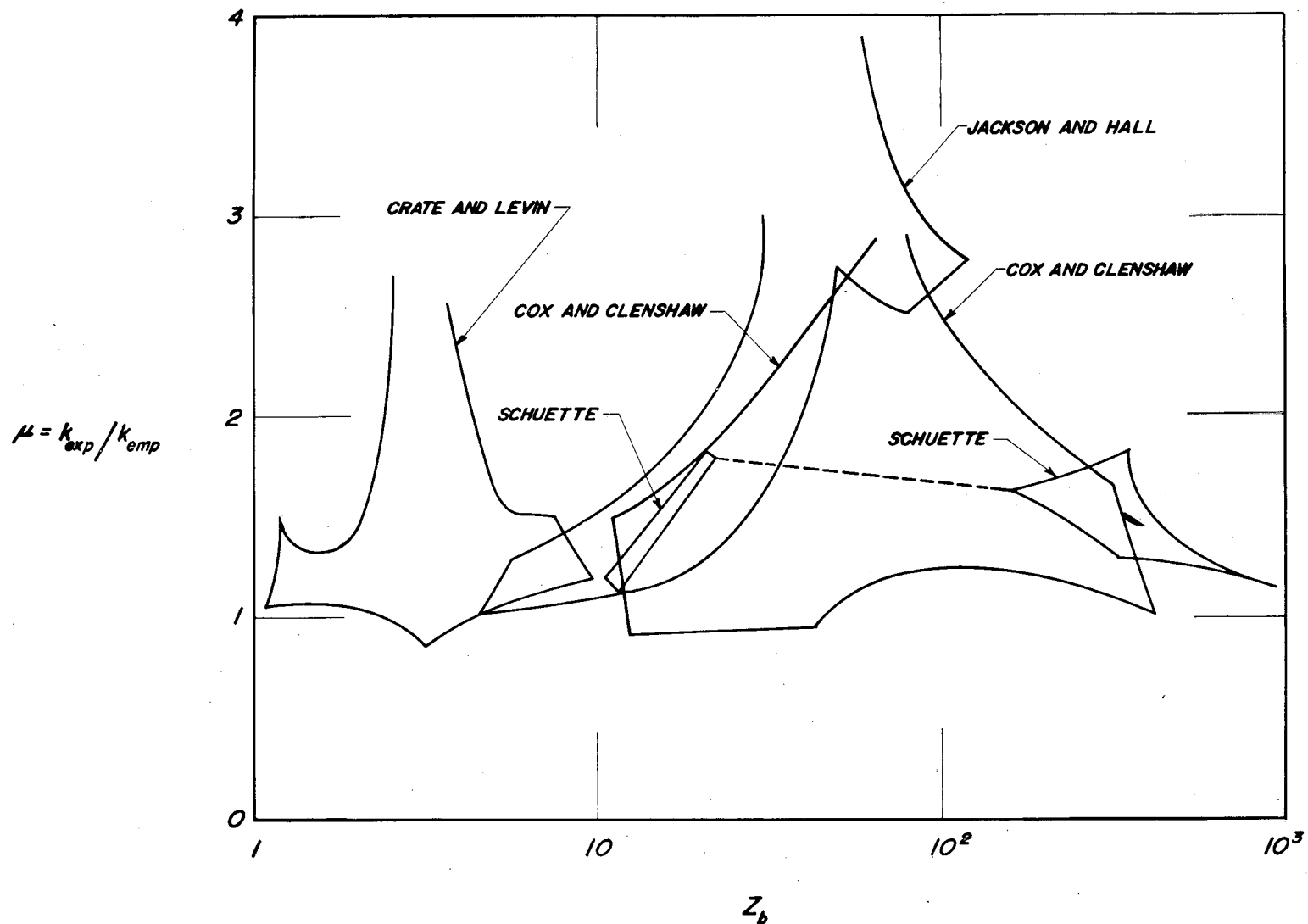
Figure 40.- Ranges of magnification factors for test data of figure 38(a). Data from Crate and Levine, reference 61; Cox and Clenshaw, reference 60; Jackson and Hall, reference 62; and Schuette, reference 65.
