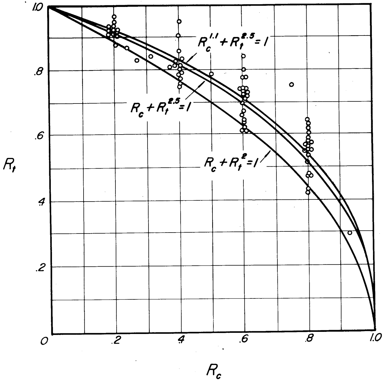
(b) Combined compression and torsion.
