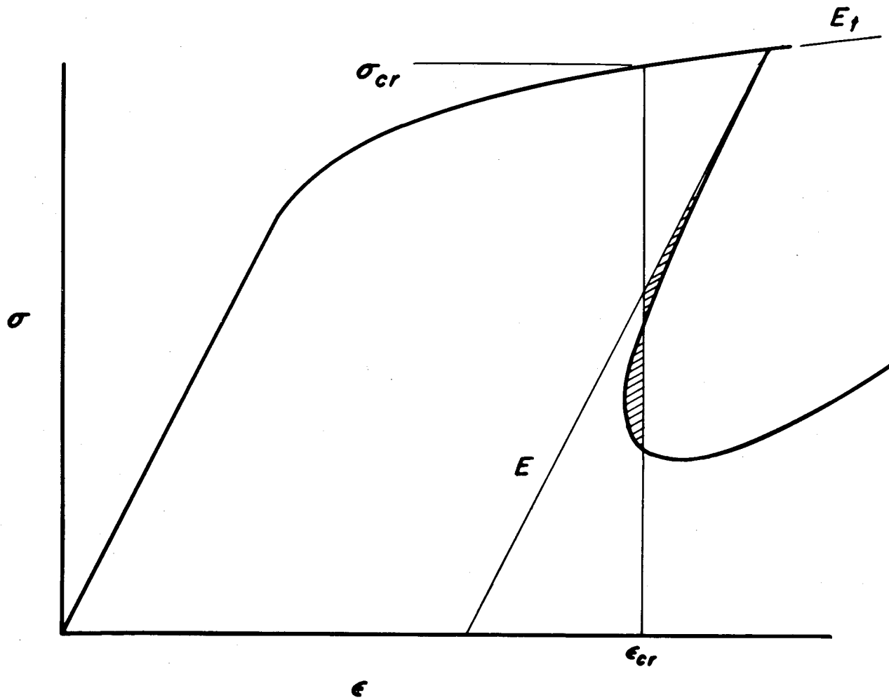
Figure 12.- Hypothetical buckling behavior of axially compressed circular cylinders in inelastic range.
