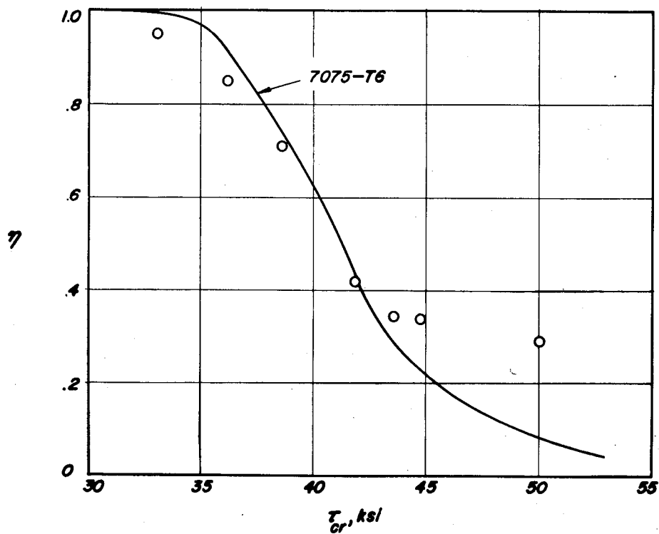
Figure 30.- Comparison of test data with theoretical plasticity-reduction factor for long cylinders in torsion.
