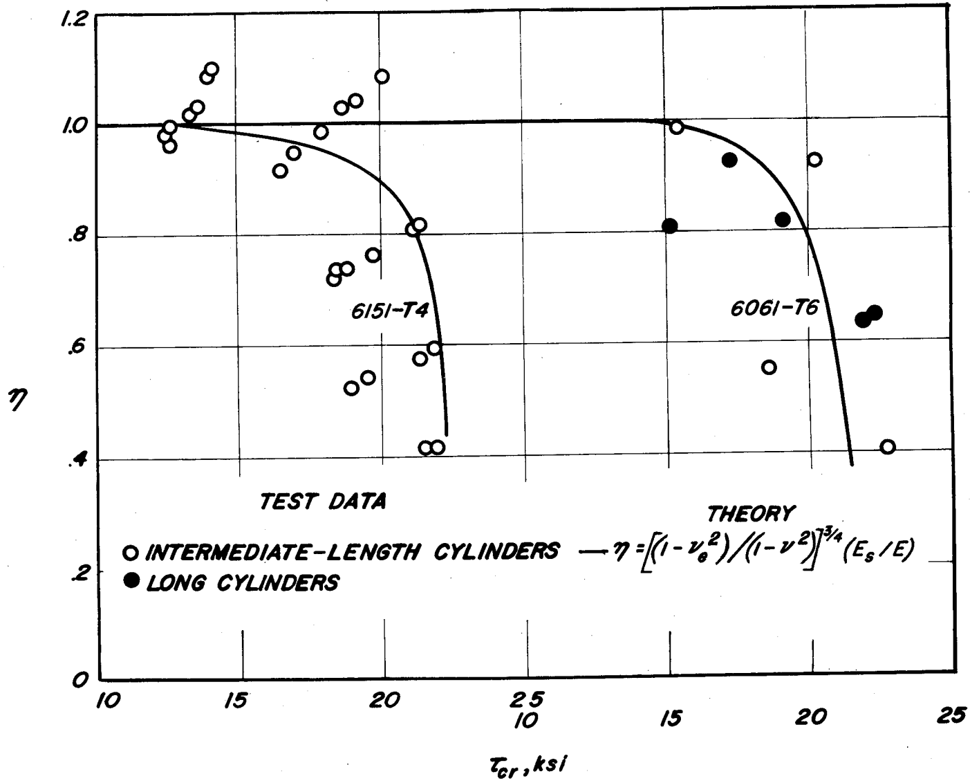
Figure 31.- Comparison of test data for intermediate-length cylinders with theory for long cylinders in torsion.
