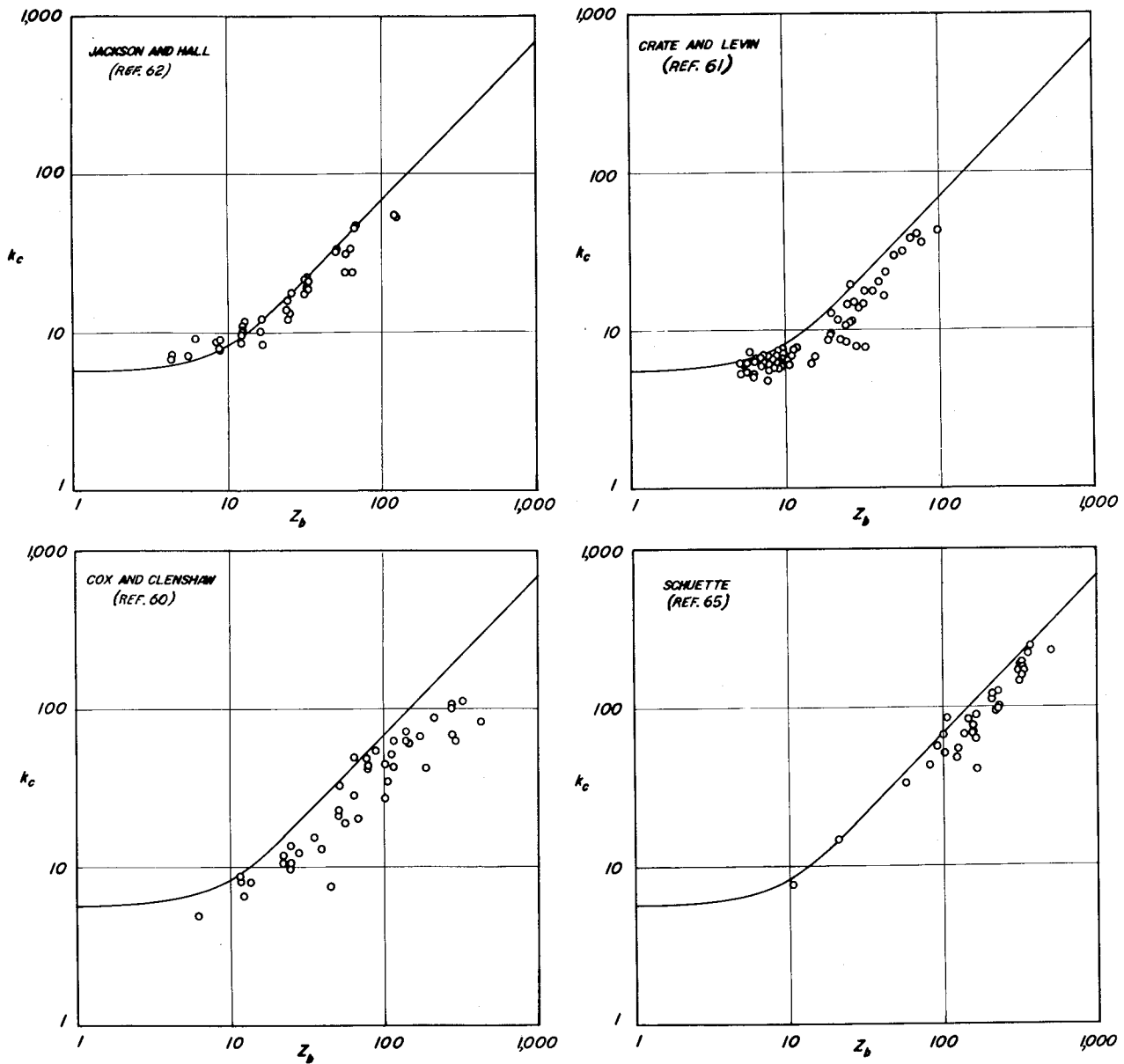
(a) Comparison of test data with linear theory.
