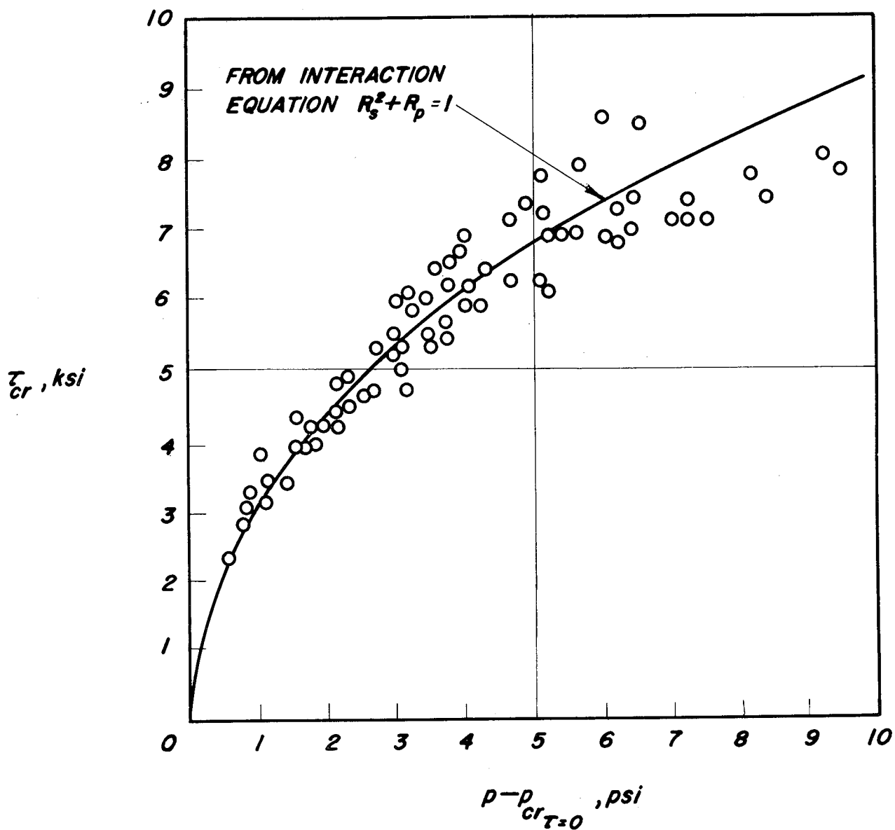
Figure 50.- Effect of internal pressure on buckling of curved plates in shear. Test data from Rafel and Sandlin (ref. 70).
