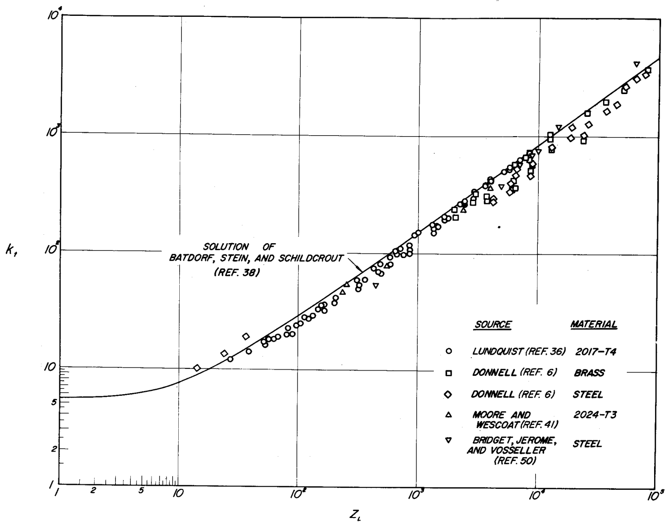
Figure 26.- Comparison of test data and theory for simply supported circular cylinders in torsion.
