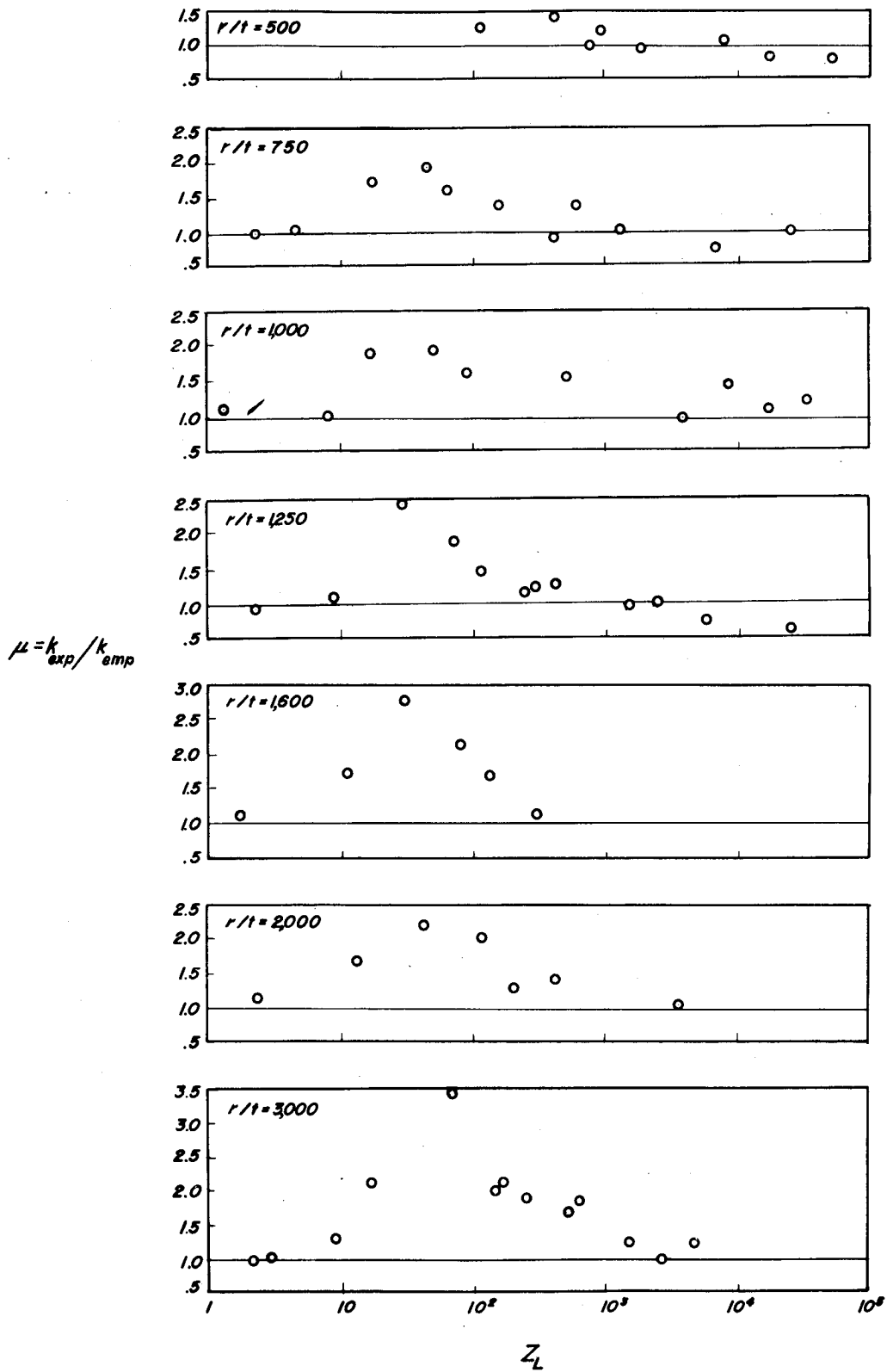
Figure 8.- Magnification factor for axially compressed cylinders derived from figure 6.
