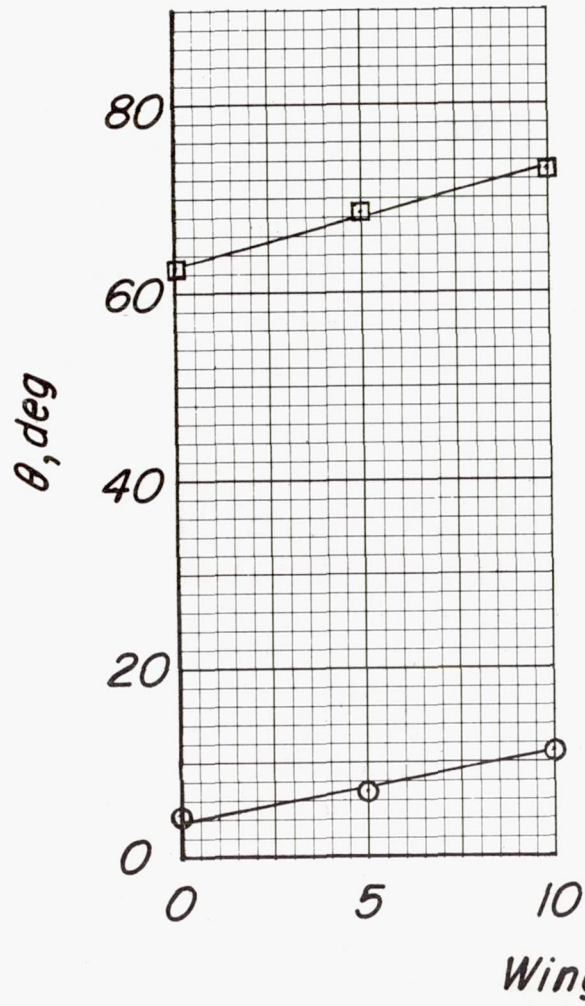
Figure 10.- Variation of turning effectiveness with wing incidence. Vane off.
