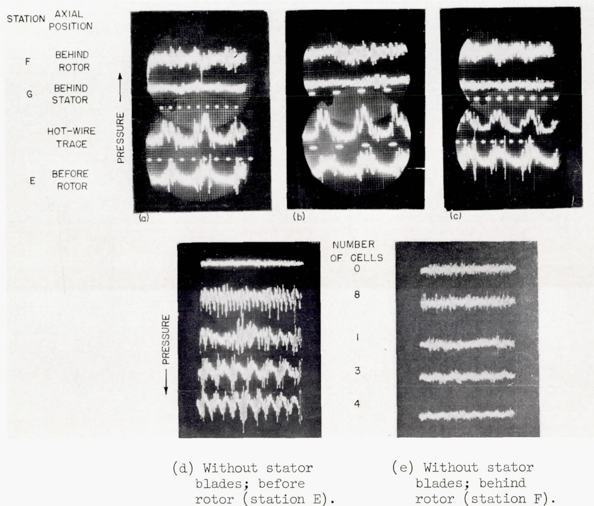
Figure 5.- Static pressure fluctuations. Hot-wire trace is added for comparison in parts (a) to (c).
