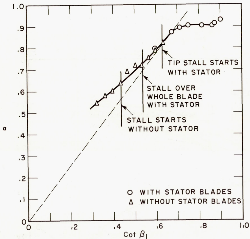
Figure 7.- Blockage coefficient \alpha against \cot \beta_1 .
