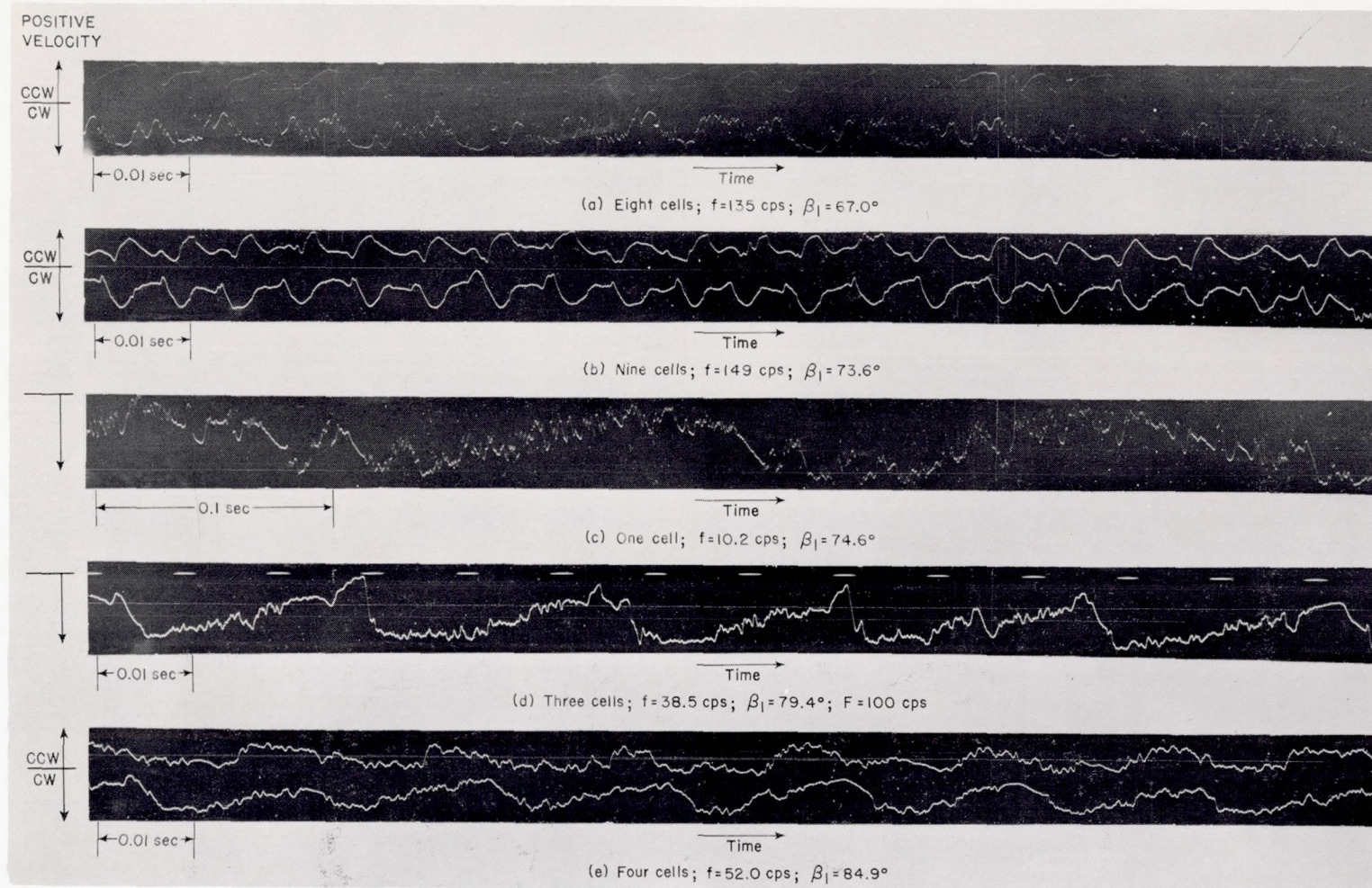
Figure 4.- Representative strip film records of hot-wire traces without stator blades. Probes are before rotor and 45^\circ apart; clockwise probe receives signal first. CW, clockwise probe; CCW, counterclockwise probe.
