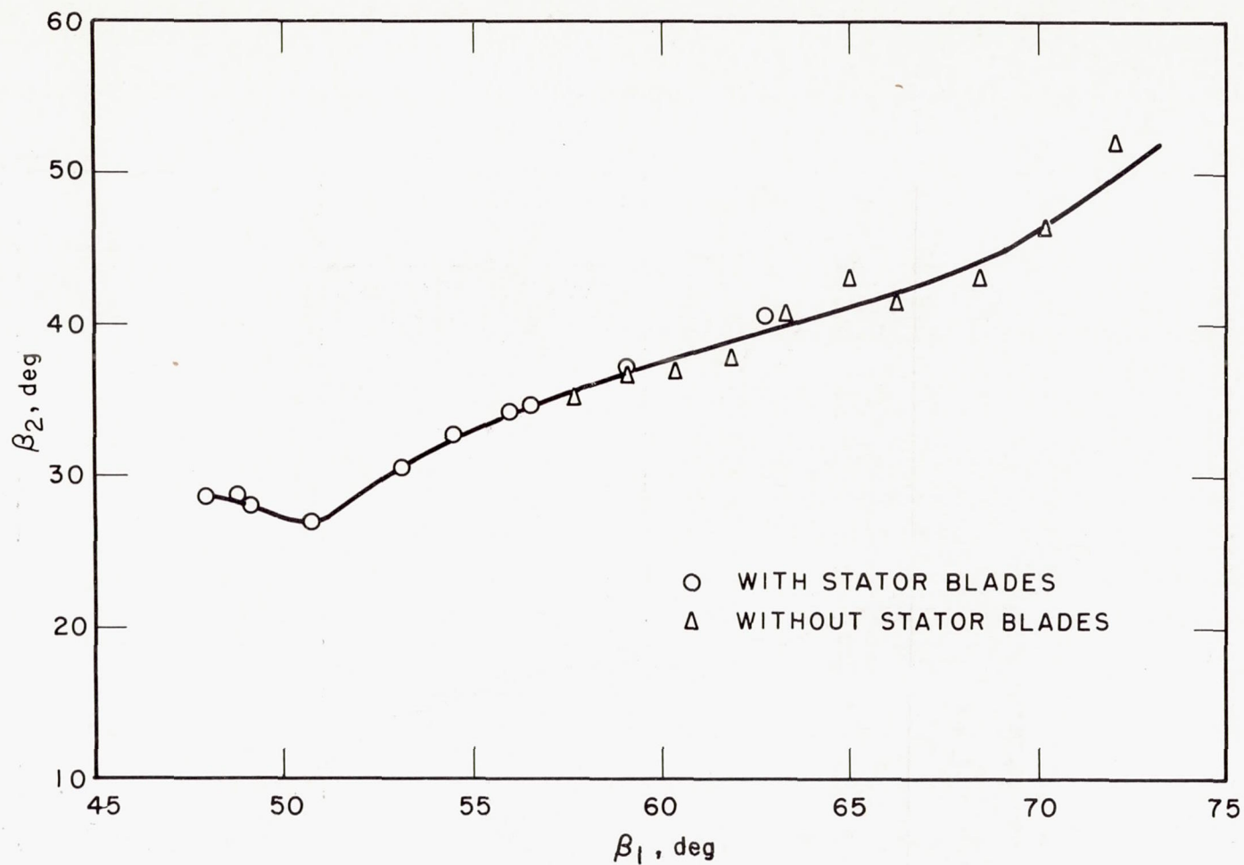
(a) \beta_2 against \beta_1 .
