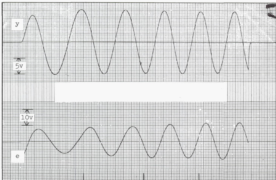
(d) Linear system; \Omega = \omega/\omega_v = 0.5 to 0.8 in 0.1 steps.
