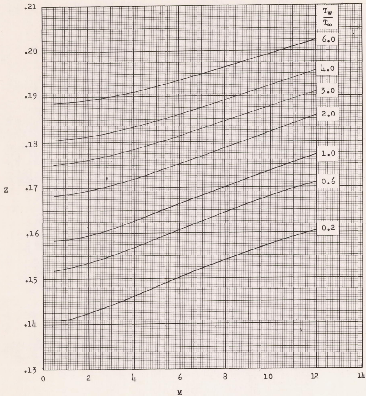
(a) Variation with Mach number for several temperature ratios.
