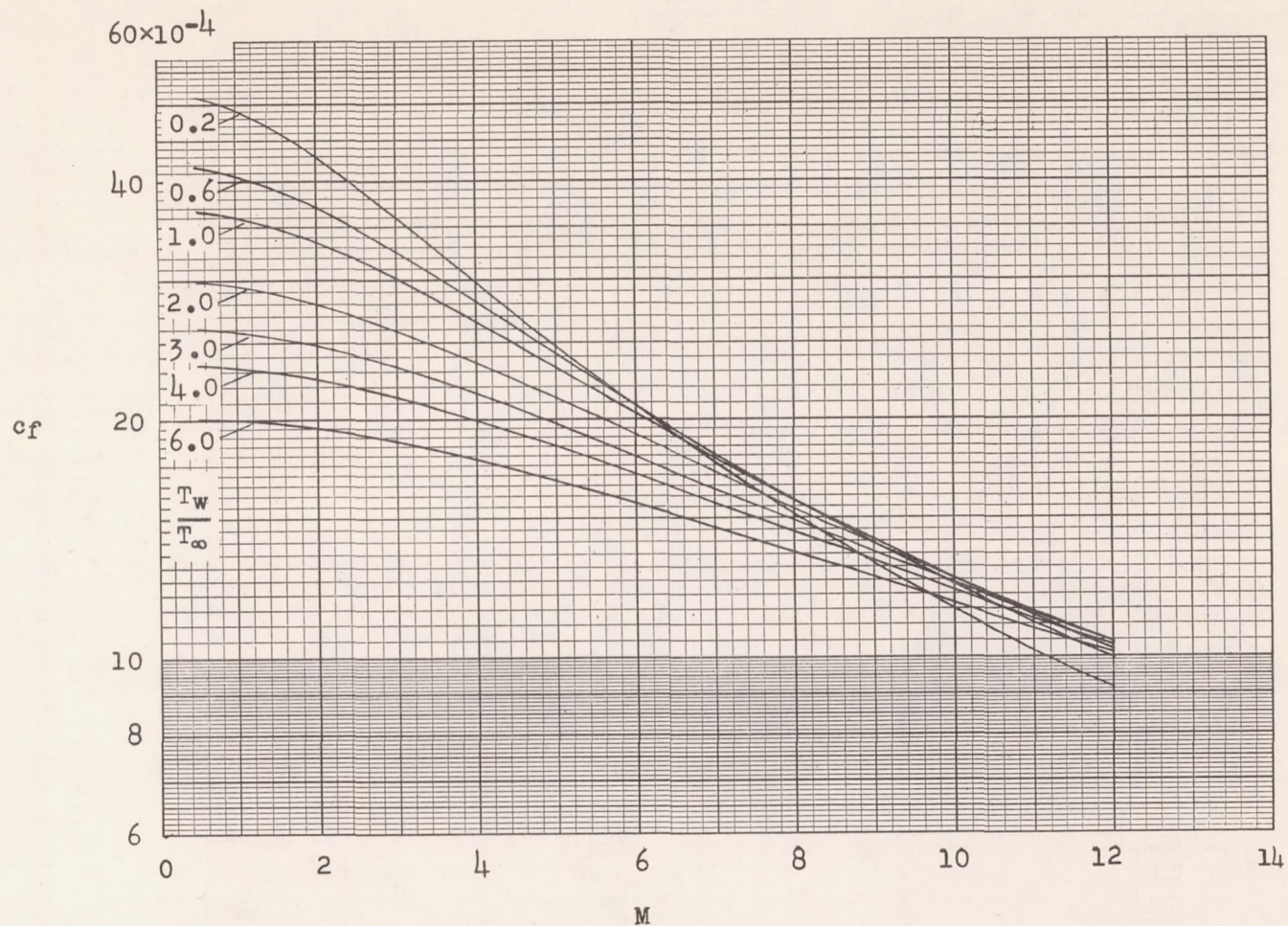
(a) Variation with Mach number for several temperature ratios.
