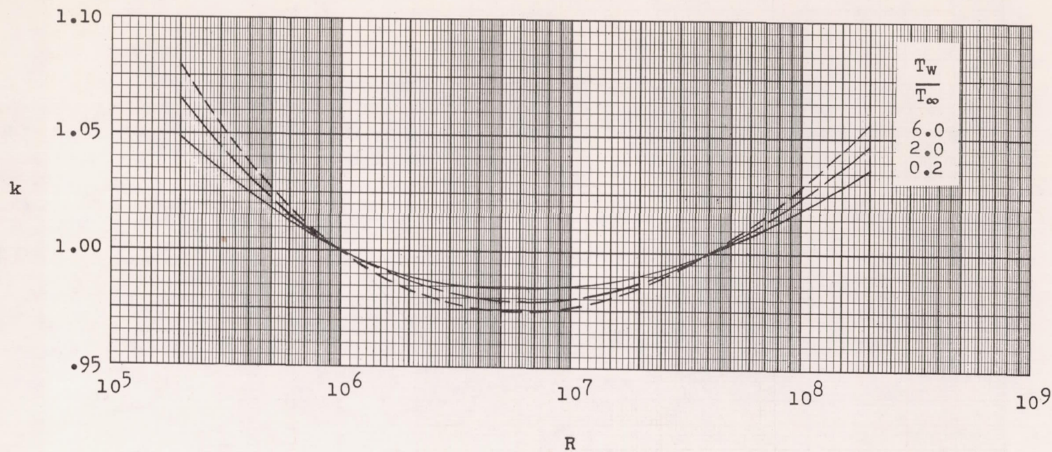
Figure 4.- Correction factor for all Mach numbers.
