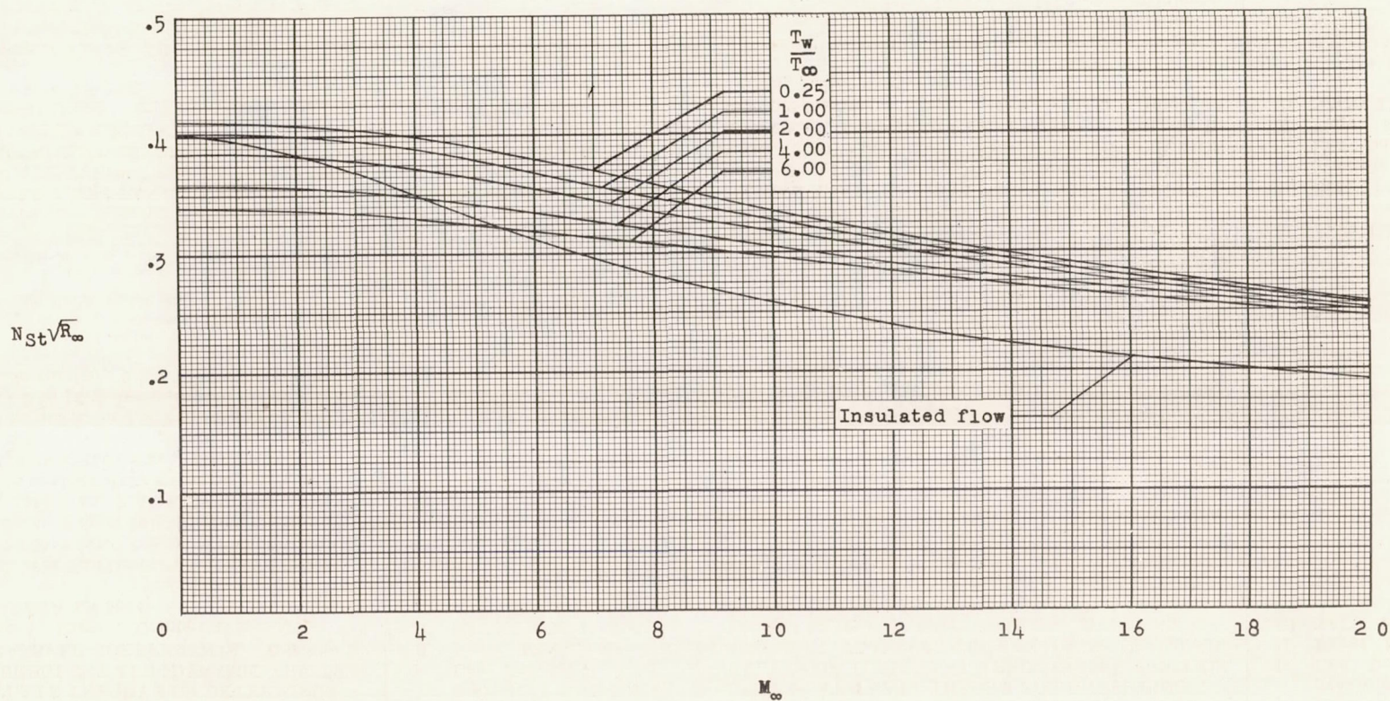
Figure 5.- Local heat-transfer coefficient for laminar boundary layer of a compressible fluid flowing along a flat plate.
