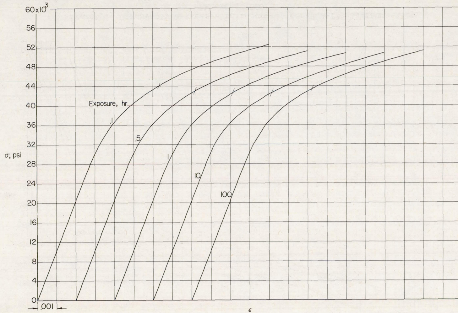
Figure 4.- Compressive stress-strain curves for 2024-T3 aluminum-alloy sheet at 250° F.
