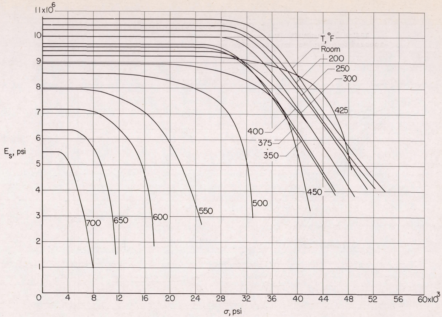
Figure 19.- Variation of secant modulus with stress for 2024-T3 aluminum-alloy sheet. 0.5-hour exposure.
