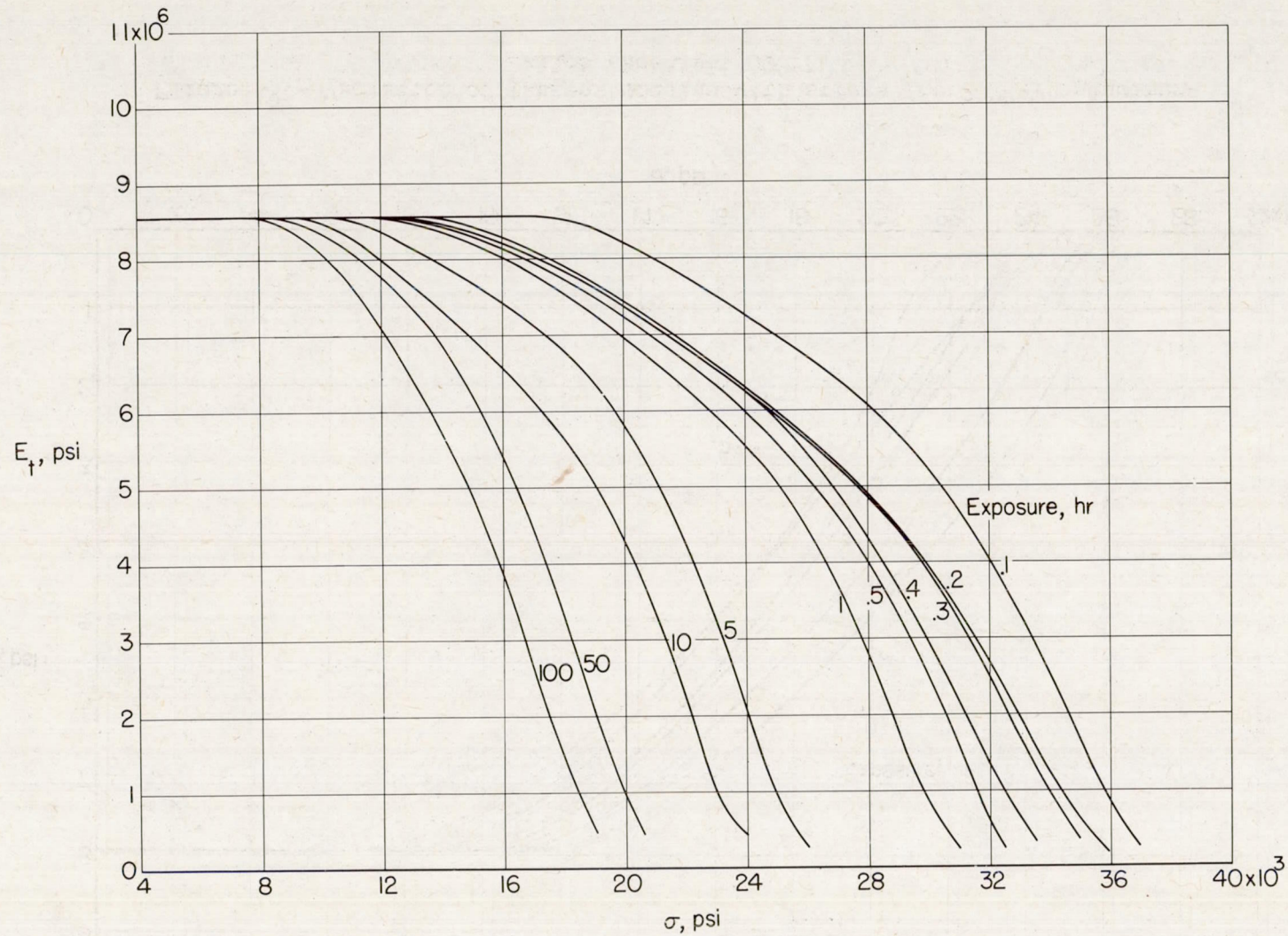
Figure 42.- Variation of tangent modulus with stress for 2024-T3 aluminum-alloy sheet at 500° F.
