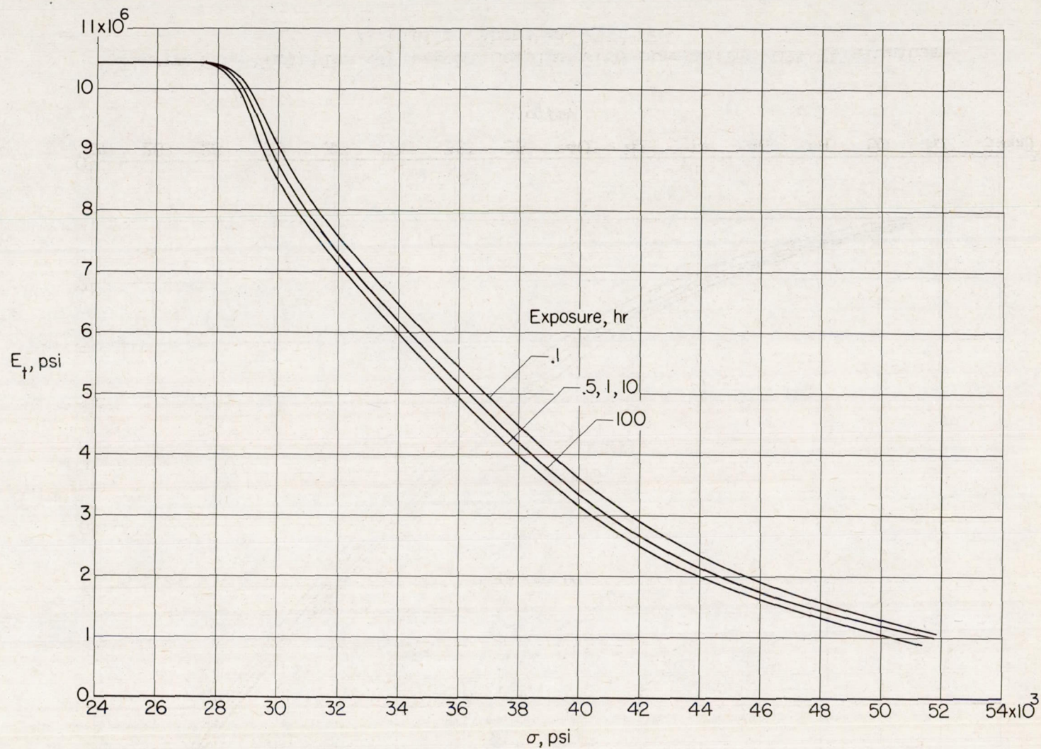
Figure 34.- Variation of tangent modulus with stress for 2024-T3 aluminum-alloy sheet at 200^\circ\text{F} .
