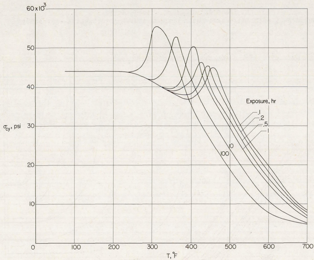
Figure 18.- Effect of temperature and exposure time on the 0.2-percent-offset compressive yield stress for 2024-T3 aluminum-alloy sheet (obtained by cross-plotting data in fig. 17).
