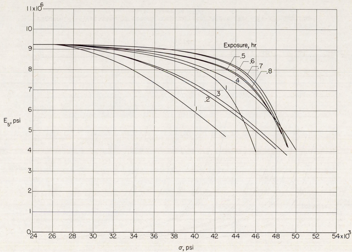
Figure 26.- Variation of secant modulus with stress for 2024-T3 aluminum-alloy sheet at 425^\circ\text{F} .
