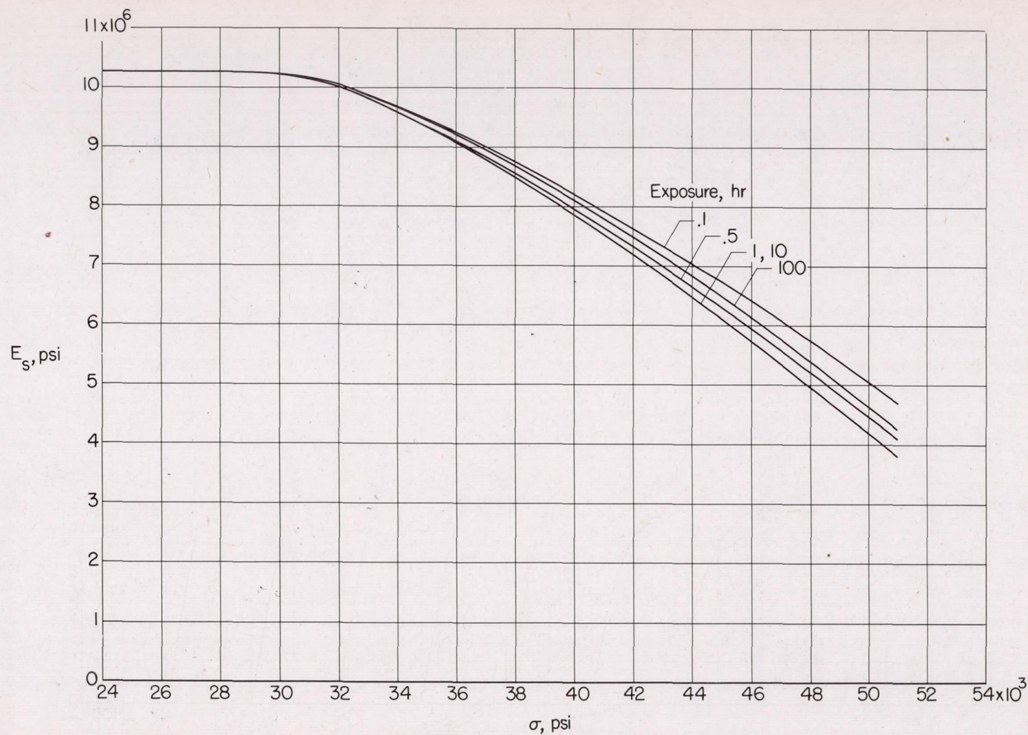
Figure 21.- Variation of secant modulus with stress for 2024-T3 aluminum-alloy sheet at 250^\circ\text{F} .
