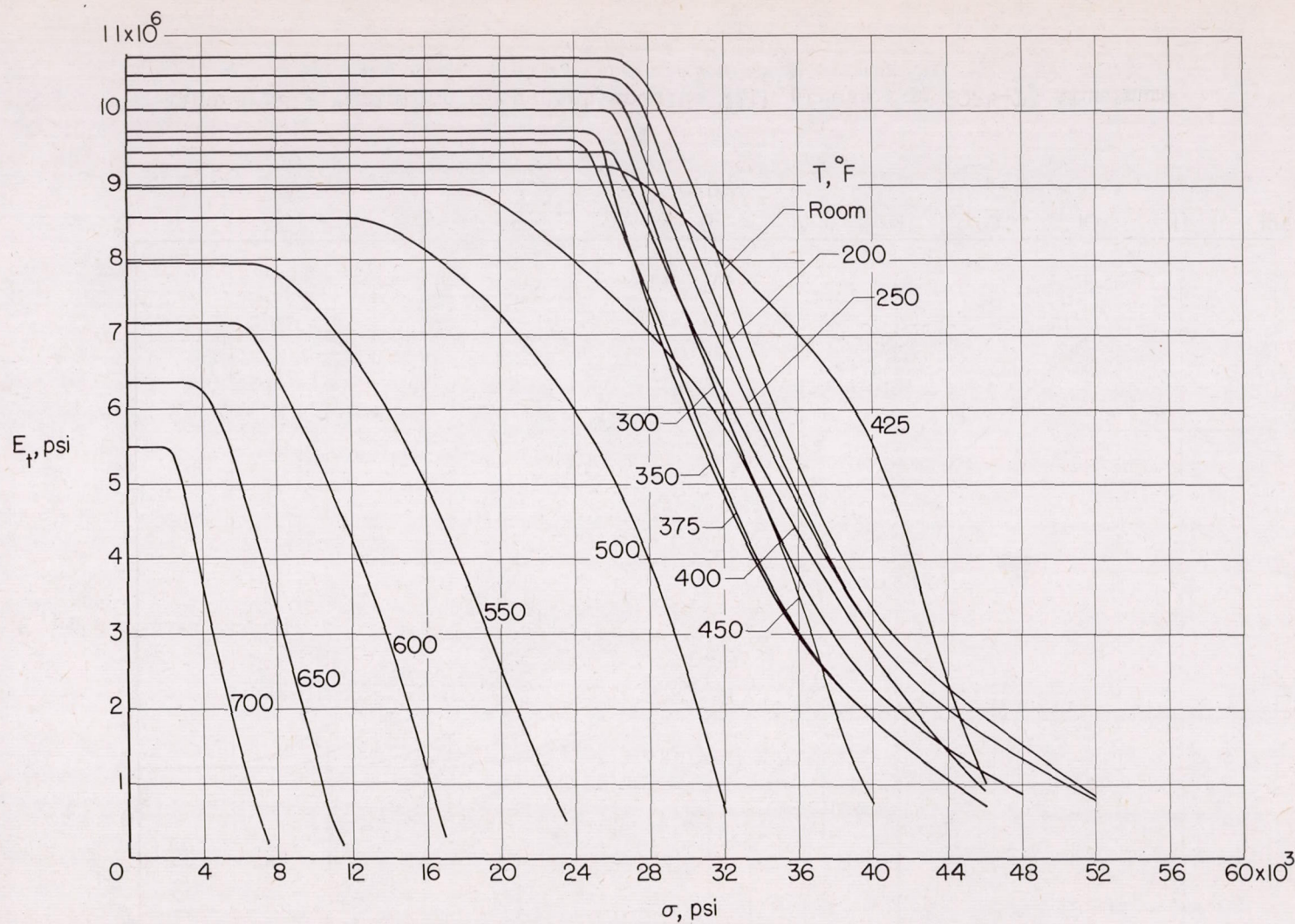
Figure 33.- Variation of tangent modulus with stress for 2024-T3 aluminum-alloy sheet. 0.5-hour exposure.
