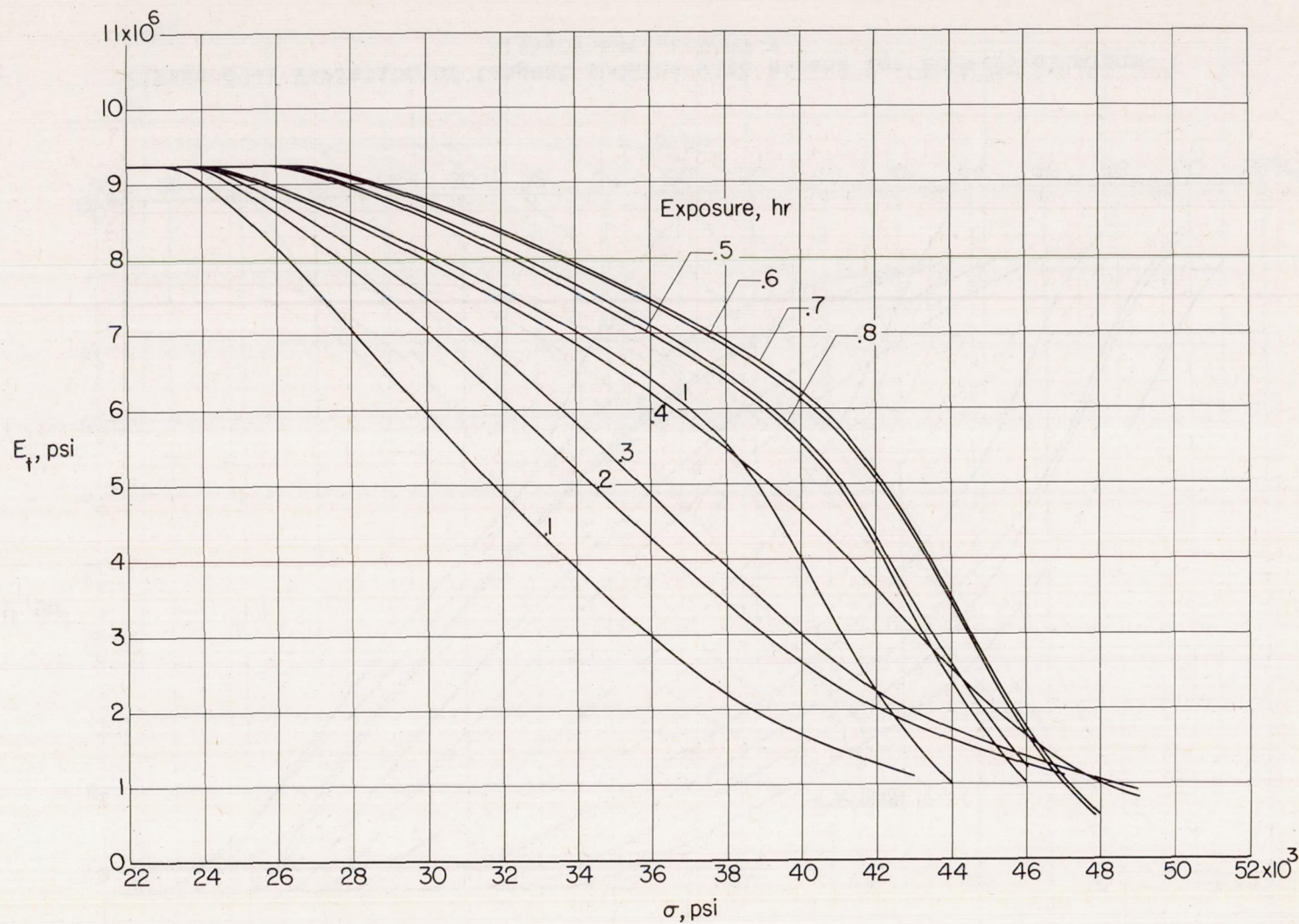
Figure 40.- Variation of tangent modulus with stress for 2024-T3 aluminum-alloy sheet at 425° F.
