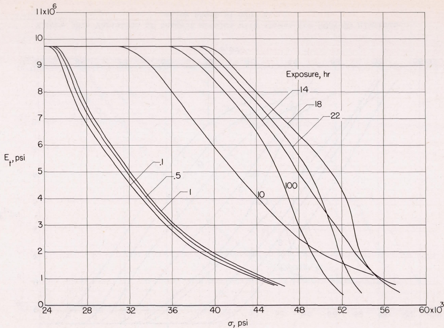
Figure 37.- Variation of tangent modulus with stress for 2024-T3 aluminum-alloy sheet at 350° F.
