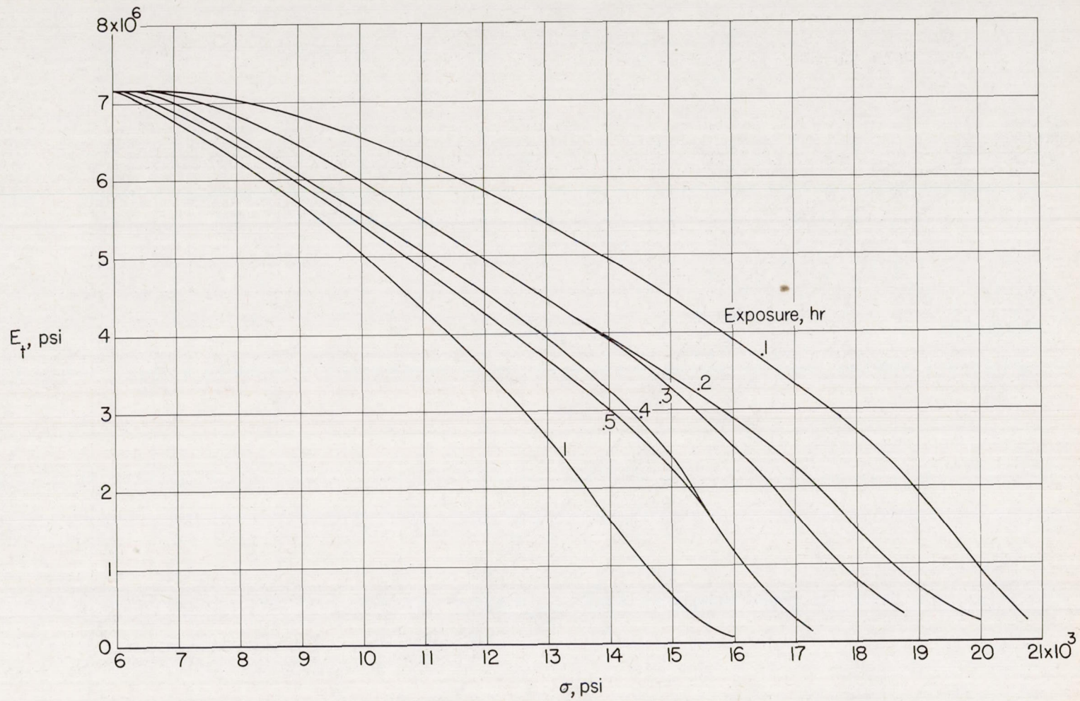
Figure 44.- Variation of tangent modulus with stress for 2024-T3 aluminum-alloy sheet at 600^\circ\text{F} .
