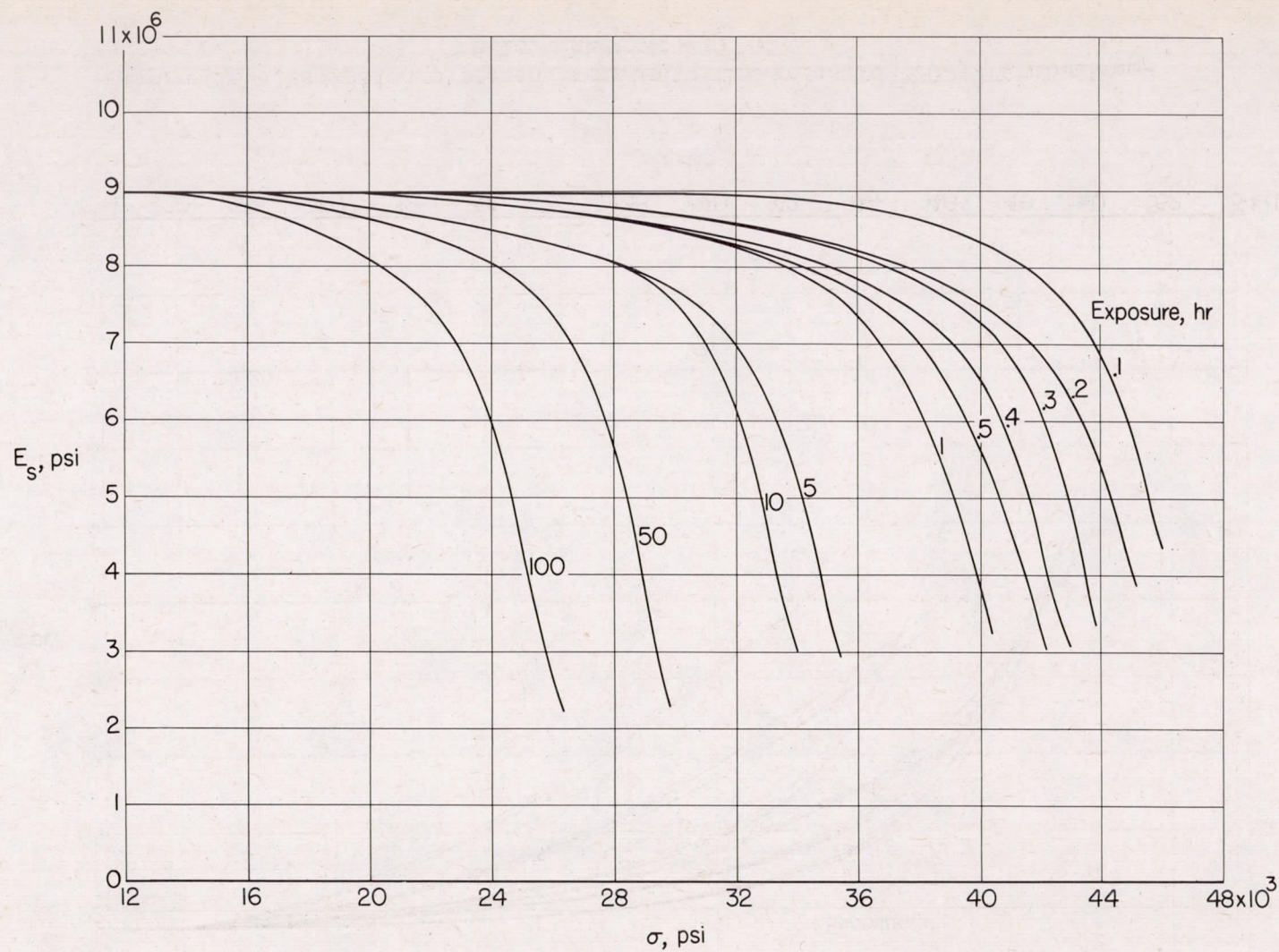
Figure 27.- Variation of secant modulus with stress for 2024-T3 aluminum-alloy sheet at 450° F.
