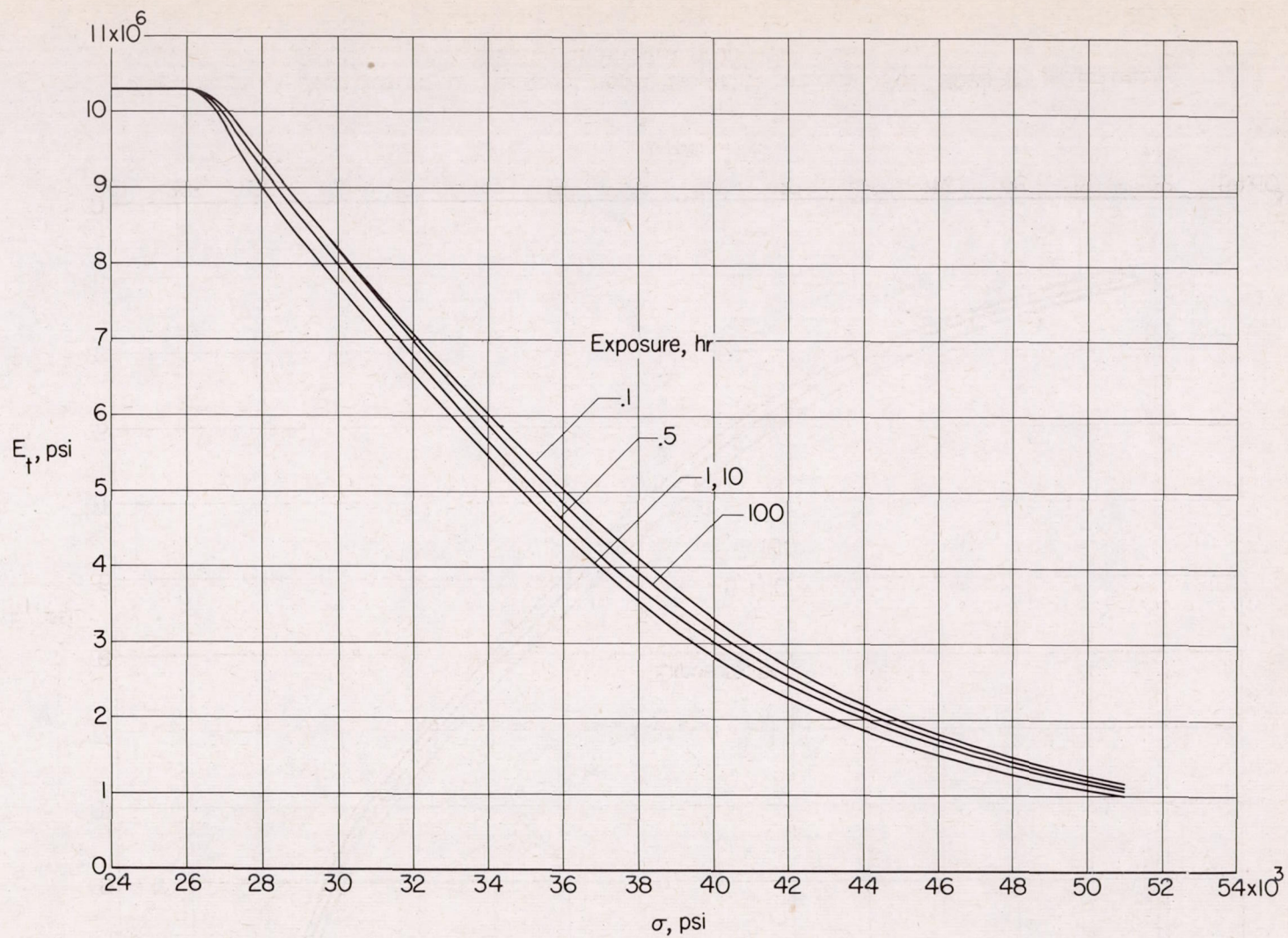
Figure 35.- Variation of tangent modulus with stress for 2024-T3 aluminum-alloy sheet at 250° F.
