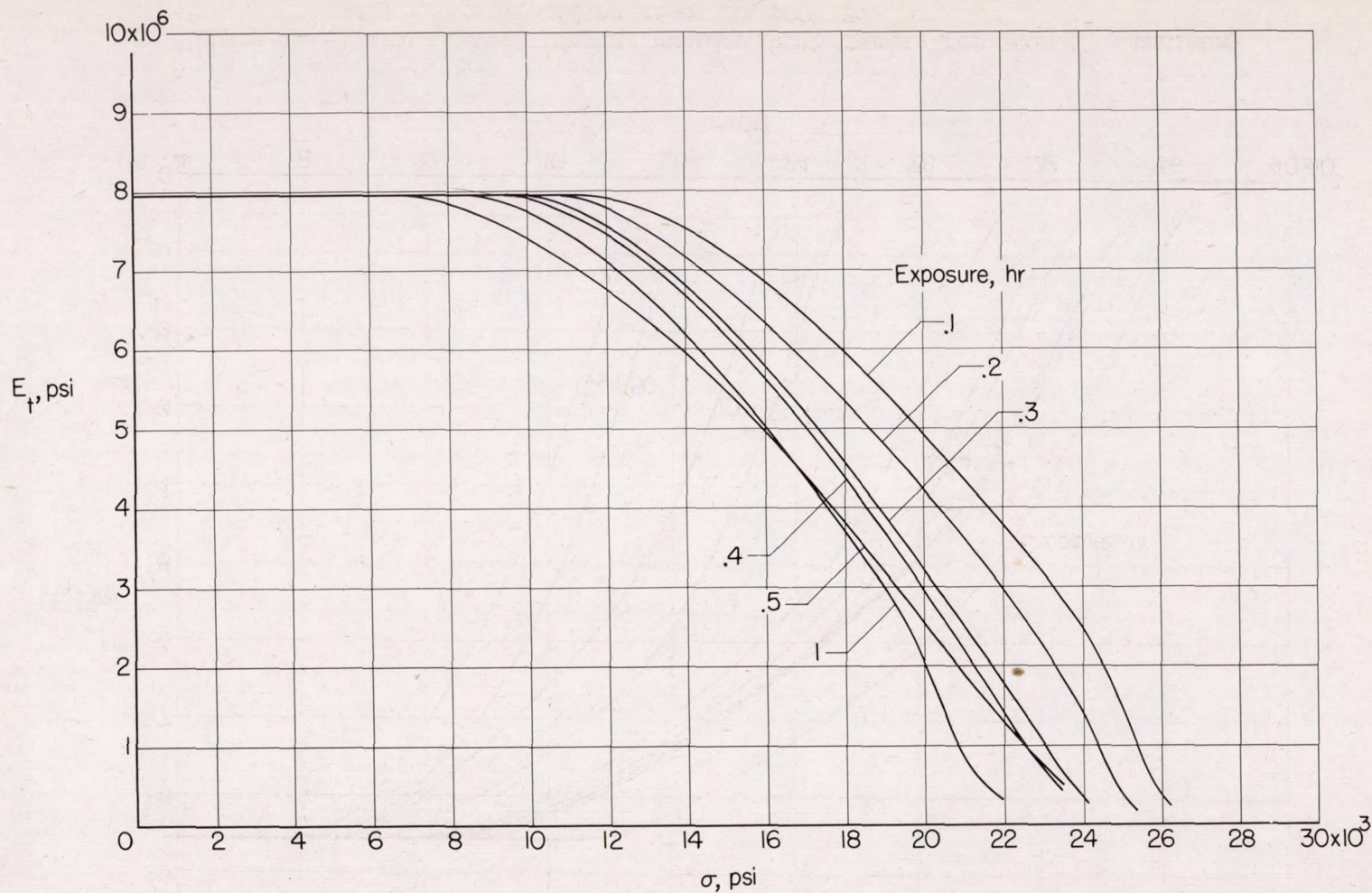
Figure 43.- Variation of tangent modulus with stress for 2024-T3 aluminum-alloy sheet at 550°F.
