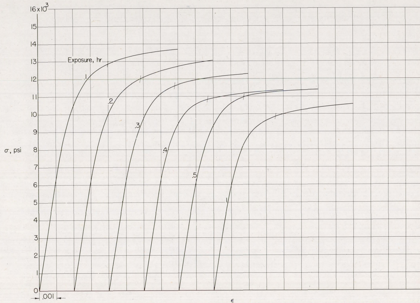
Figure 14.- Compressive stress-strain curves for 2024-T3 aluminum-alloy sheet at 650° F.
