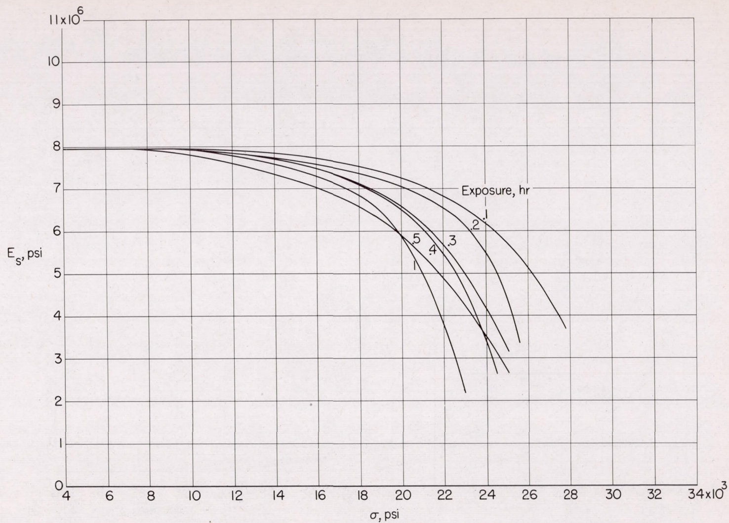
Figure 29.- Variation of secant modulus with stress for 2024-T3 aluminum-alloy sheet at 550° F.
