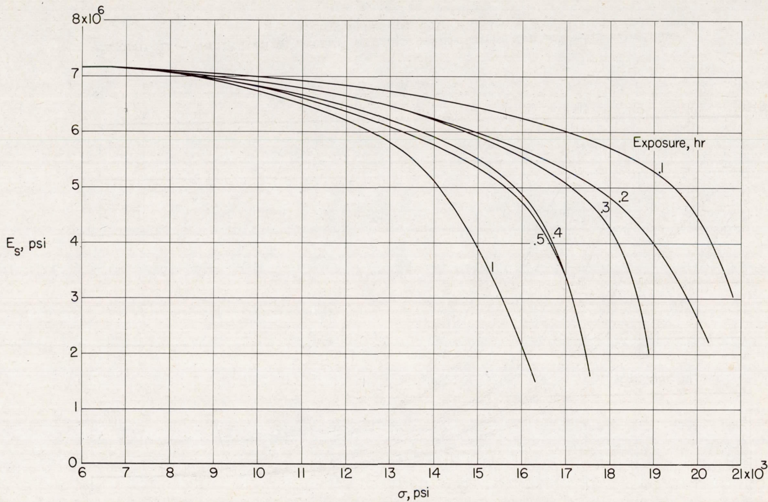
Figure 30.- Variation of secant modulus with stress for 2024-T3 aluminum-alloy sheet at 600^\circ\text{F} .
