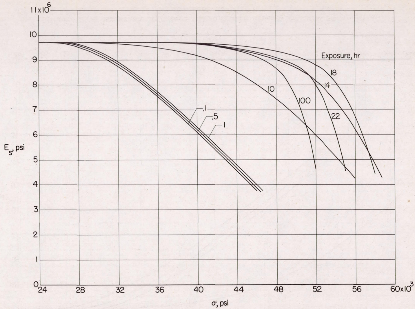
Figure 23.- Variation of secant modulus with stress for 2024-T3 aluminum-alloy sheet at 350° F.
