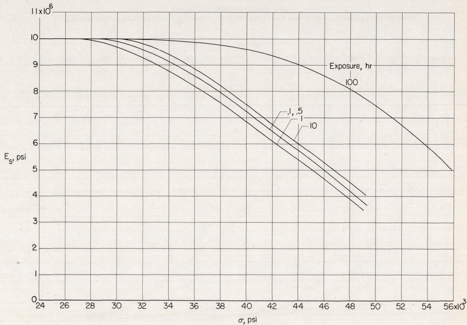
Figure 22.- Variation of secant modulus with stress for 2024-T3 aluminum-alloy sheet at 300° F.
