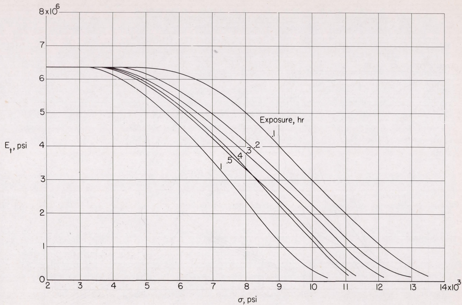
Figure 45.- Variation of tangent modulus with stress for 2024-T3 aluminum-alloy sheet at 650° F.
