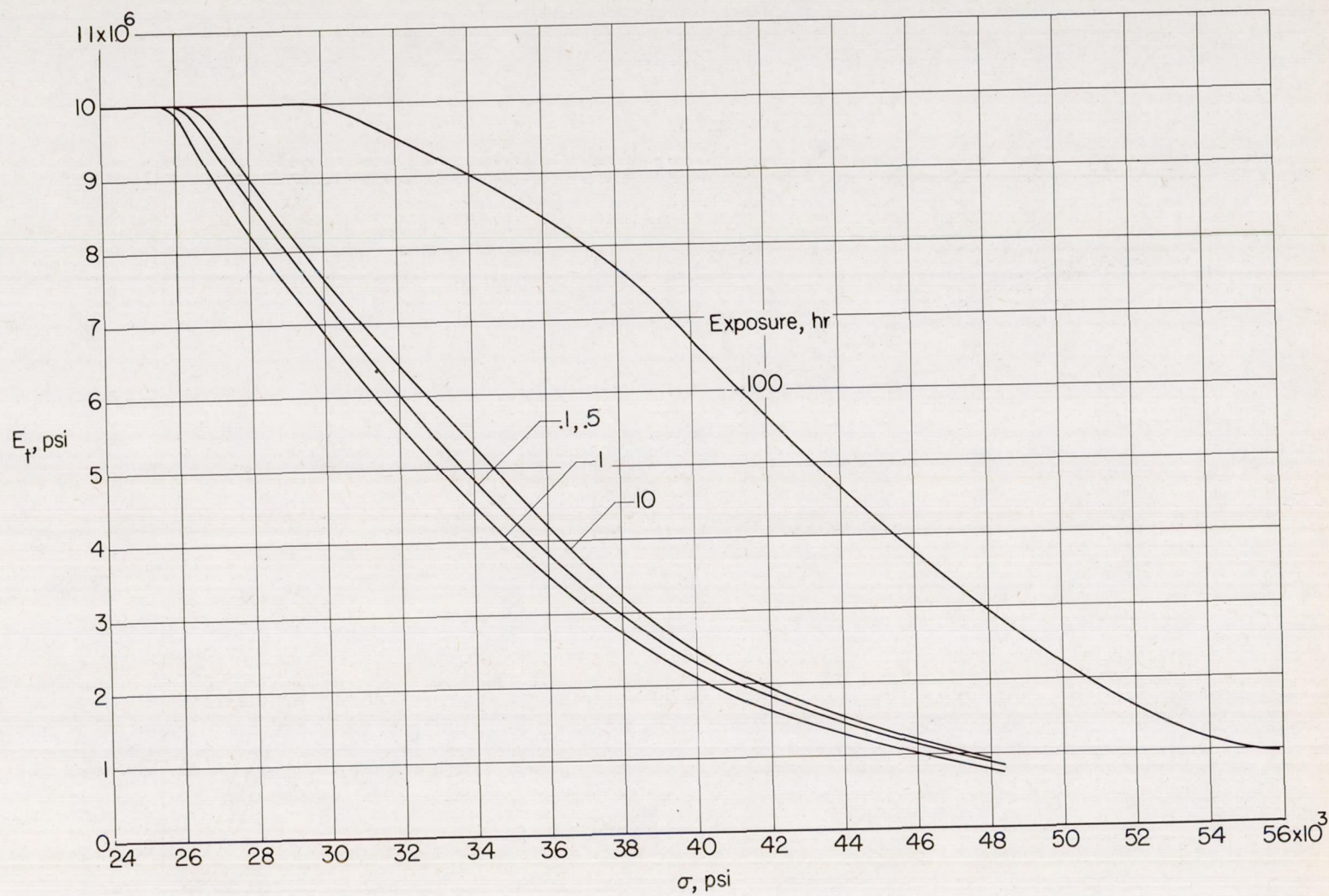
Figure 36.- Variation of tangent modulus with stress for 2024-T3 aluminum-alloy sheet at 300° F.
