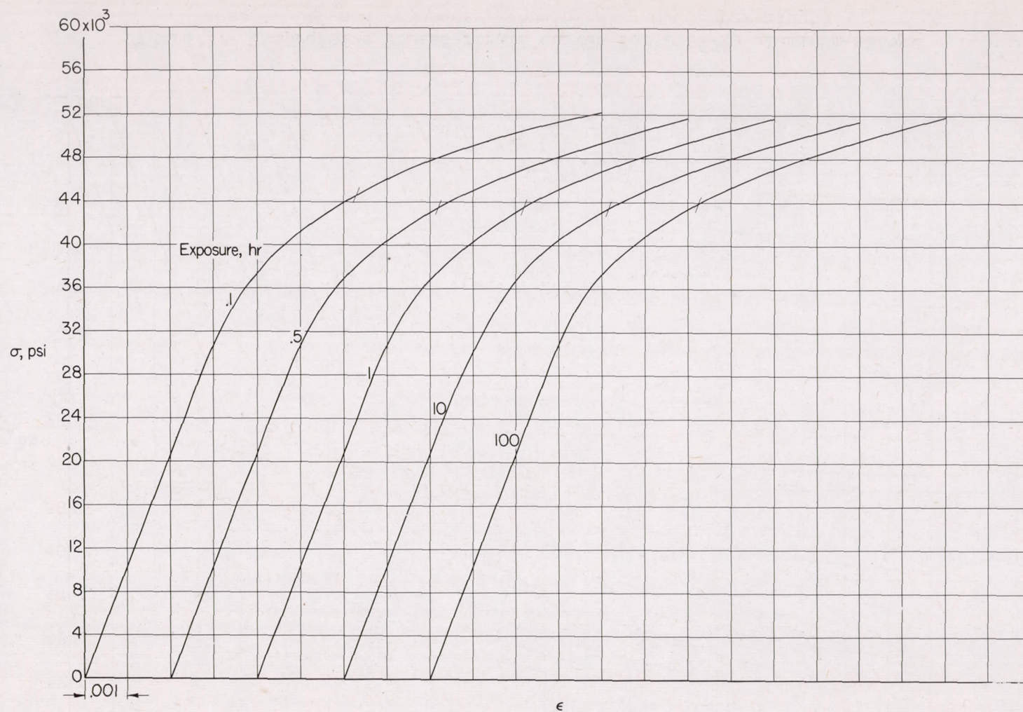
Figure 3.- Compressive stress-strain curves for 2024-T3 aluminum-alloy sheet at 200° F.
