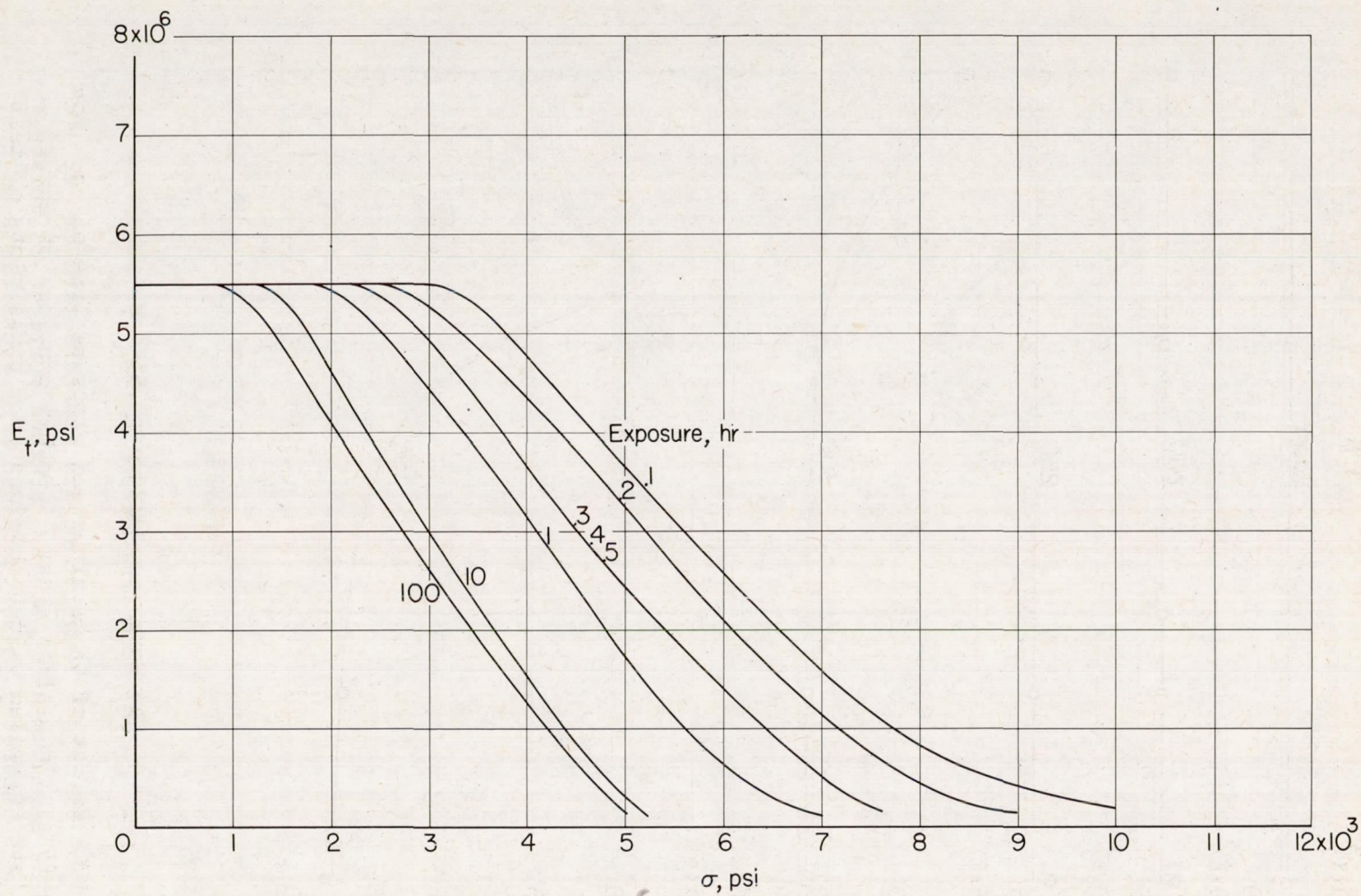
Figure 46.- Variation of tangent modulus with stress for 2024-T3 aluminum-alloy sheet at 700° F.
