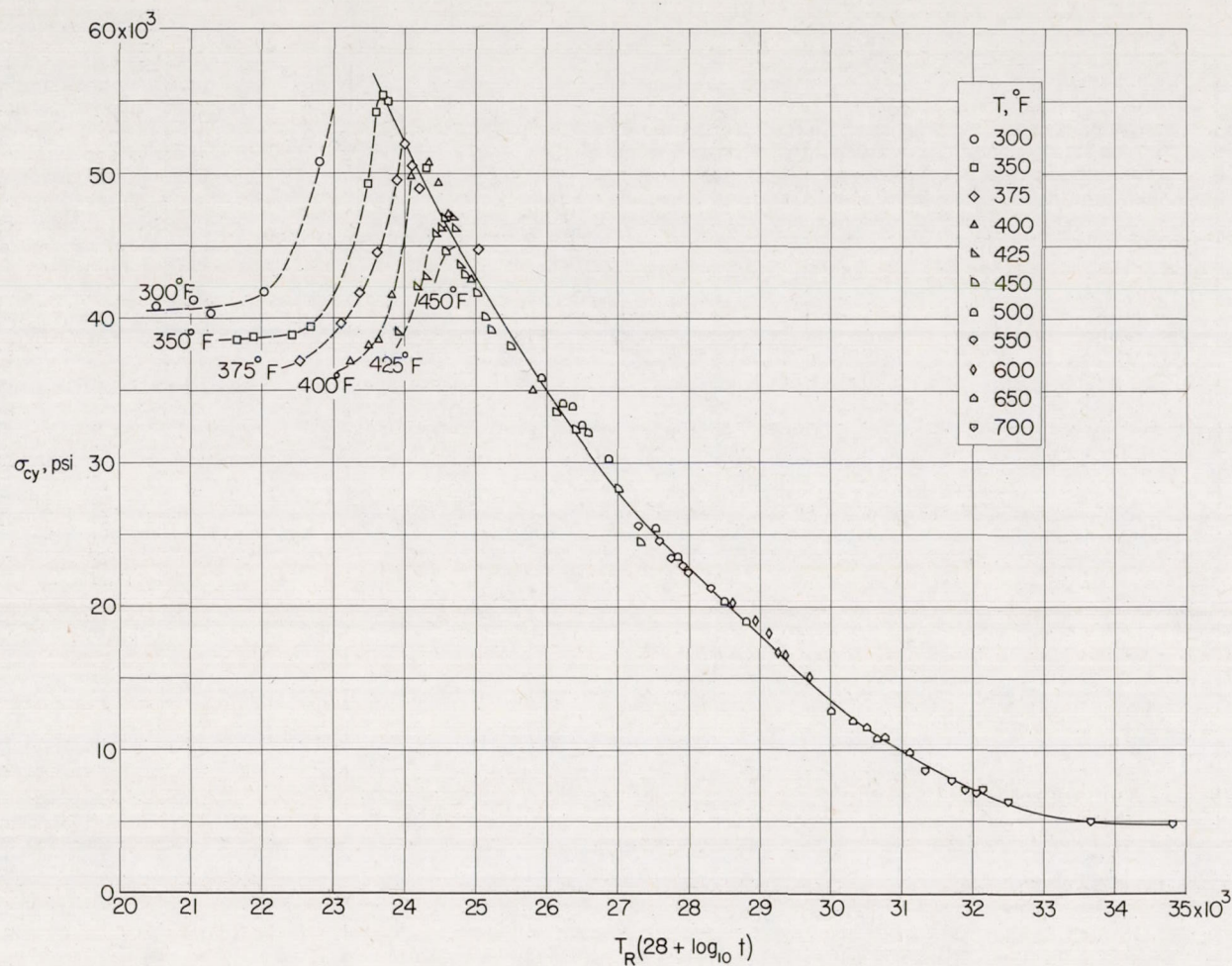
Figure 50.- Master curve of 0.2-percent-offset compressive yield stress for 2024-T3 aluminum-alloy sheet. (Dashed curves indicate time-temperature combinations which do not produce either maximum compressive yield stress or overaging of the material.)
