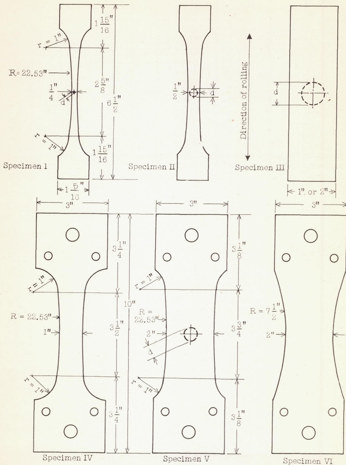
Figure 3.- Fatigue specimens.
