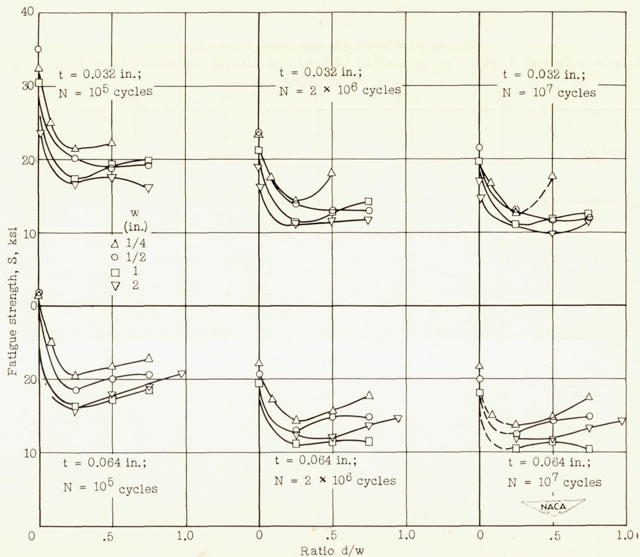
Figure 8.- Fatigue strength for failure at specific values of N . 24S-T sheet.
