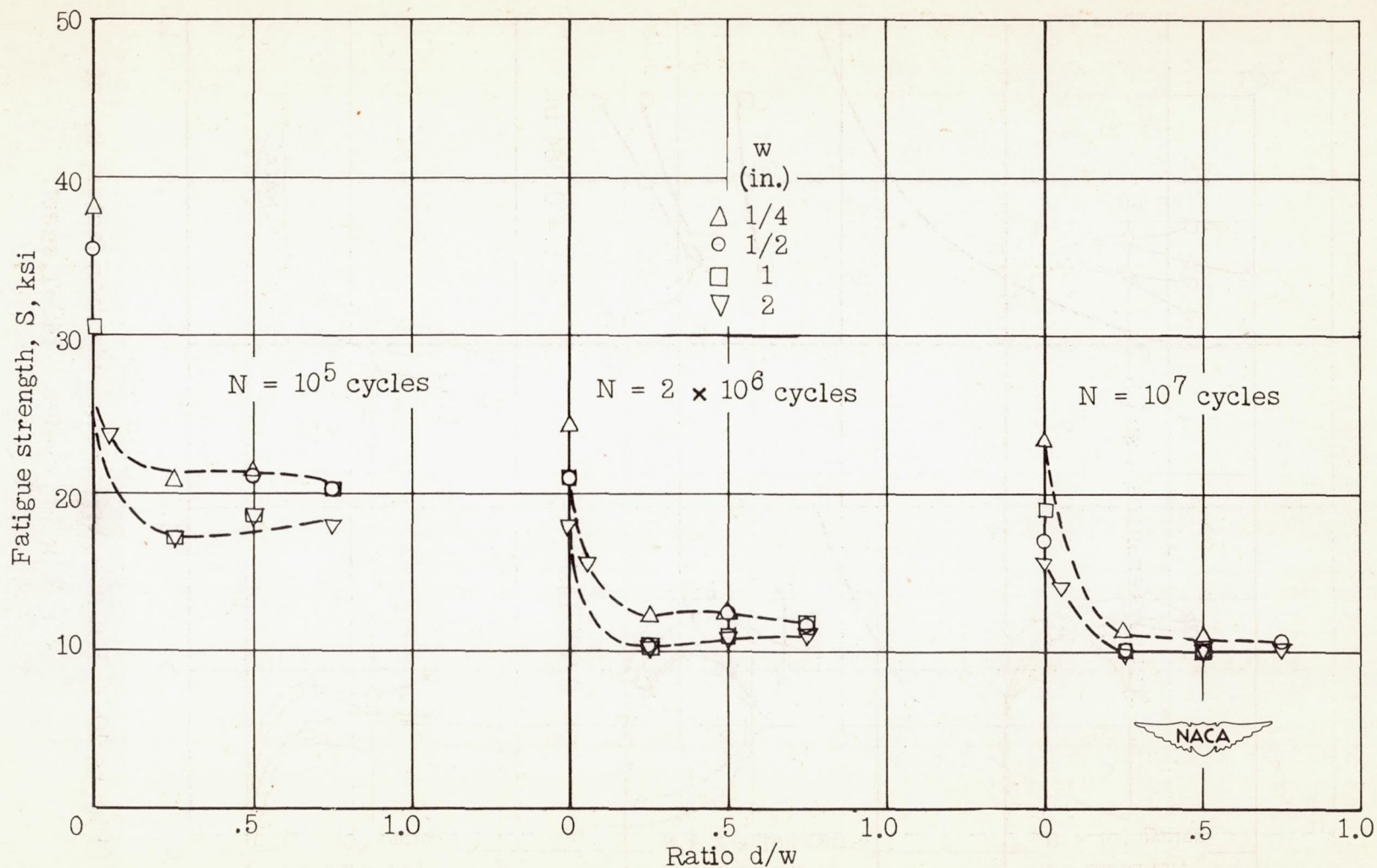
Figure 9.- Fatigue strength for failure at specific values of N . 75S-T sheet; t = 0.032 in. Scatter band for all widths is shown.
