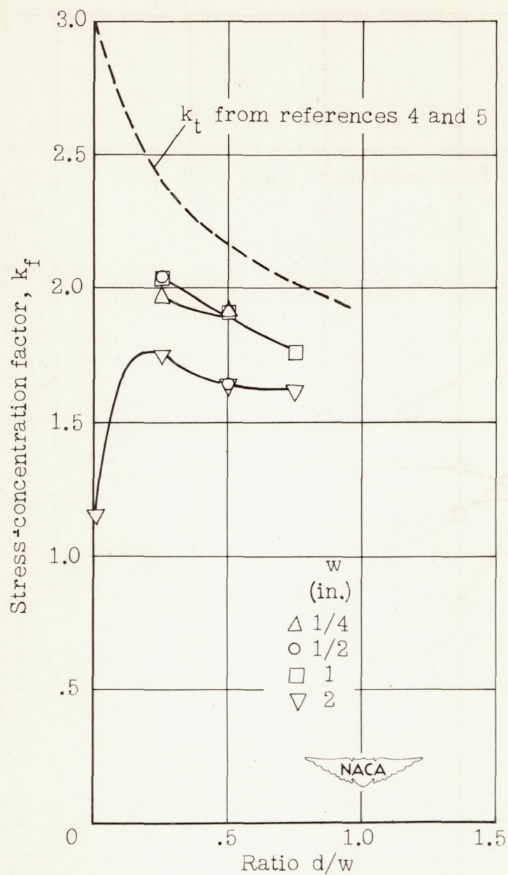
Figure 11.- Fatigue stress-concentration factor k_f at N = 2 \times 10^6 cycles. 75S-T sheet; t = 0.032 in.
