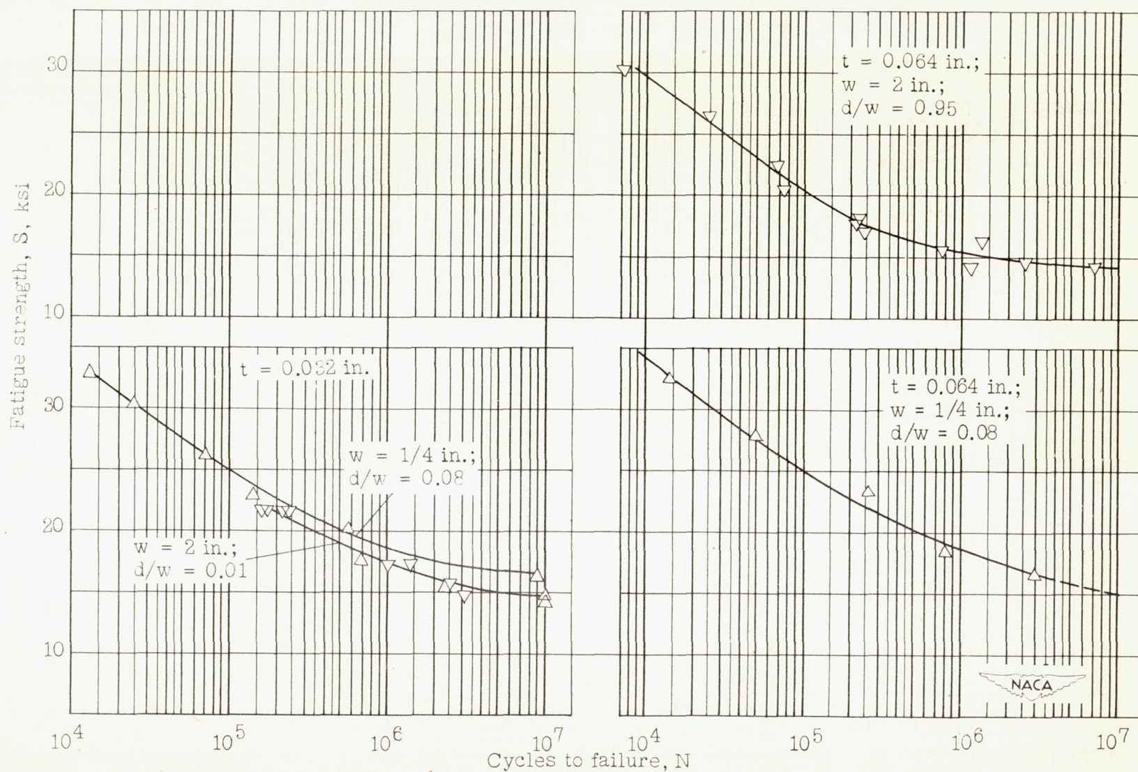
Figure 6.- S-N curves. 24S-T sheet. Specimens having ratio d/w = 0.08 and 0.95 .
