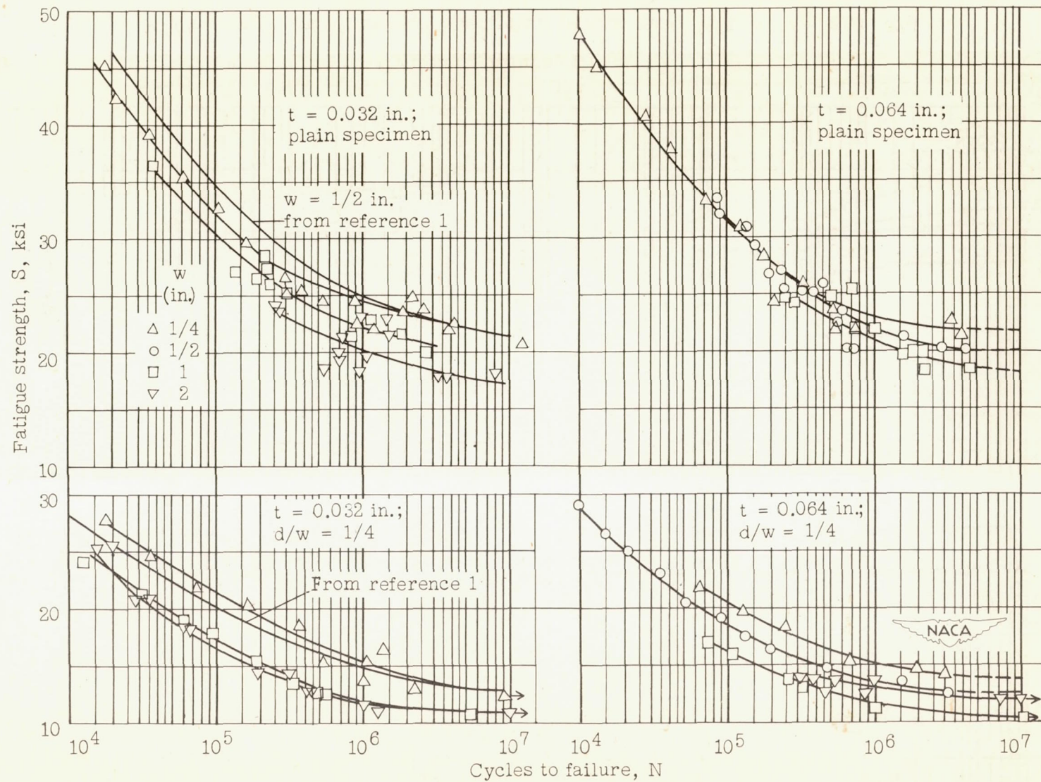
Figure 4.- S-N curves. 24S-T sheet. Plain specimens and specimens having ratio d/w = 1/4 .
