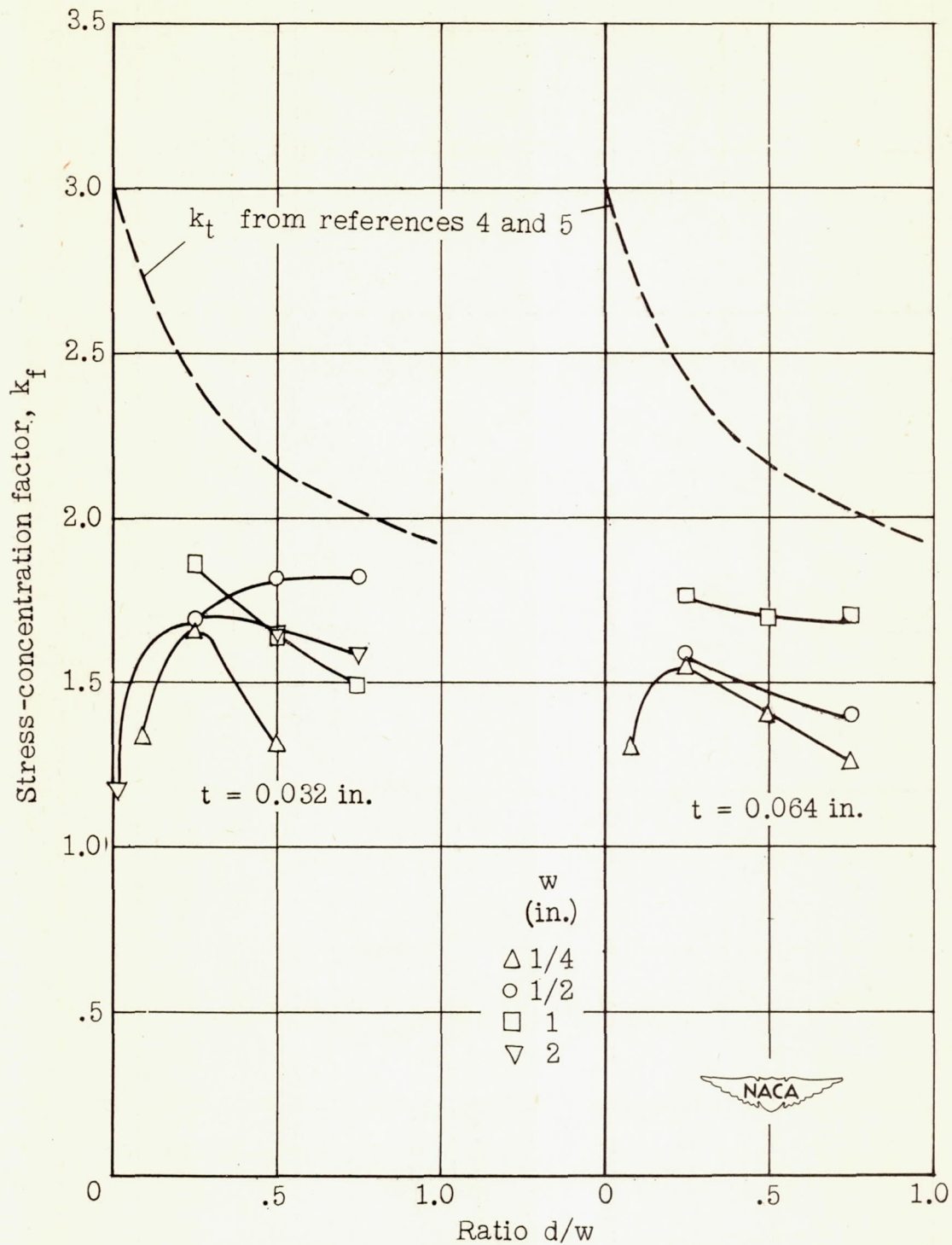
Figure 10.- Fatigue stress-concentration factor k_f at N = 2 \times 10^6 cycles. 24S-T sheet.
