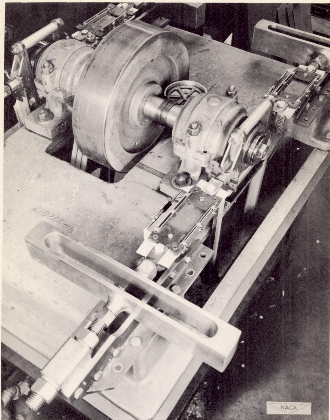
Figure 2.- Fatigue testing machine b.
