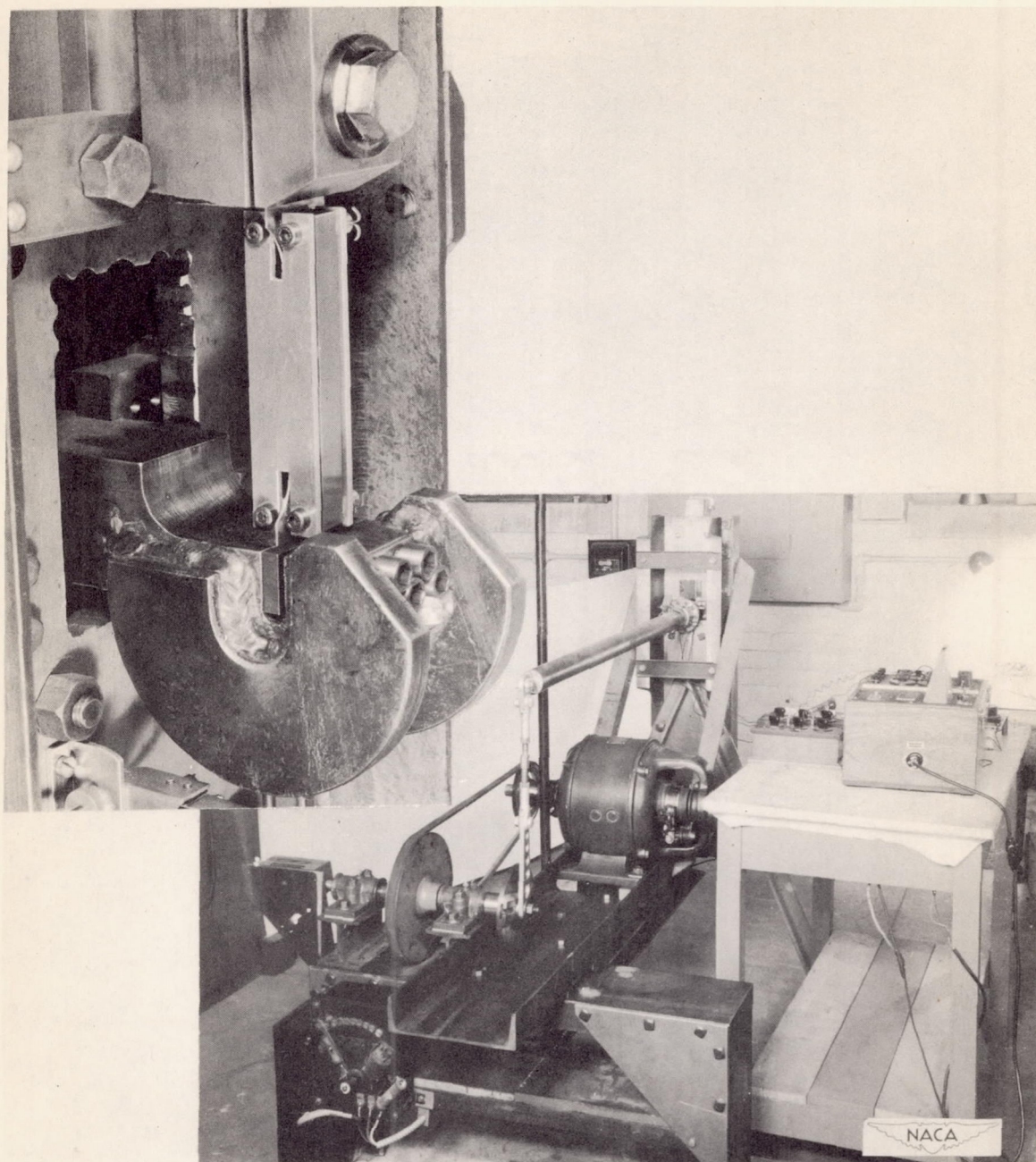
Figure 1.- Fatigue testing machine a.
