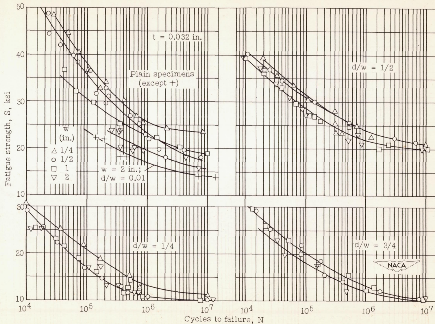
Figure 7.- S-N curves. 75S-T sheet.
