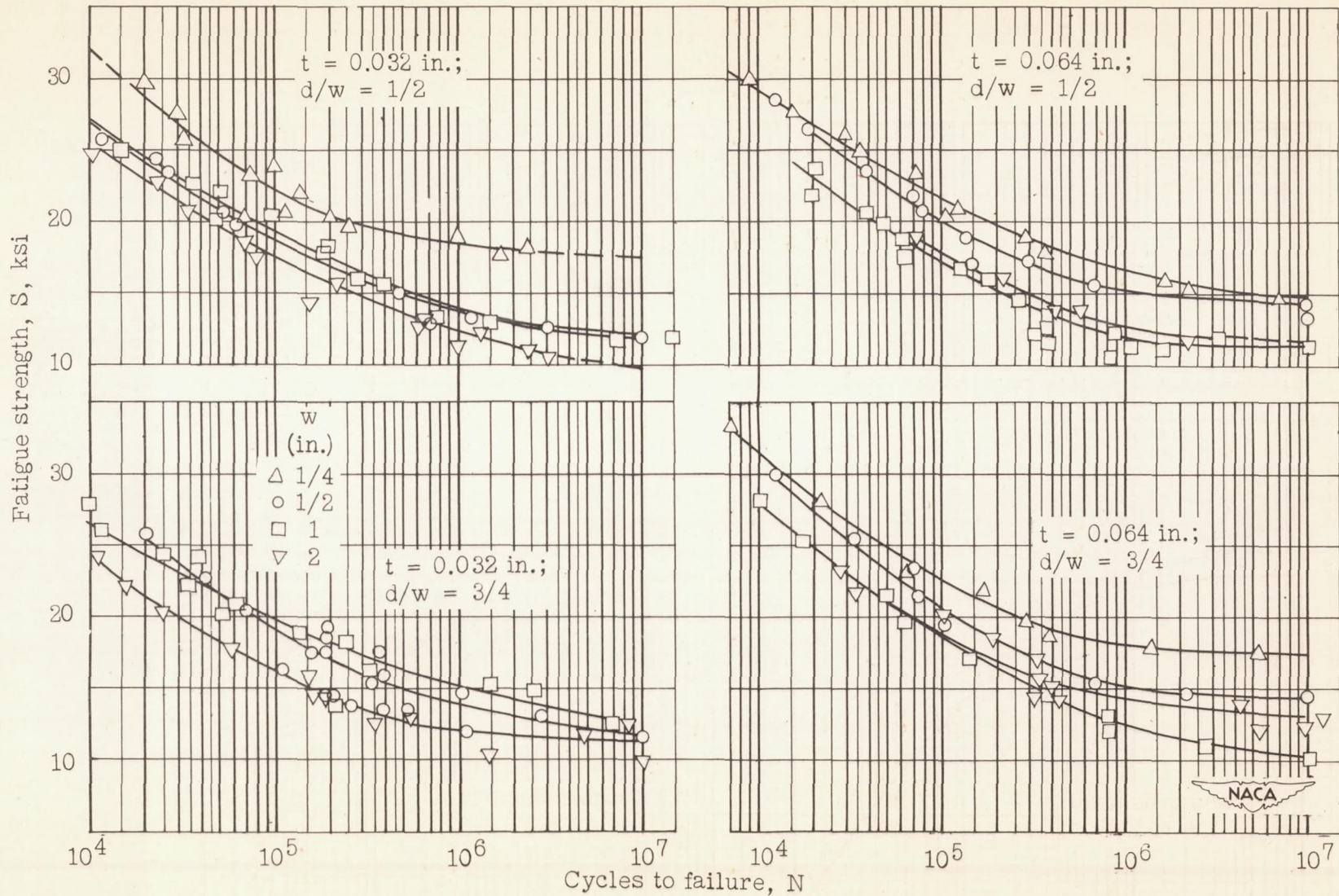
Figure 5.- S-N curves. 24S-T sheet. Specimens having ratio d/w = 1/2 and 3/4 .
