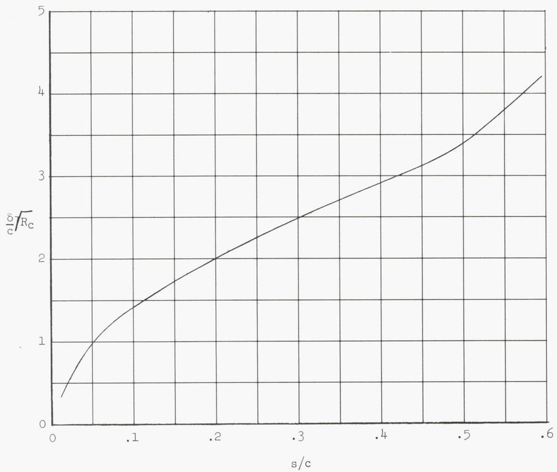
Figure 8.- Nondimensional laminar-boundary-layer thickness distribution for NACA 65(215)-114 airfoil section.
