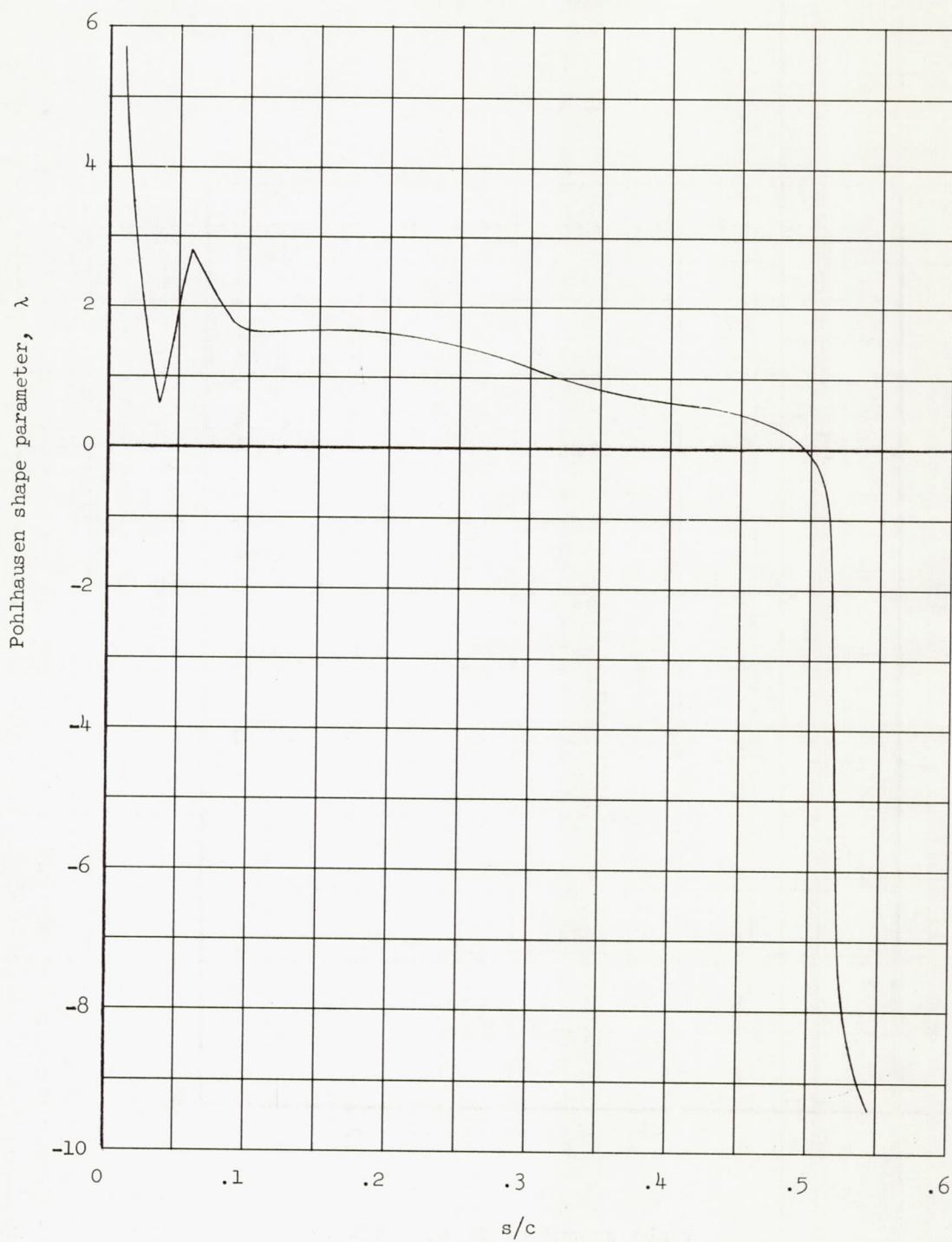
Figure 7.- Pohlhausen shape parameter \lambda for a laminar boundary layer on NACA 65(215)-114 airfoil section at angle of attack of 0^\circ .
