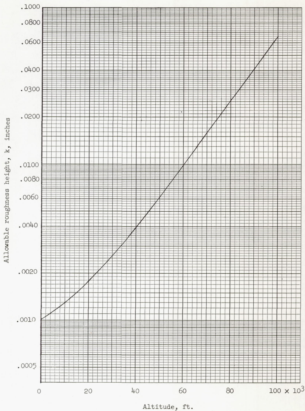
Figure 18.- Allowable roughness height for critical roughness Reynolds number, R_{k,t} of 600, as function of altitude for Mach number of 1.0.
