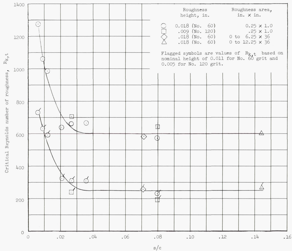
Figure 13.- Roughness Reynolds number for transition on NACA 65(215)-114 airfoil section as a function of roughness location.
