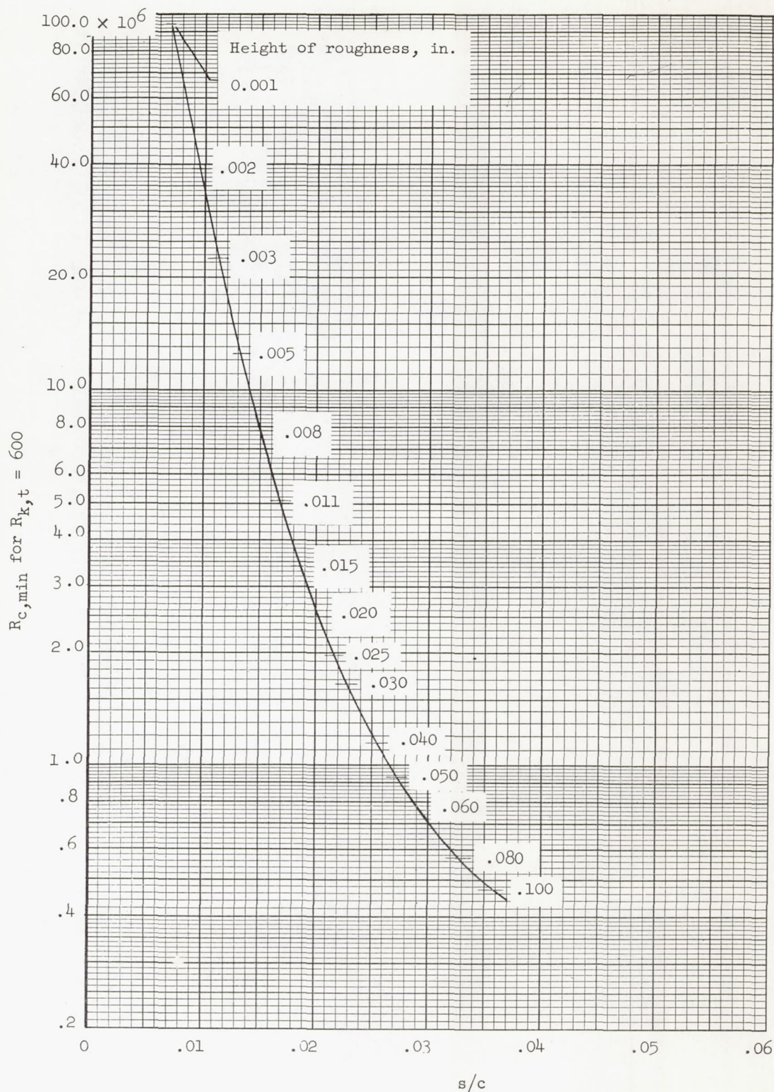
Figure 16.- The theoretical location, for various heights of roughness on an 85-inch-chord NACA 65(215)-114 airfoil section, at which, for a value of R_{k,t} of 600, the airfoil Reynolds number R_c will be a minimum.
