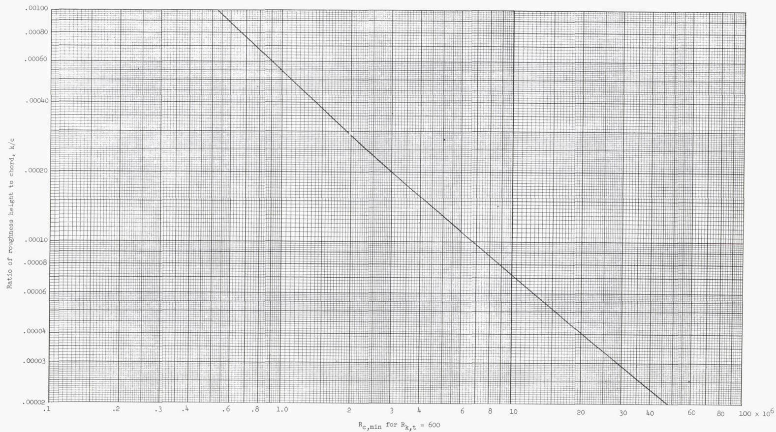
Figure 17.- Variation of the minimum airfoil Reynolds number R_{c,min} , for critical roughness Reynolds number R_{k,t} of 600, with roughness height as calculated for an 85-inch-chord NACA 65(215)-114 airfoil section.
